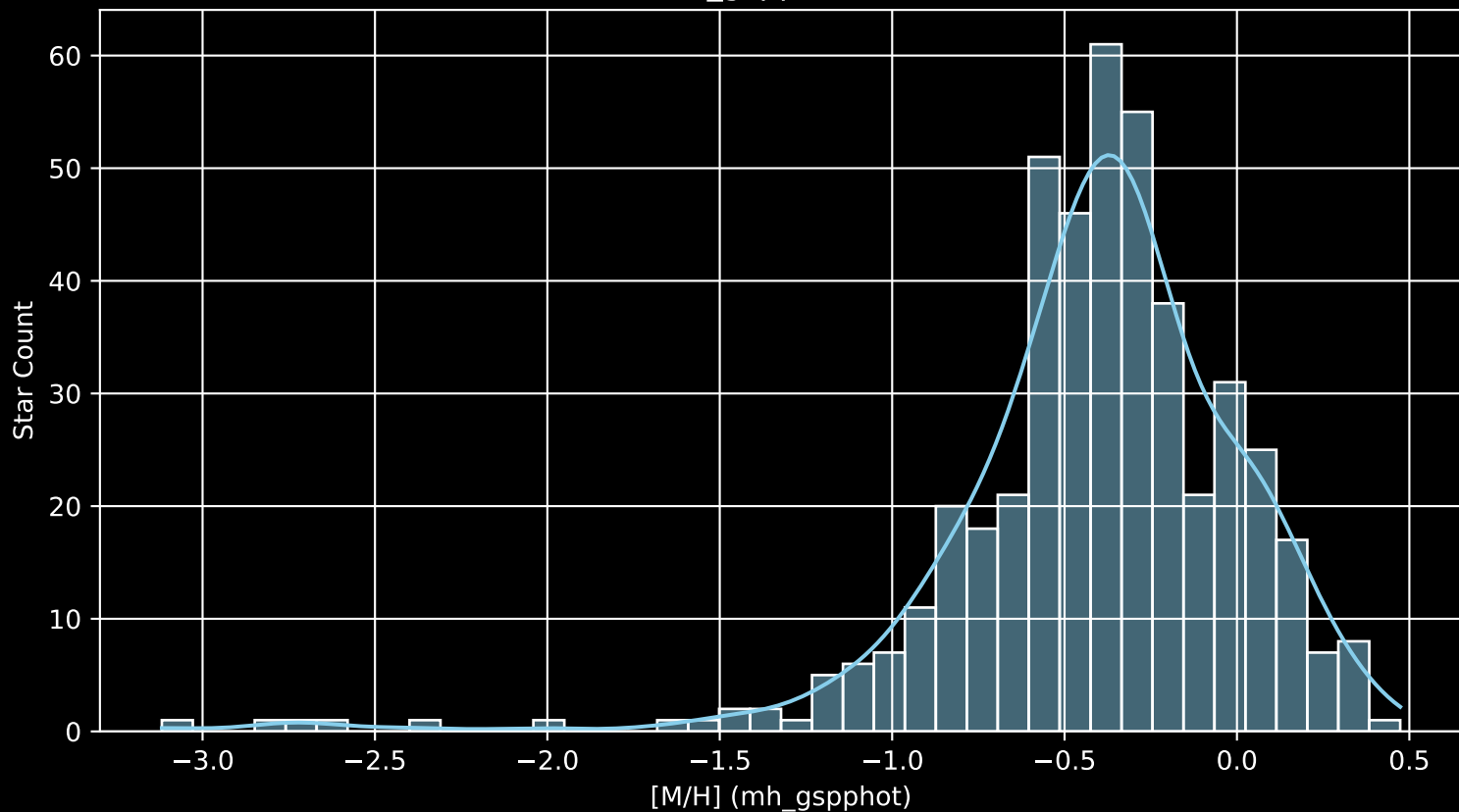
Gaia Cluster: [Collinder_359 [M/H] (mh_gspphot) (n= 462)
