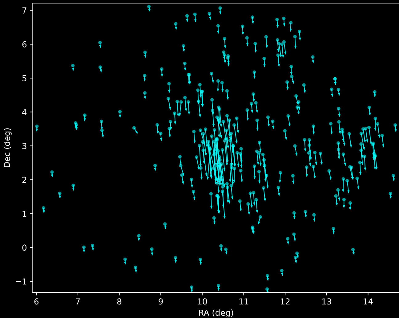
Gaia DR3 Noise Stream Proper Motion Vectors (n=261)
