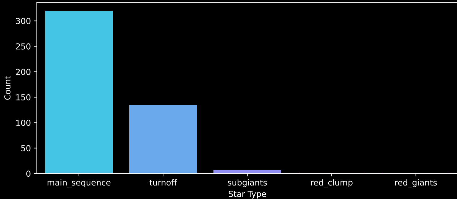
Gaia Cluster: [Collinder_359] Count plot of Star Type
