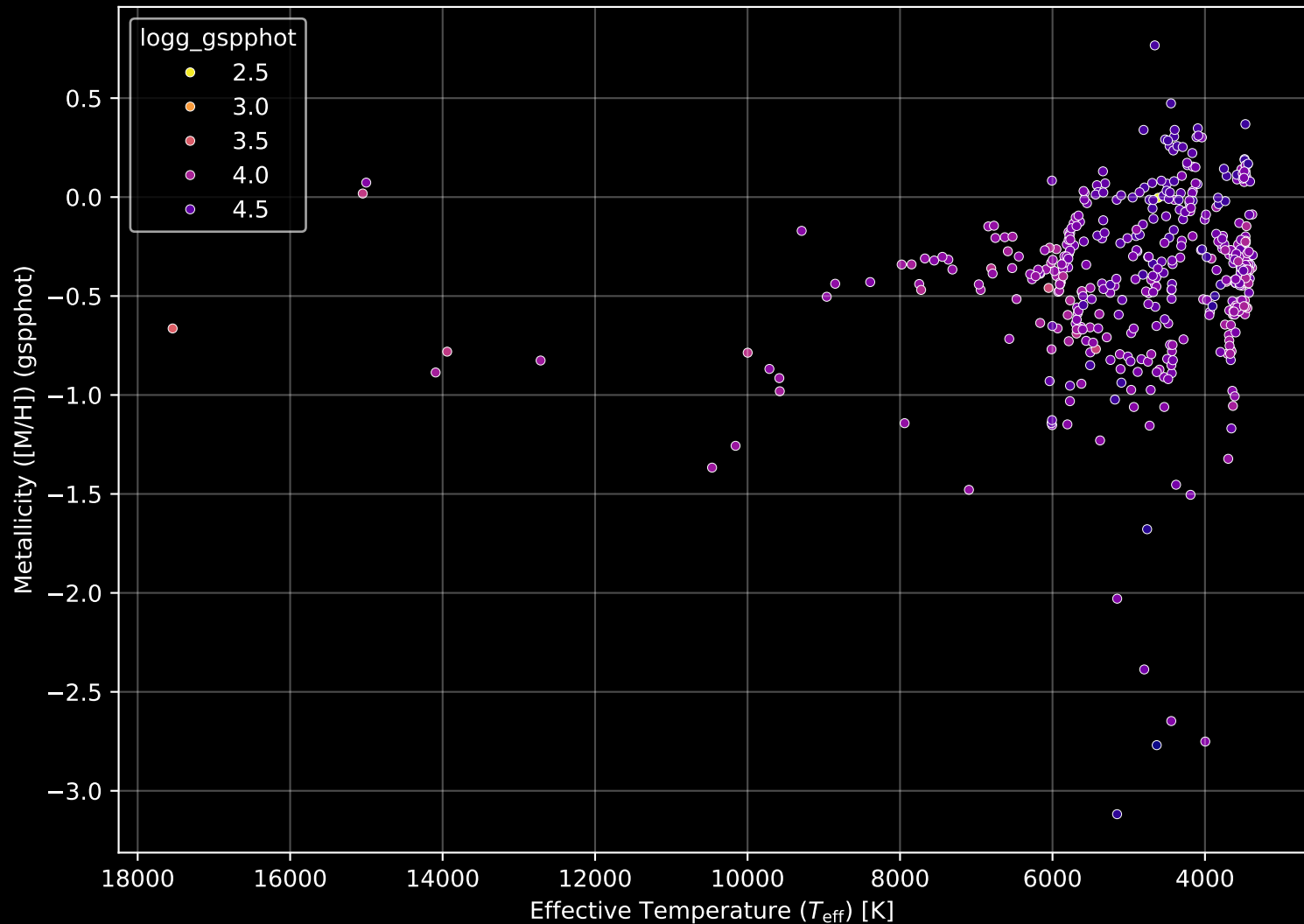
Gaia Cluster: [Collinder_359] Stellar Population Parameters (n= 463)
