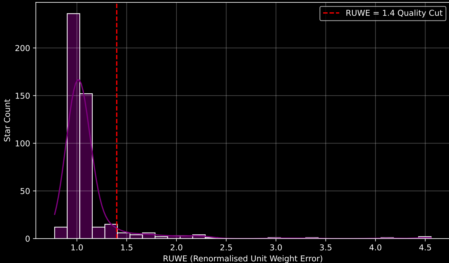
Gaia Cluster: [Collinder_359] RUWE Distribution (n= 461)
