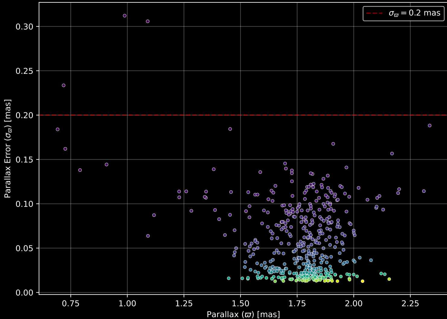
Gaia Cluster: [Collinder_359] Parallax Quality (n= 463)
