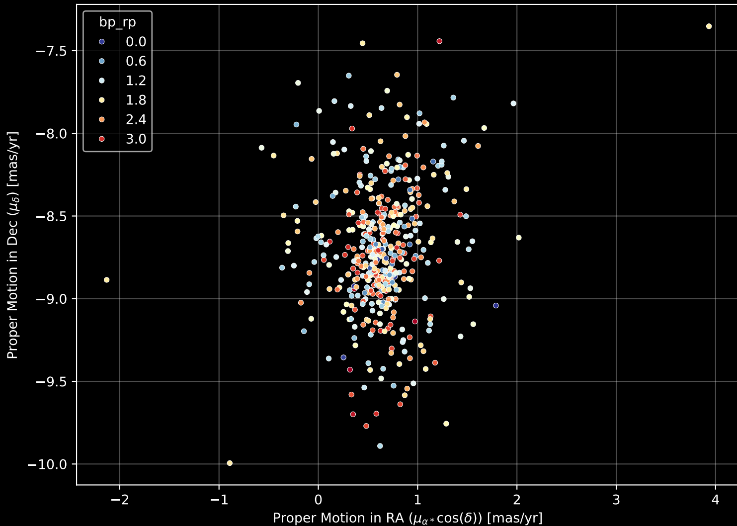
Gaia Cluster: [Collinder_359] Proper Motion Diagram (n= 463)
