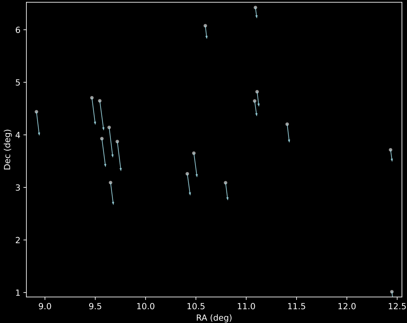
Gaia DR3 Cluster 19 Proper Motion Vectors (n=17)
