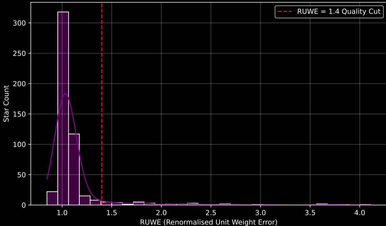
Gaia Cluster: [Collinder_69] RUWE Distribution (n= 513)
