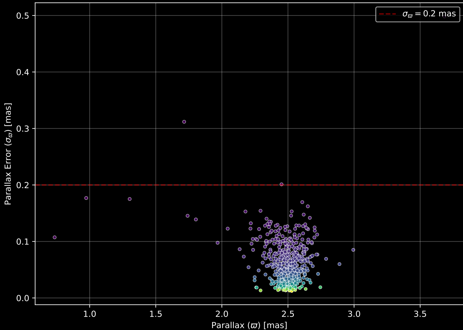
Gaia Cluster: [Collinder_69] Parallax Quality (n= 518)
