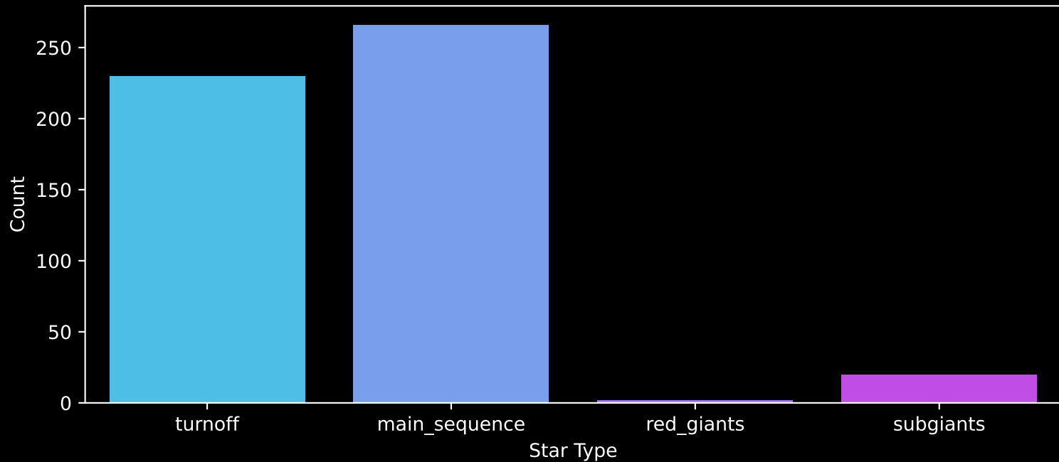
Gaia Cluster: [Collinder_69] Count plot of Star Type
