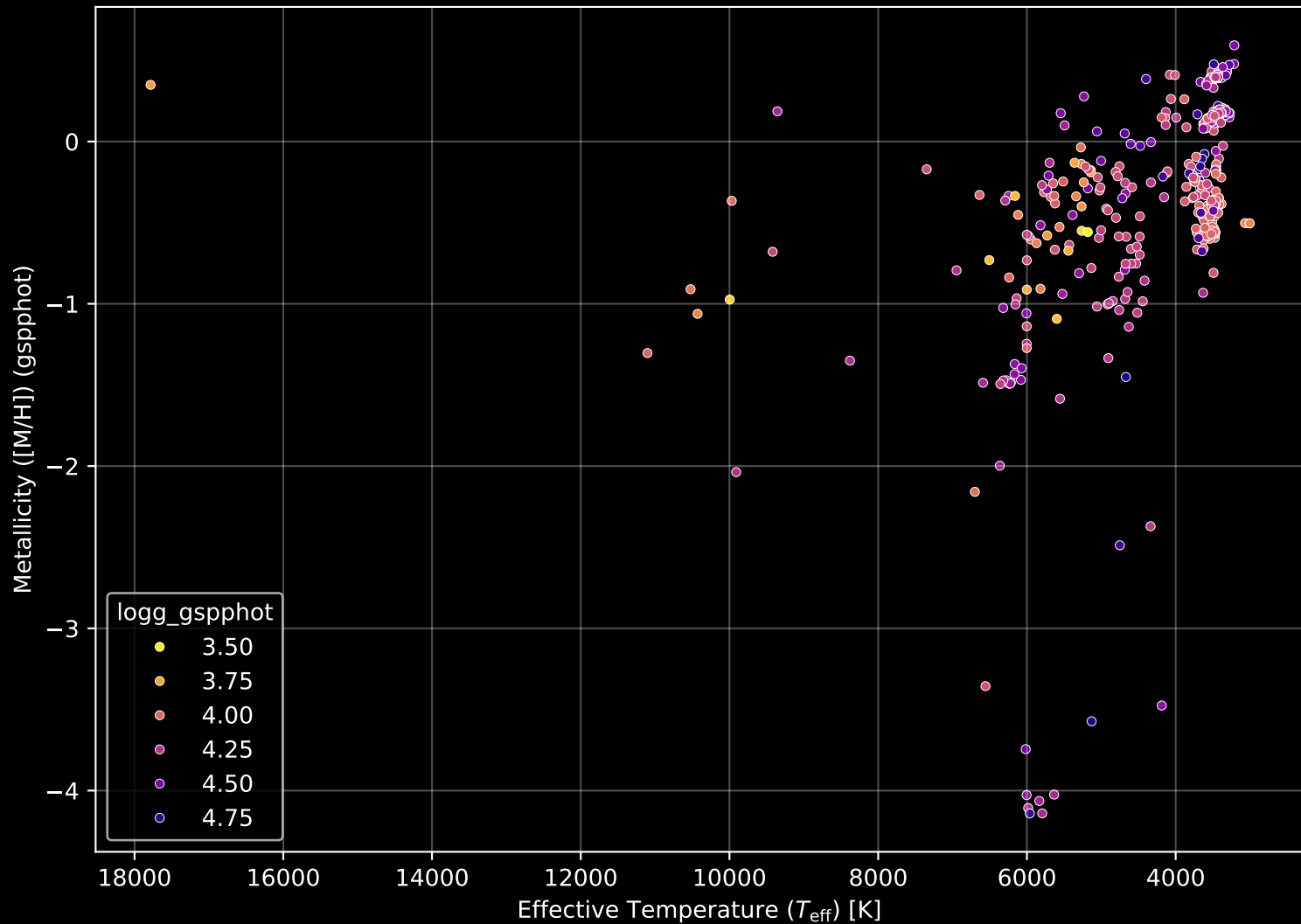
Gaia Cluster: [Collinder_69] Stellar Population Parameters (n= 518)
