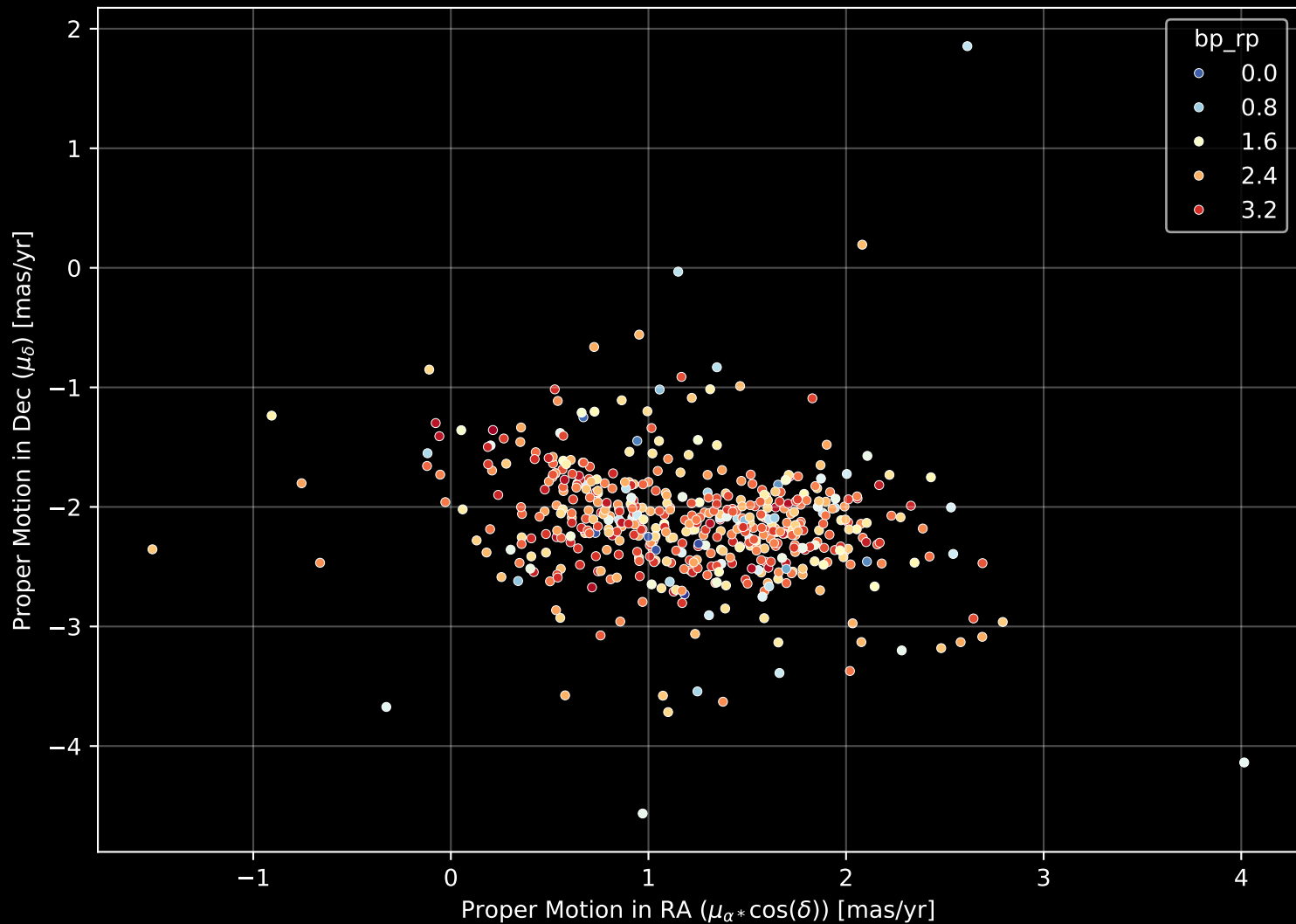
Gaia Cluster: [Collinder_69] Proper Motion Diagram (n= 518)
