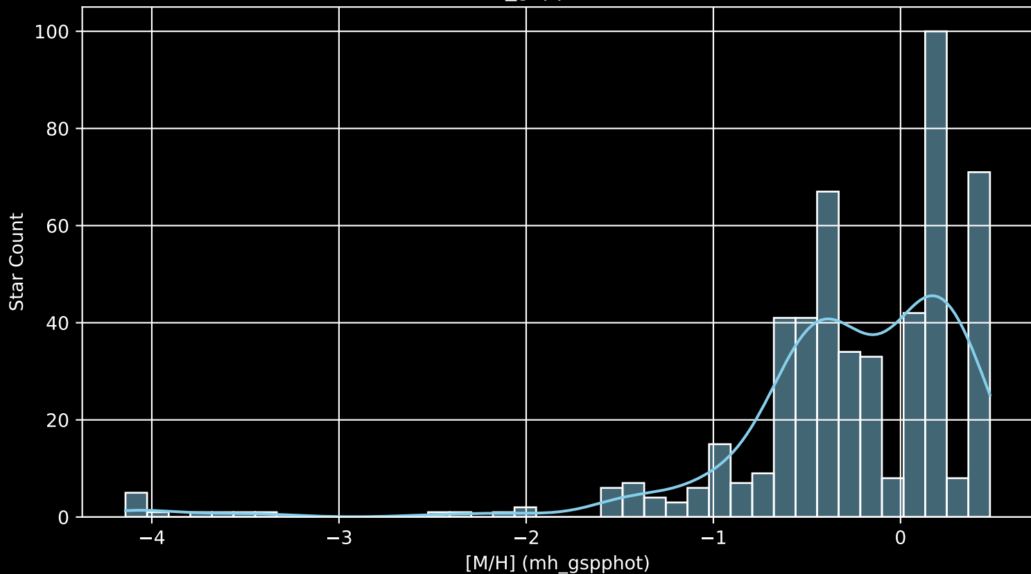
Gaia Cluster: [Collinder_69 [M/H] (mh_gspphot) (n= 517)
