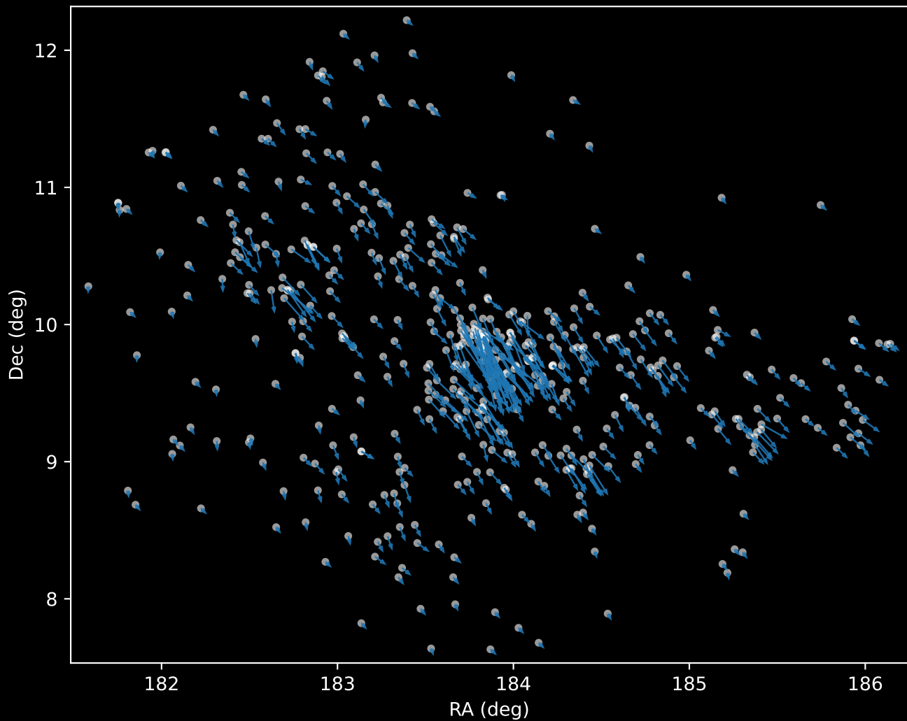
Gaia DR3 Cluster 0 Proper Motion Vectors (n=488)
