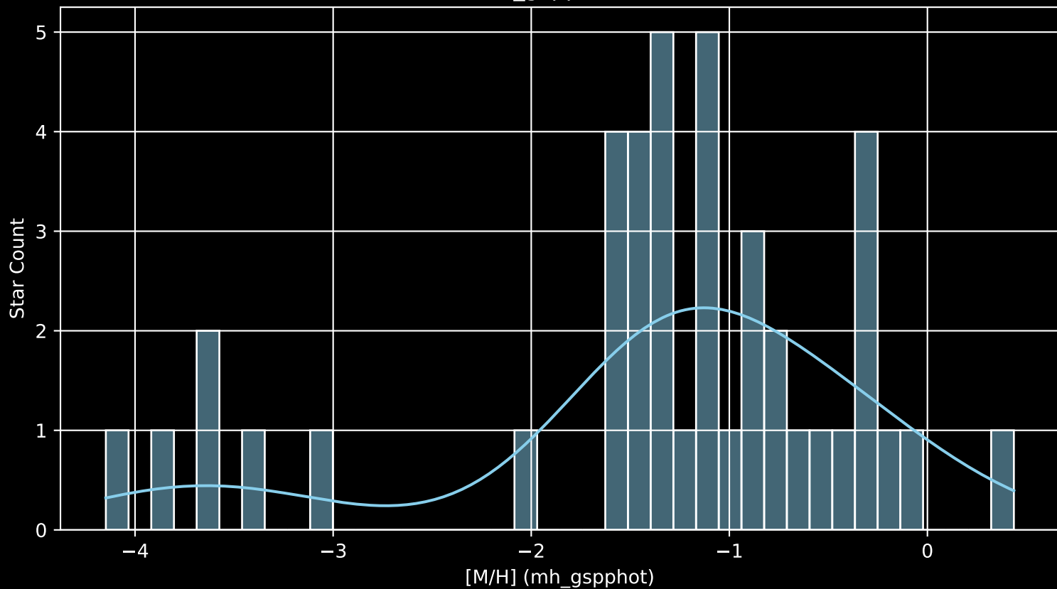
Gaia Cluster: [Czernik_1 [M/H] (mh_gspphot) (n= 42)
