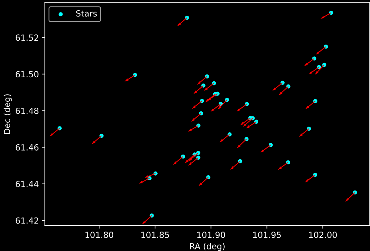
Gaia Cluster: [Czernik_1] Proper Motion Vectors for Gaia Star Field (n= 42)
