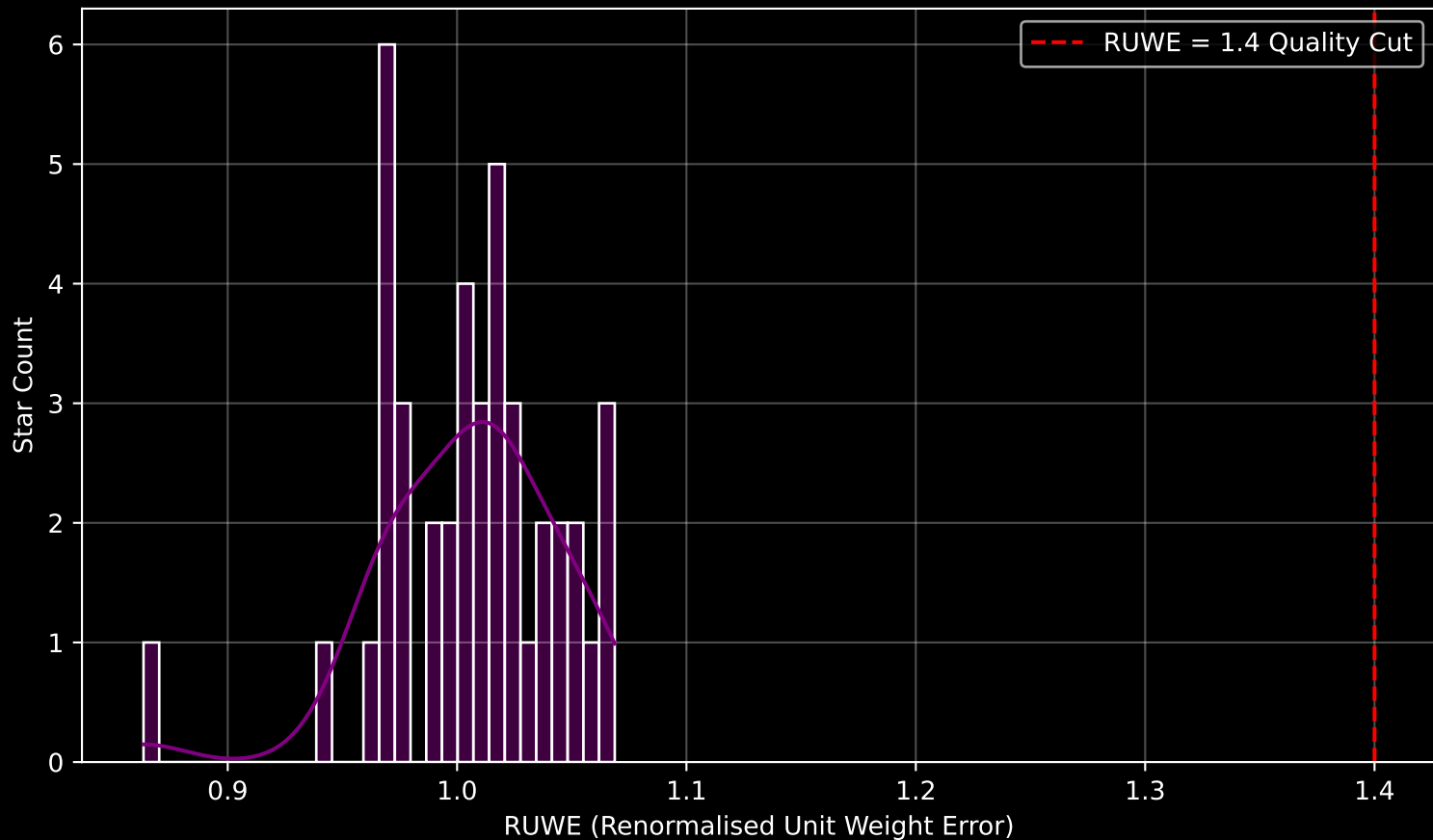
Gaia Cluster: [Czernik_1] RUWE Distribution (n= 42)
