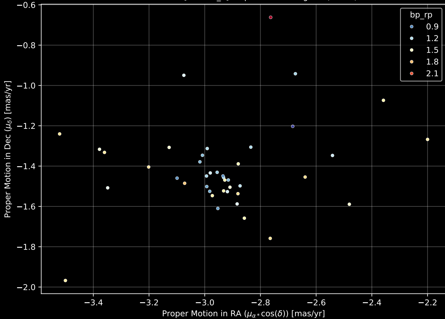
Gaia Cluster: [Czernik_1] Proper Motion Diagram (n= 42)
