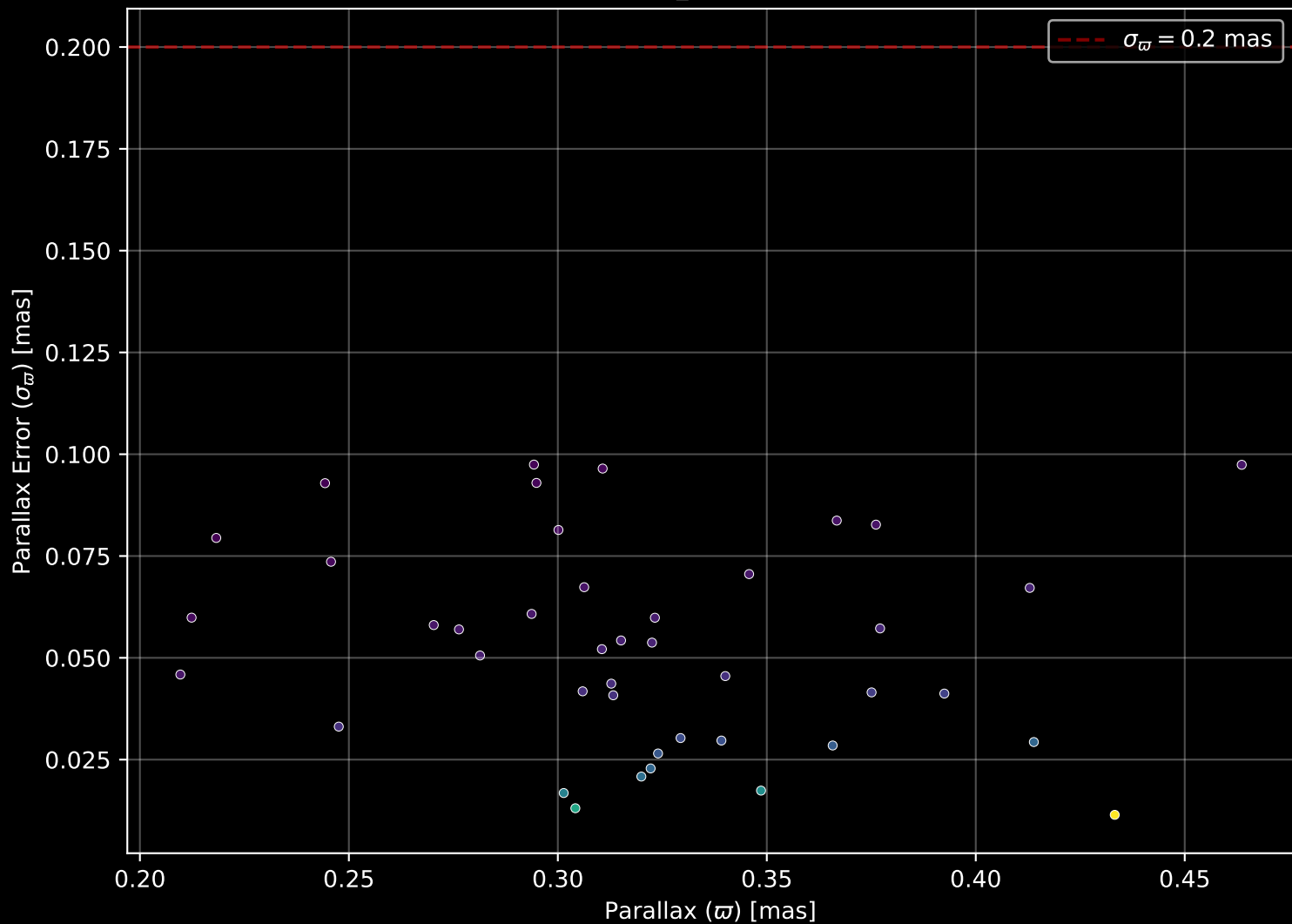
Gaia Cluster: [Czernik_1] Parallax Quality (n= 42)
