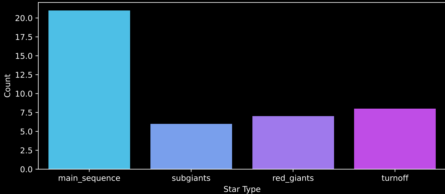
Gaia Cluster: [Czernik_1] Count plot of Star Type
