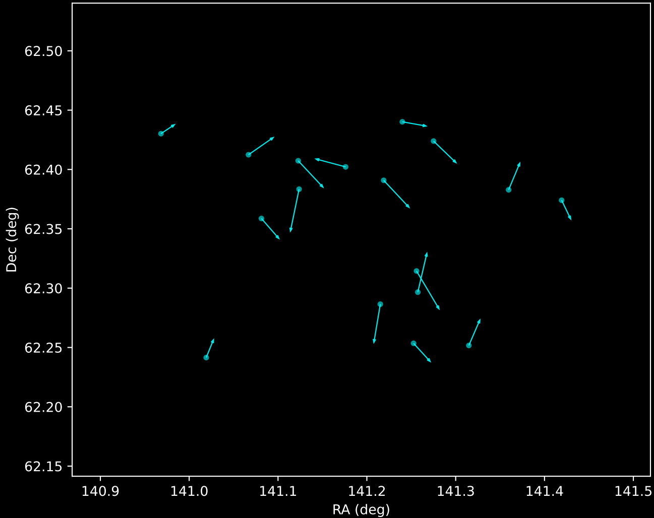
Gaia DR3 Noise Stream Proper Motion Vectors (n=17)
