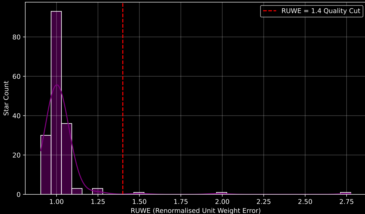
Gaia Cluster: [Czernik_13] RUWE Distribution (n= 168)
