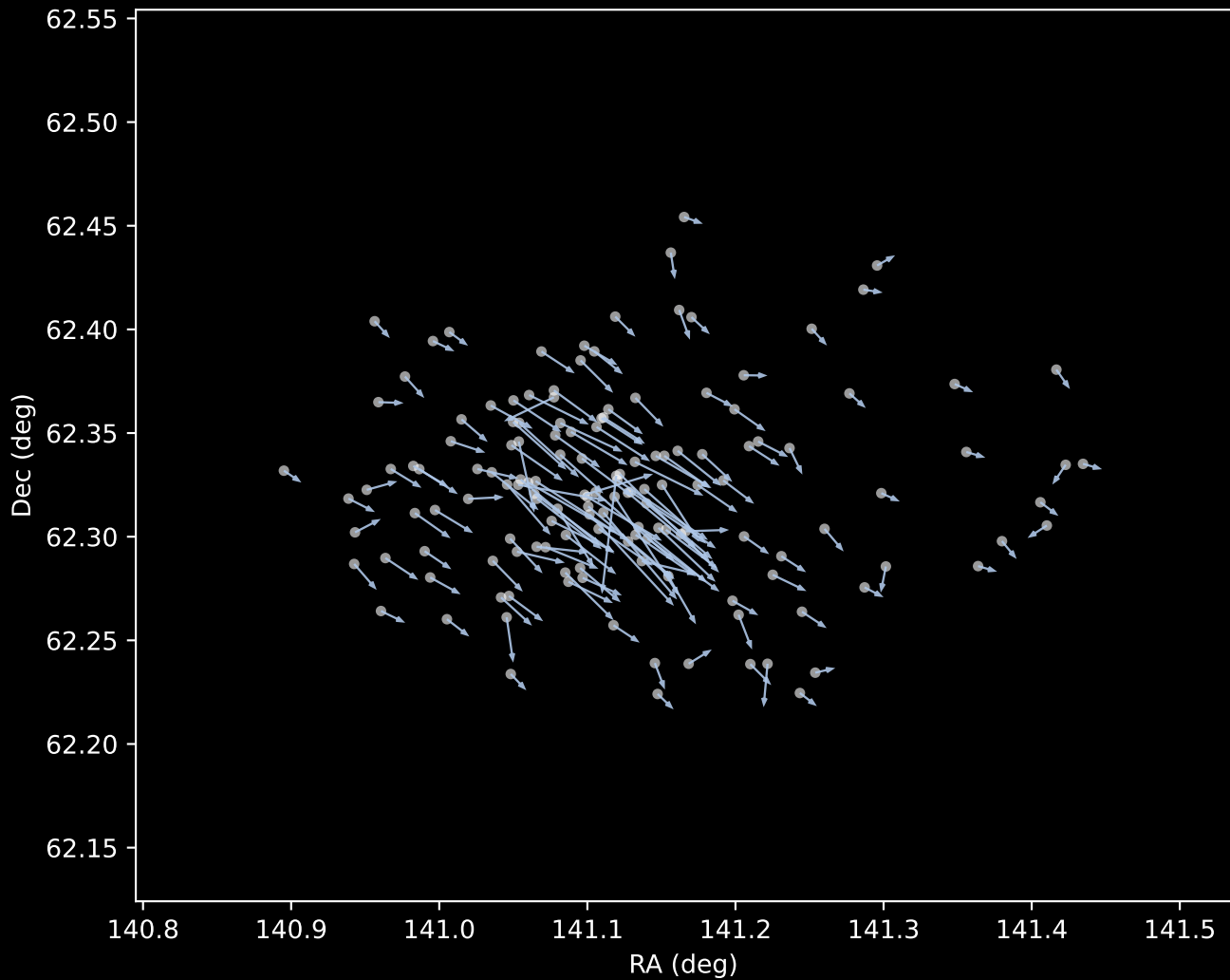
Gaia DR3 Cluster 1 Proper Motion Vectors (n=146)
