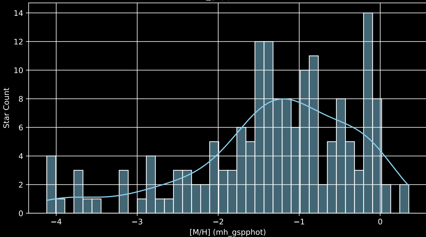
Gaia Cluster: [Czernik_13 [M/H] (mh_gspphot) (n= 168)
