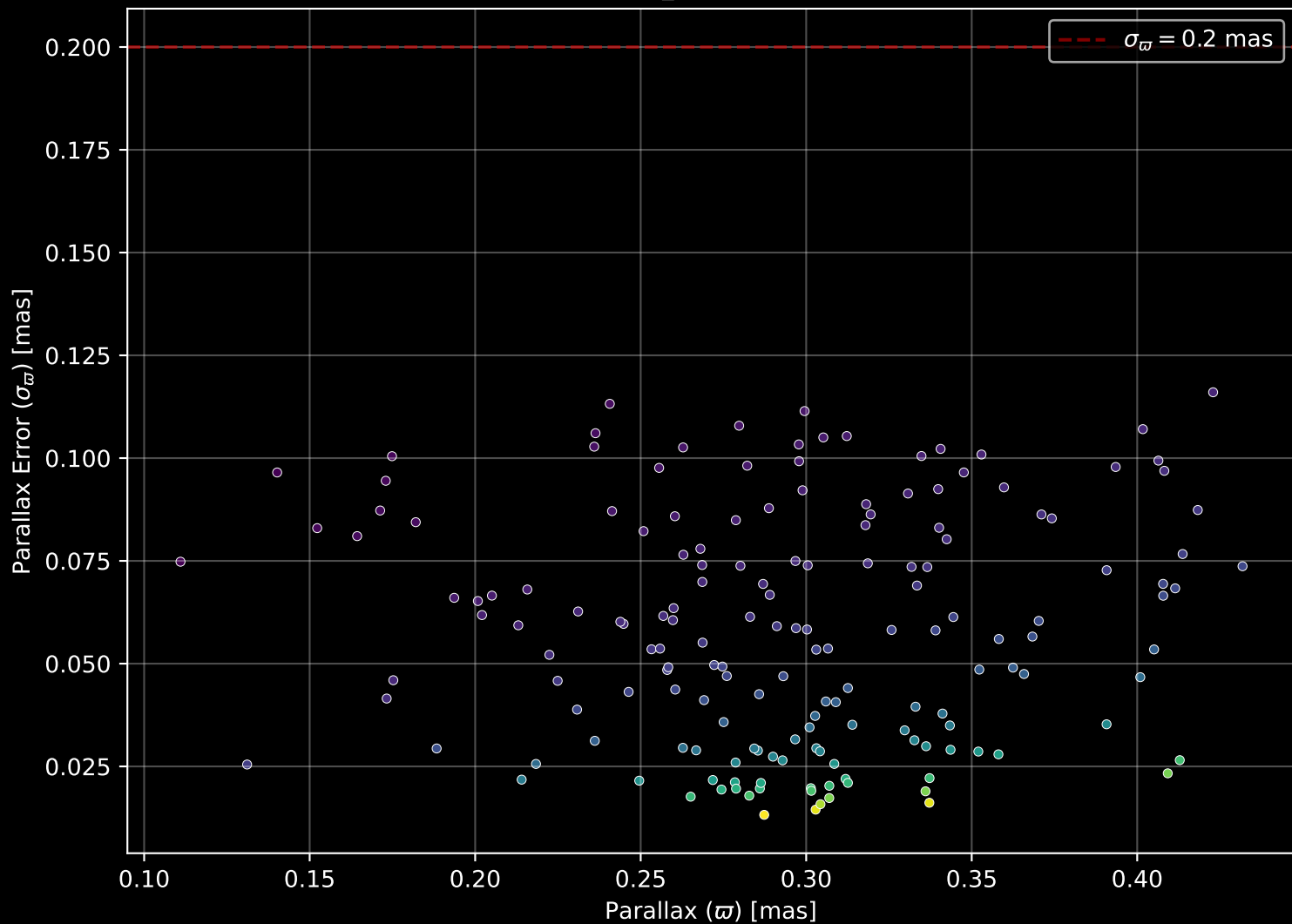
Gaia Cluster: [Czernik_13] Parallax Quality (n= 168)
