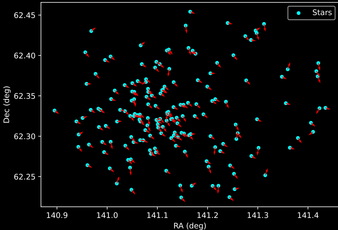
Gaia Cluster: [Czernik_13] Proper Motion Vectors for Gaia Star Field (n= 168)
