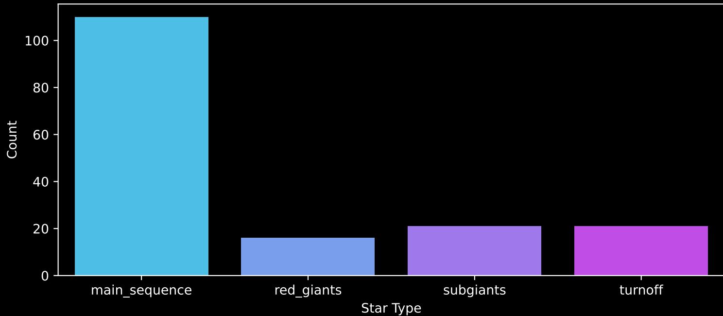
Gaia Cluster: [Czernik_13] Count plot of Star Type
