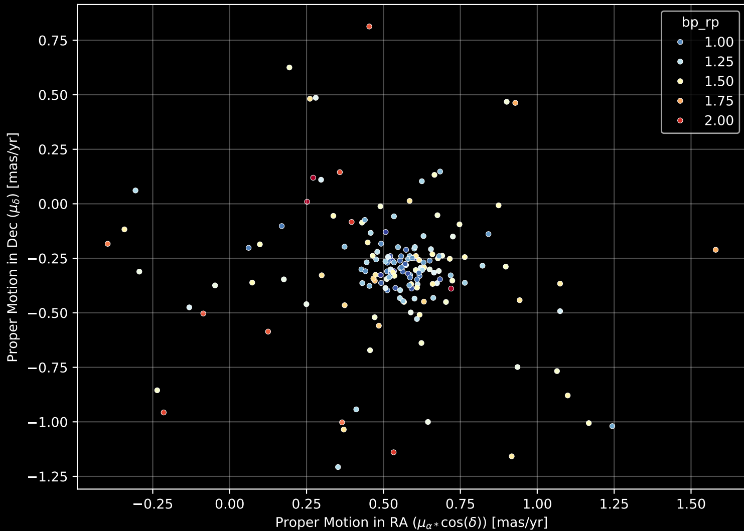
Gaia Cluster: [Czernik_13] Proper Motion Diagram (n= 168)
