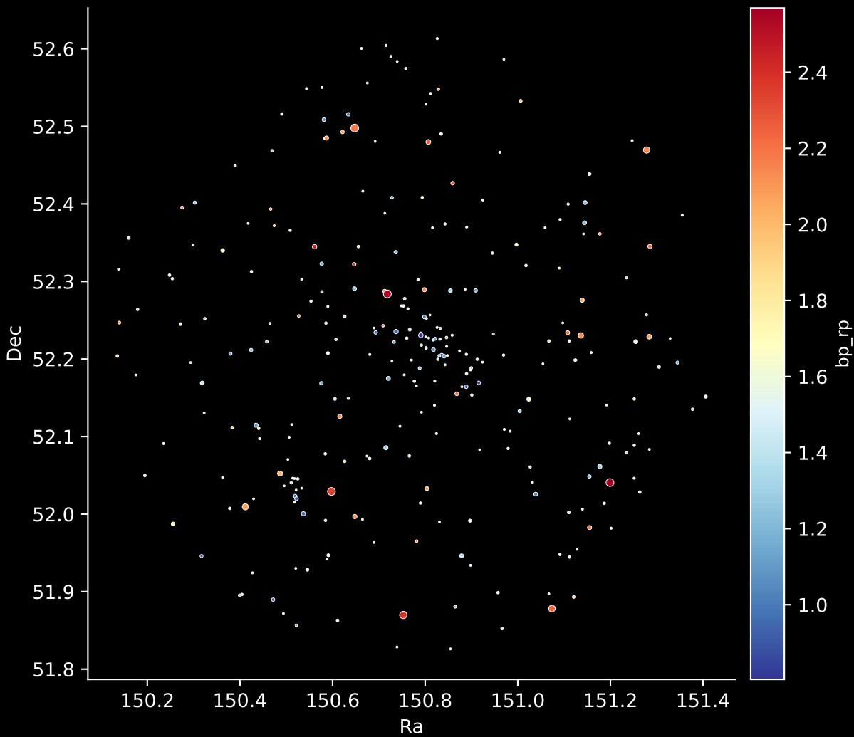
Gaia Cluster: [Czernik_15] Stars: 281
