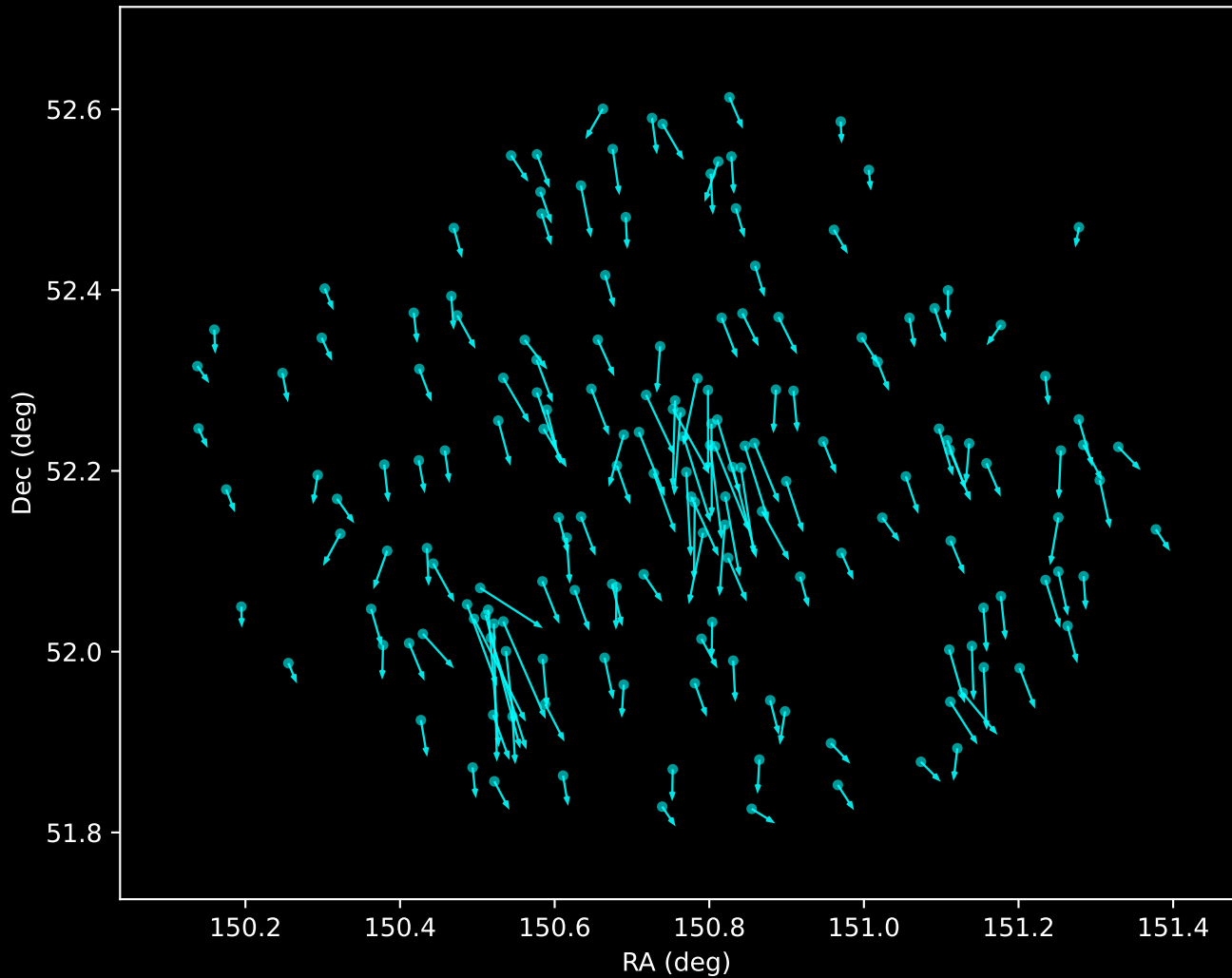
Gaia DR3 Noise Stream Proper Motion Vectors (n=169)
