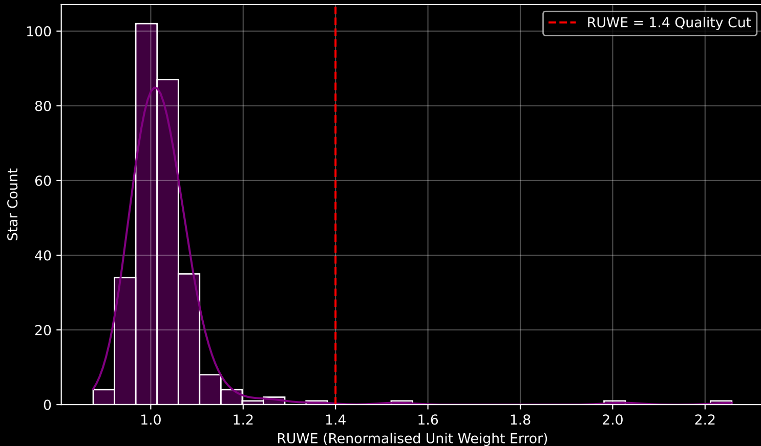
Gaia Cluster: [Czernik_15] RUWE Distribution (n= 281)
