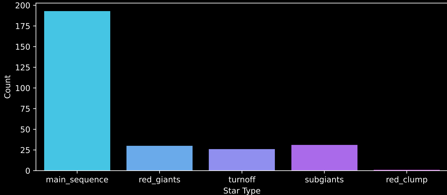
Gaia Cluster: [Czernik_15] Count plot of Star Type
