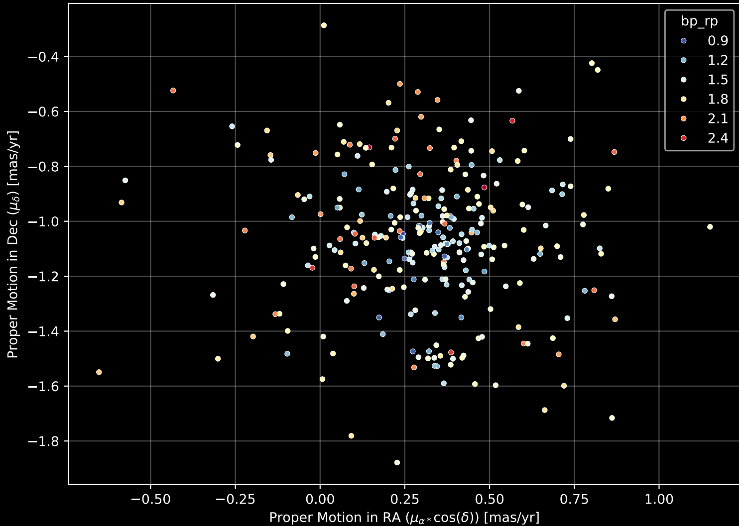
Gaia Cluster: [Czernik_15] Proper Motion Diagram (n= 281)
