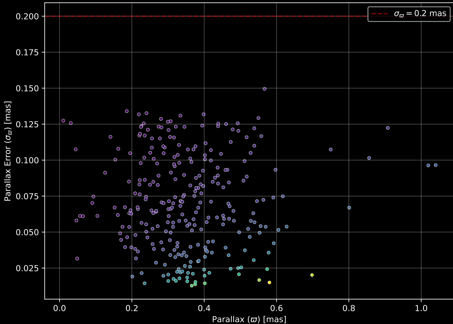
Gaia Cluster: [Czernik_15] Parallax Quality (n= 281)
