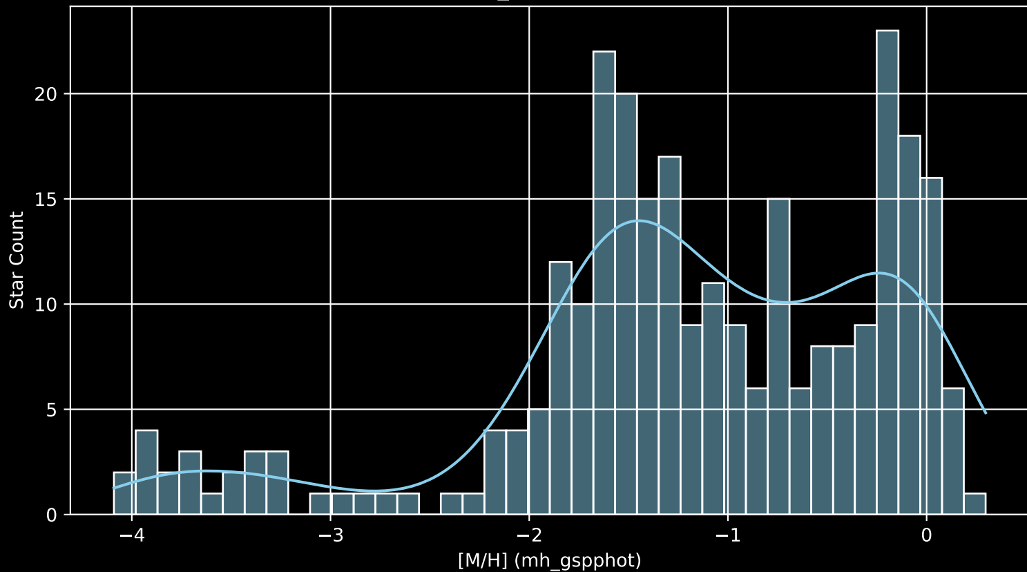
Gaia Cluster: [Czernik_15 [M/H] (mh_gspphot) (n= 281)
