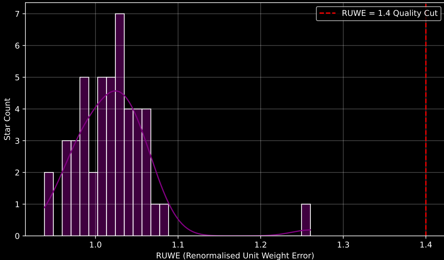
Gaia Cluster: [Czernik_16] RUWE Distribution (n= 47)
