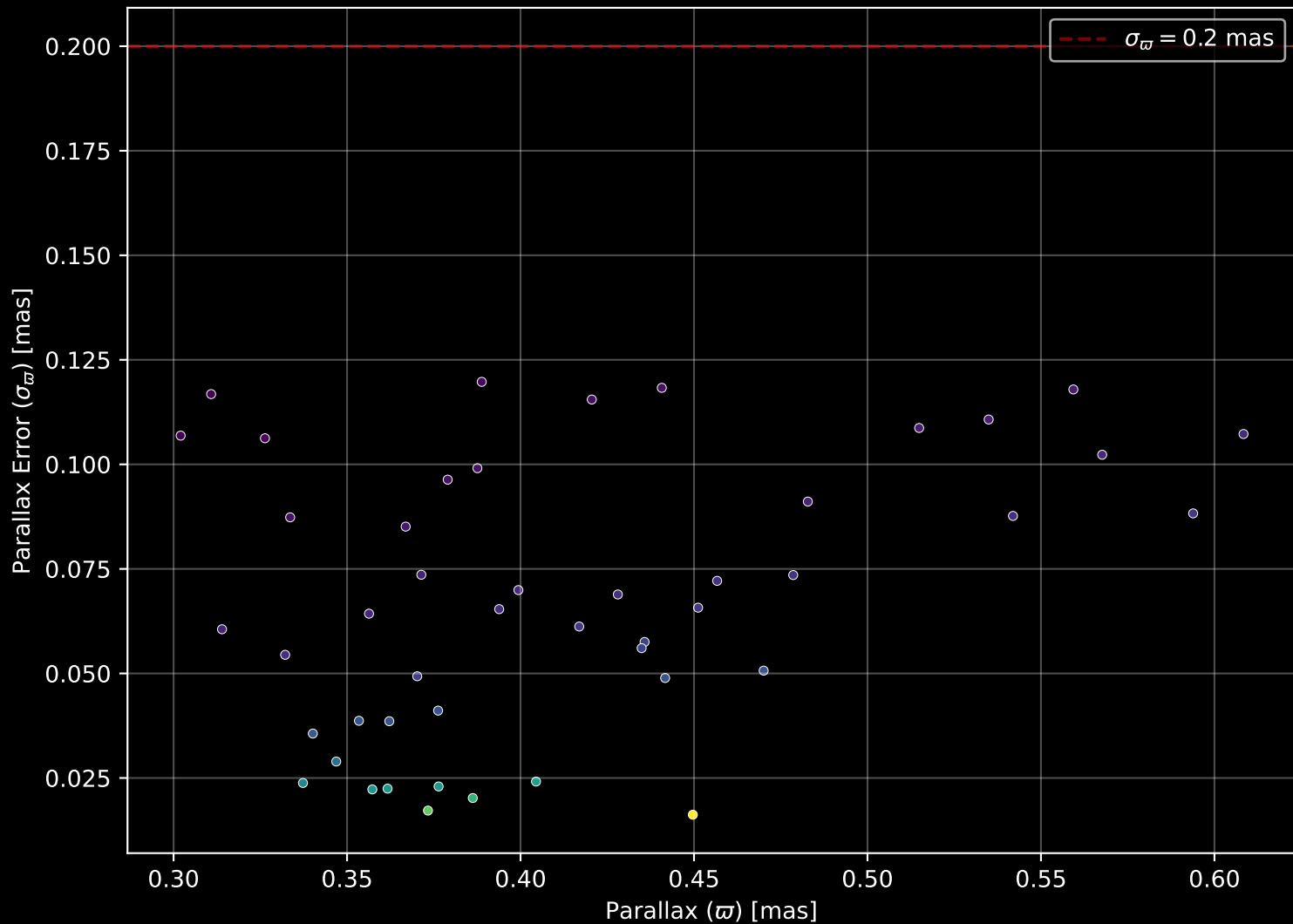
Gaia Cluster: [Czernik_16] Parallax Quality (n= 47)
