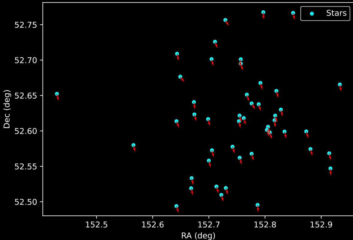
Gaia Cluster: [Czernik_16] Proper Motion Vectors for Gaia Star Field (n= 47)
