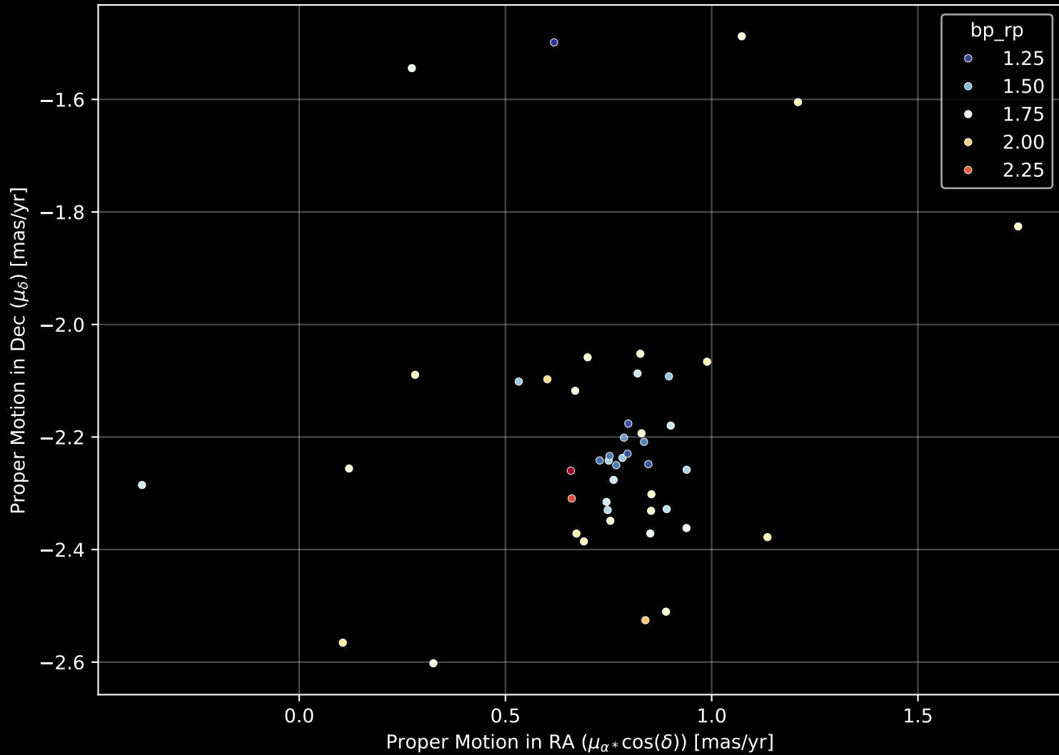
Gaia Cluster: [Czernik_16] Proper Motion Diagram (n= 47)
