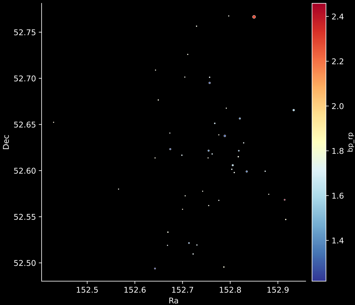
Gaia Cluster: [Czernik_16] Stars: 47
