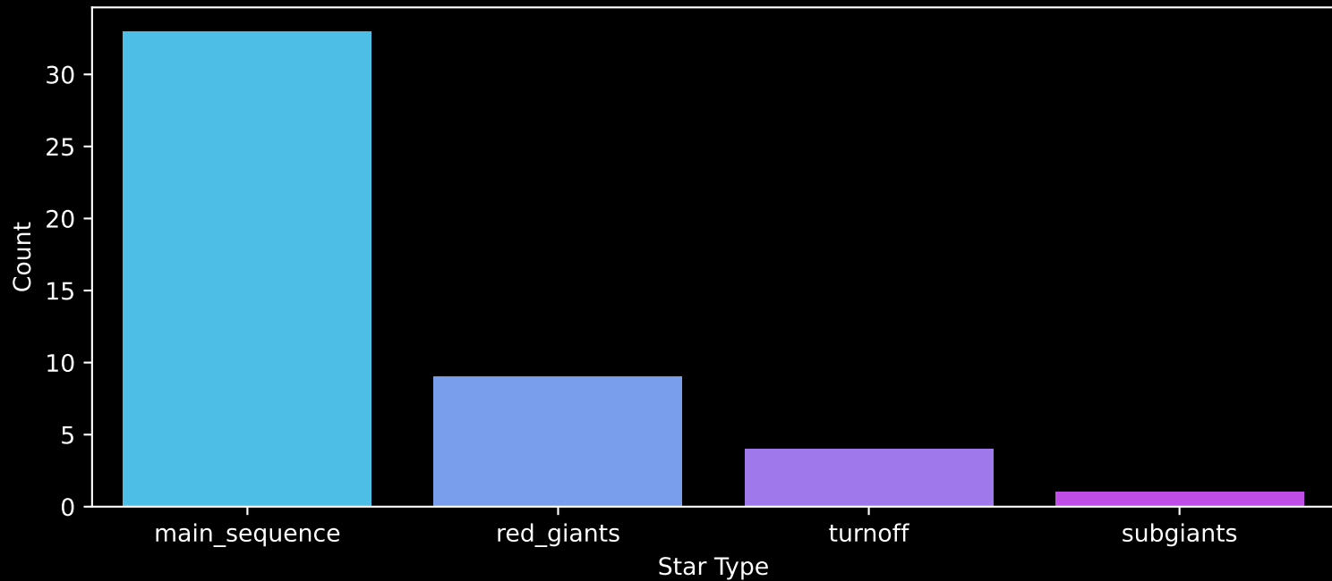
Gaia Cluster: [Czernik_16] Count plot of Star Type
