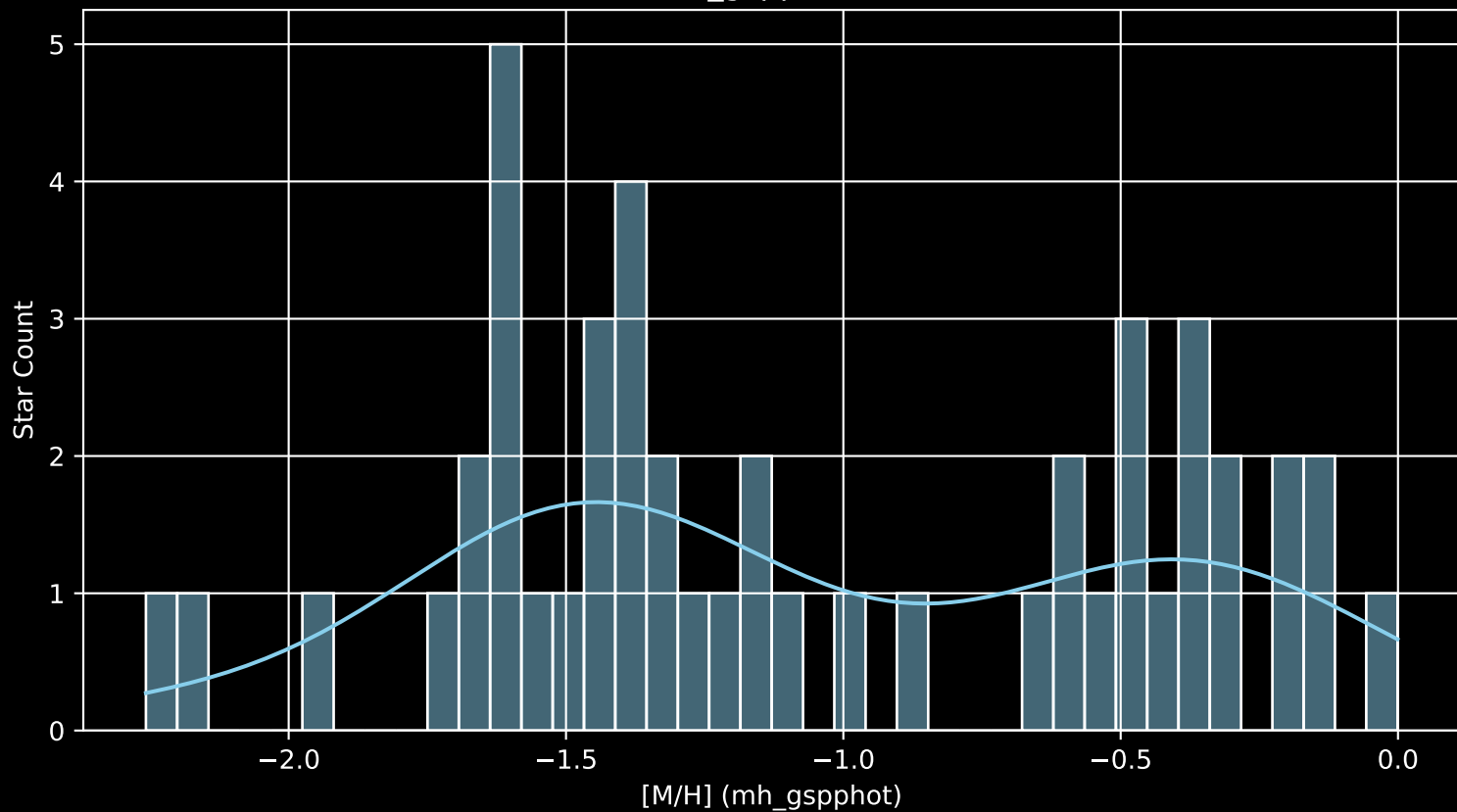
Gaia Cluster: [Czernik_16 [M/H] (mh_gspphot) (n= 47)
