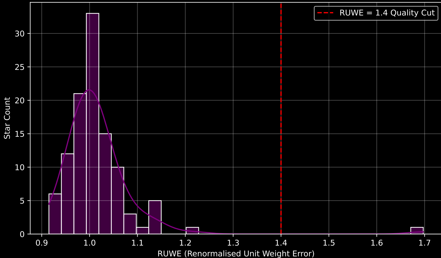
Gaia Cluster: [Czernik_2] RUWE Distribution (n= 108)
