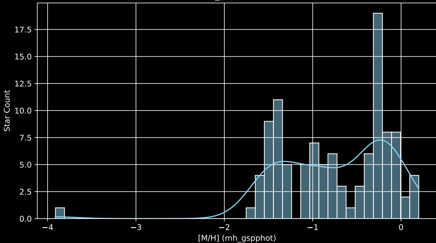
Gaia Cluster: [Czernik_2 [M/H] (mh_gspphot) (n=108)
