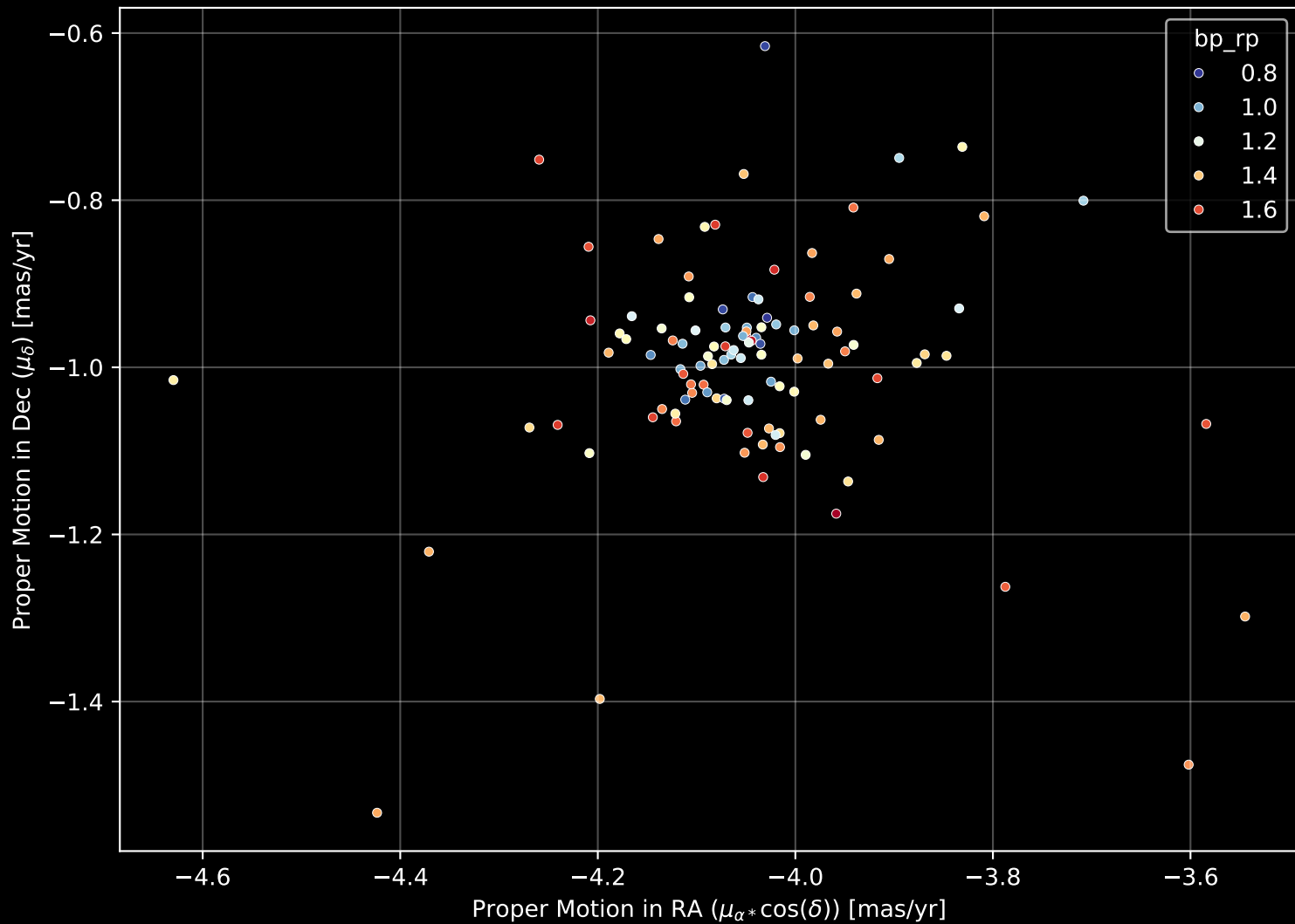
Gaia Cluster: [Czernik_2] Proper Motion Diagram (n= 108)
