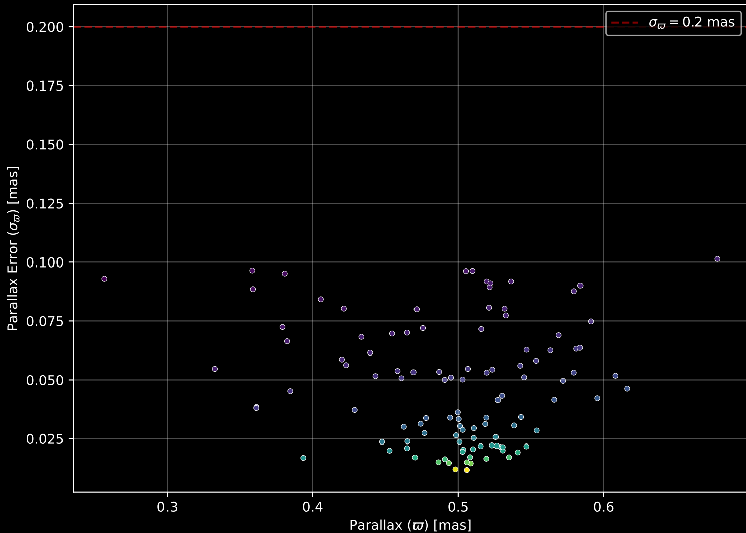
Gaia Cluster: [Czernik_2] Parallax Quality (n= 108)
