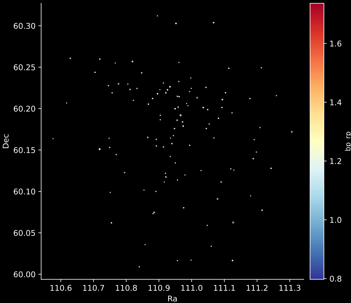
Gaia Cluster: [Czernik_2] Stars: 108
