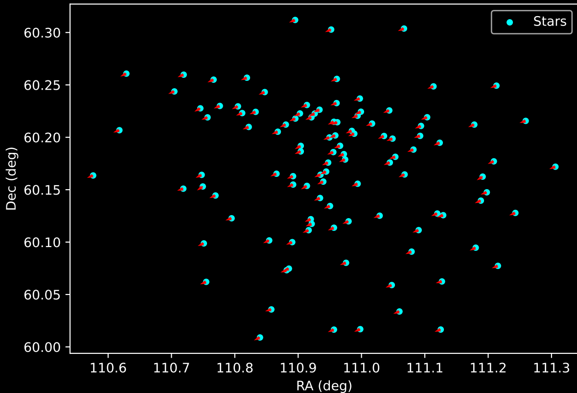
Gaia Cluster: [Czernik_2] Proper Motion Vectors for Gaia Star Field (n= 108)
