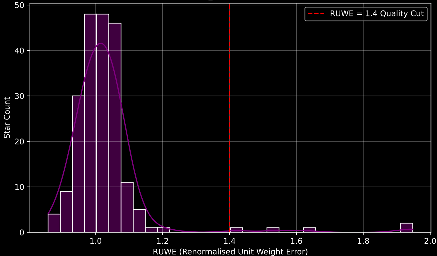
Gaia Cluster: [Czernik_24] RUWE Distribution (n= 208)
