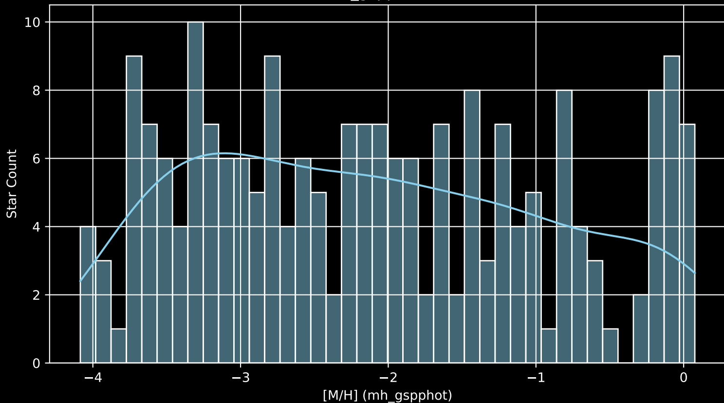
Gaia Cluster: [Czernik_24 [M/H] (mh_gspphot) (n= 208)
