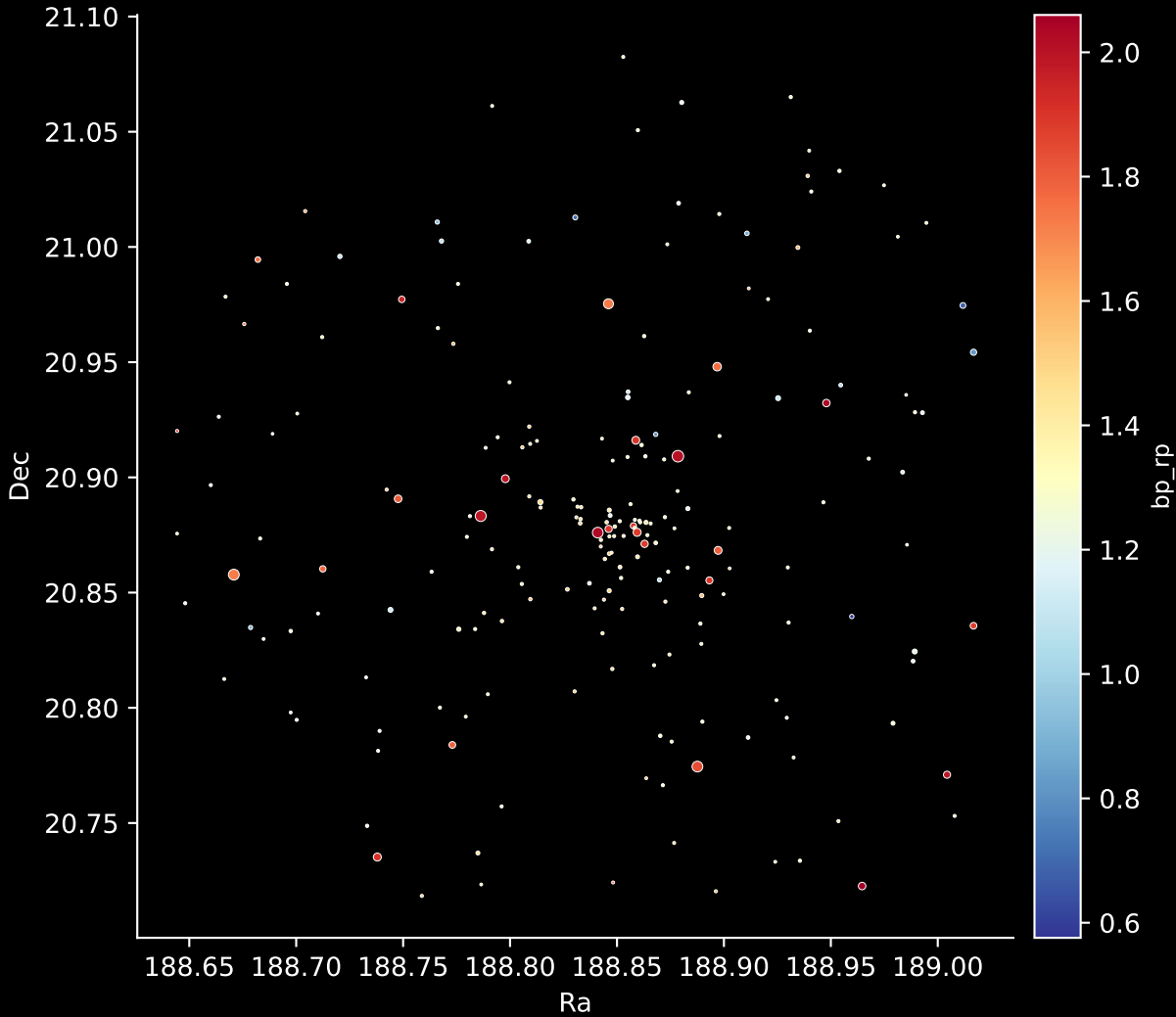
Gaia Cluster: [Czernik_24] Stars: 208
