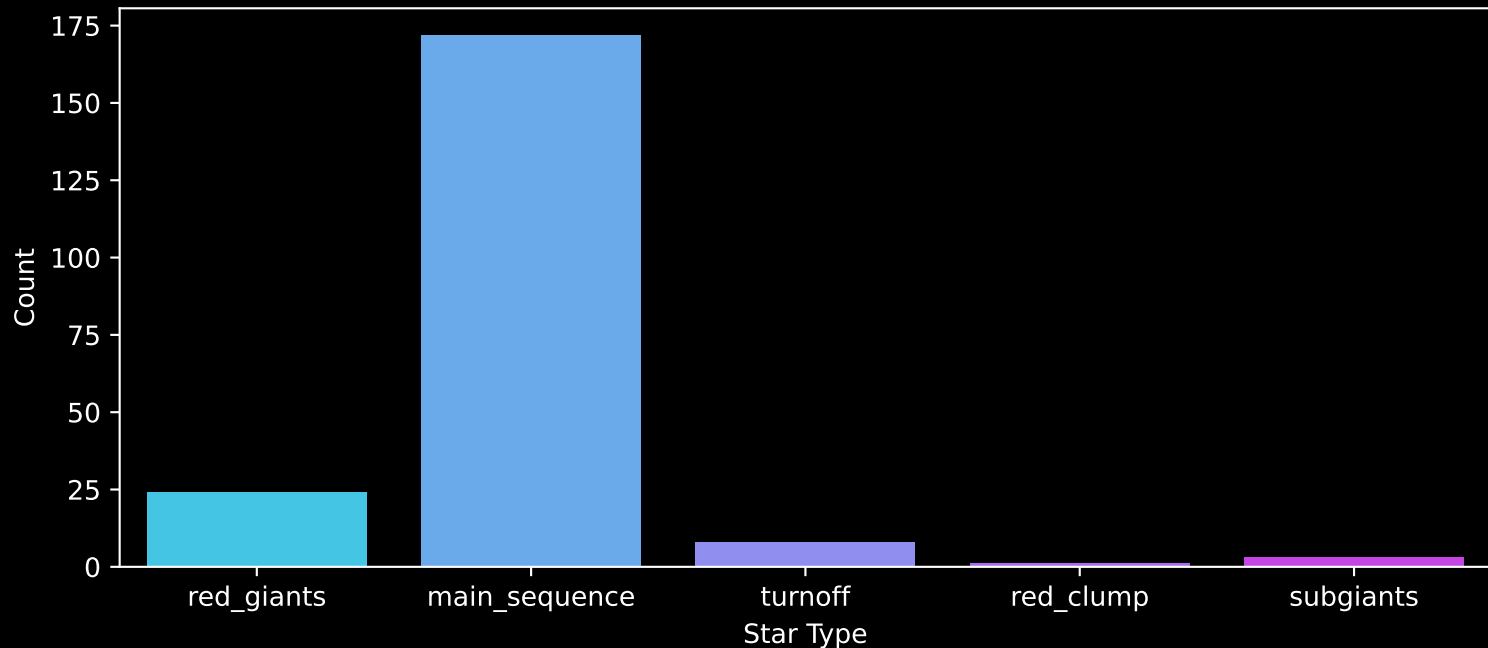
Gaia Cluster: [Czernik_24] Count plot of Star Type
