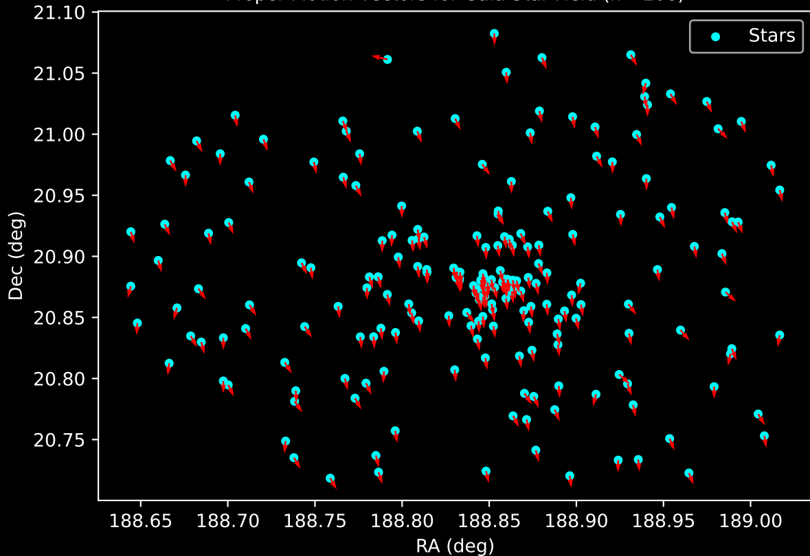
Gaia Cluster: [Czernik_24] Proper Motion Vectors for Gaia Star Field (n= 208)
