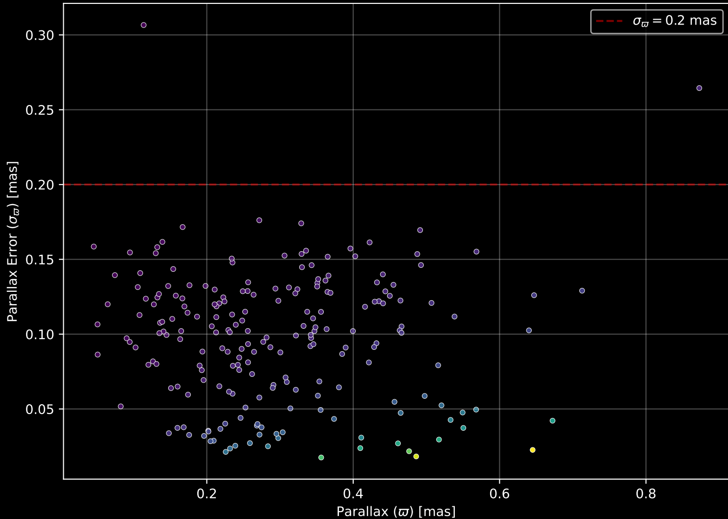
Gaia Cluster: [Czernik_24] Parallax Quality (n= 208)
