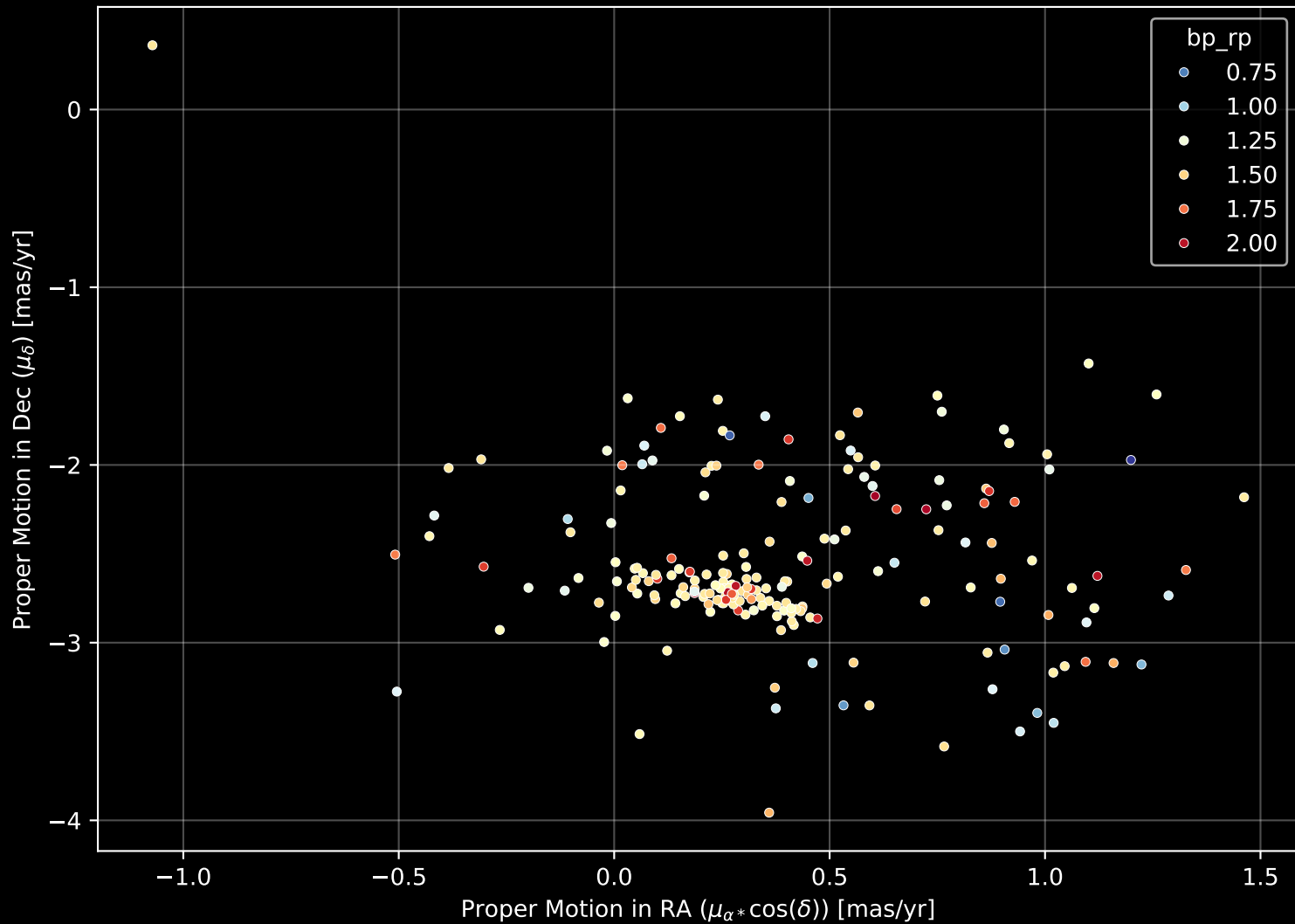
Gaia Cluster: [Czernik_24] Proper Motion Diagram (n= 208)
