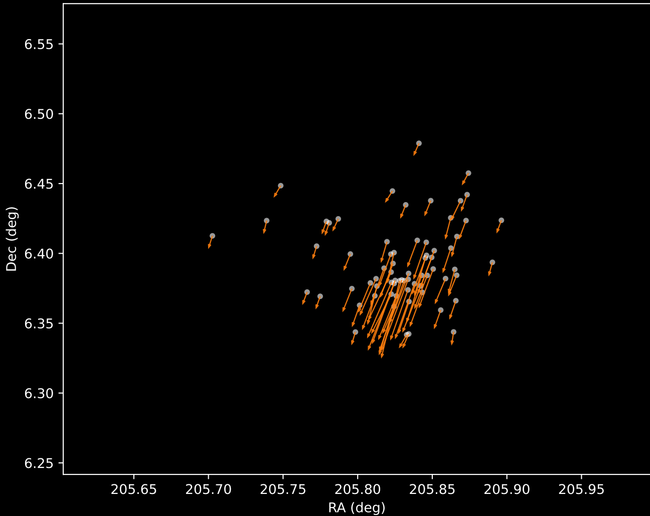
Gaia DR3 Cluster 2 Proper Motion Vectors (n=69)
