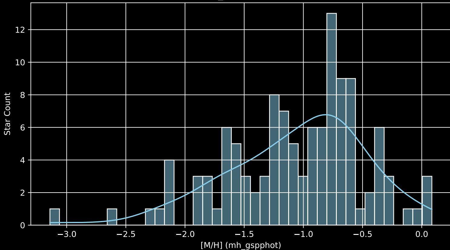
Gaia Cluster: [Czernik_27 [M/H] (mh_gspphot) (n= 117)
