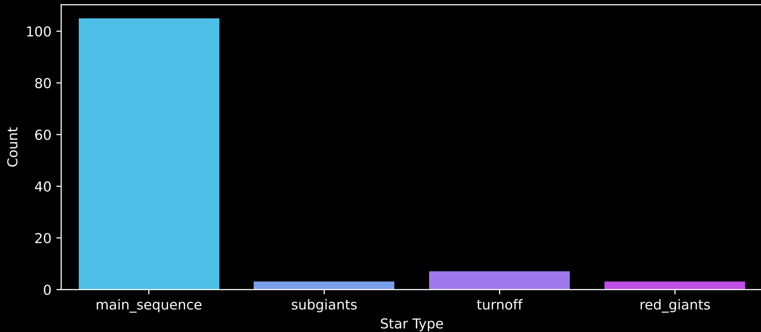
Gaia Cluster: [Czernik_27] Count plot of Star Type
