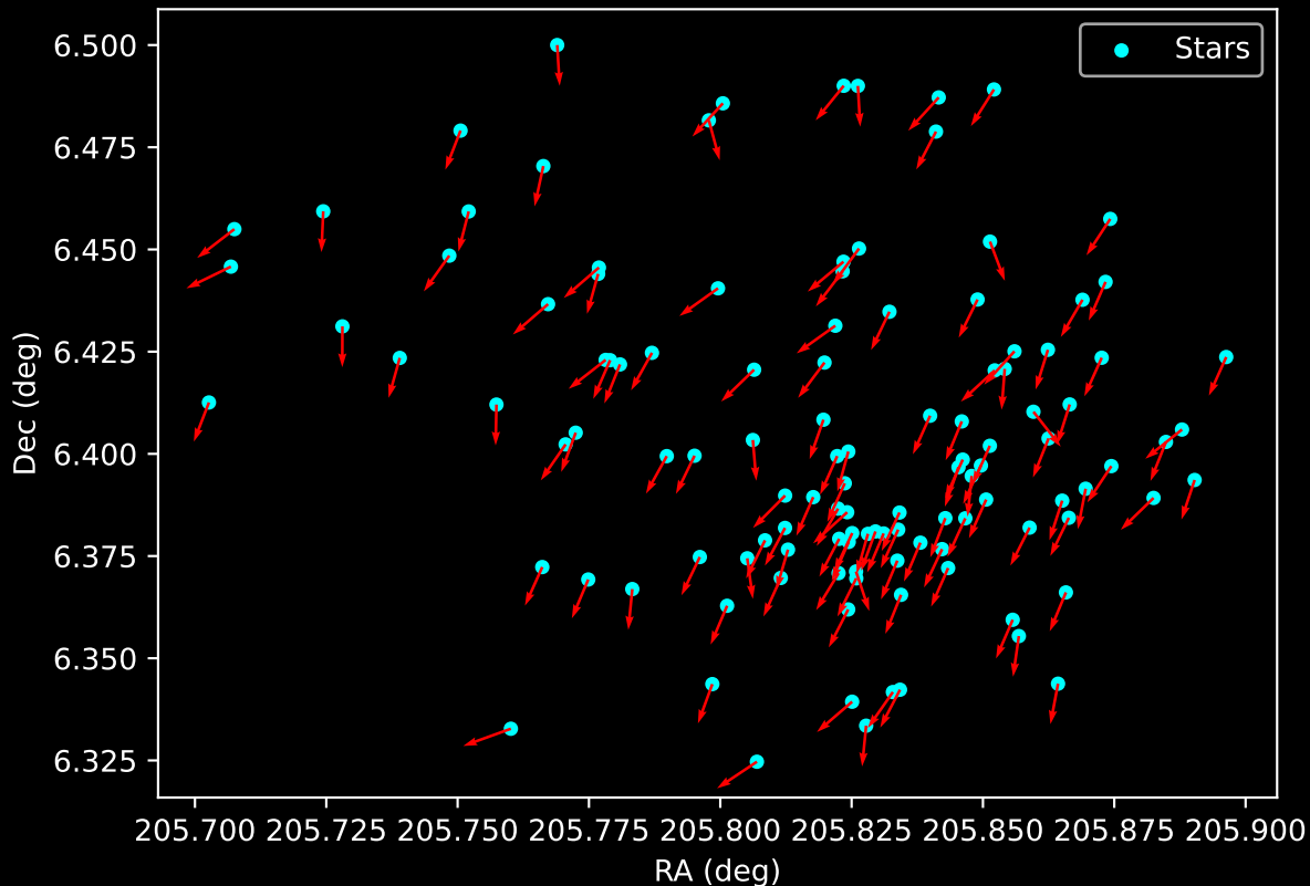
Gaia Cluster: [Czernik_27] Proper Motion Vectors for Gaia Star Field (n= 118)
