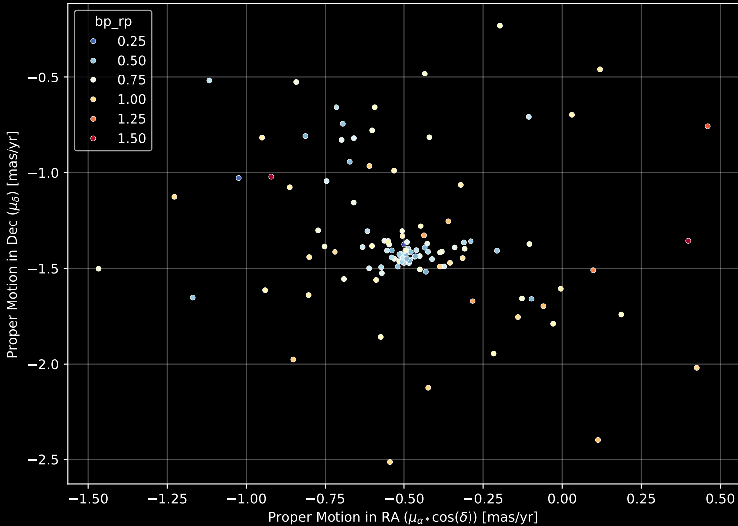
Gaia Cluster: [Czernik_27] Proper Motion Diagram (n= 118)
