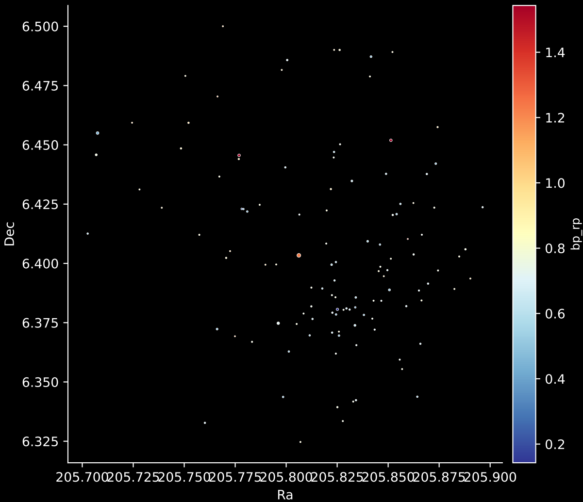
Gaia Cluster: [Czernik_27] Stars: 118
