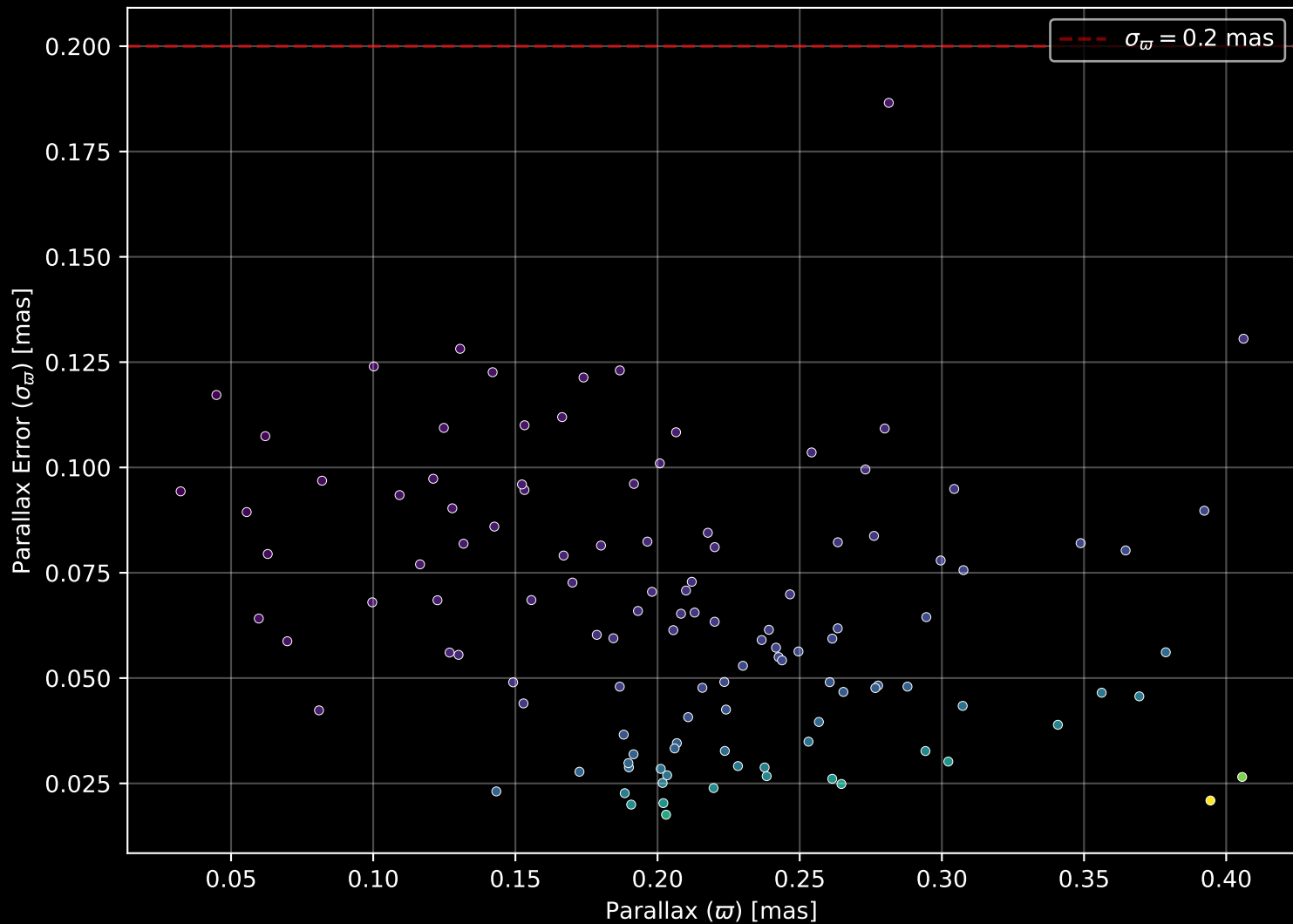
Gaia Cluster: [Czernik_27] Parallax Quality (n= 118)
