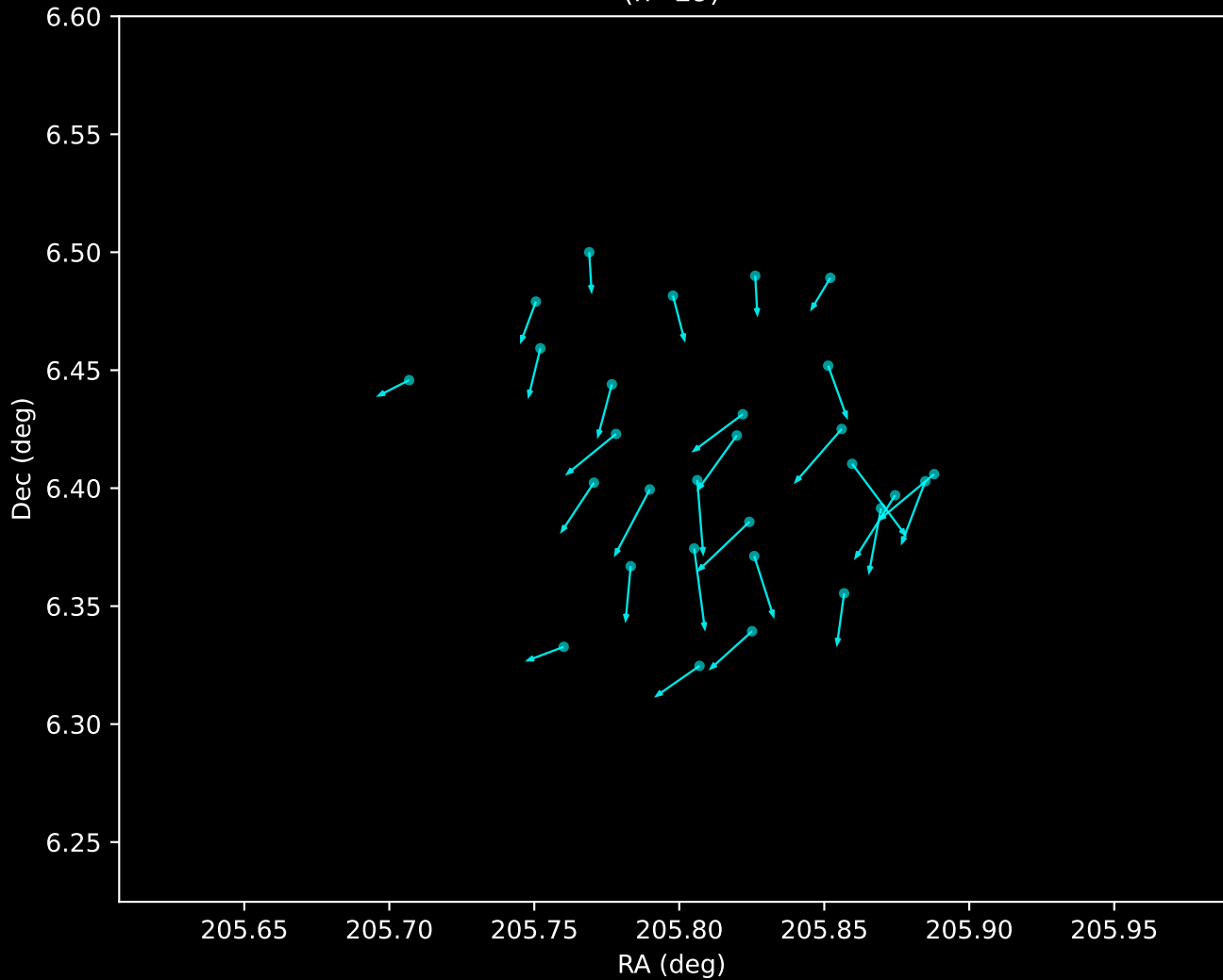
Gaia DR3 Noise Stream Proper Motion Vectors (n=29)
