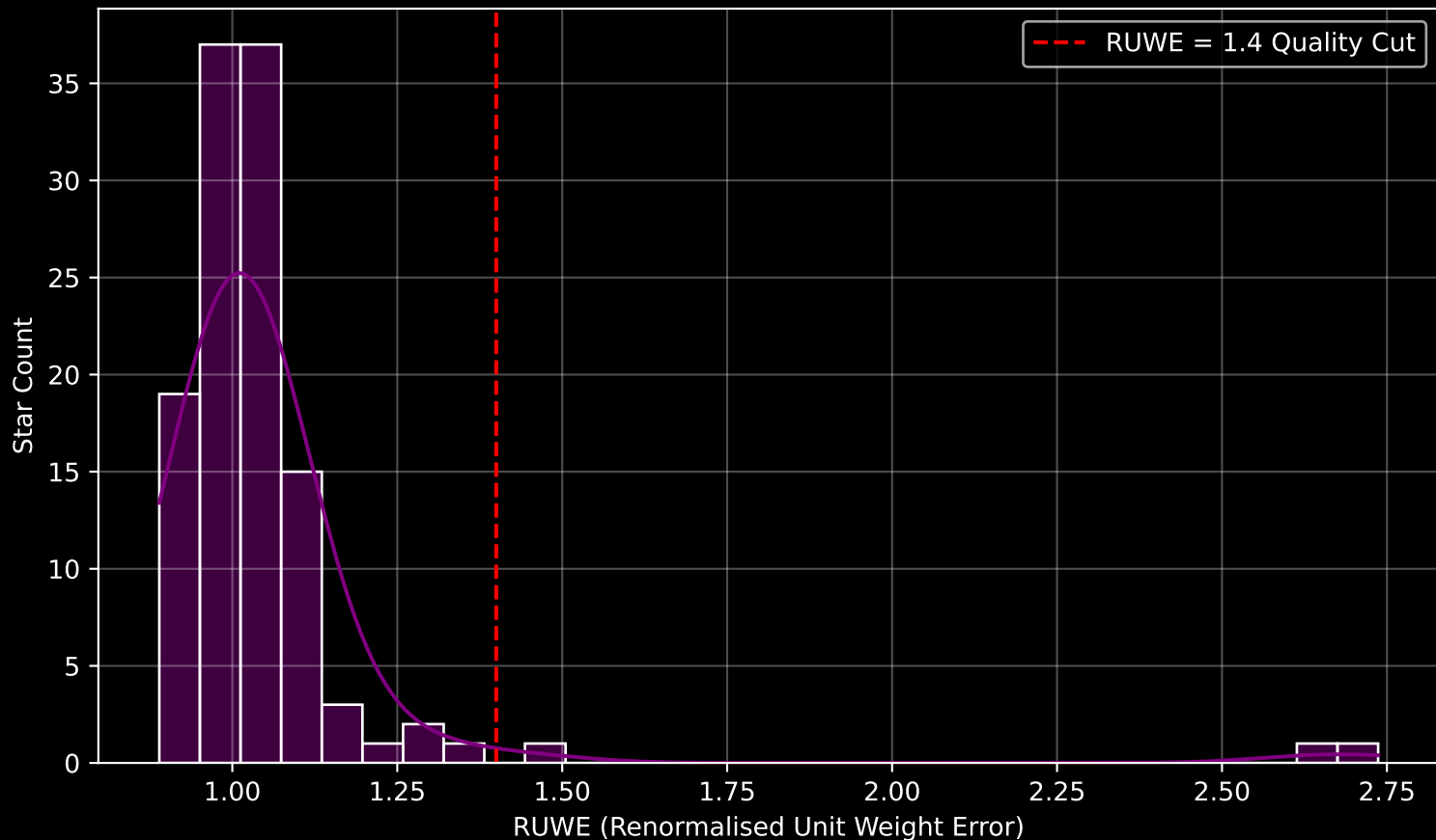
Gaia Cluster: [Czernik_27] RUWE Distribution (n= 118)
