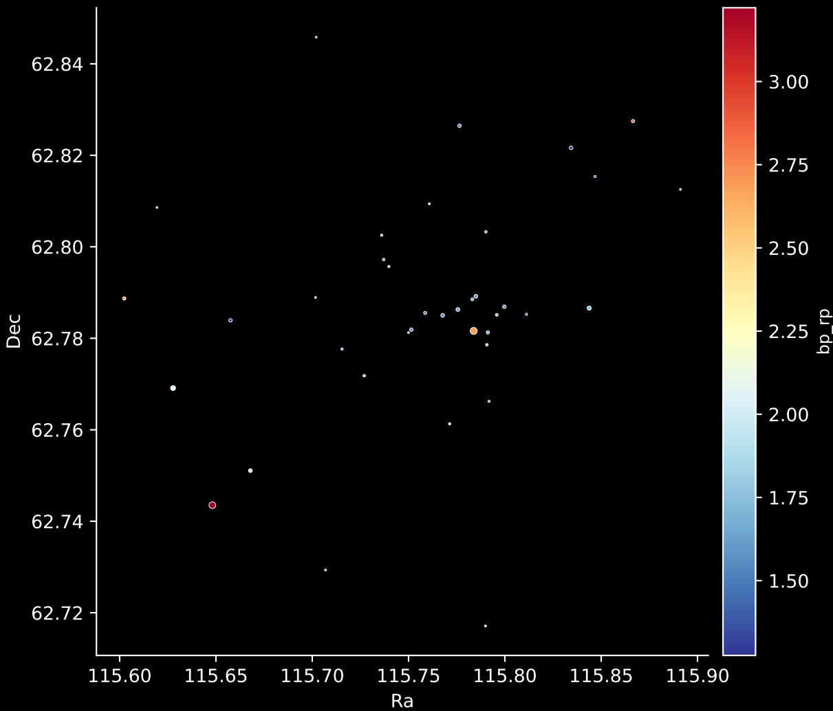
Gaia Cluster: [Czernik_3] Stars: 38
