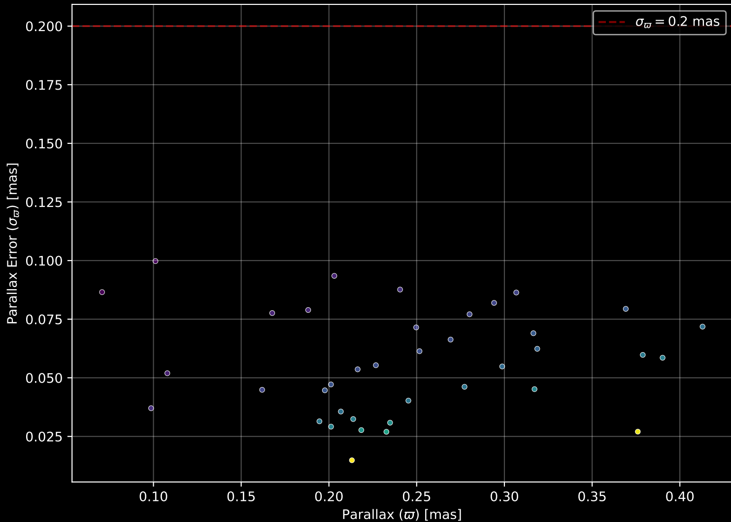
Gaia Cluster: [Czernik_3] Parallax Quality (n= 38)
