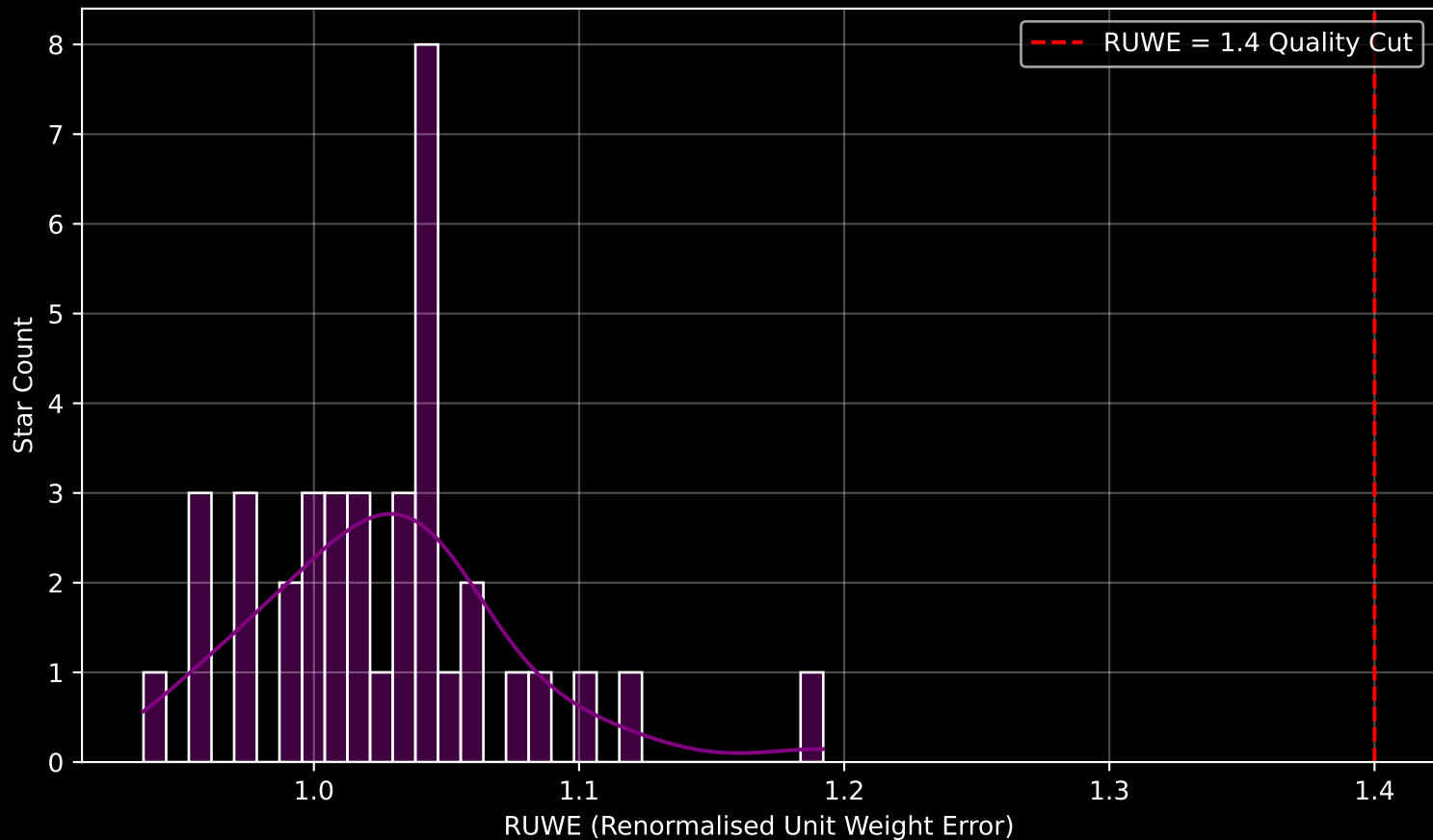
Gaia Cluster: [Czernik_3] RUWE Distribution (n= 38)
