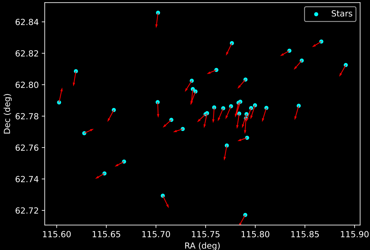
Gaia Cluster: [Czernik_3] Proper Motion Vectors for Gaia Star Field (n= 38)
