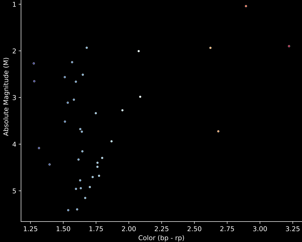
Gaia Cluster: [Czernik_3] Stars (n= 38) Hertzsprung-Russel Diagram
