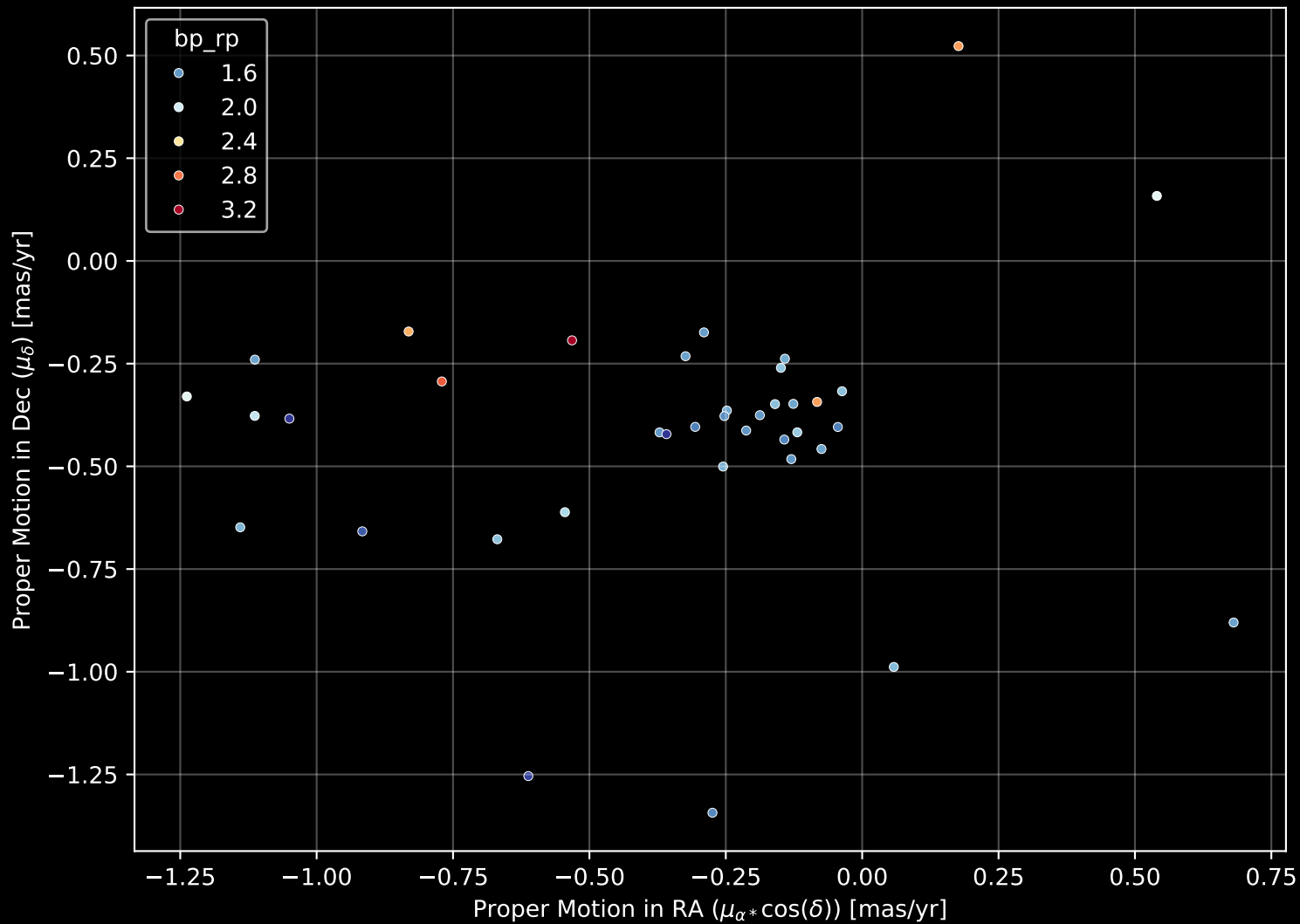
Gaia Cluster: [Czernik_3] Proper Motion Diagram (n= 38)
