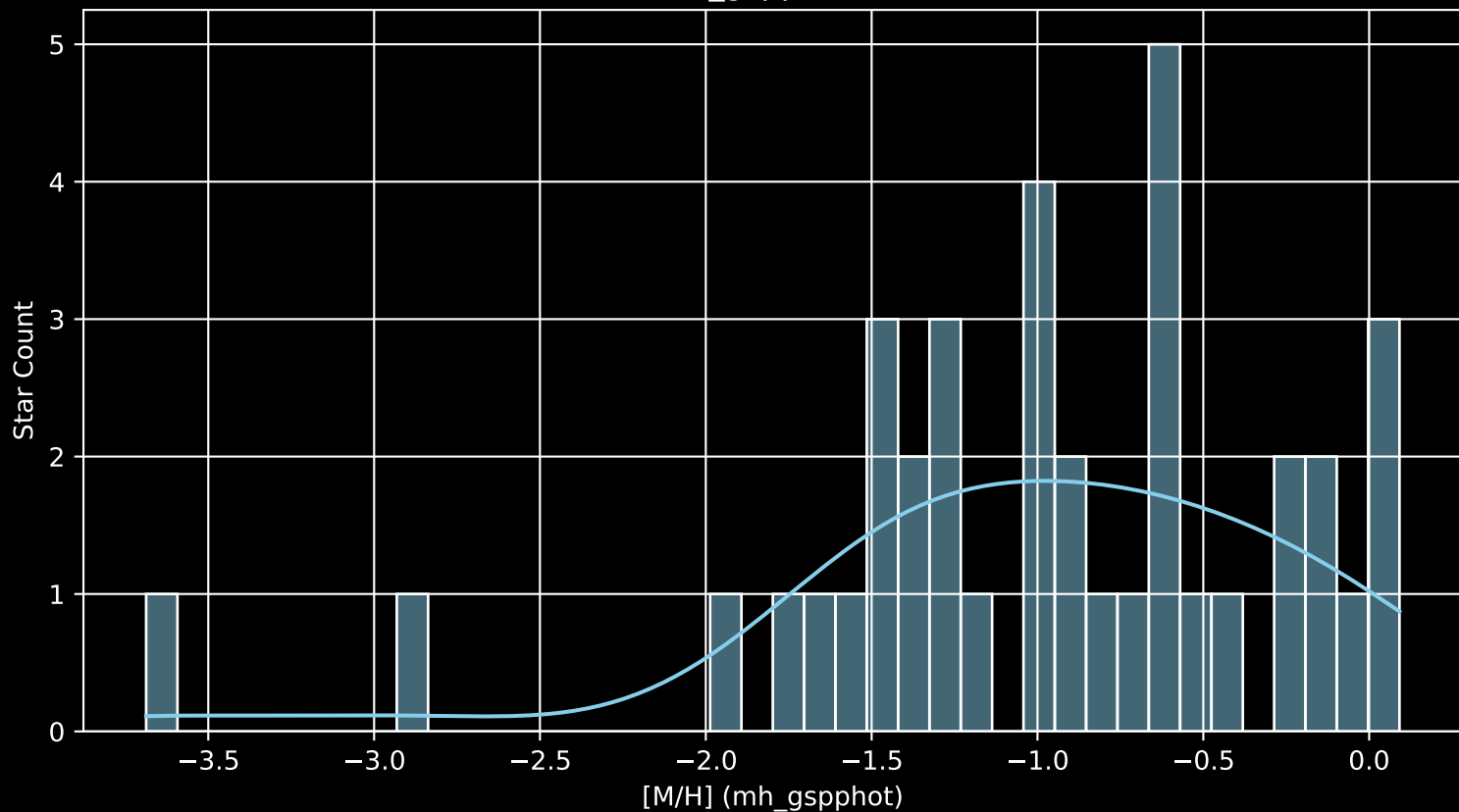
Gaia Cluster: [Czernik_3 [M/H] (mh_gspphot) (n= 38)
