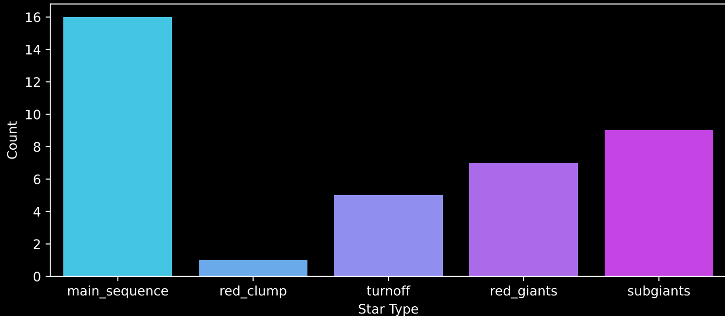
Gaia Cluster: [Czernik_3] Count plot of Star Type
