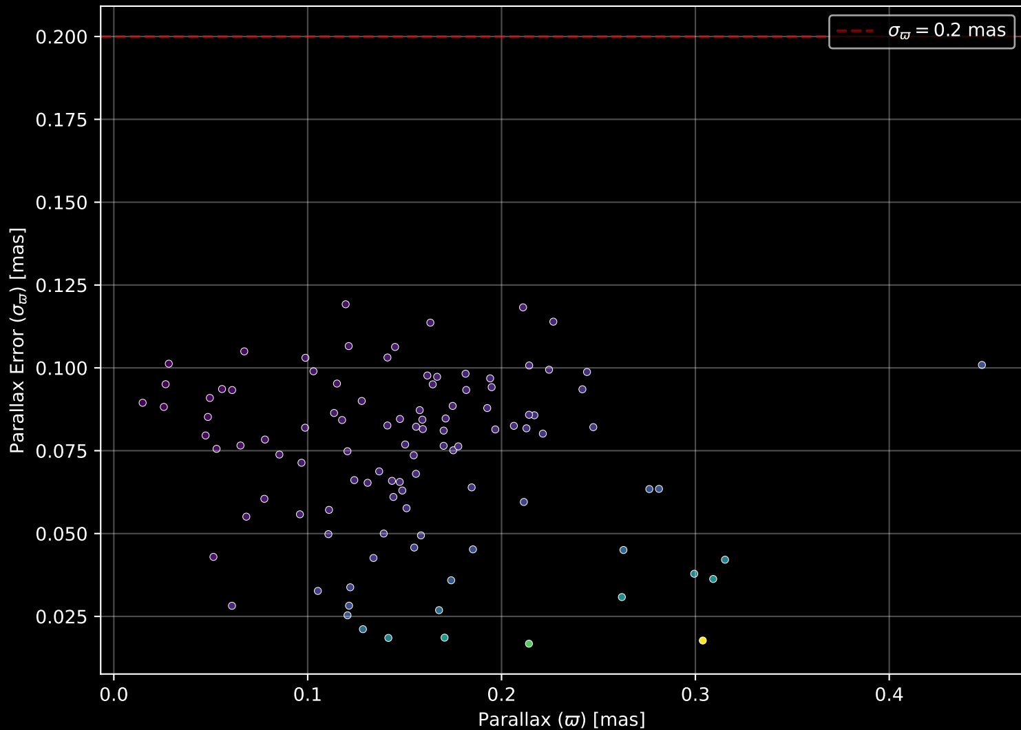
Gaia Cluster: [Czernik_30] Parallax Quality (n= 105)
