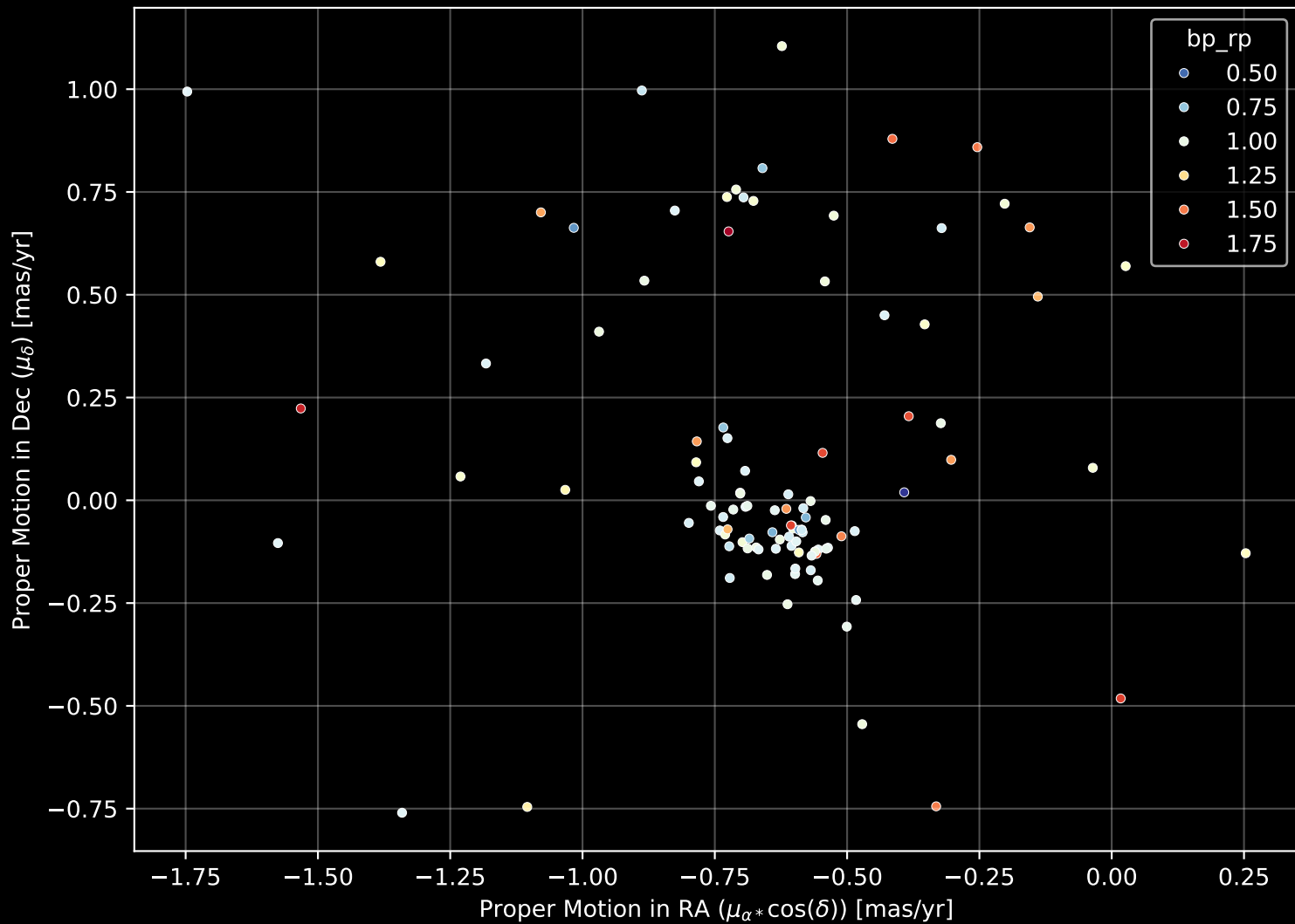
Gaia Cluster: [Czernik_30] Proper Motion Diagram (n= 105)
