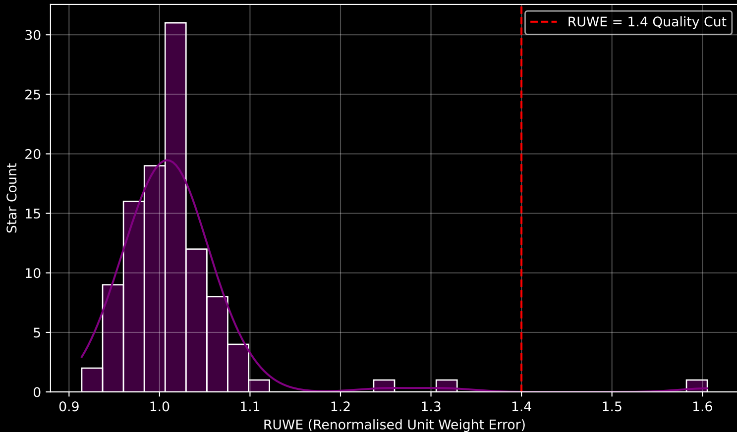
Gaia Cluster: [Czernik_30] RUWE Distribution (n= 105)
