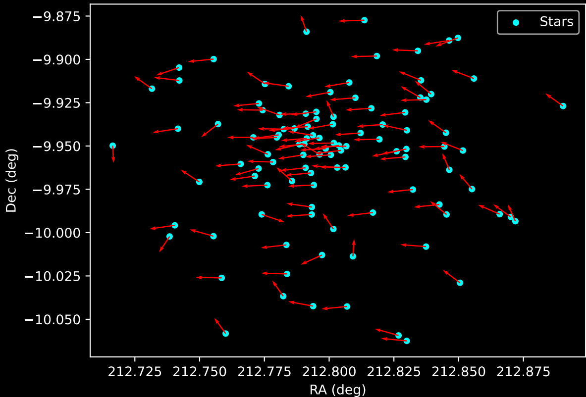
Gaia Cluster: [Czernik_30] Proper Motion Vectors for Gaia Star Field (n= 105)
