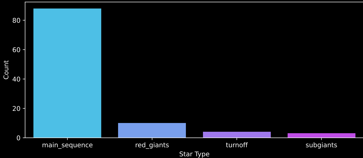
Gaia Cluster: [Czernik_30] Count plot of Star Type
