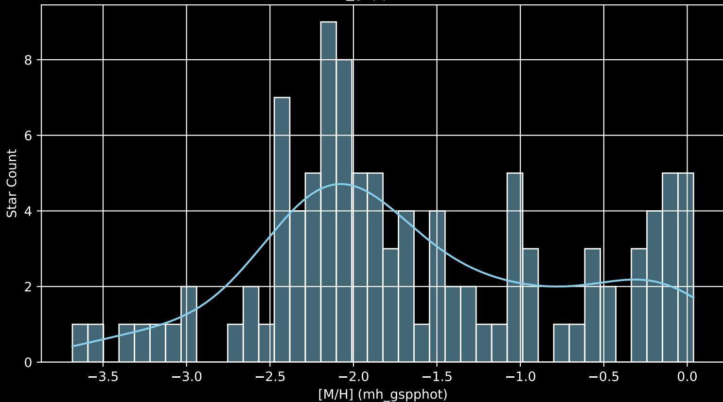
Gaia Cluster: [Czernik_30 [M/H] (mh_gspphot) (n= 105)
