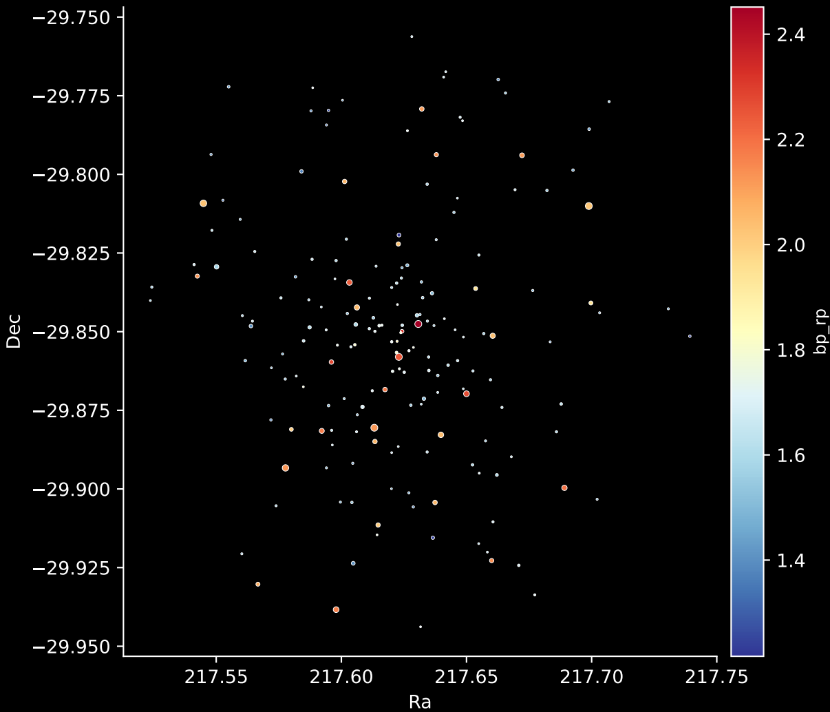
Gaia Cluster: [Czernik_32] Stars: 181
