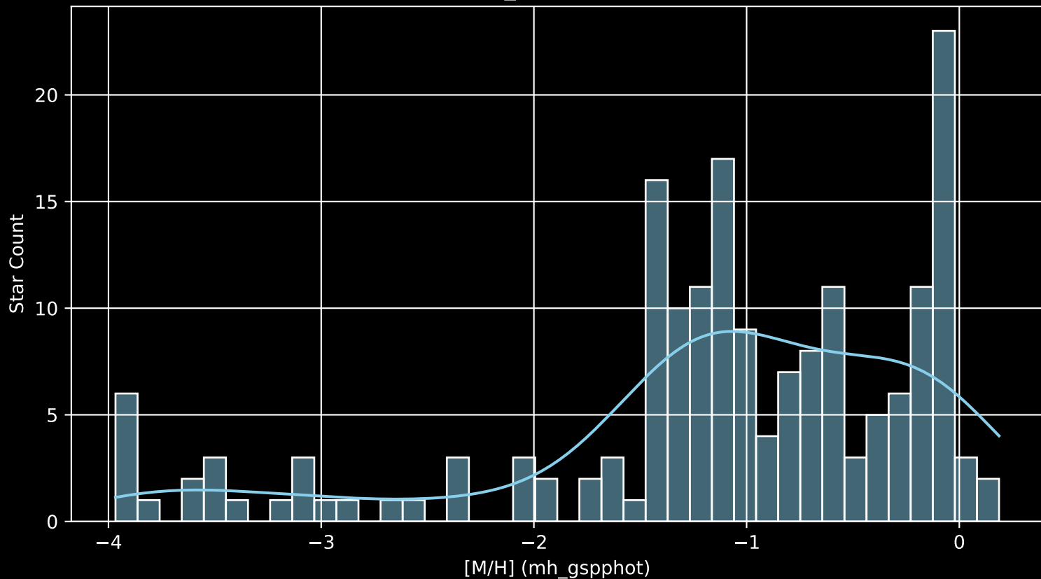
Gaia Cluster: [Czernik_32 [M/H] (mh_gspphot) (n= 181)
