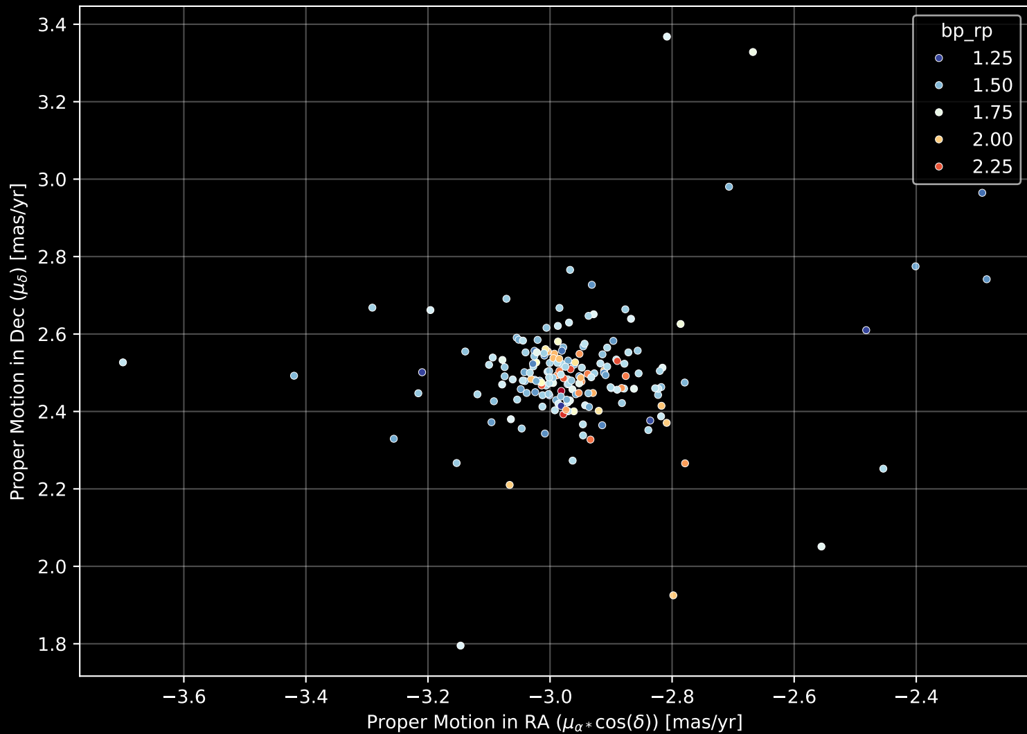
Gaia Cluster: [Czernik_32] Proper Motion Diagram (n= 181)
