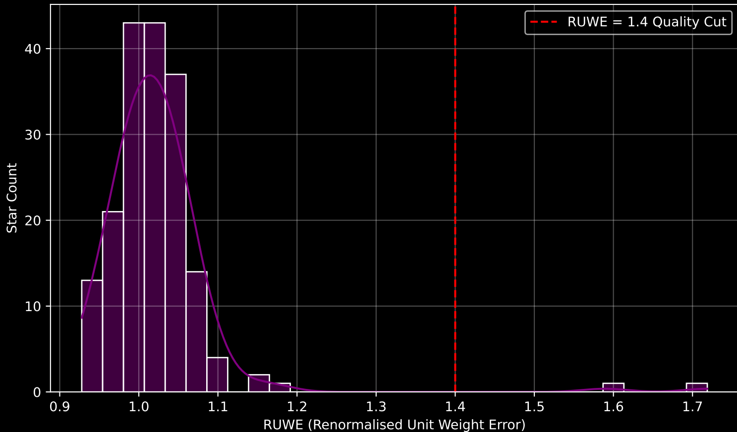
Gaia Cluster: [Czernik_32] RUWE Distribution (n= 180)
