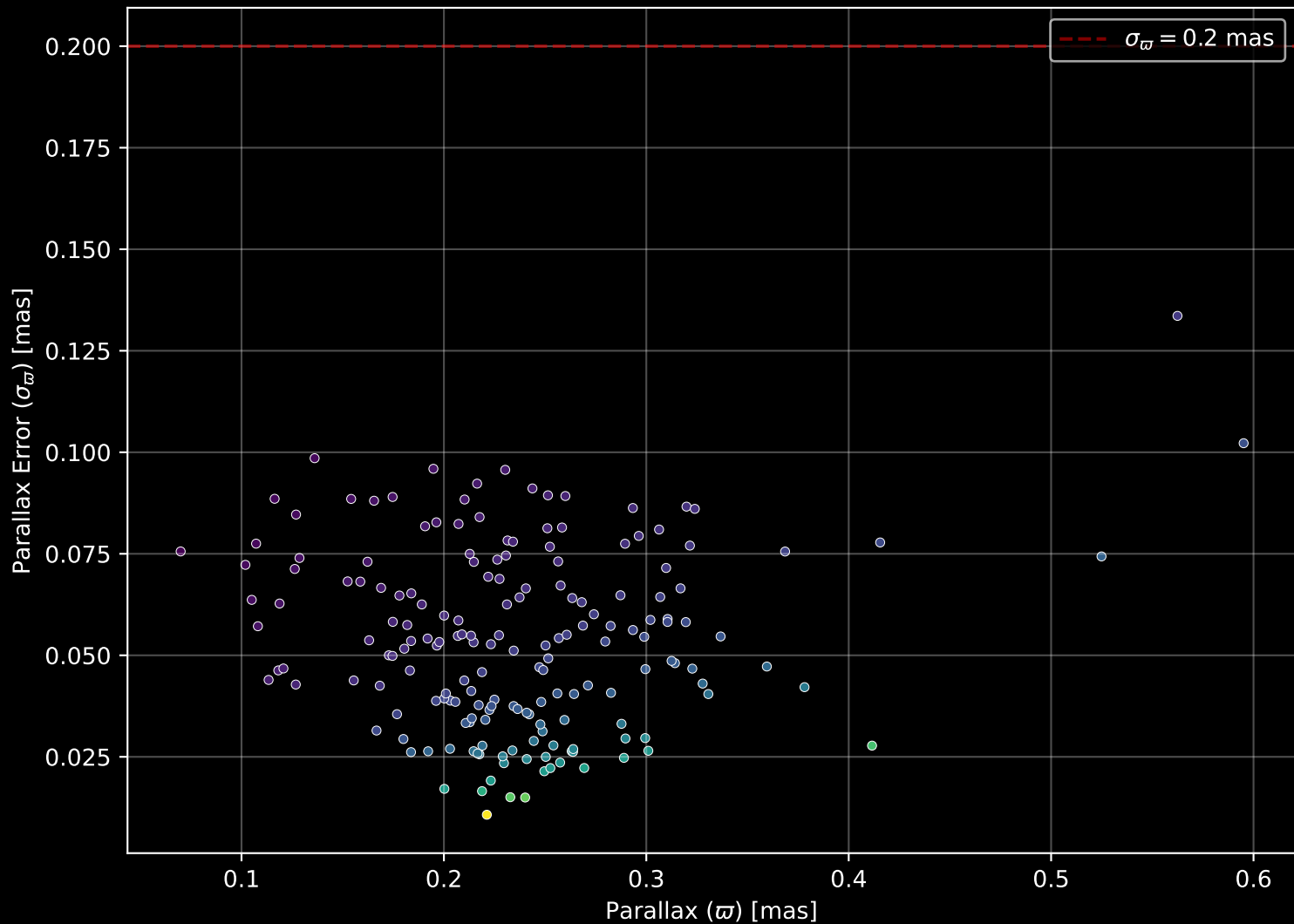
Gaia Cluster: [Czernik_32] Parallax Quality (n= 181)
