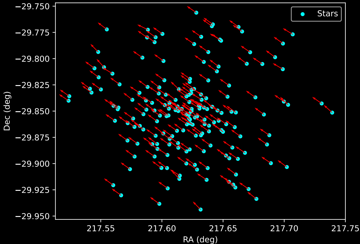
Gaia Cluster: [Czernik_32] Proper Motion Vectors for Gaia Star Field (n= 181)
