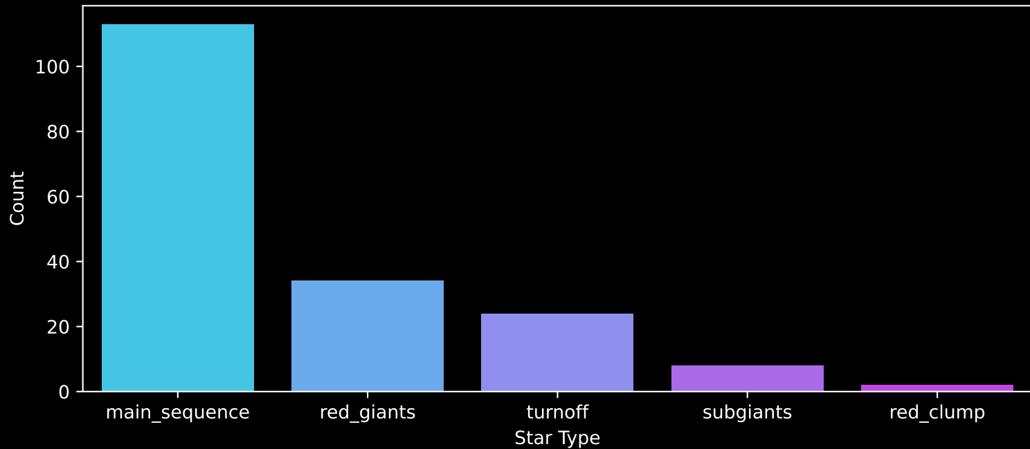
Gaia Cluster: [Czernik_32] Count plot of Star Type
