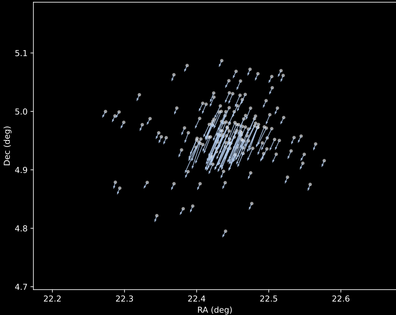
Gaia DR3 Cluster 1 Proper Motion Vectors (n=159)
