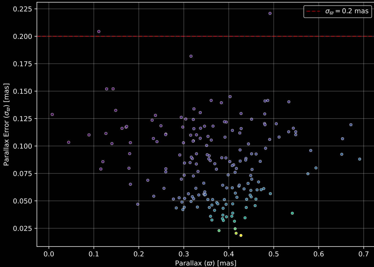
Gaia Cluster: [Czernik_38] Parallax Quality (n= 186)
