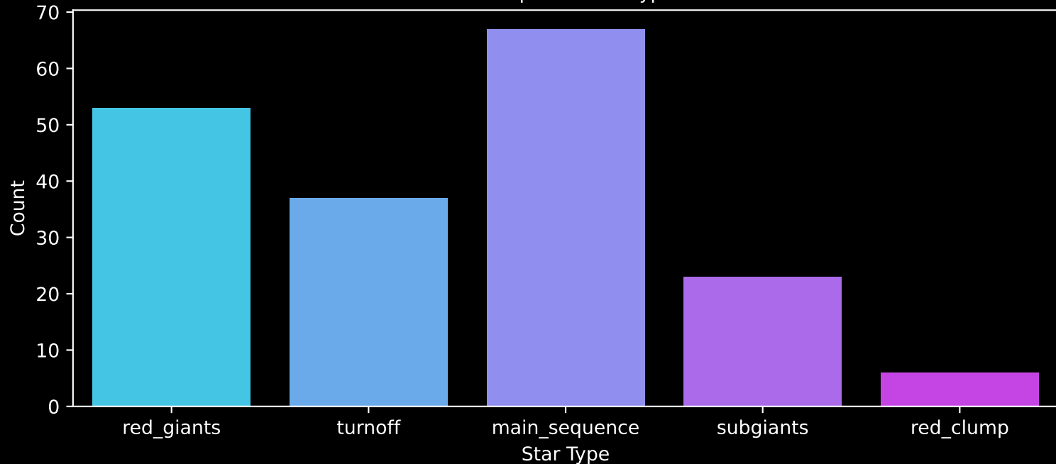
Gaia Cluster: [Czernik_38] Count plot of Star Type
