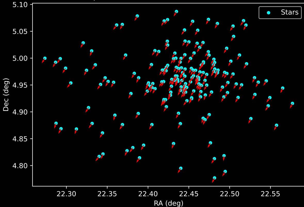
Gaia Cluster: [Czernik_38] Proper Motion Vectors for Gaia Star Field (n= 186)
