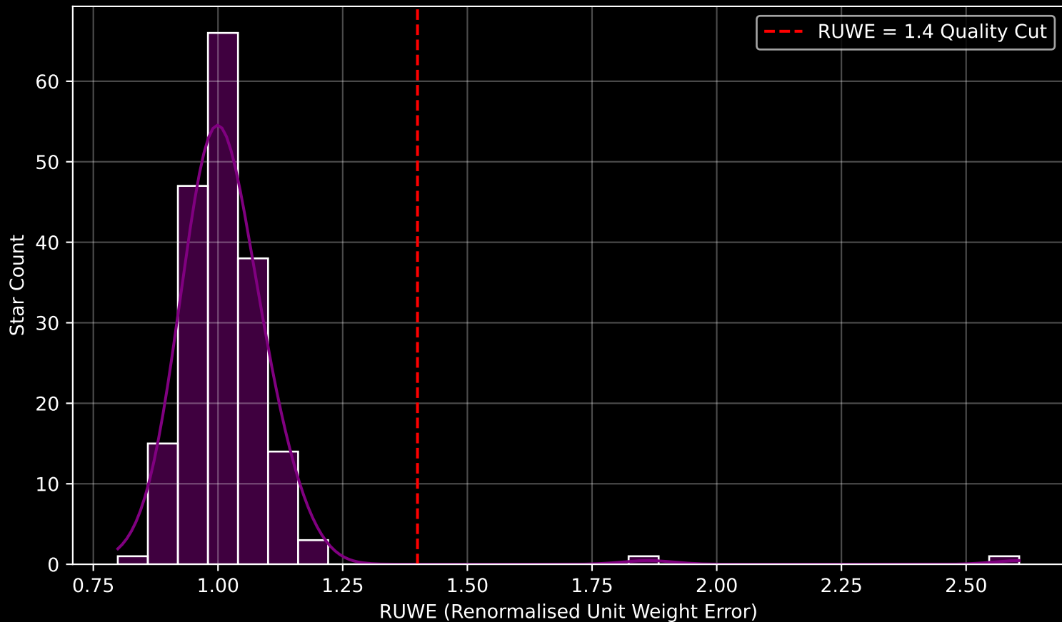
Gaia Cluster: [Czernik_38] RUWE Distribution (n= 186)
