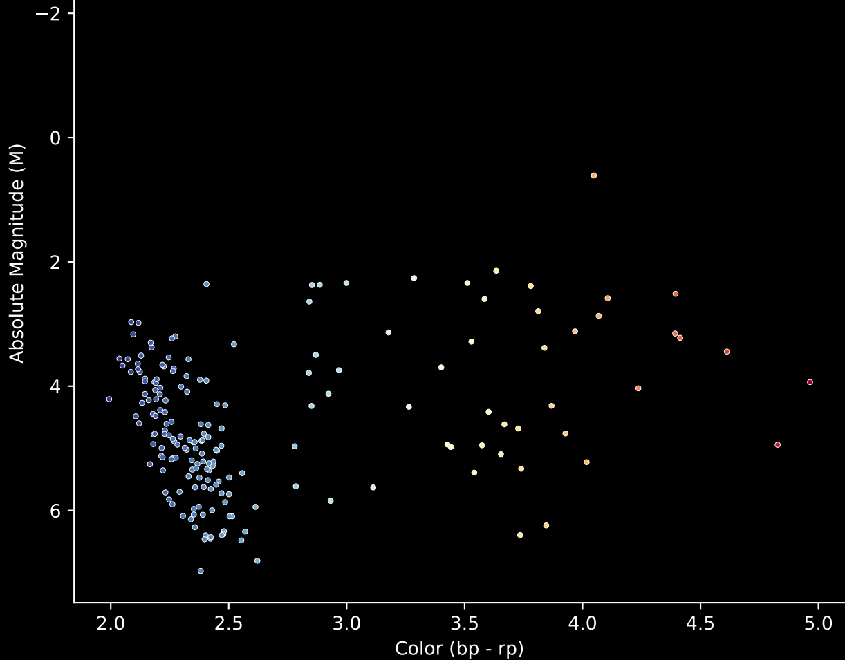
Gaia Cluster: [Czernik_38] Stars (n= 186) Hertzsprung-Russel Diagram
