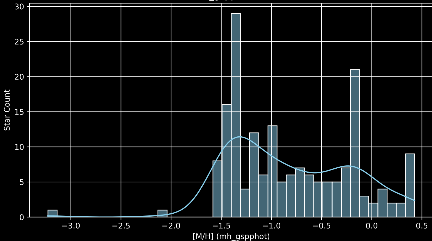
Gaia Cluster: [Czernik_38 [M/H] (mh_gspphot) (n= 179)
