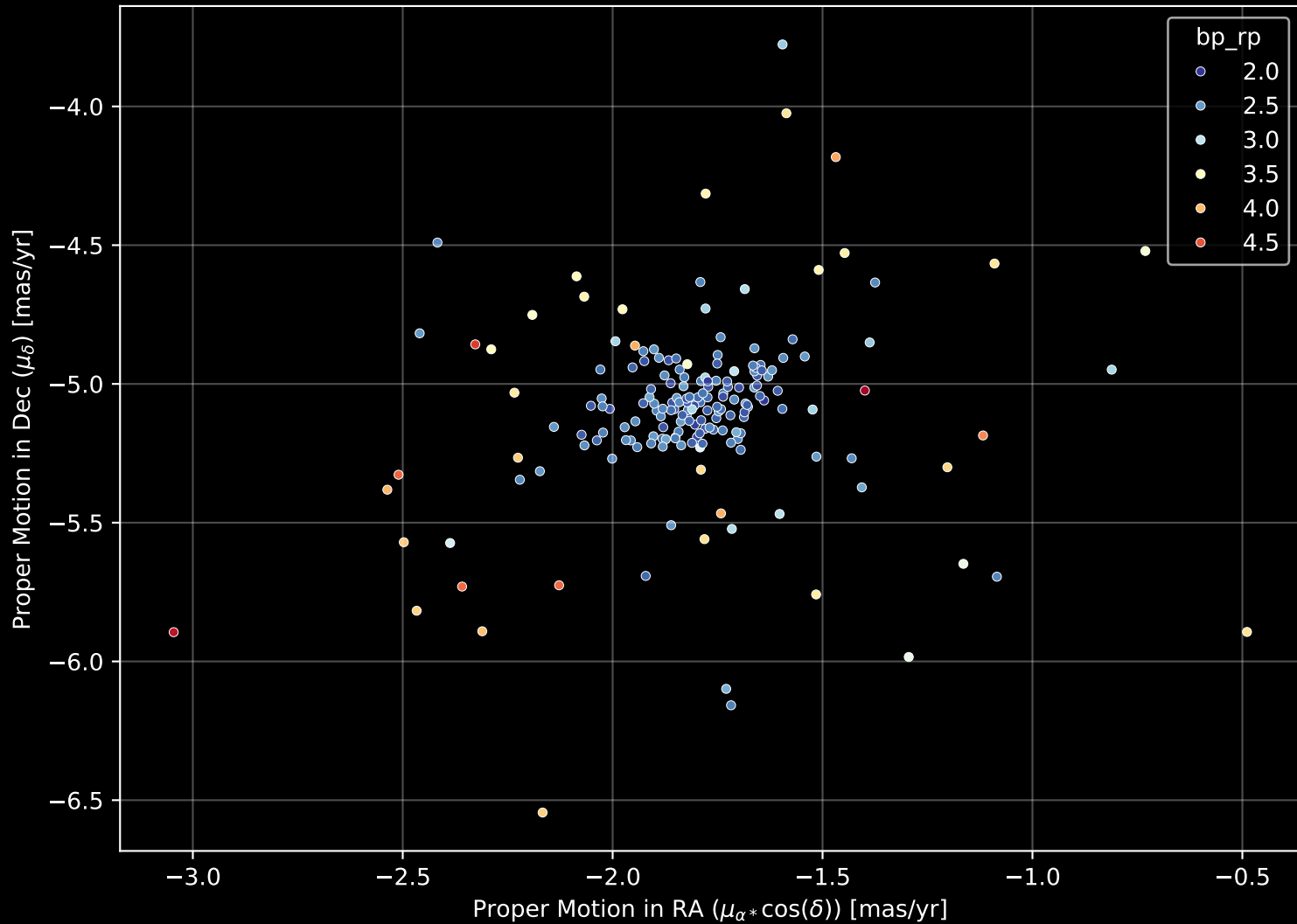
Gaia Cluster: [Czernik_38] Proper Motion Diagram (n= 186)
