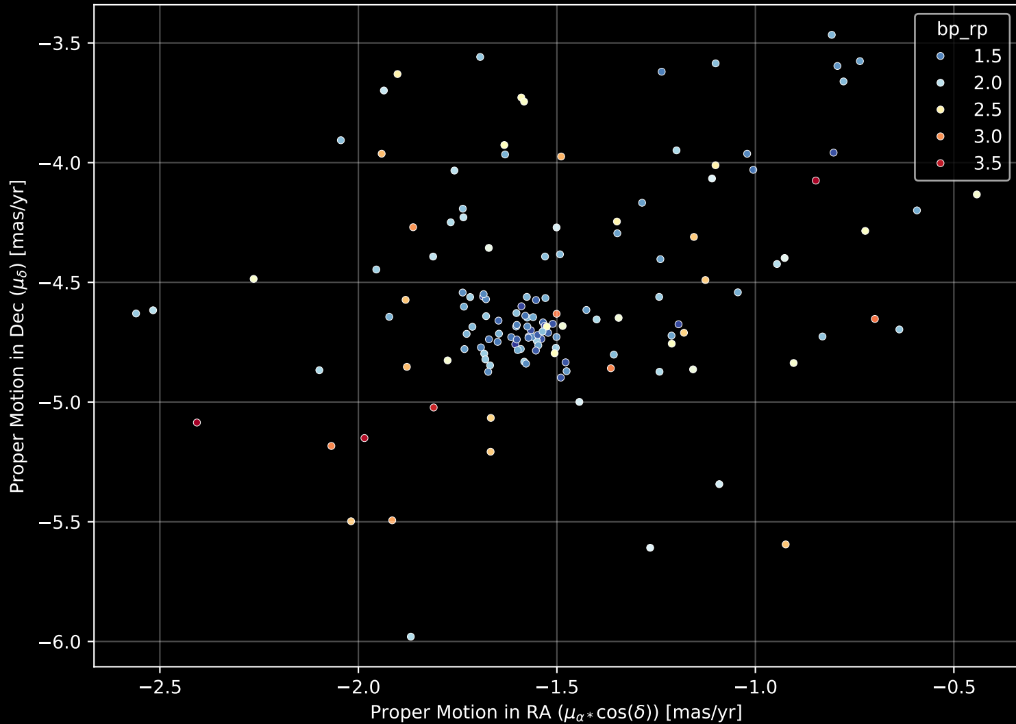
Gaia Cluster: [Czernik_39] Proper Motion Diagram (n= 143)
