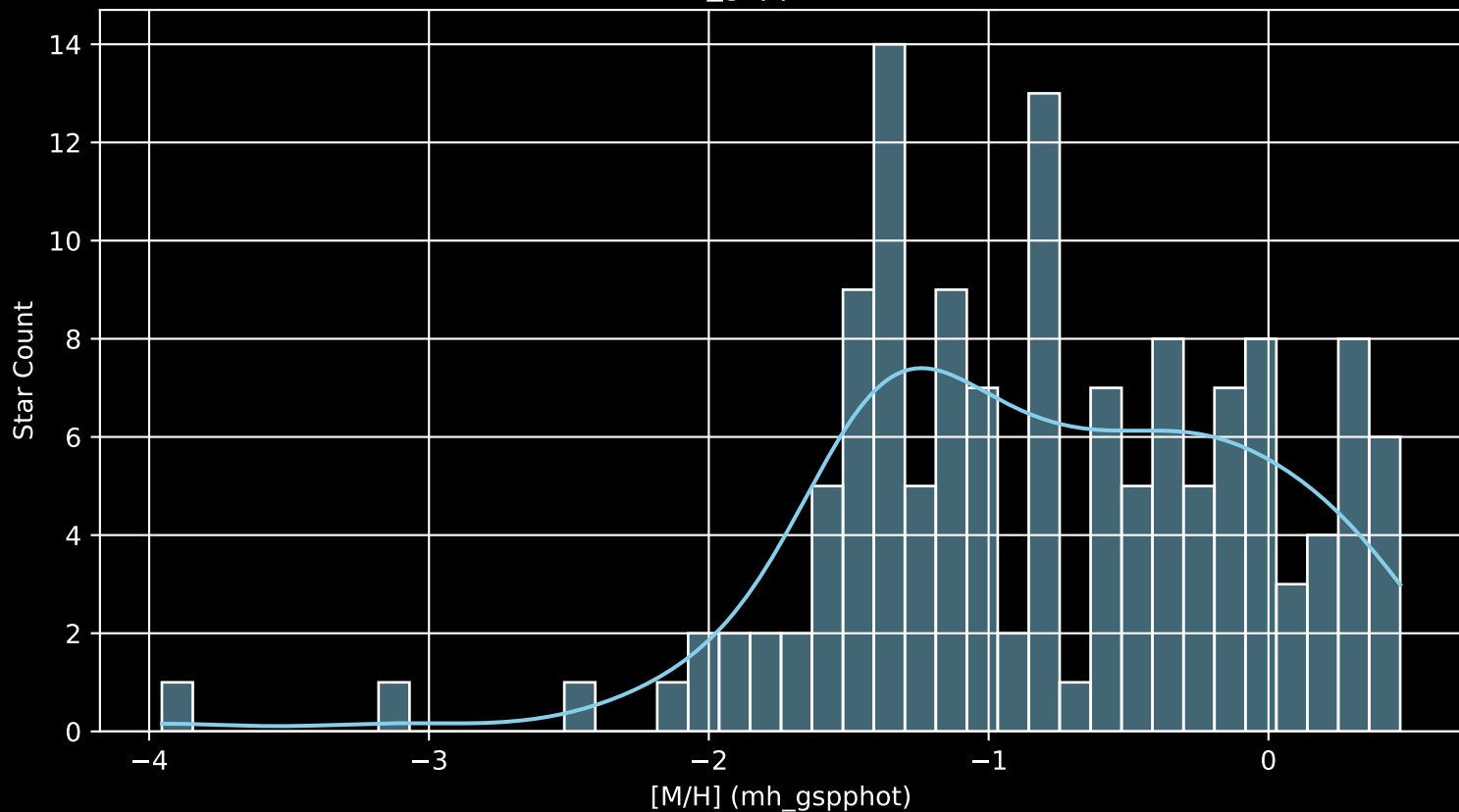
Gaia Cluster: [Czernik_39 [M/H] (mh_gspphot) (n= 138)
