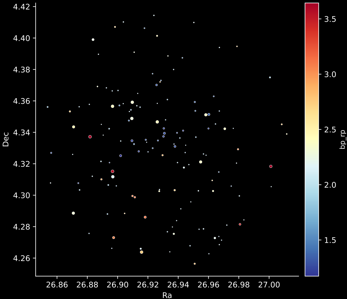
Gaia Cluster: [Czernik_39] Stars: 143
