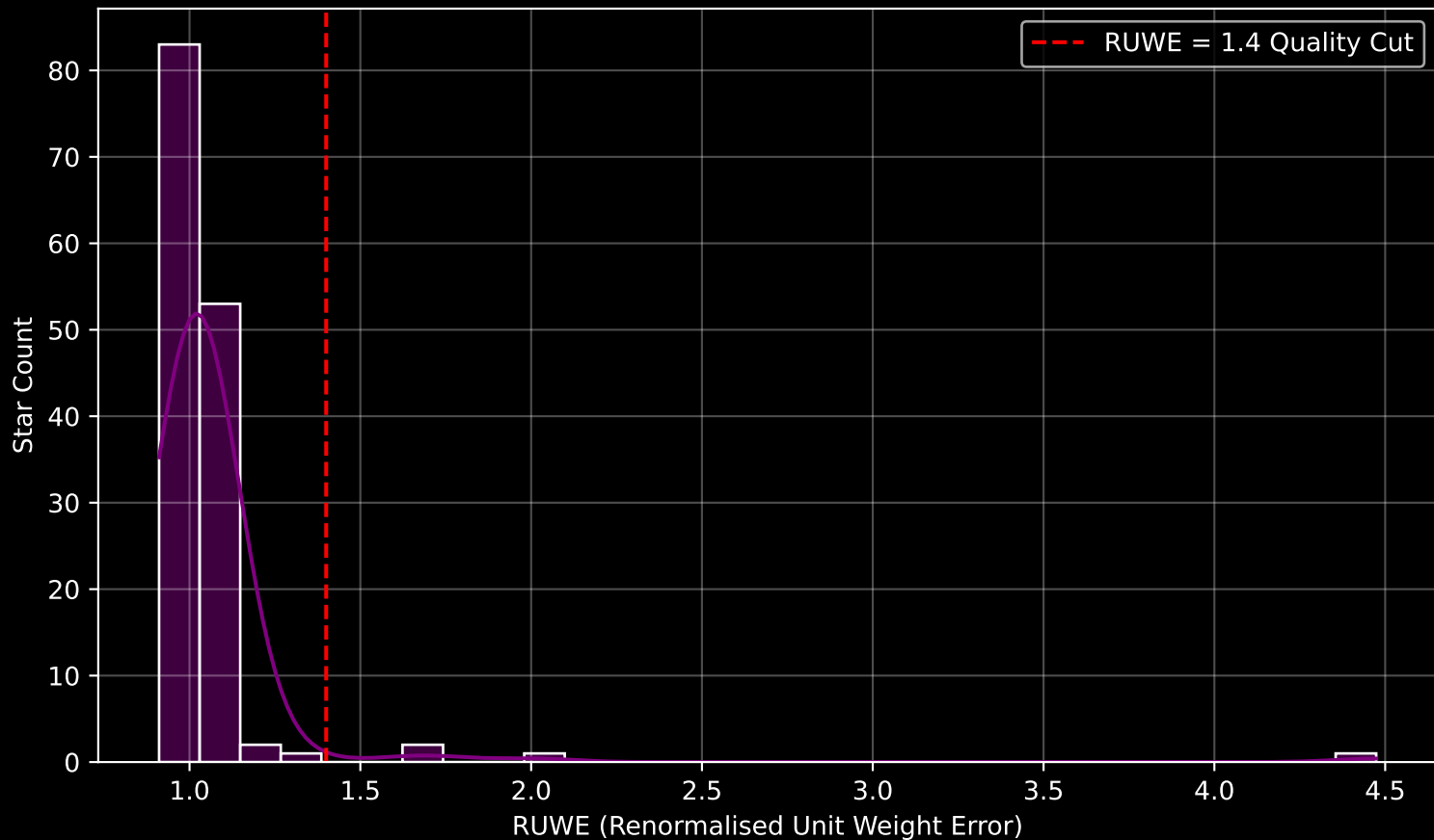
Gaia Cluster: [Czernik_39] RUWE Distribution (n= 143)
