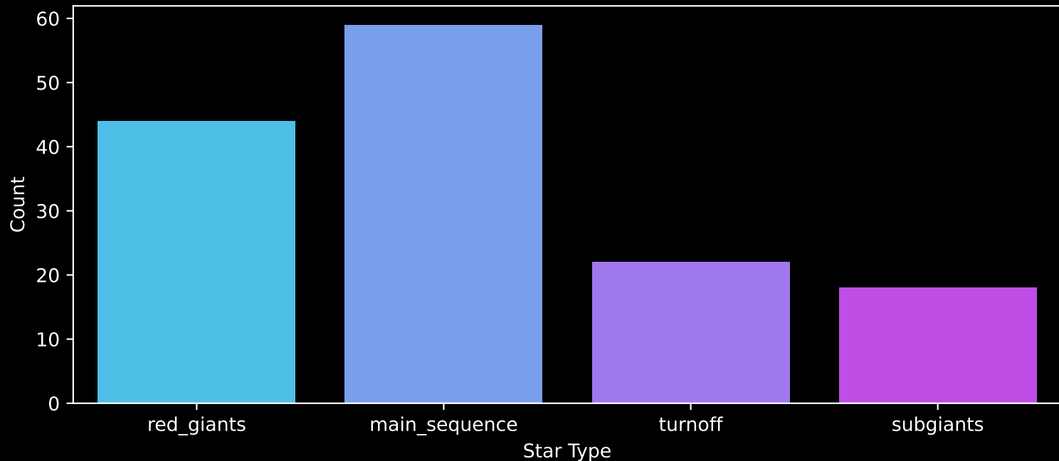
Gaia Cluster: [Czernik_39] Count plot of Star Type
