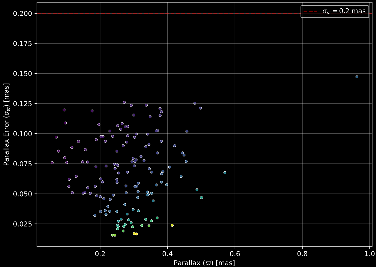
Gaia Cluster: [Czernik_39] Parallax Quality (n= 143)
