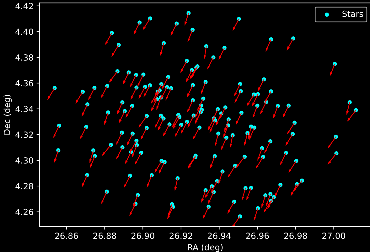
Gaia Cluster: [Czernik_39] Proper Motion Vectors for Gaia Star Field (n= 143)
