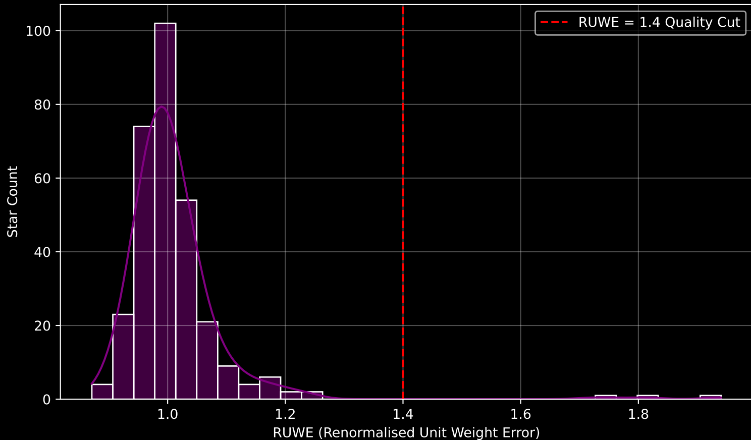
Gaia Cluster: [Czernik_40] RUWE Distribution (n= 304)
