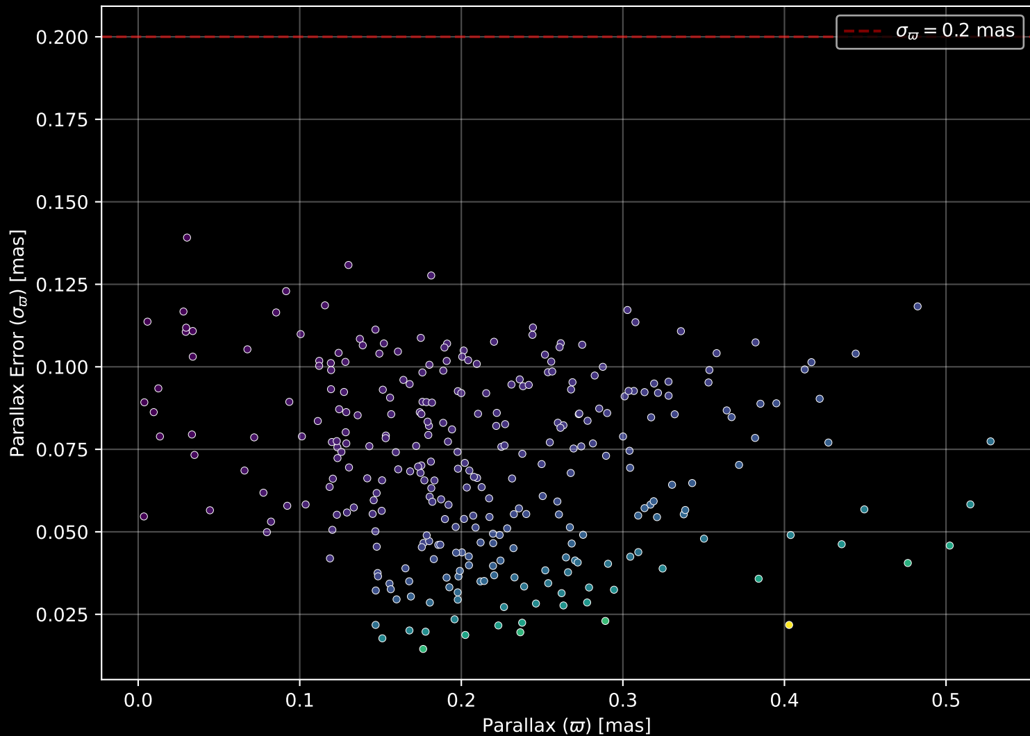
Gaia Cluster: [Czernik_40] Parallax Quality (n= 304)
