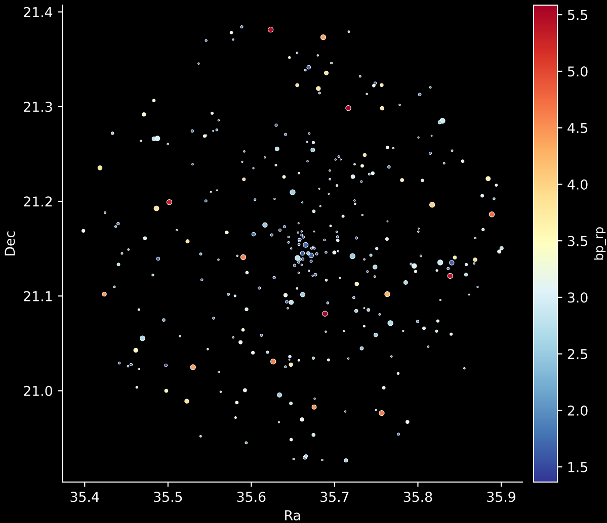
Gaia Cluster: [Czernik_40] Stars: 304
