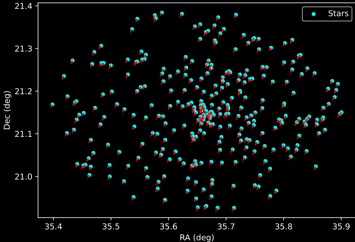
Gaia Cluster: [Czernik_40] Proper Motion Vectors for Gaia Star Field (n= 304)
