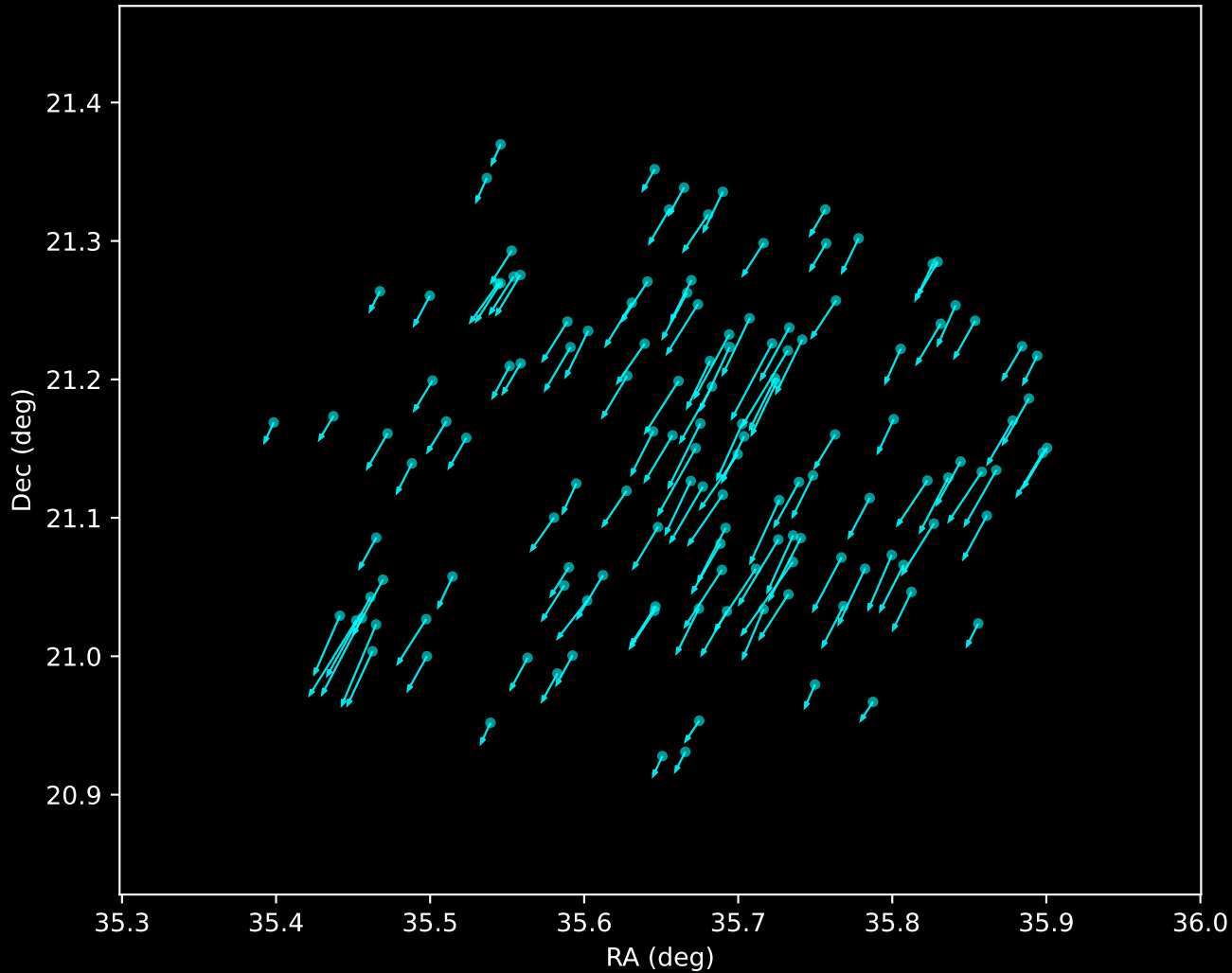
Gaia DR3 Noise Stream Proper Motion Vectors (n=134)
