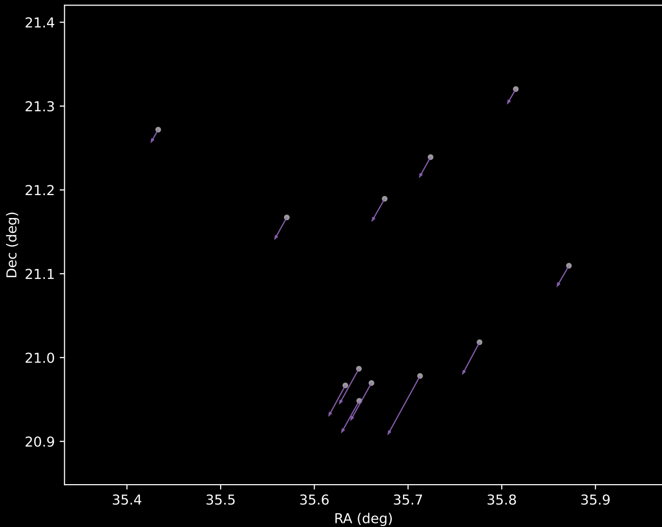
Gaia DR3 Cluster 8 Proper Motion Vectors (n=12)
