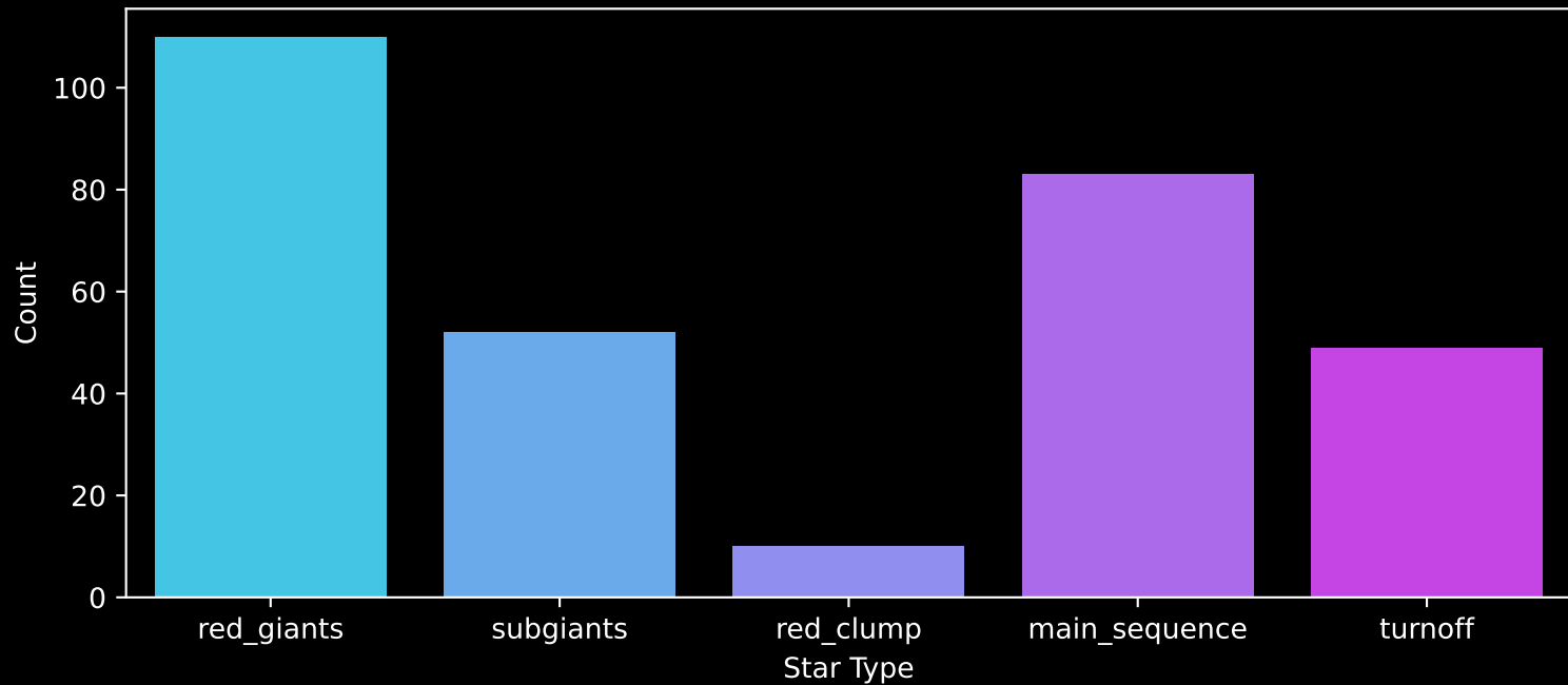
Gaia Cluster: [Czernik_40] Count plot of Star Type
