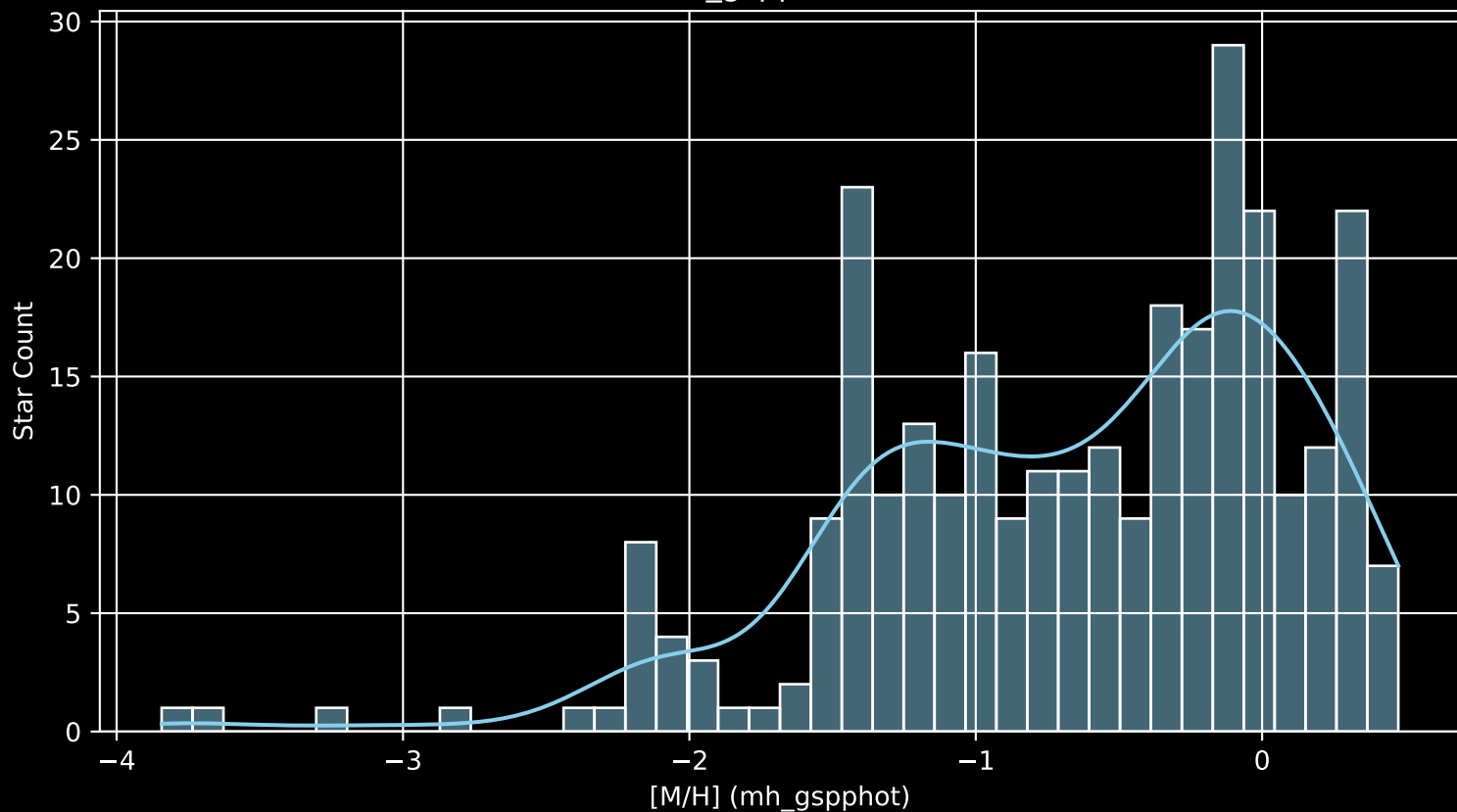
Gaia Cluster: [Czernik_40 [M/H] (mh_gspphot) (n= 295)
