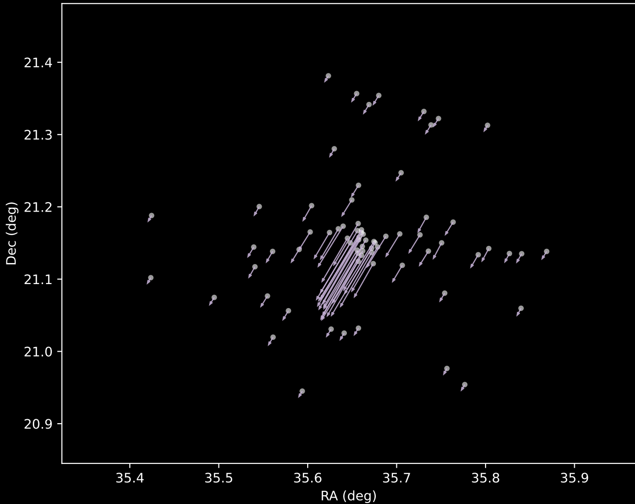
Gaia DR3 Cluster 9 Proper Motion Vectors (n=71)
