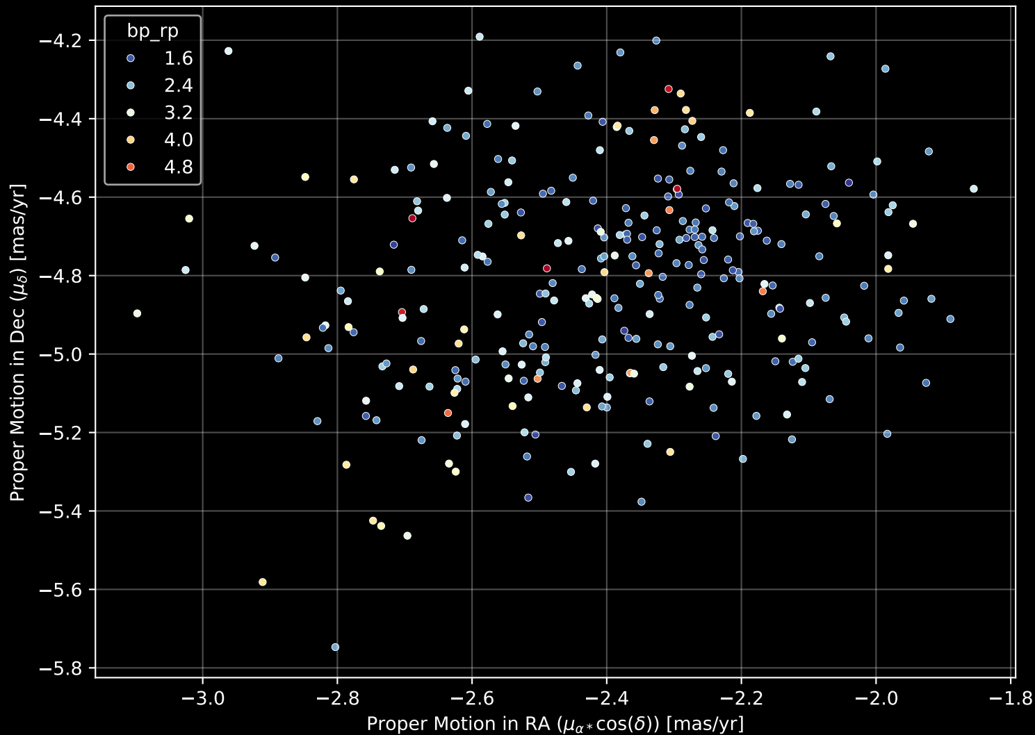
Gaia Cluster: [Czernik_40] Proper Motion Diagram (n= 304)
