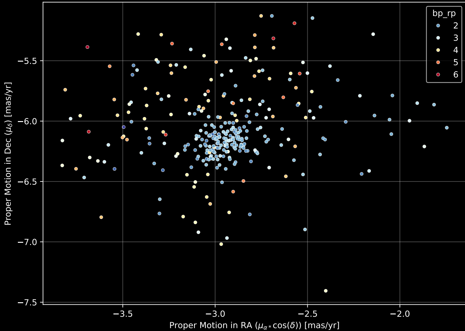
Gaia Cluster: [Czernik_41] Proper Motion Diagram (n= 315)
