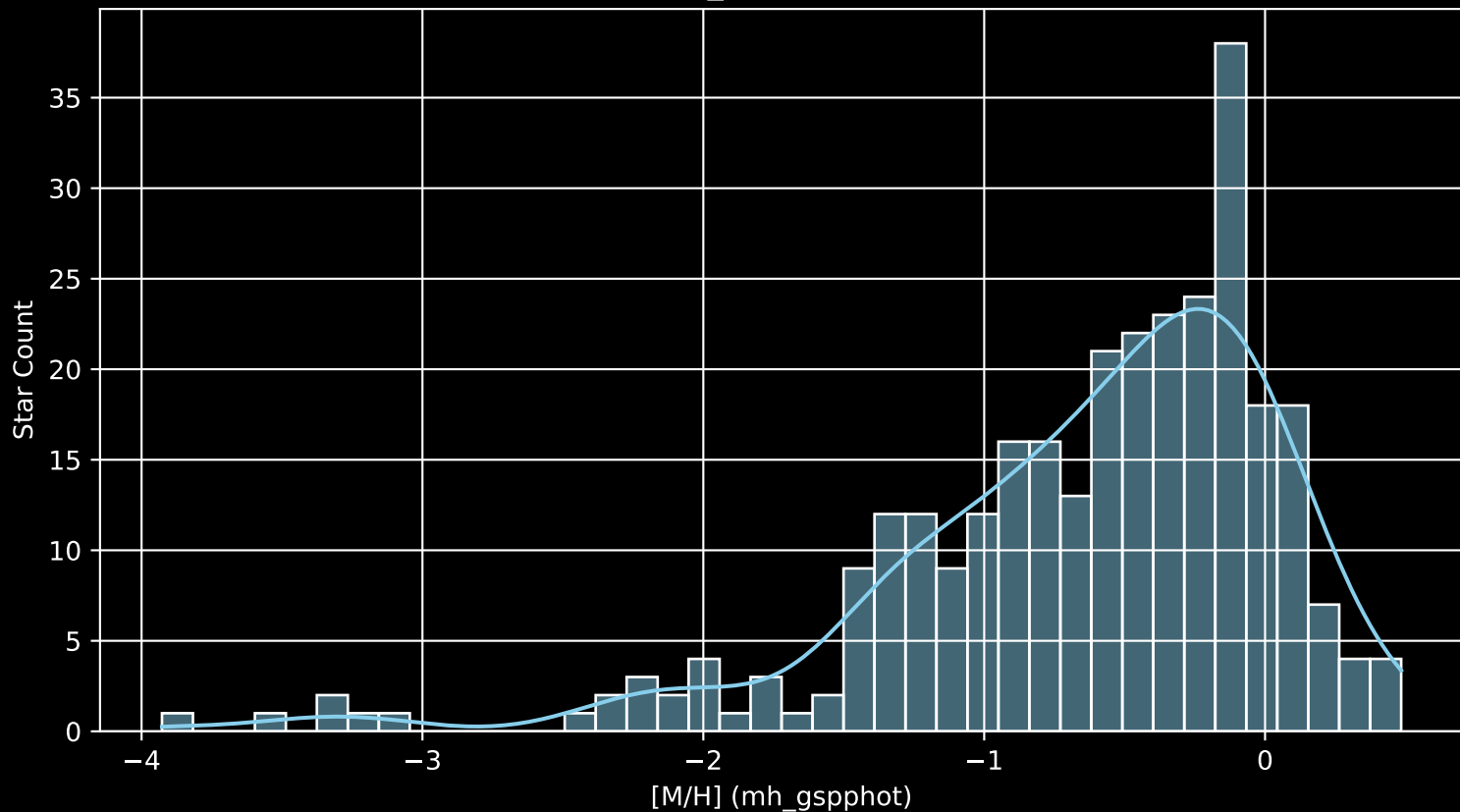
Gaia Cluster: [Czernik_41 [M/H] (mh_gspphot) (n= 303)
