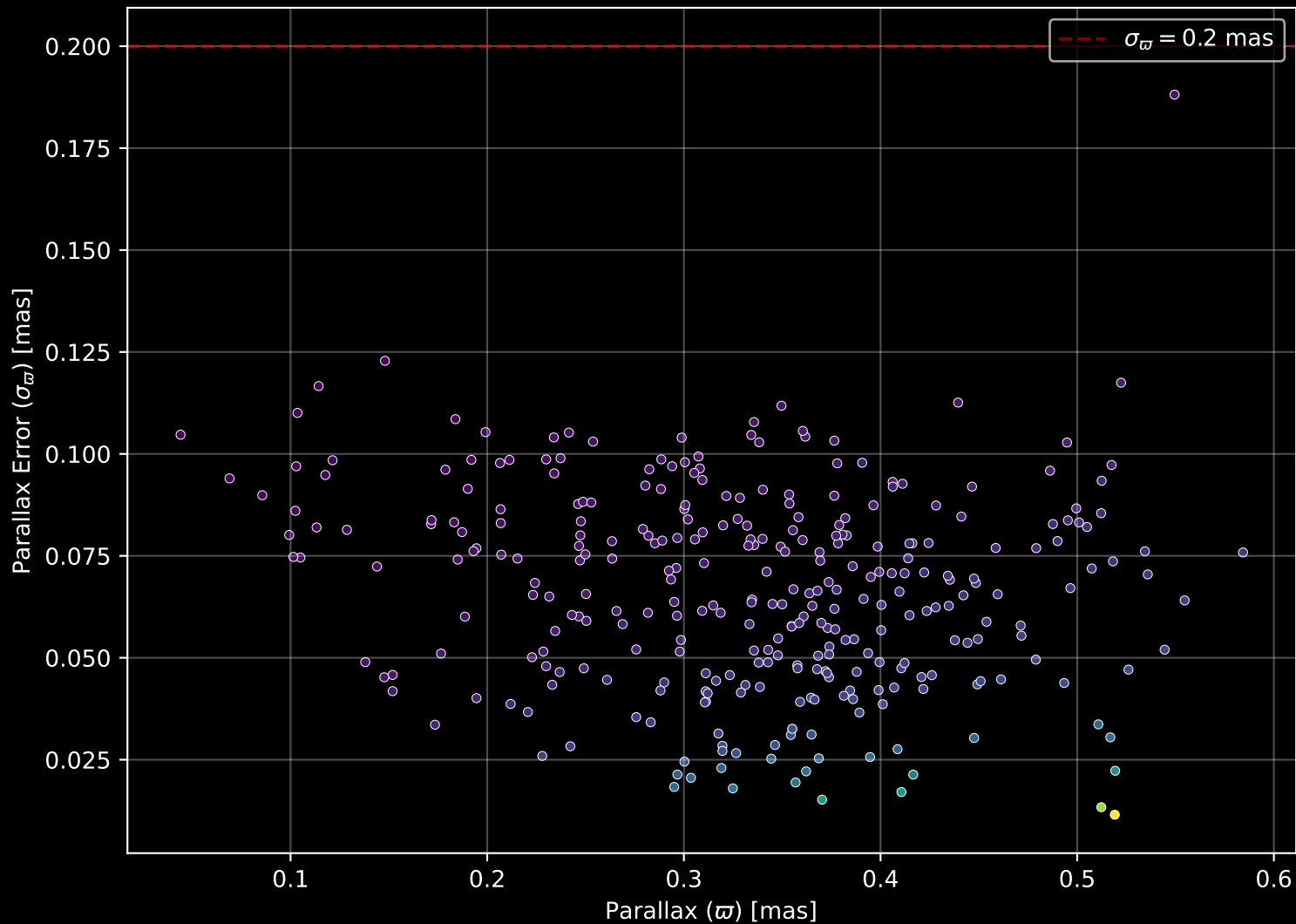
Gaia Cluster: [Czernik_41] Parallax Quality (n= 315)
