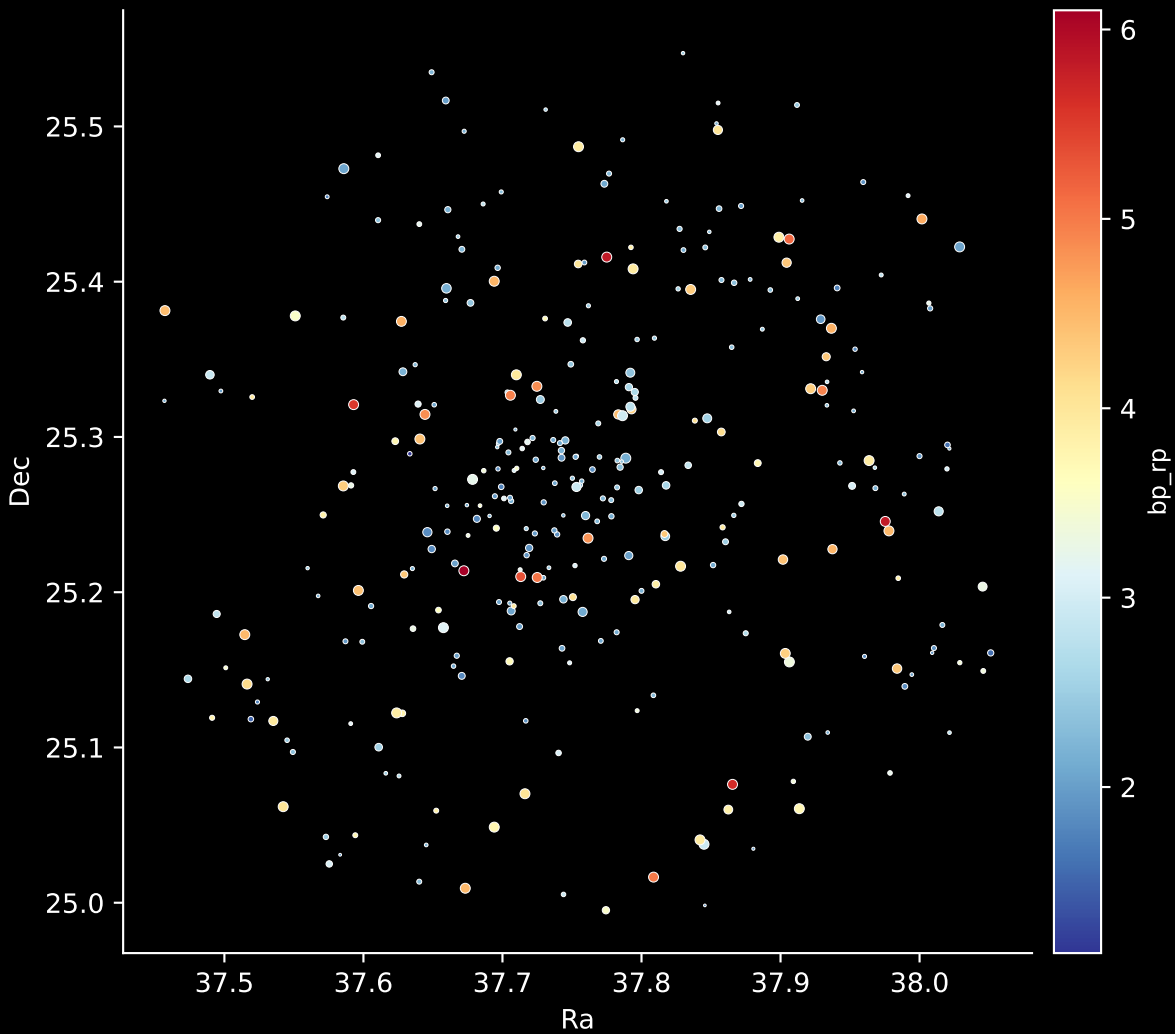
Gaia Cluster: [Czernik_41] Stars: 315
