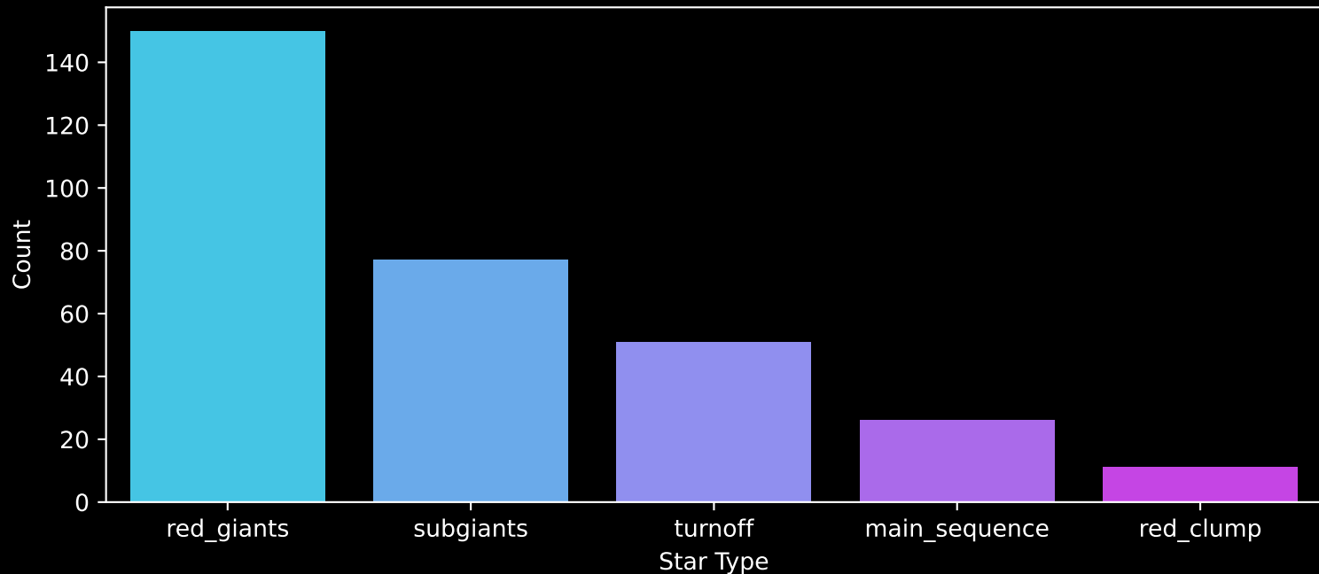
Gaia Cluster: [Czernik_41] Count plot of Star Type
