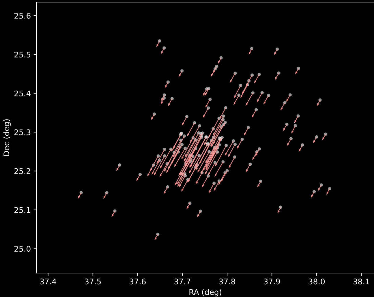
Gaia DR3 Cluster 7 Proper Motion Vectors (n=134)
