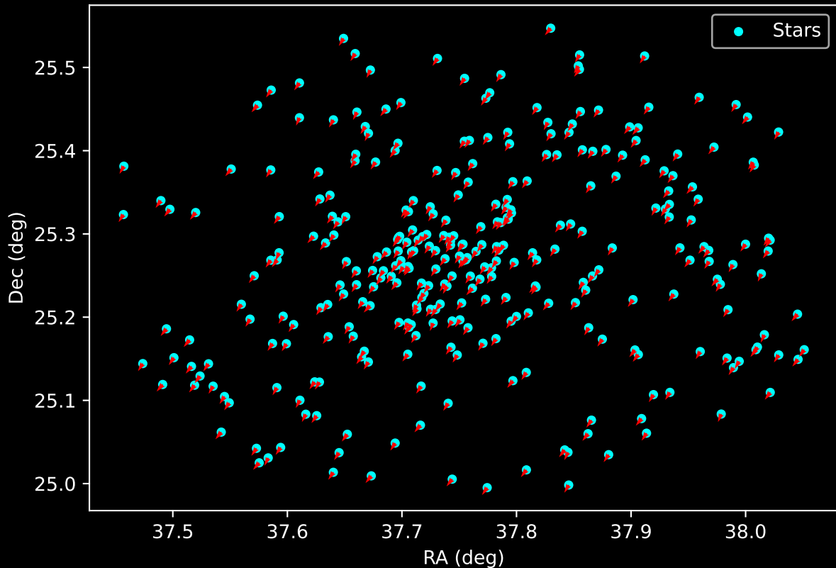
Gaia Cluster: [Czernik_41] Proper Motion Vectors for Gaia Star Field (n= 315)
