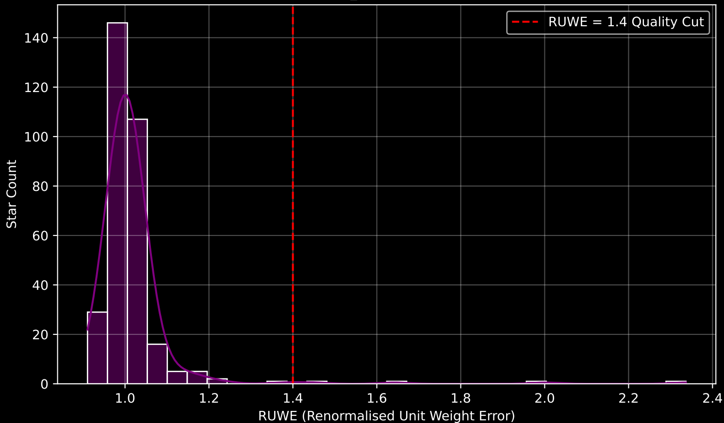
Gaia Cluster: [Czernik_41] RUWE Distribution (n= 315)
