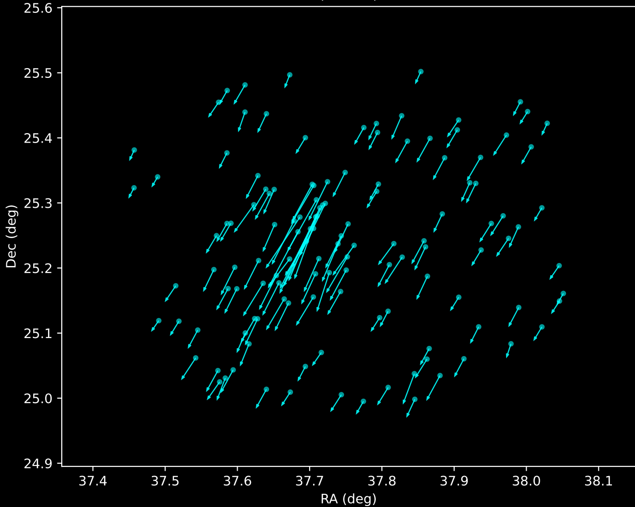
Gaia DR3 Noise Stream Proper Motion Vectors (n=127)
