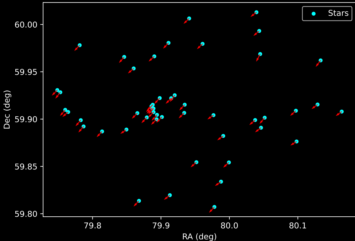
Gaia Cluster: [Czernik_42] Proper Motion Vectors for Gaia Star Field (n= 49)
