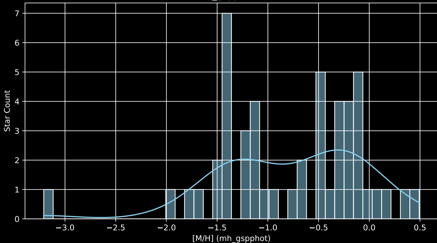
Gaia Cluster: [Czernik_42 [M/H] (mh_gspphot) (n= 49)
