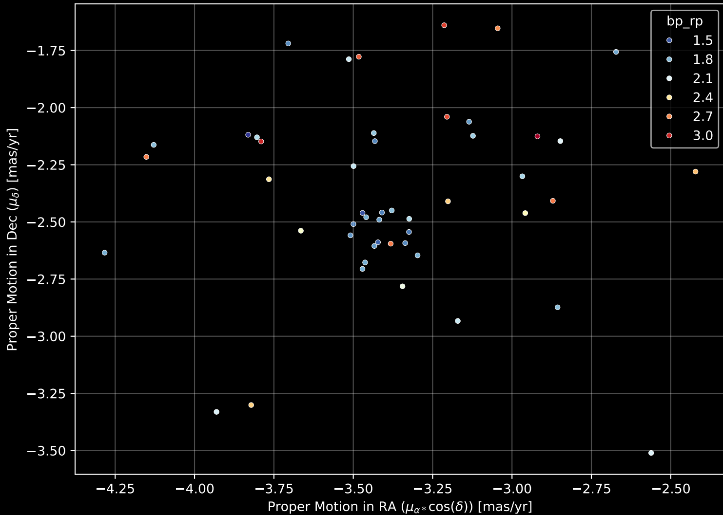
Gaia Cluster: [Czernik_42] Proper Motion Diagram (n= 49)
