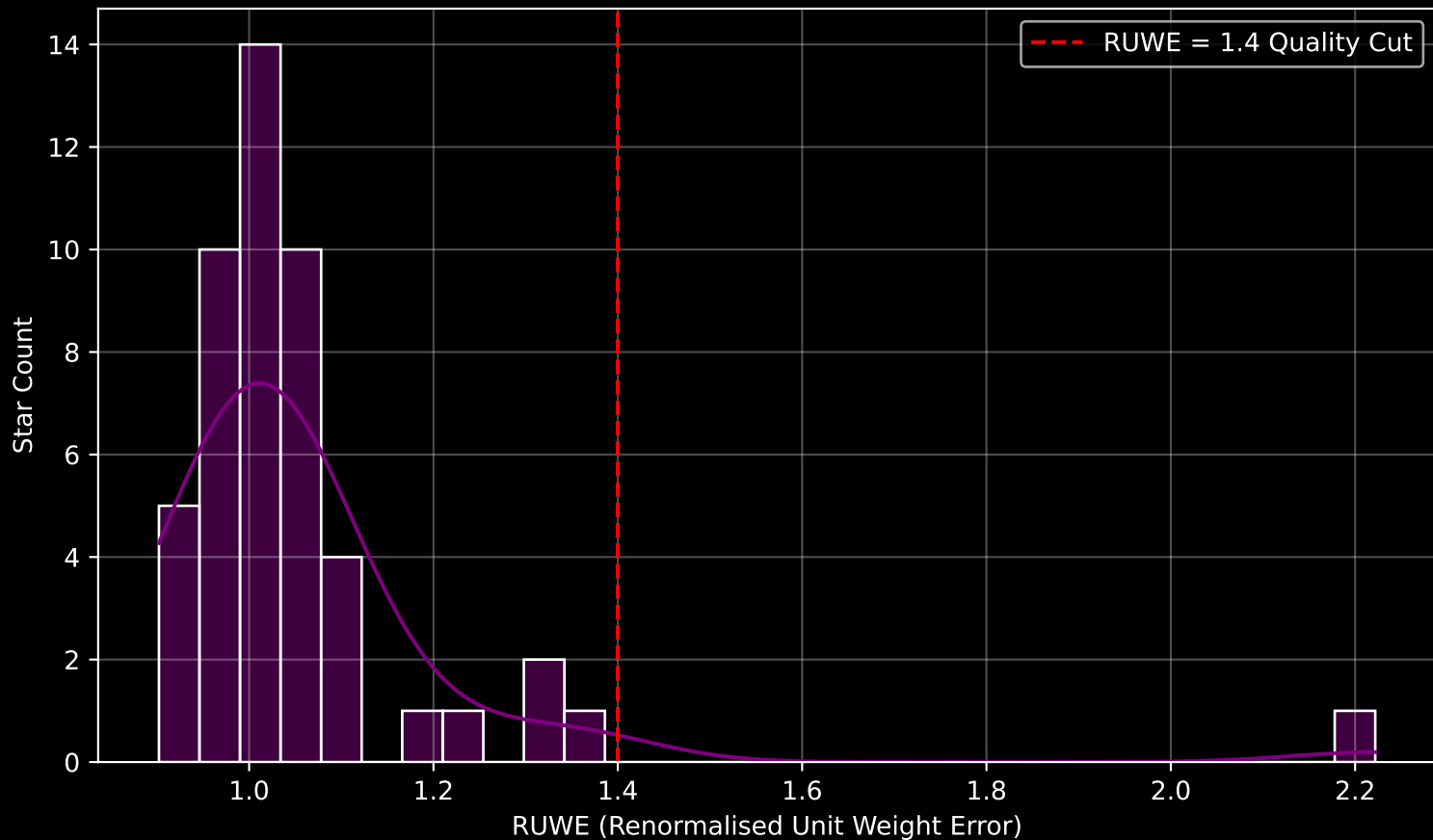
Gaia Cluster: [Czernik_42] RUWE Distribution (n= 49)
