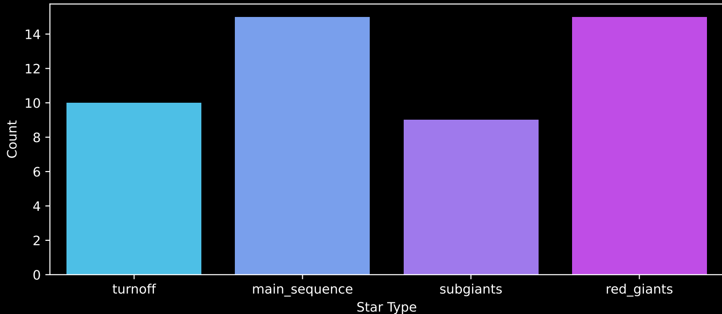
Gaia Cluster: [Czernik_42] Count plot of Star Type
