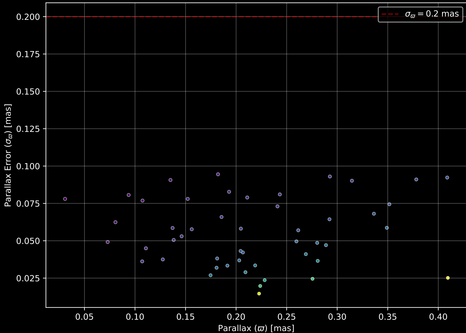
Gaia Cluster: [Czernik_42] Parallax Quality (n= 49)
