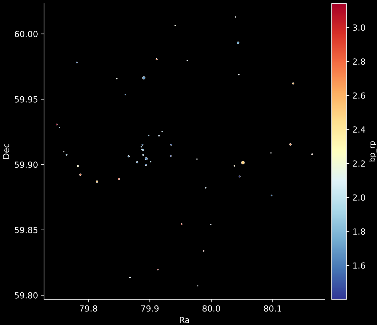
Gaia Cluster: [Czernik_42] Stars: 49
