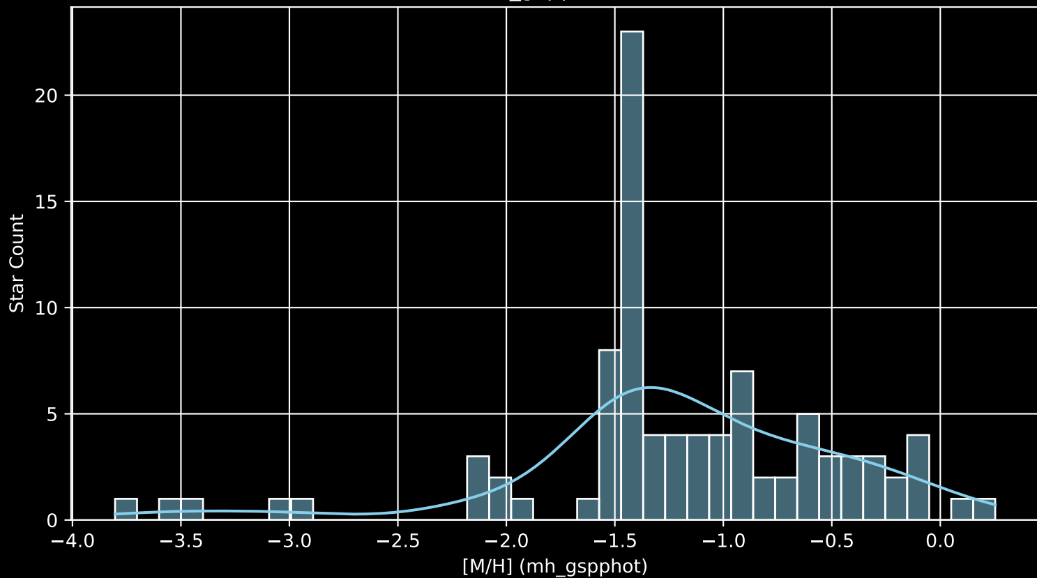
Gaia Cluster: [Czernik_44 [M/H] (mh_gspphot) (n= 92)
