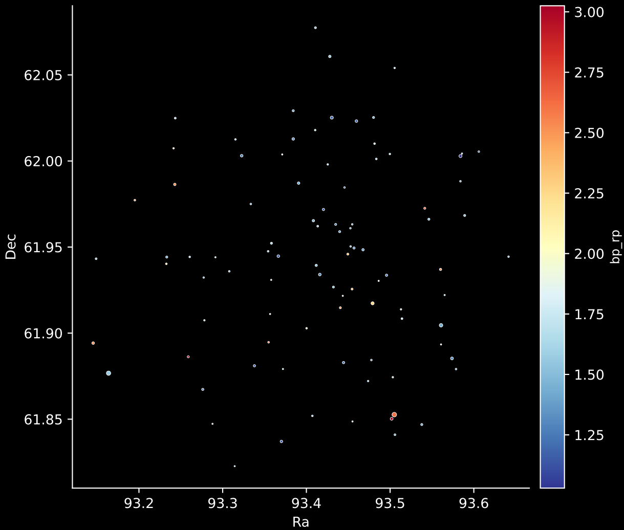
Gaia Cluster: [Czernik_44] Stars: 93
