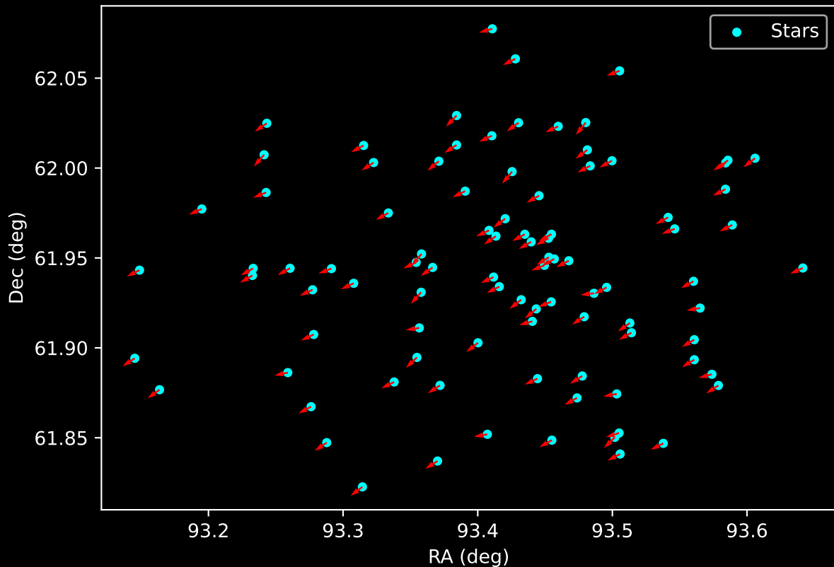
Gaia Cluster: [Czernik_44] Proper Motion Vectors for Gaia Star Field (n= 93)
