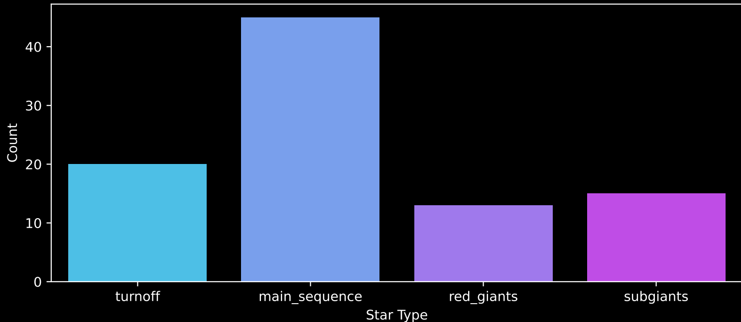
Gaia Cluster: [Czernik_44] Count plot of Star Type
