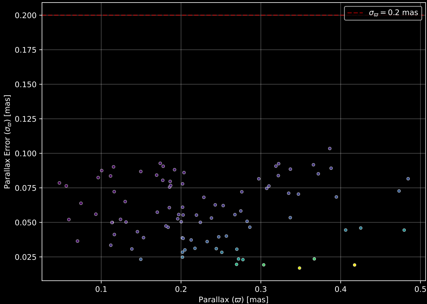
Gaia Cluster: [Czernik_44] Parallax Quality (n= 93)
