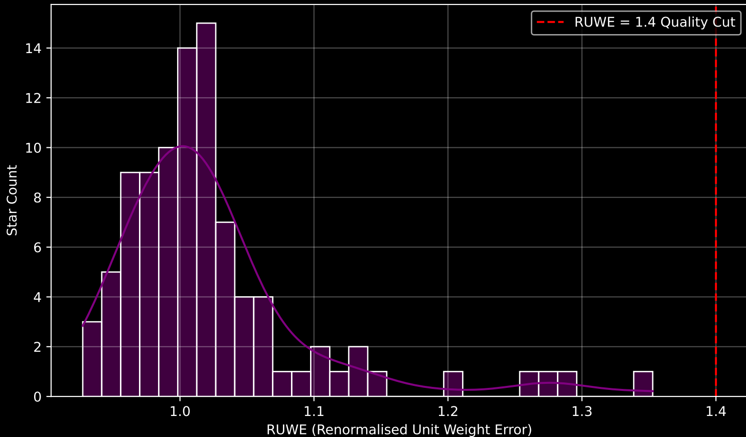
Gaia Cluster: [Czernik_44] RUWE Distribution (n= 93)
