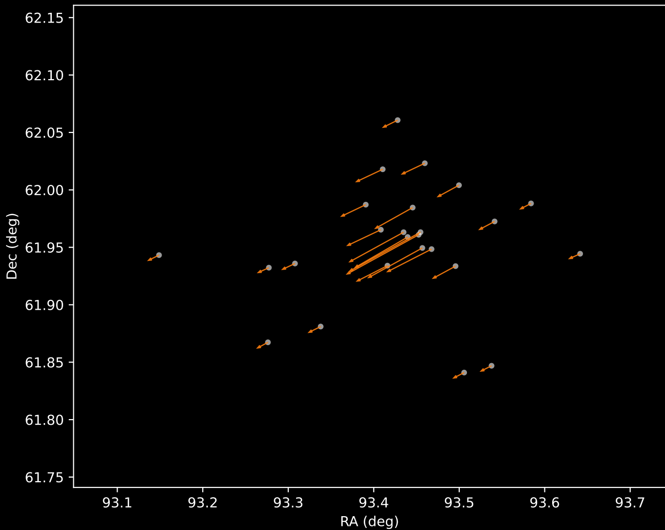
Gaia DR3 Cluster 2 Proper Motion Vectors (n=25)
