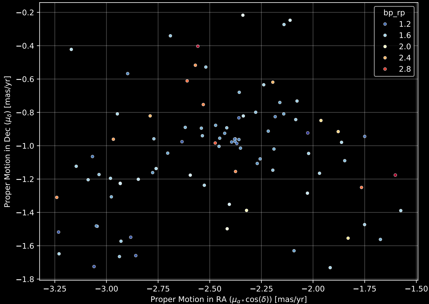
Gaia Cluster: [Czernik_44] Proper Motion Diagram (n= 93)
