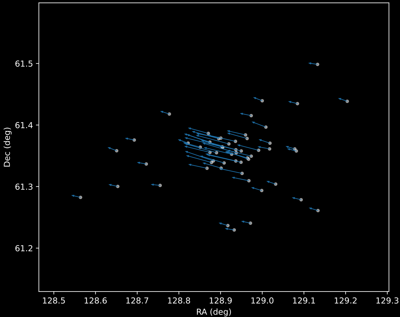
Gaia DR3 Cluster 0 Proper Motion Vectors (n=55)
