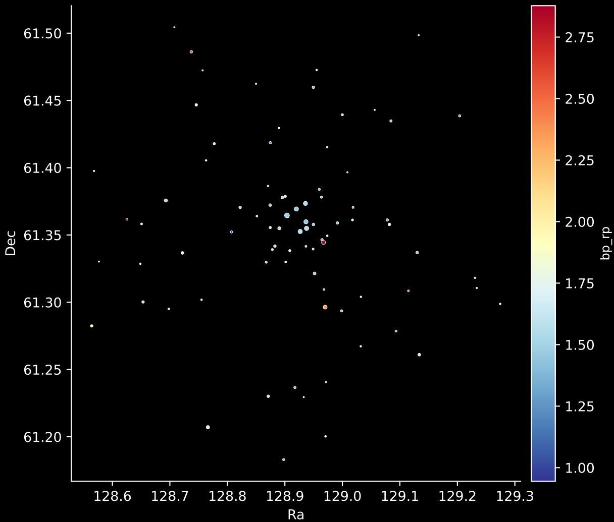
Gaia Cluster: [Czernik_5] Stars: 83
