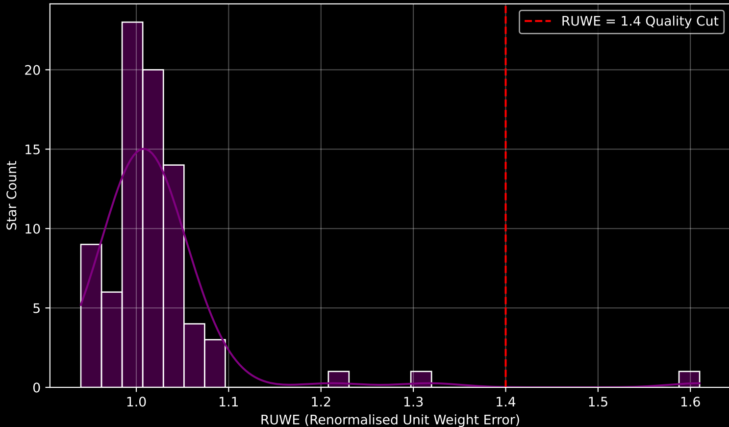
Gaia Cluster: [Czernik_5] RUWE Distribution (n= 82)
