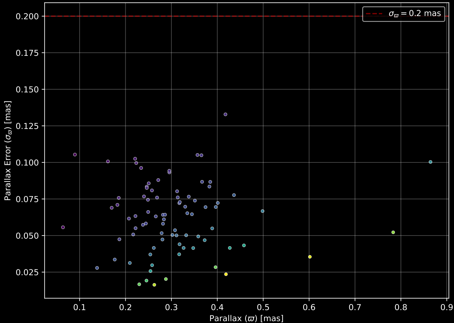
Gaia Cluster: [Czernik_5] Parallax Quality (n= 83)
