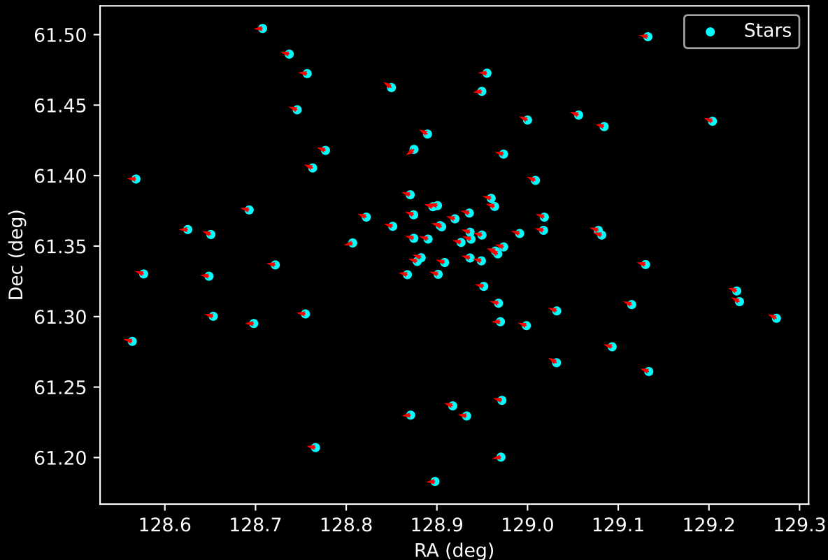
Gaia Cluster: [Czernik_5] Proper Motion Vectors for Gaia Star Field (n= 83)
