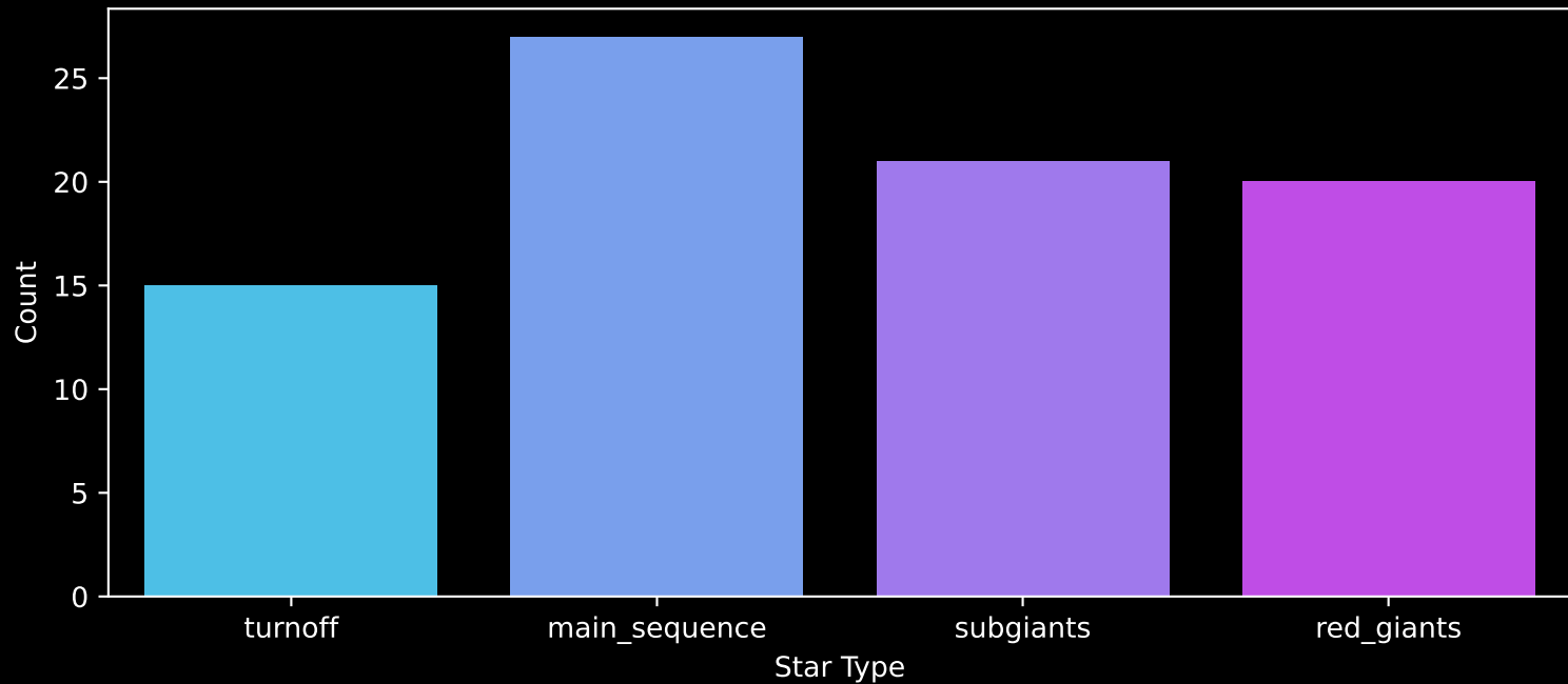
Gaia Cluster: [Czernik_5] Count plot of Star Type
