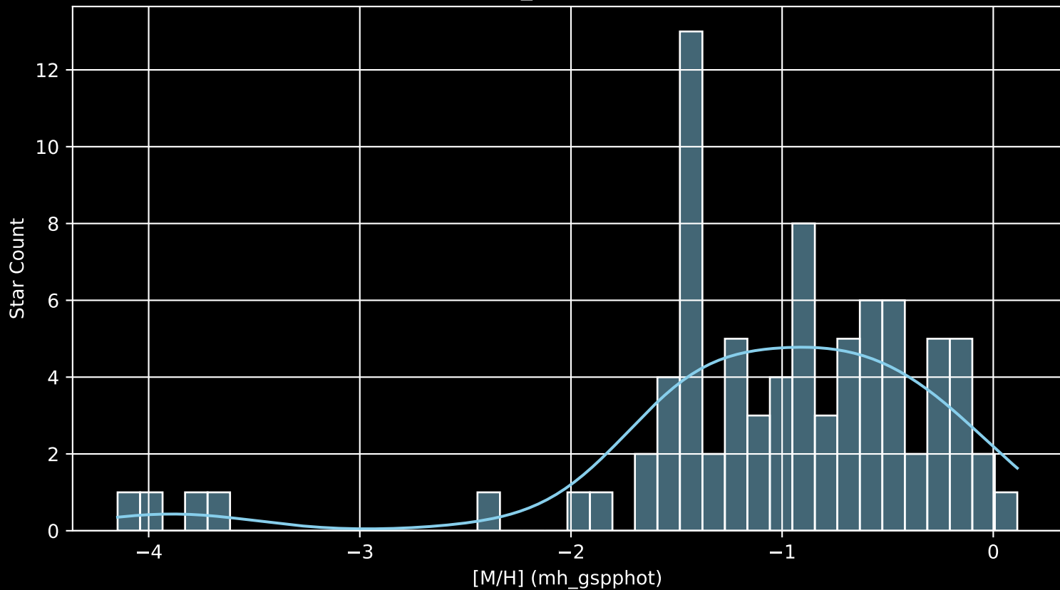
Gaia Cluster: [Czernik_5 [M/H] (mh_gspphot) (n= 83)
