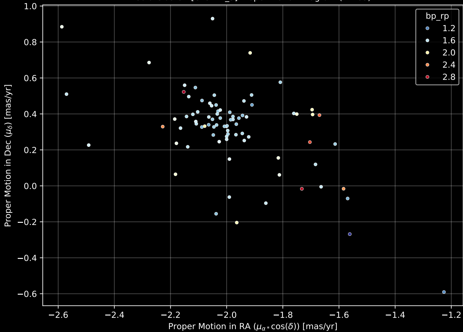
Gaia Cluster: [Czernik_5] Proper Motion Diagram (n= 83)
