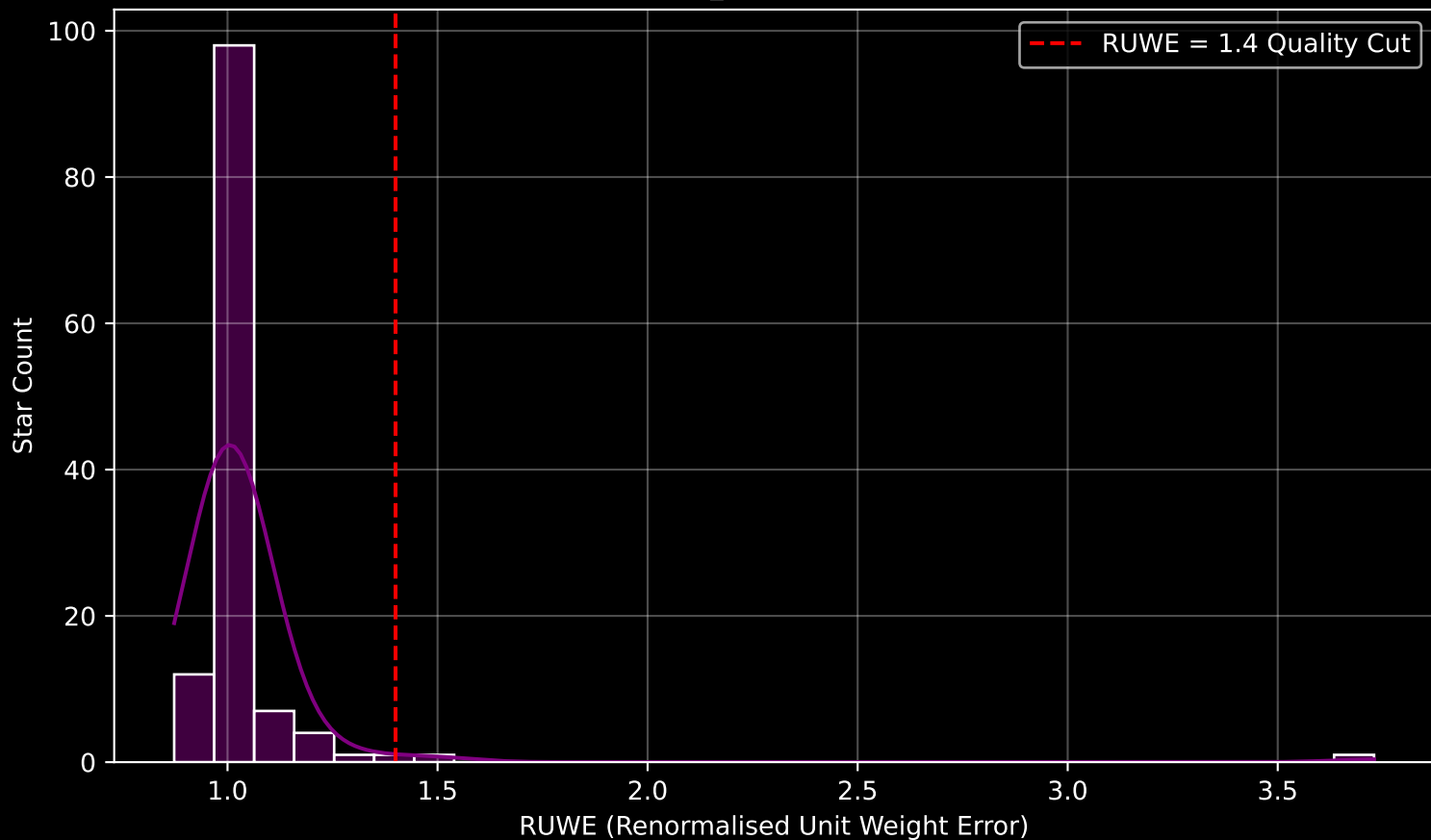
Gaia Cluster: [Czernik_6] RUWE Distribution (n= 125)
