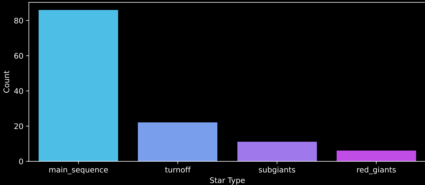
Gaia Cluster: [Czernik_6] Count plot of Star Type
