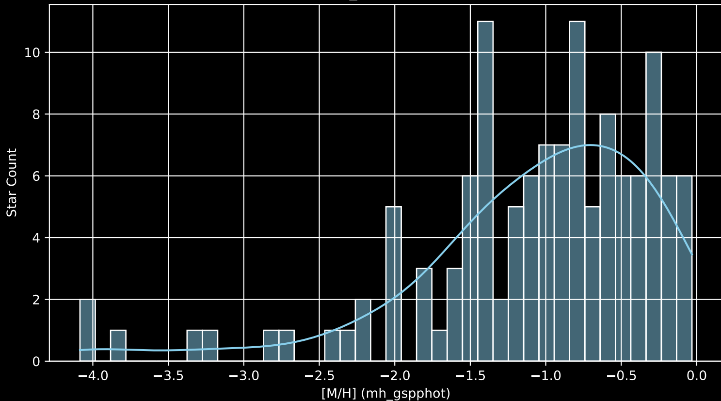
Gaia Cluster: [Czernik_6 [M/H] (mh_gspphot) (n= 125)
