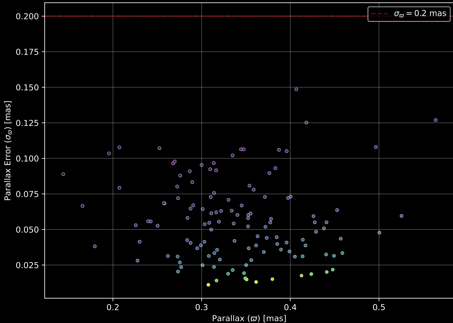
Gaia Cluster: [Czernik_6] Parallax Quality (n= 125)
