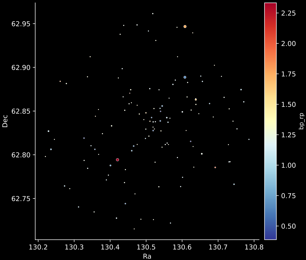
Gaia Cluster: [Czernik_6] Stars: 125
