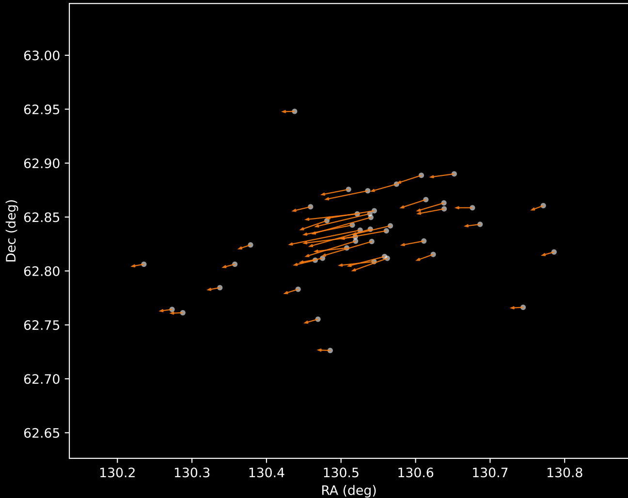
Gaia DR3 Cluster 2 Proper Motion Vectors (n=45)
