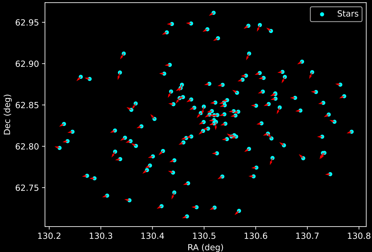
Gaia Cluster: [Czernik_6] Proper Motion Vectors for Gaia Star Field (n= 125)
