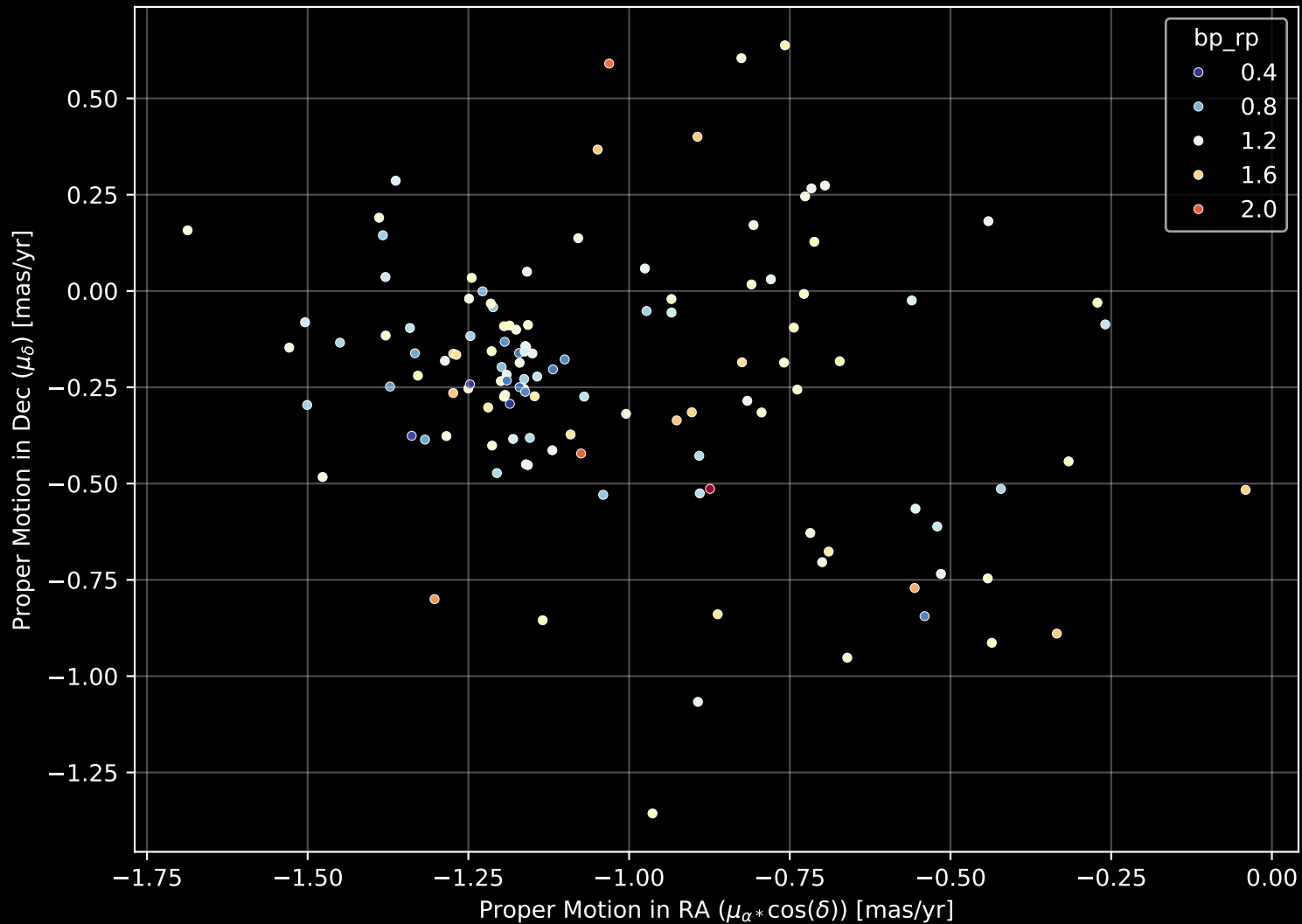
Gaia Cluster: [Czernik_6] Proper Motion Diagram (n= 125)
