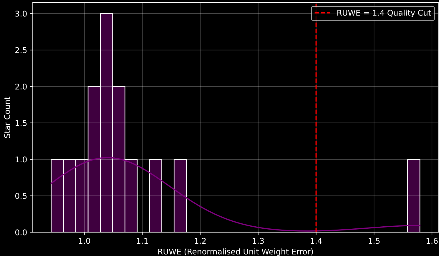
Gaia Cluster: [DB2001_22] RUWE Distribution (n= 14)
