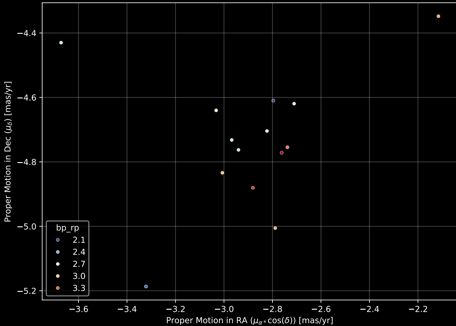
Gaia Cluster: [DB2001_22] Proper Motion Diagram (n= 14)
