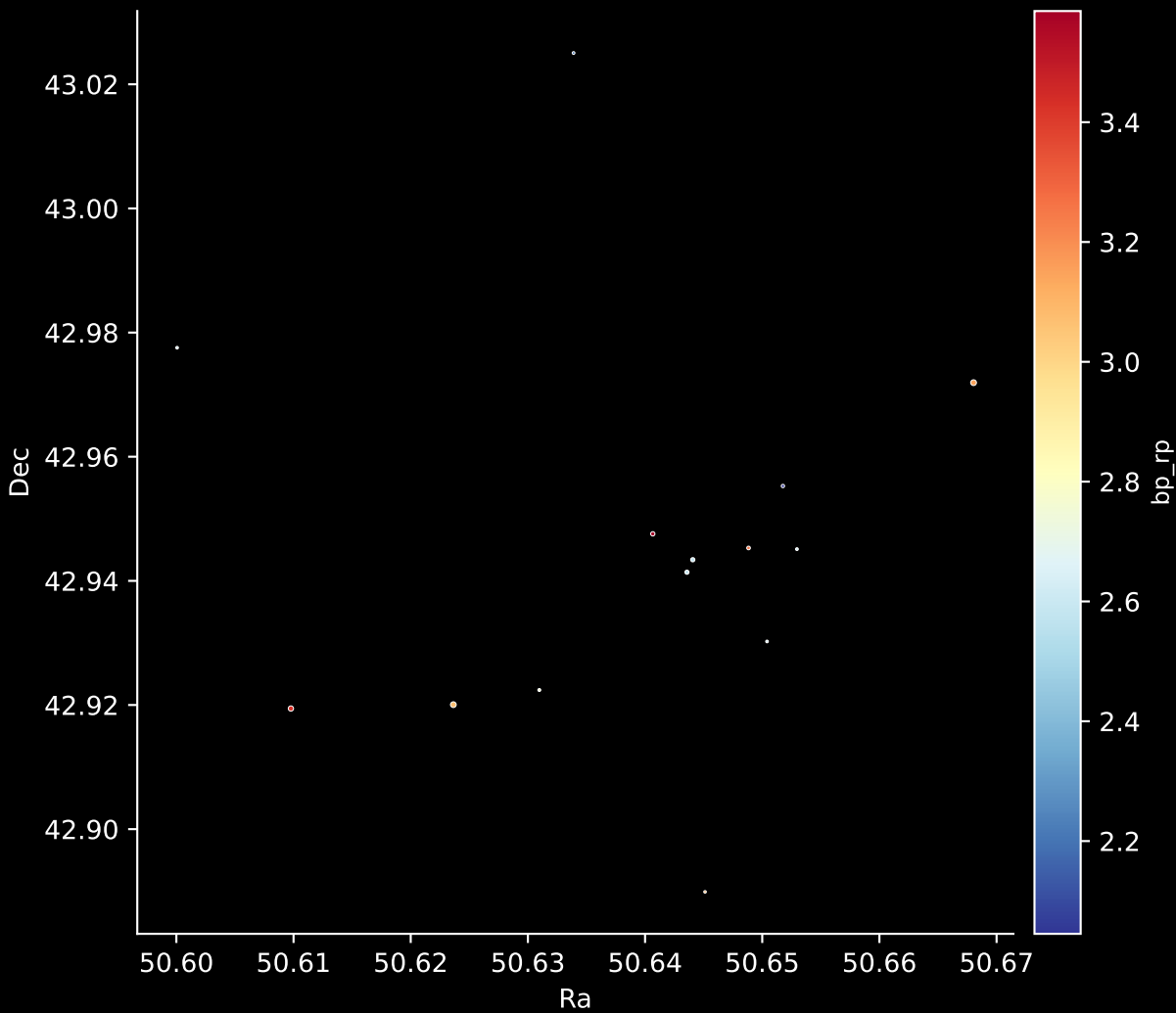
Gaia Cluster: [DB2001_22] Stars: 14
