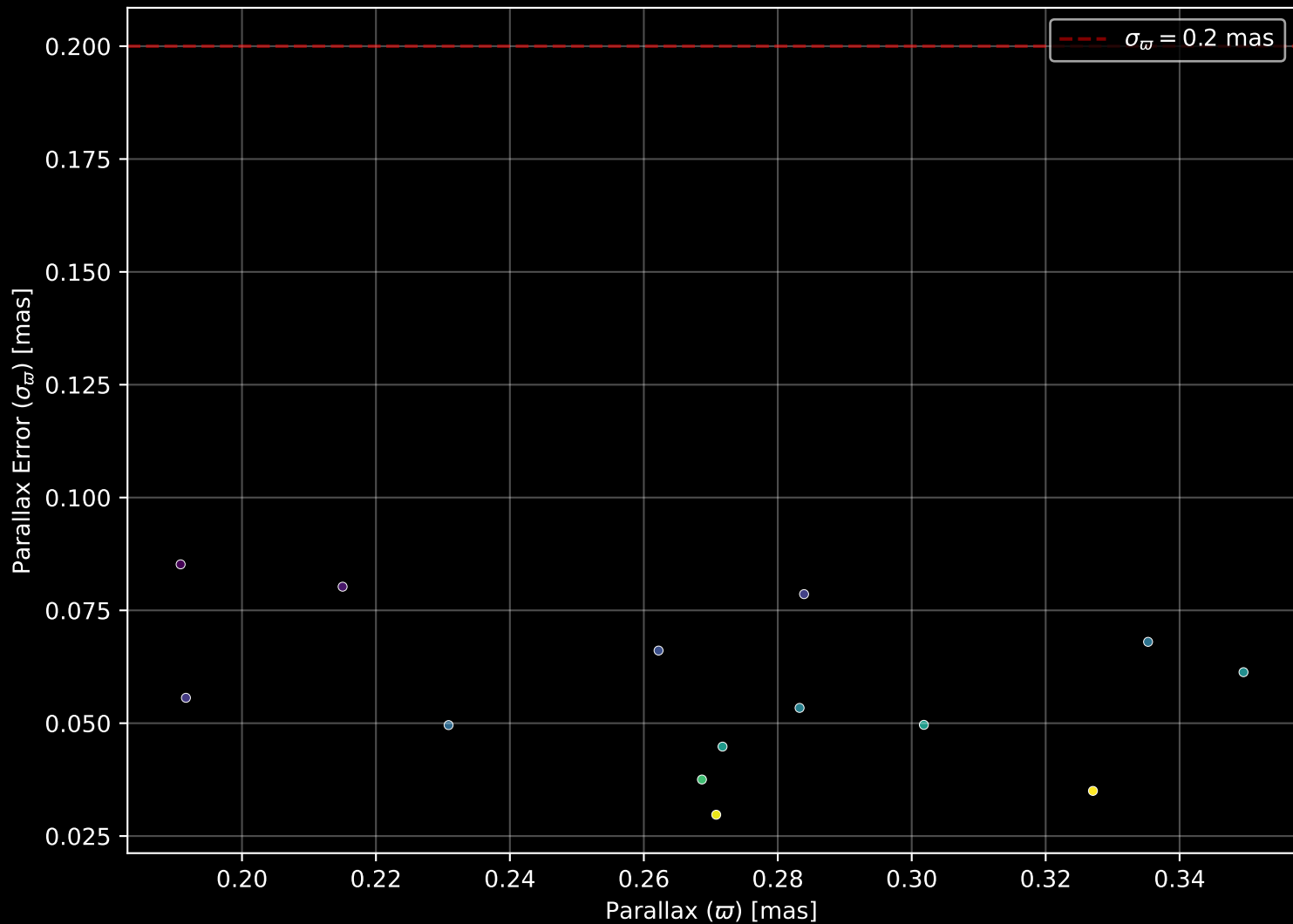
Gaia Cluster: [DB2001_22] Parallax Quality (n= 14)
