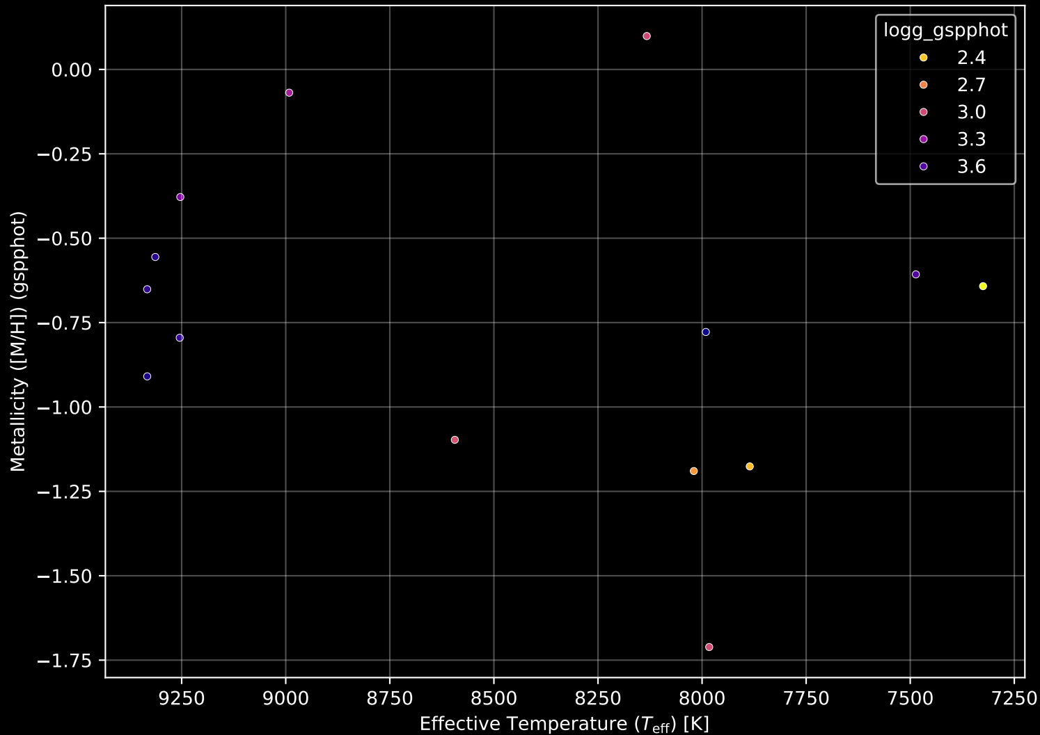
Gaia Cluster: [DB2001_22] Stellar Population Parameters (n= 14)
