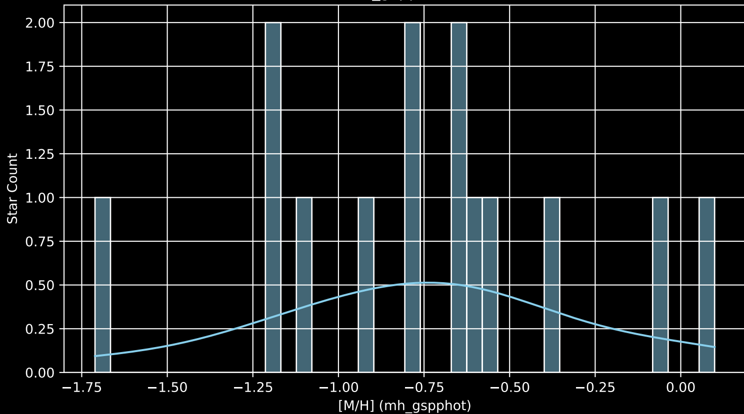
Gaia Cluster: [DB2001_22 [M/H] (mh_gspphot) (n= 14)
