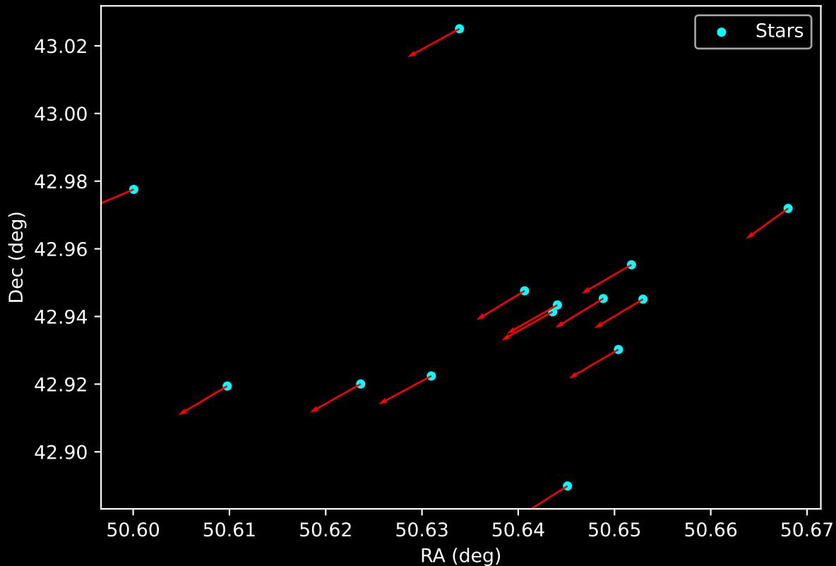
Gaia Cluster: [DB2001_22] Proper Motion Vectors for Gaia Star Field (n= 14)
