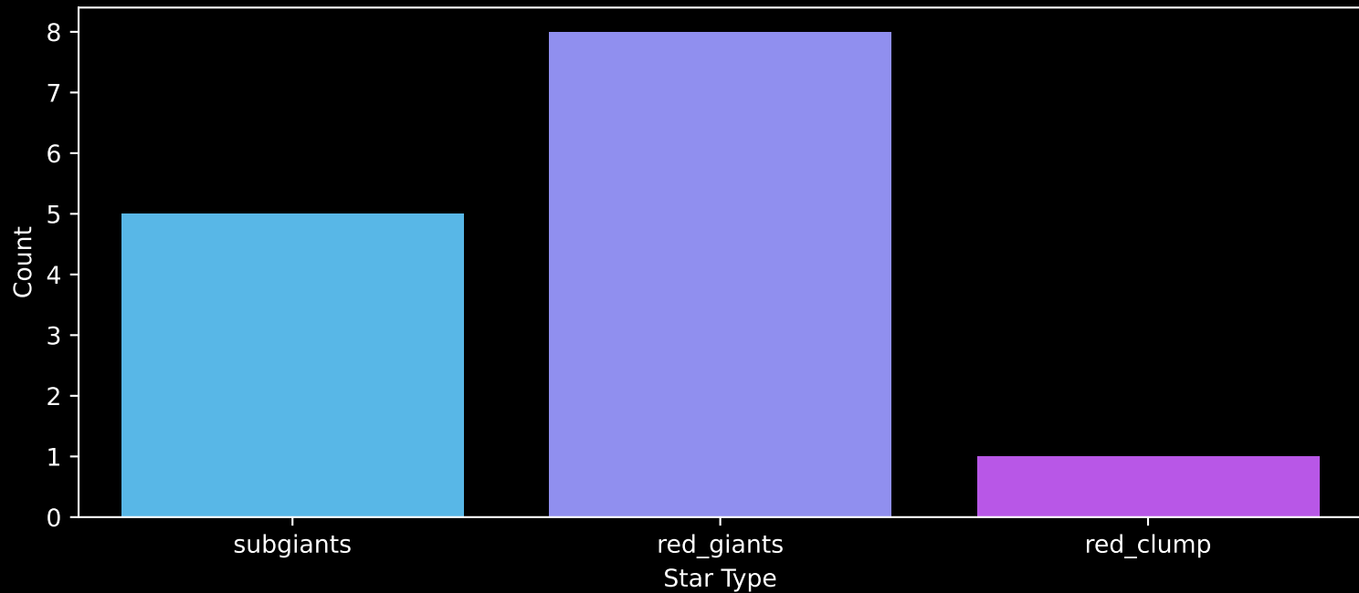
Gaia Cluster: [DB2001_22] Count plot of Star Type
