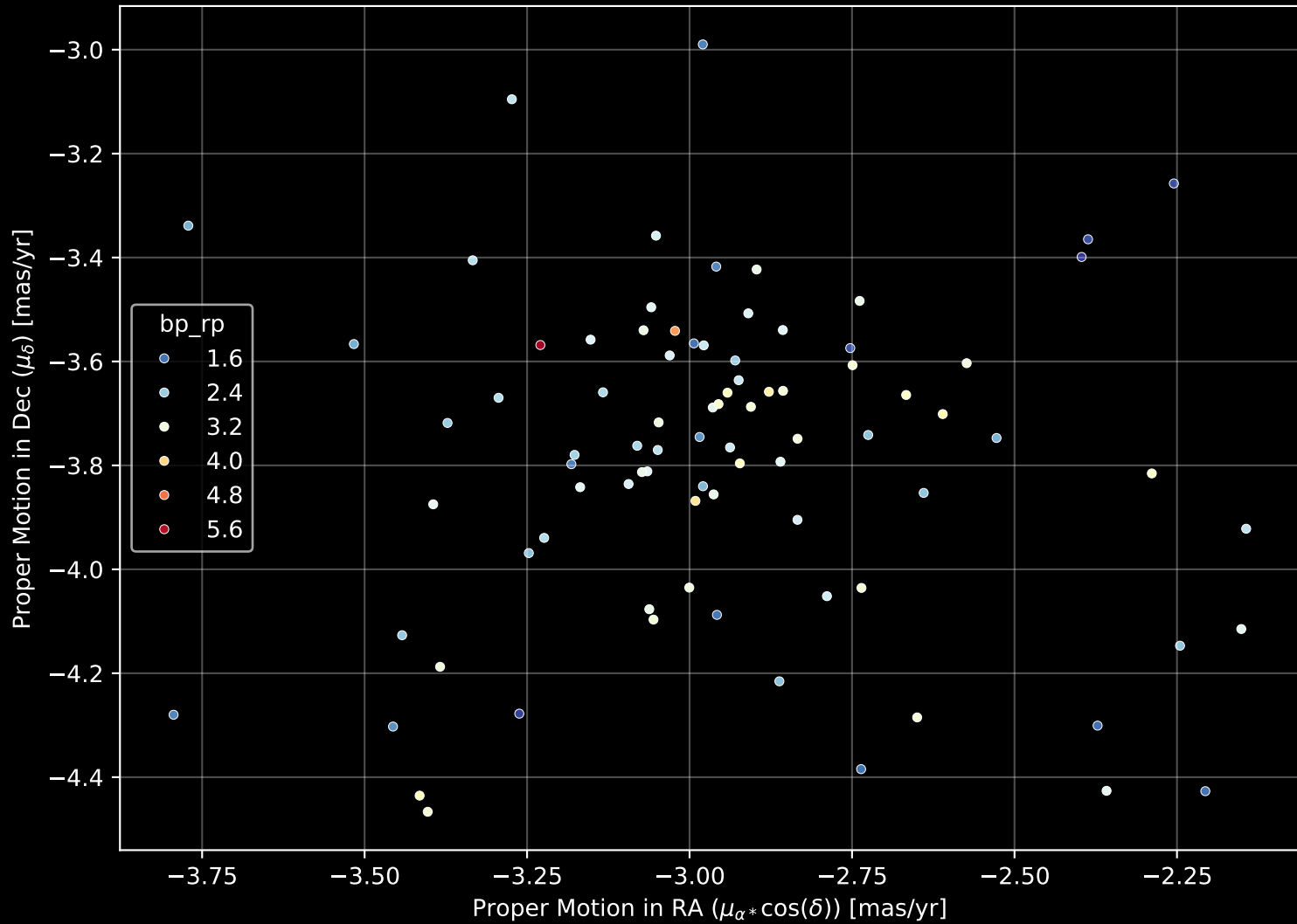
Gaia Cluster: [DBSB_100] Proper Motion Diagram (n= 85)
