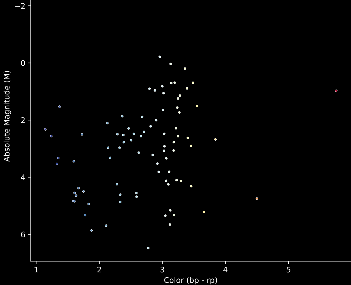
Gaia Cluster: [DBSB_100] Stars ( n = 85 ) Hertzsprung-Russell Diagram
