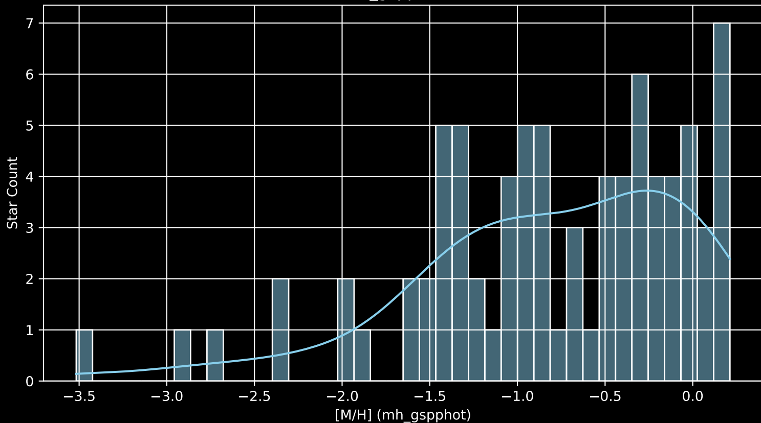
Gaia Cluster: [DBSB_100 [M/H] (mh_gspphot) (n= 81)
