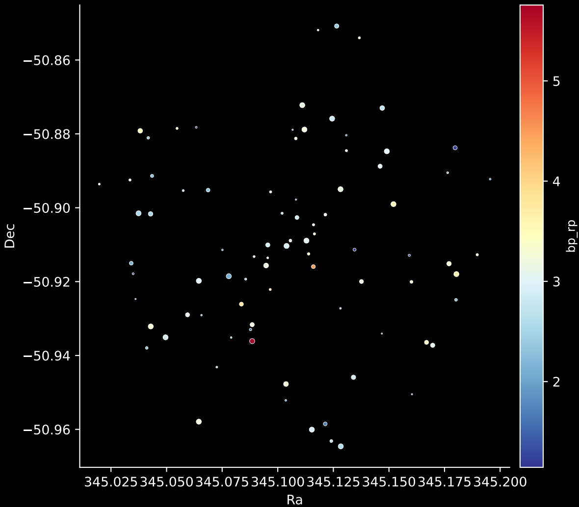
Gaia Cluster: [DBSB_100] Stars: 85
