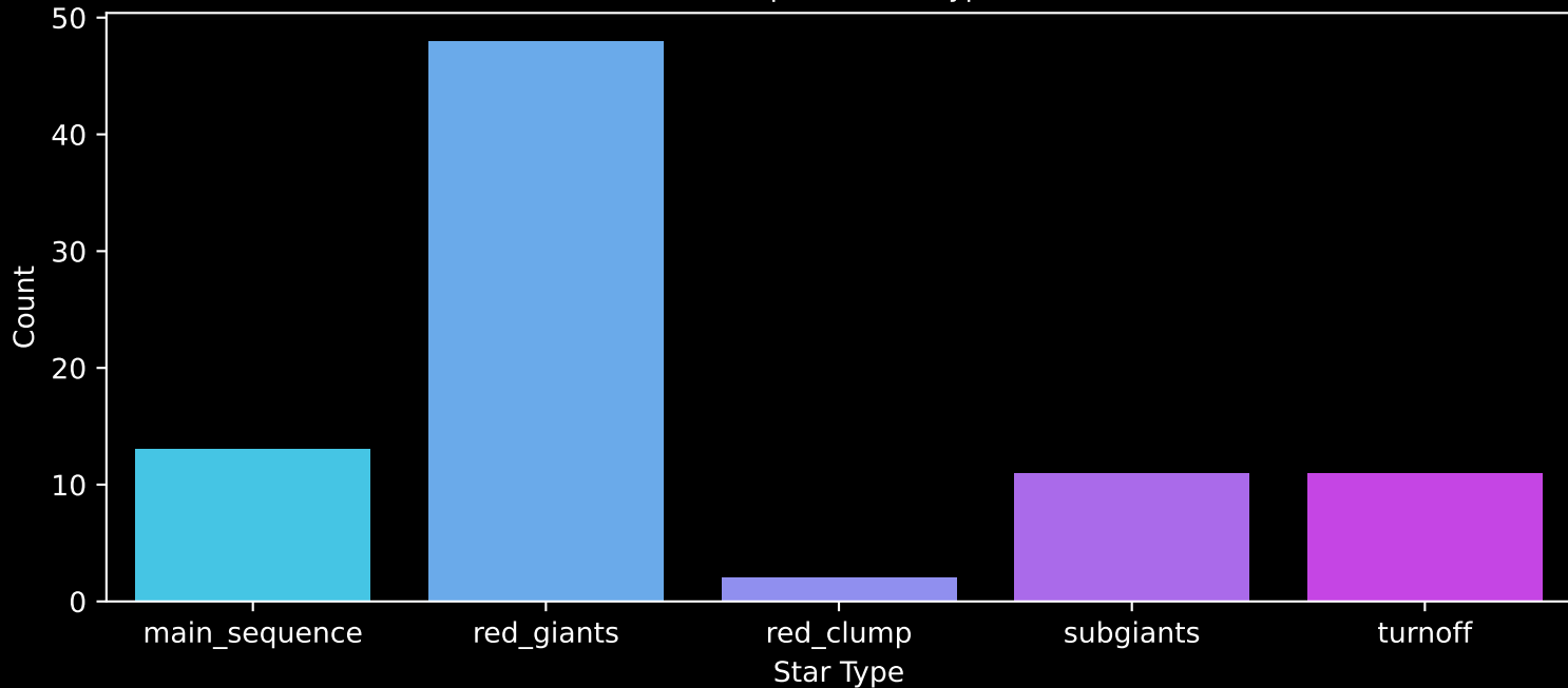
Gaia Cluster: [DBSB_100] Count plot of Star Type
