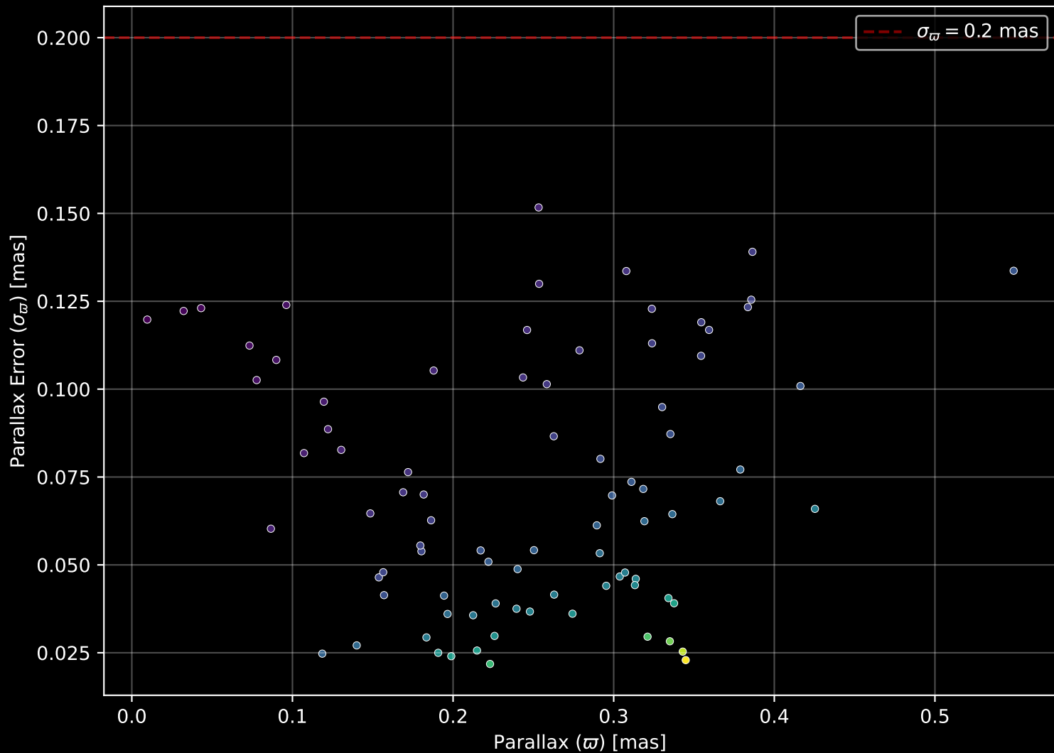
Gaia Cluster: [DBSB_100] Parallax Quality (n= 85)
