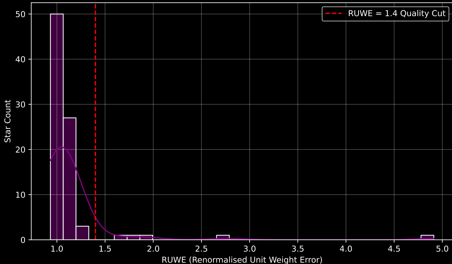
Gaia Cluster: [DBSB_100] RUWE Distribution (n= 85)
