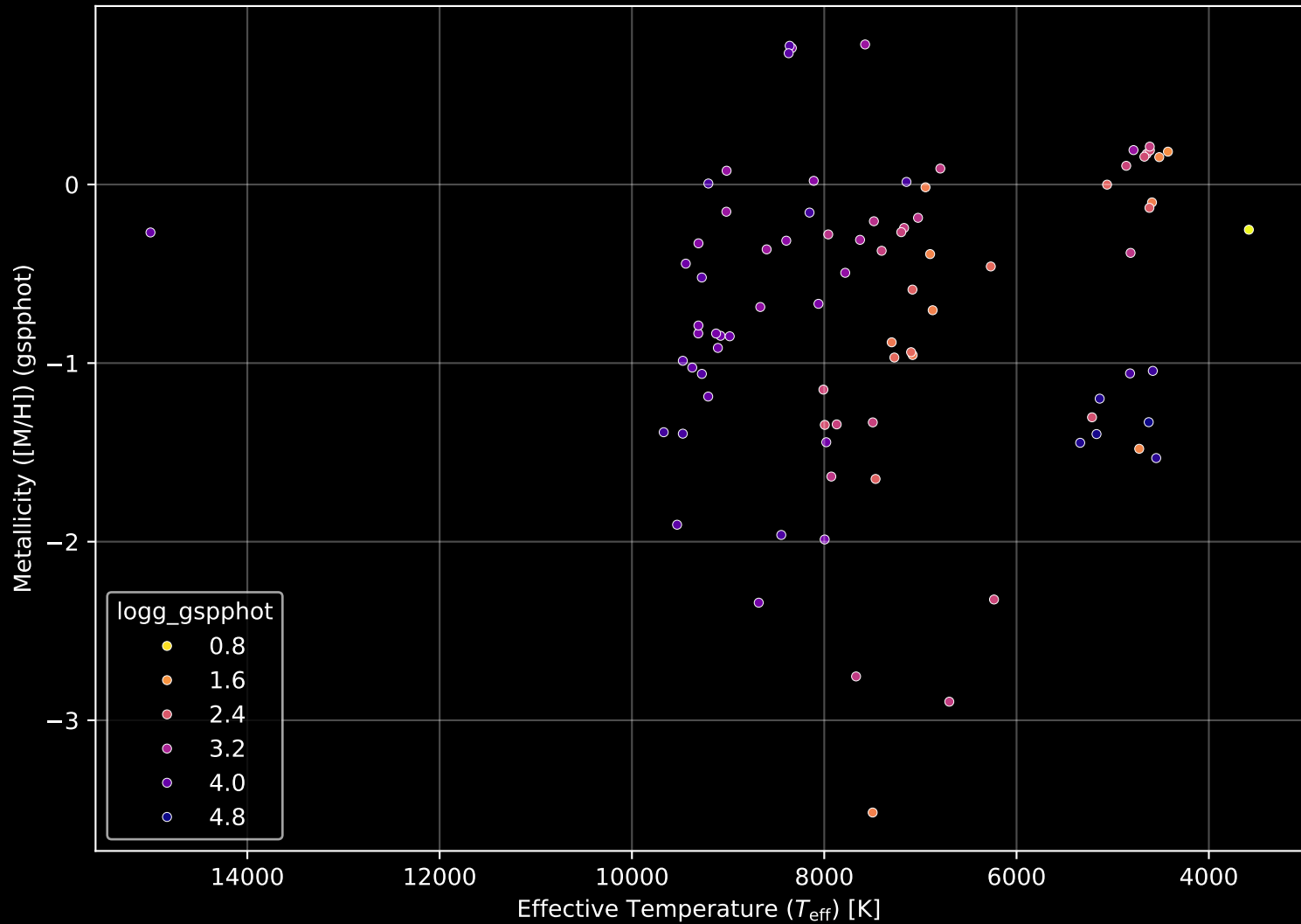
Gaia Cluster: [DBSB_100] Stellar Population Parameters (n= 85)
