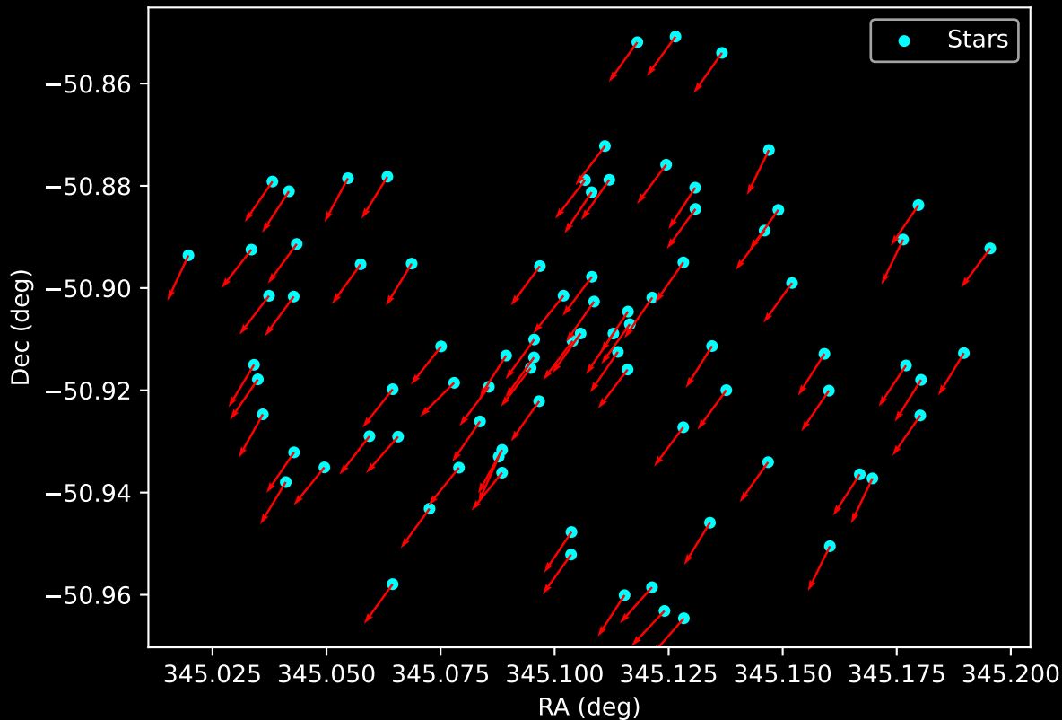
Gaia Cluster: [DBSB_100] Proper Motion Vectors for Gaia Star Field (n= 85)
