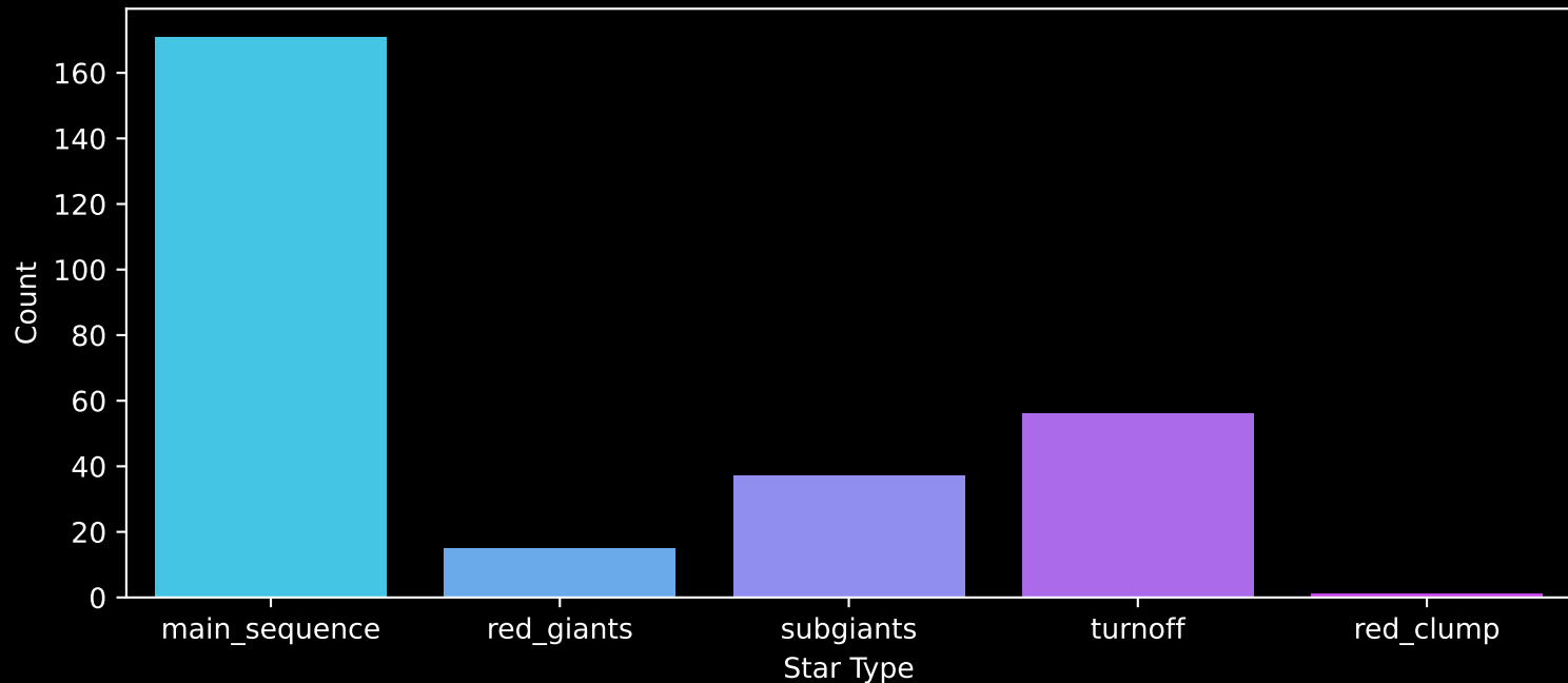
Gaia Cluster: [DBSB_7] Count plot of Star Type
