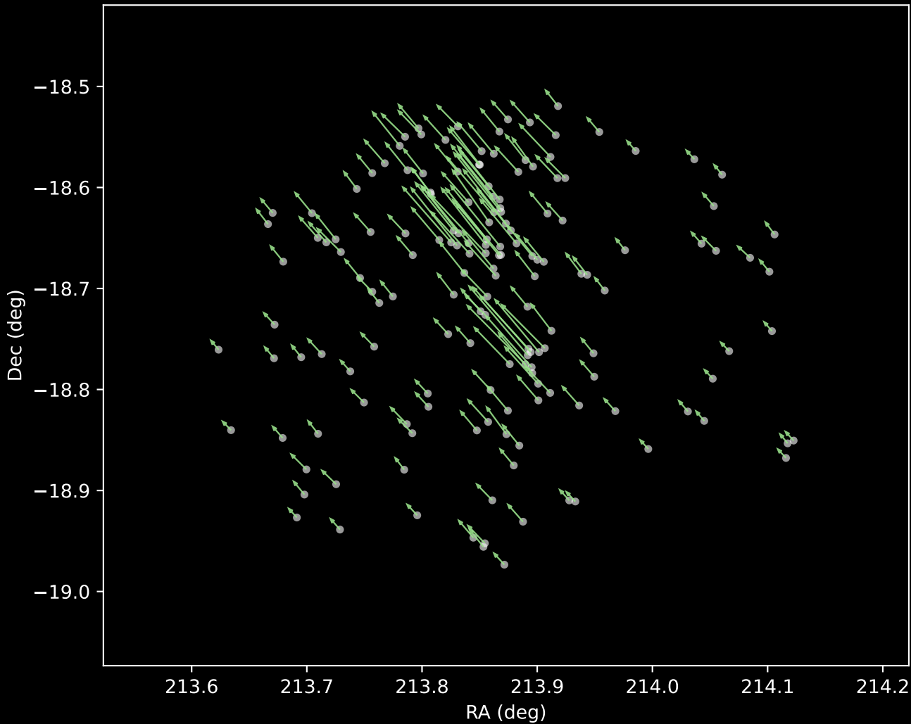
Gaia DR3 Cluster 5 Proper Motion Vectors (n=161)
