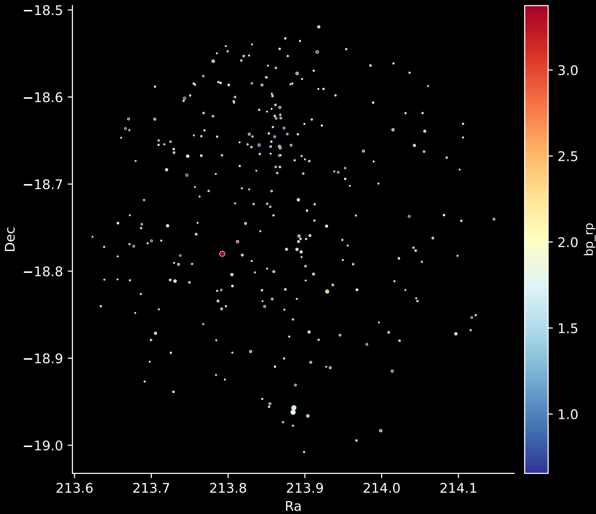
Gaia Cluster: [DBSB_7] Stars: 280
