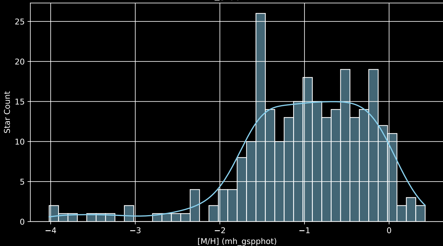
Gaia Cluster: [DBSB_7 [M/H] (mh_gspphot) (n= 278)
