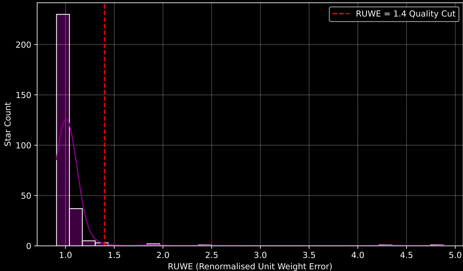
Gaia Cluster: [DBSB_7] RUWE Distribution (n= 280)
