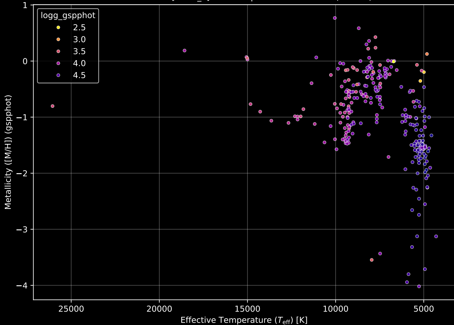
Gaia Cluster: [DBSB_7] Stellar Population Parameters (n= 280)
