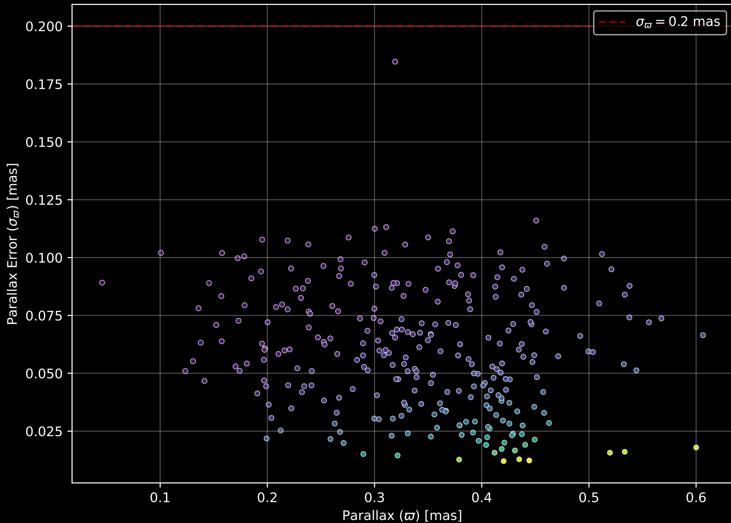
Gaia Cluster: [DBSB_7] Parallax Quality (n= 280)
