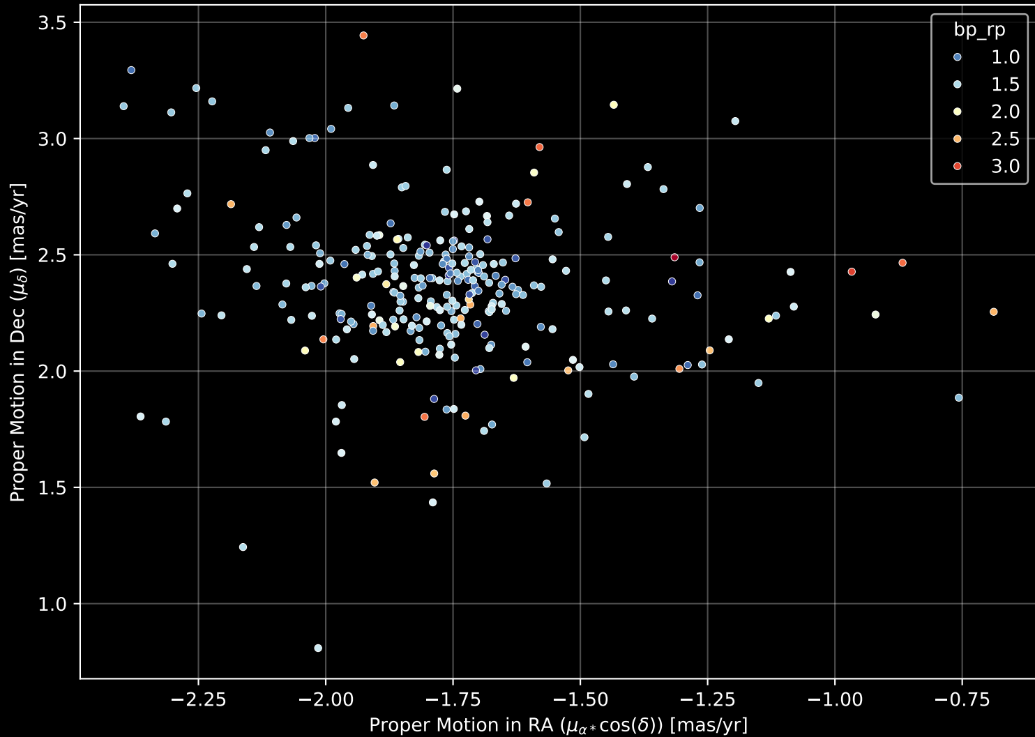
Gaia Cluster: [DBSB_7] Proper Motion Diagram (n= 280)
