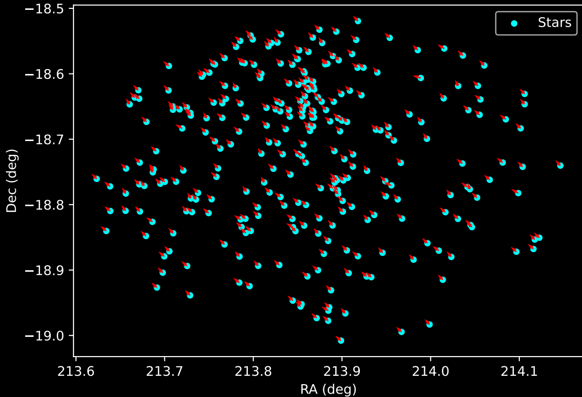
Gaia Cluster: [DBSB_7] Proper Motion Vectors for Gaia Star Field (n= 280)
