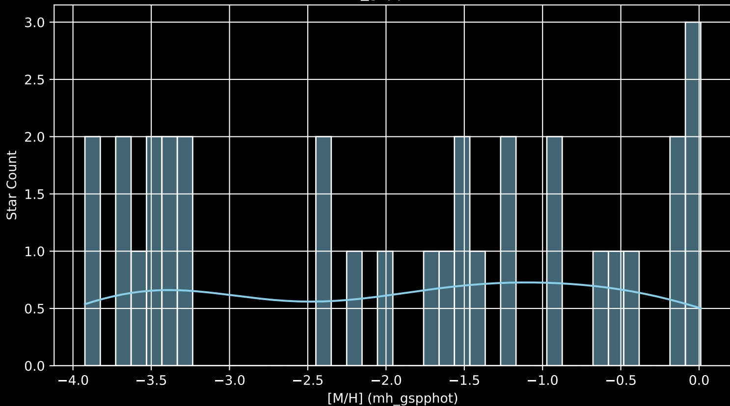
Gaia Cluster: [DC_8 [M/H] (mh_gspphot) (n= 32)
