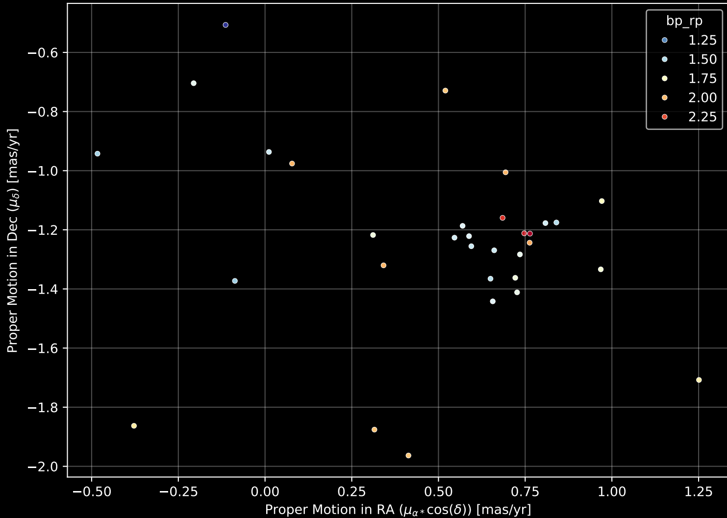
Gaia Cluster: [DC_8] Proper Motion Diagram (n= 32)
