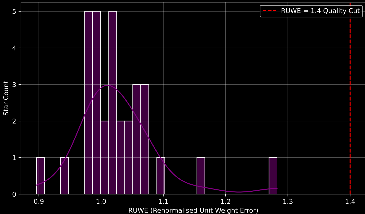
Gaia Cluster: [DC_8] RUWE Distribution (n= 32)
