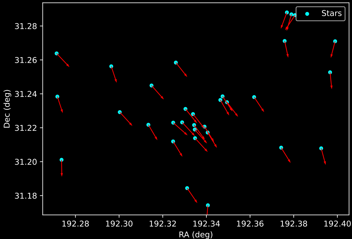
Gaia Cluster: [DC_8] Proper Motion Vectors for Gaia Star Field (n= 32)
