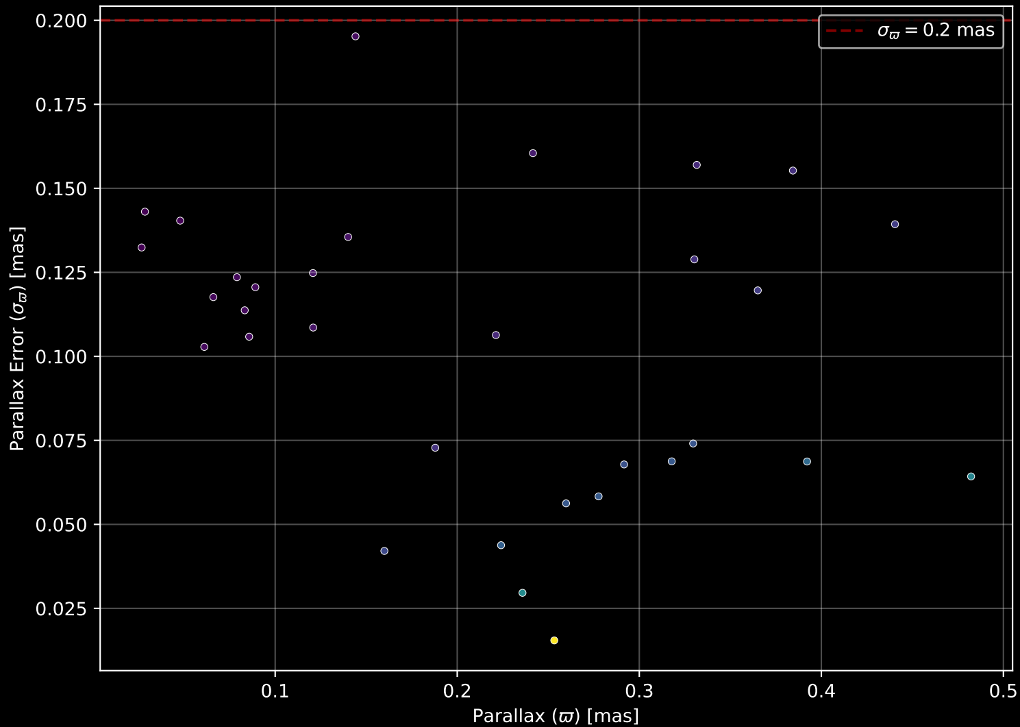
Gaia Cluster: [DC_8] Parallax Quality (n= 32)
