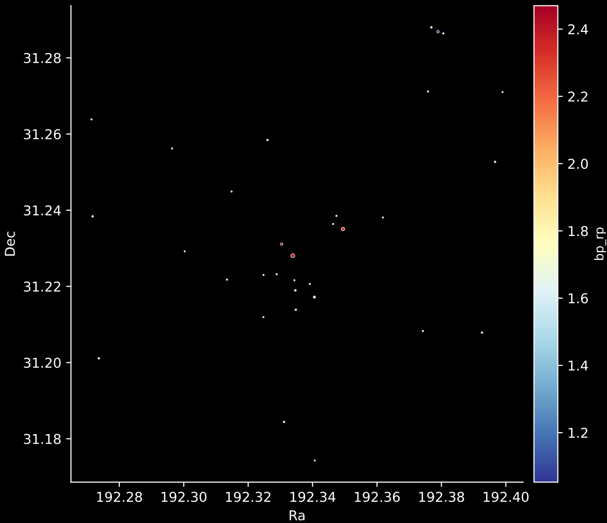
Gaia Cluster: [DC_8] Stars: 32
