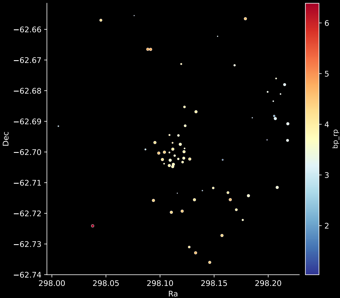
Gaia Cluster: [Danks_1] Stars: 65
