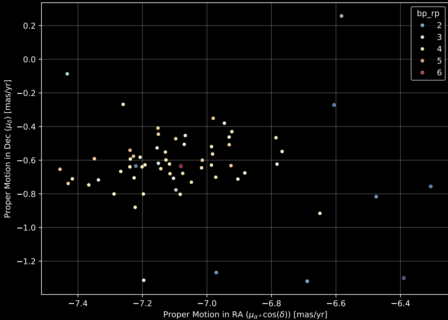
Gaia Cluster: [Danks_1] Proper Motion Diagram (n= 65)
