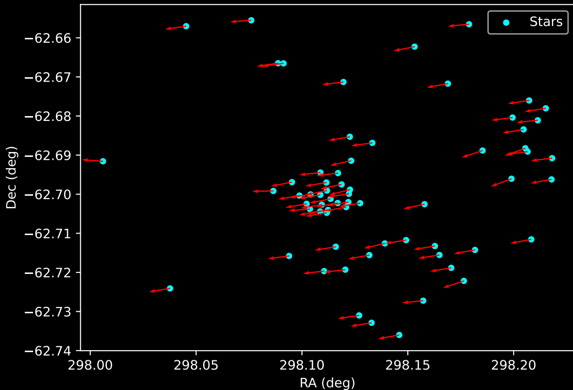
Gaia Cluster: [Danks_1] Proper Motion Vectors for Gaia Star Field (n= 65)
