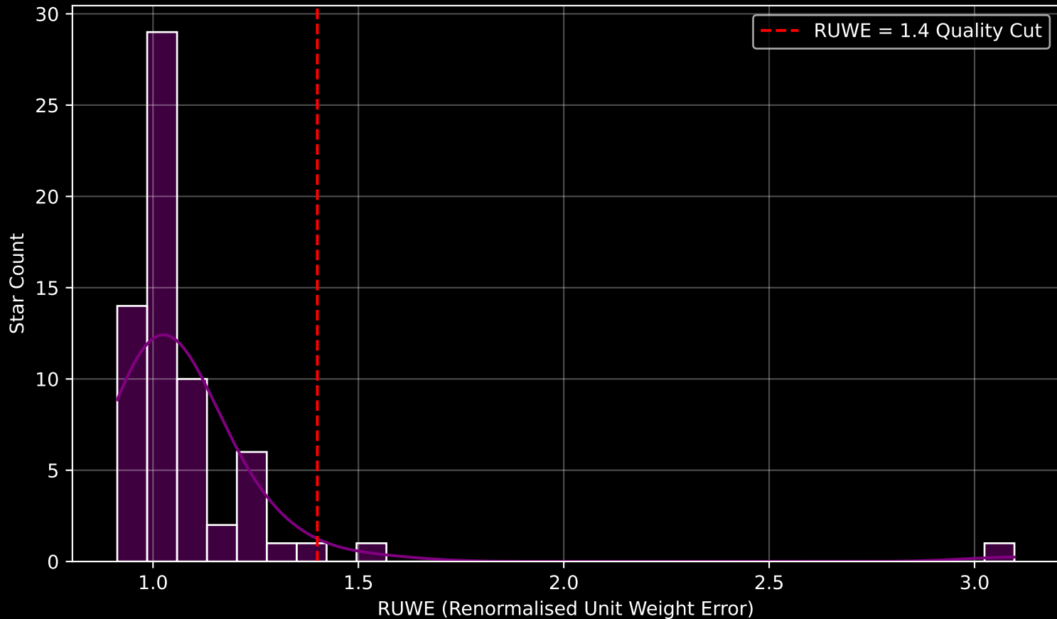
Gaia Cluster: [Danks_1] RUWE Distribution (n= 65)
