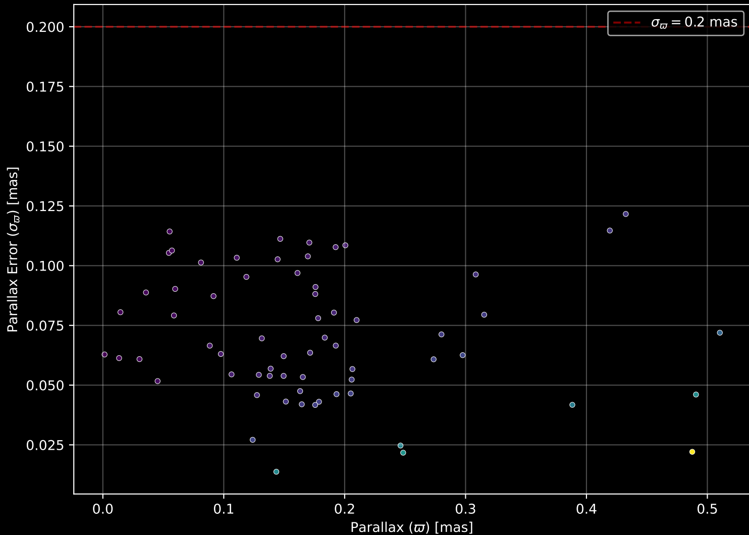
Gaia Cluster: [Danks_1] Parallax Quality (n= 65)
