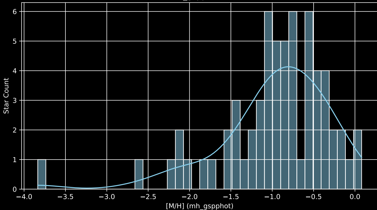
Gaia Cluster: [Danks_1 [M/H] (mh_gspphot) (n= 63)
