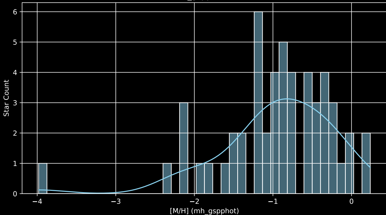
Gaia Cluster: [Danks_2 [M/H] (mh_gspphot) (n= 52)
