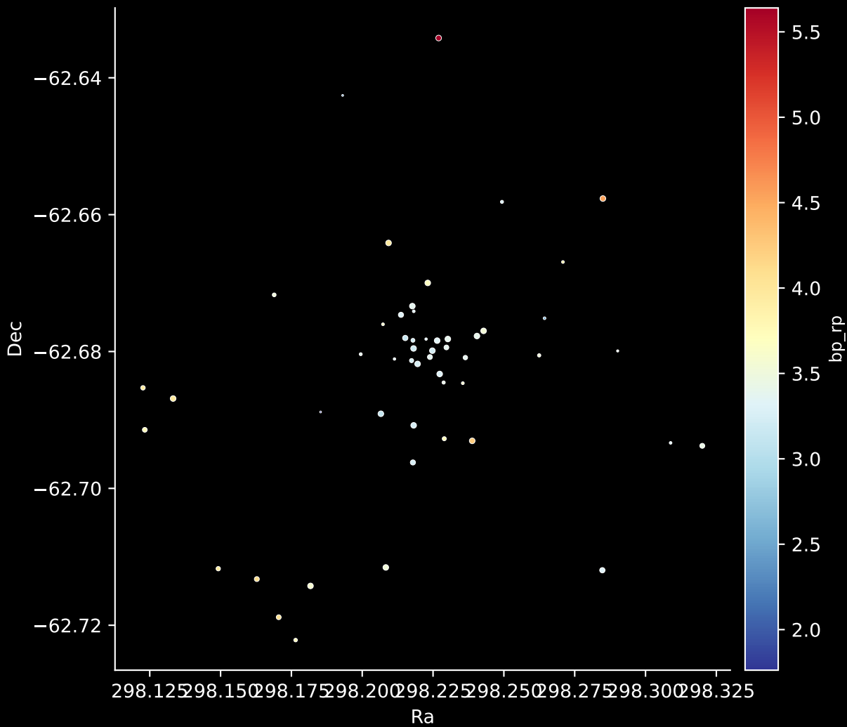
Gaia Cluster: [Danks_2] Stars: 52
