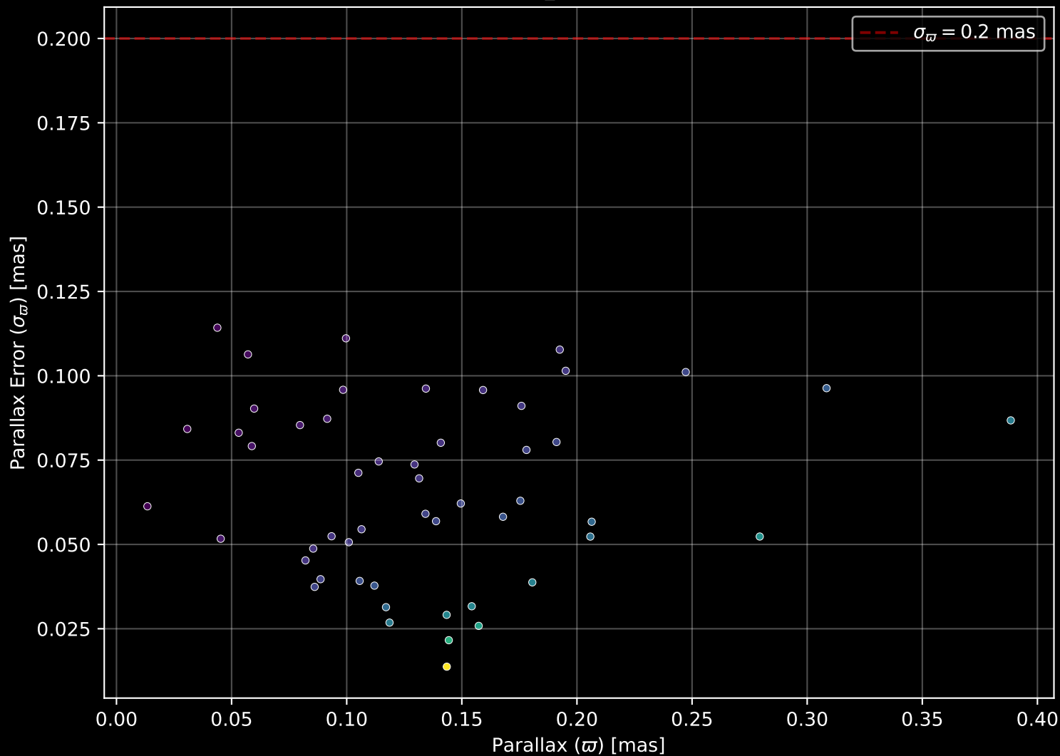
Gaia Cluster: [Danks_2] Parallax Quality (n= 52)
