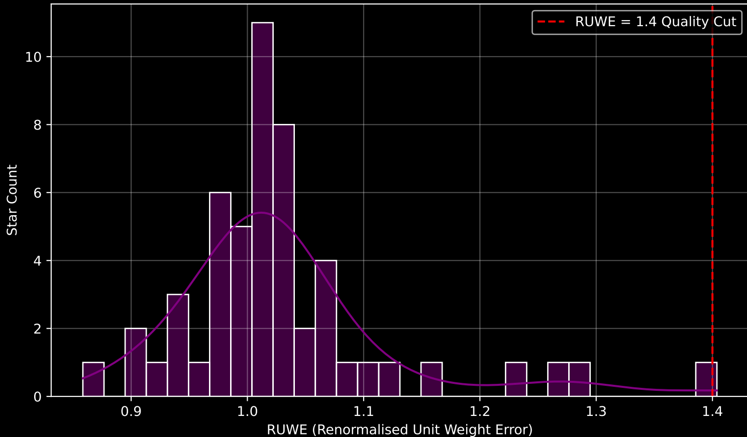
Gaia Cluster: [Danks_2] RUWE Distribution (n= 52)
