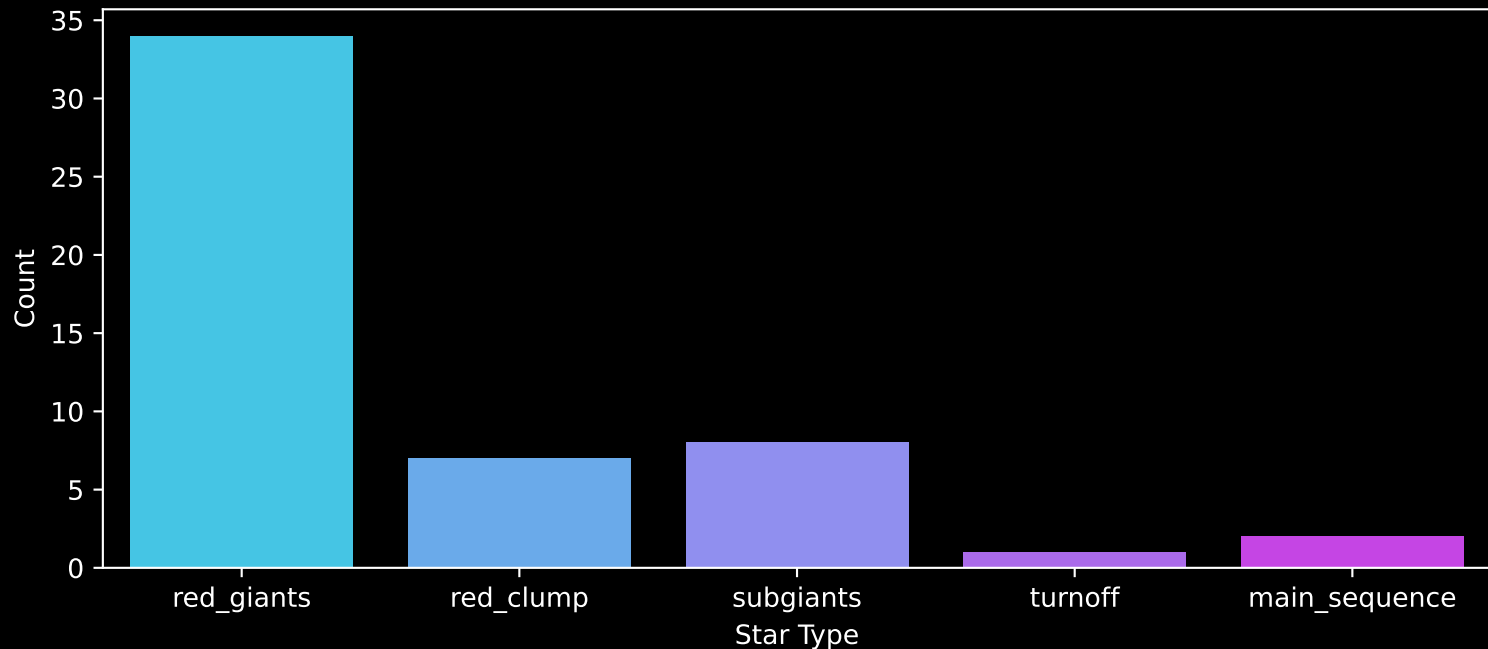
Gaia Cluster: [Danks_2] Count plot of Star Type
