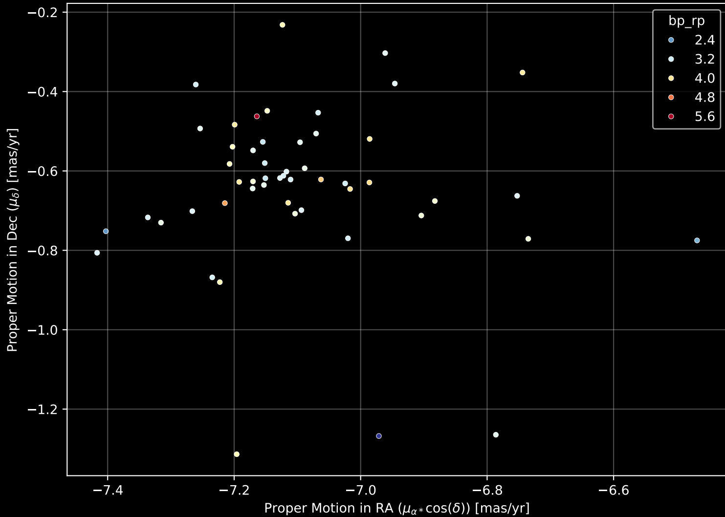
Gaia Cluster: [Danks_2] Proper Motion Diagram (n= 52)
