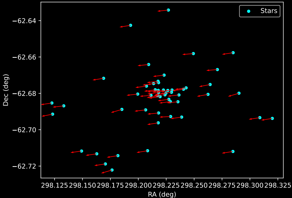
Gaia Cluster: [Danks_2] Proper Motion Vectors for Gaia Star Field (n= 52)
