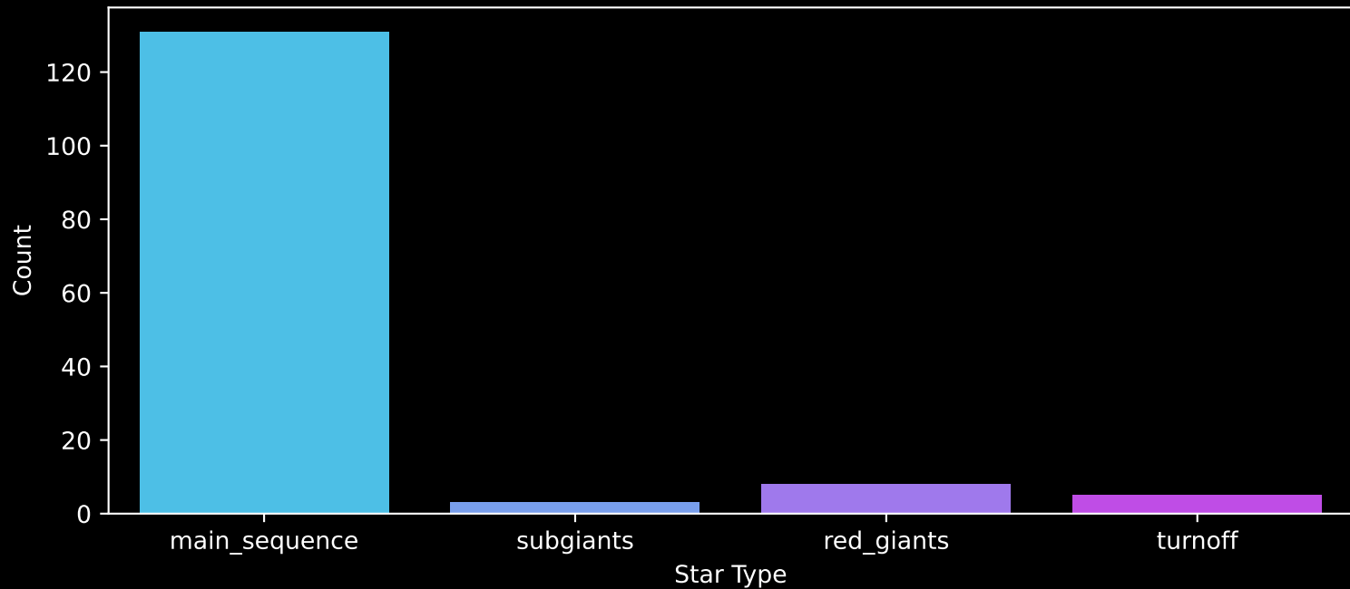
Gaia Cluster: [Dias_2] Count plot of Star Type
