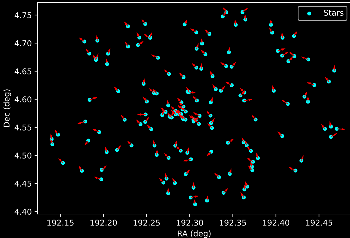
Gaia Cluster: [Dias_2] Proper Motion Vectors for Gaia Star Field (n= 147)
