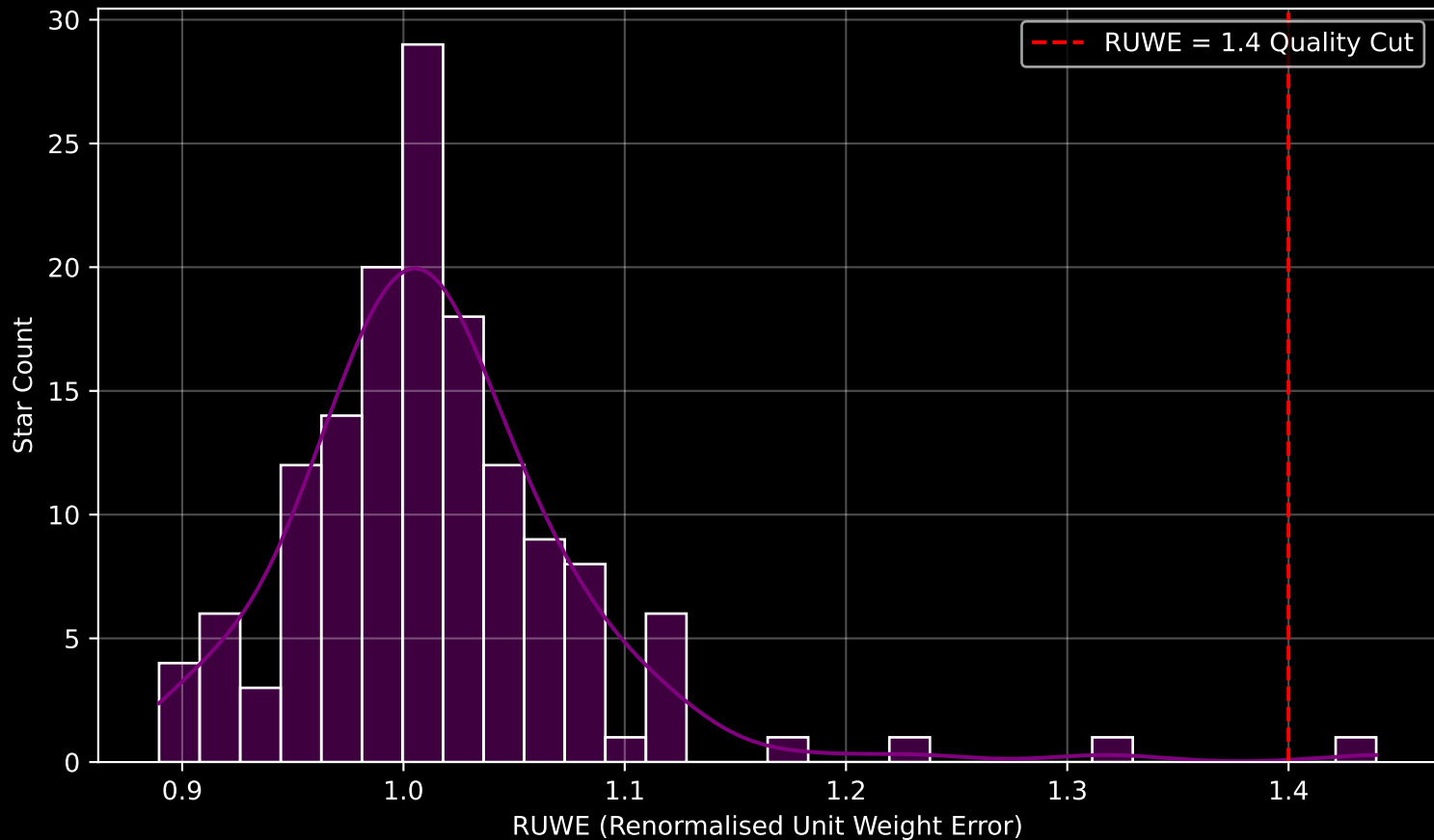
Gaia Cluster: [Dias_2] RUWE Distribution (n= 146)
