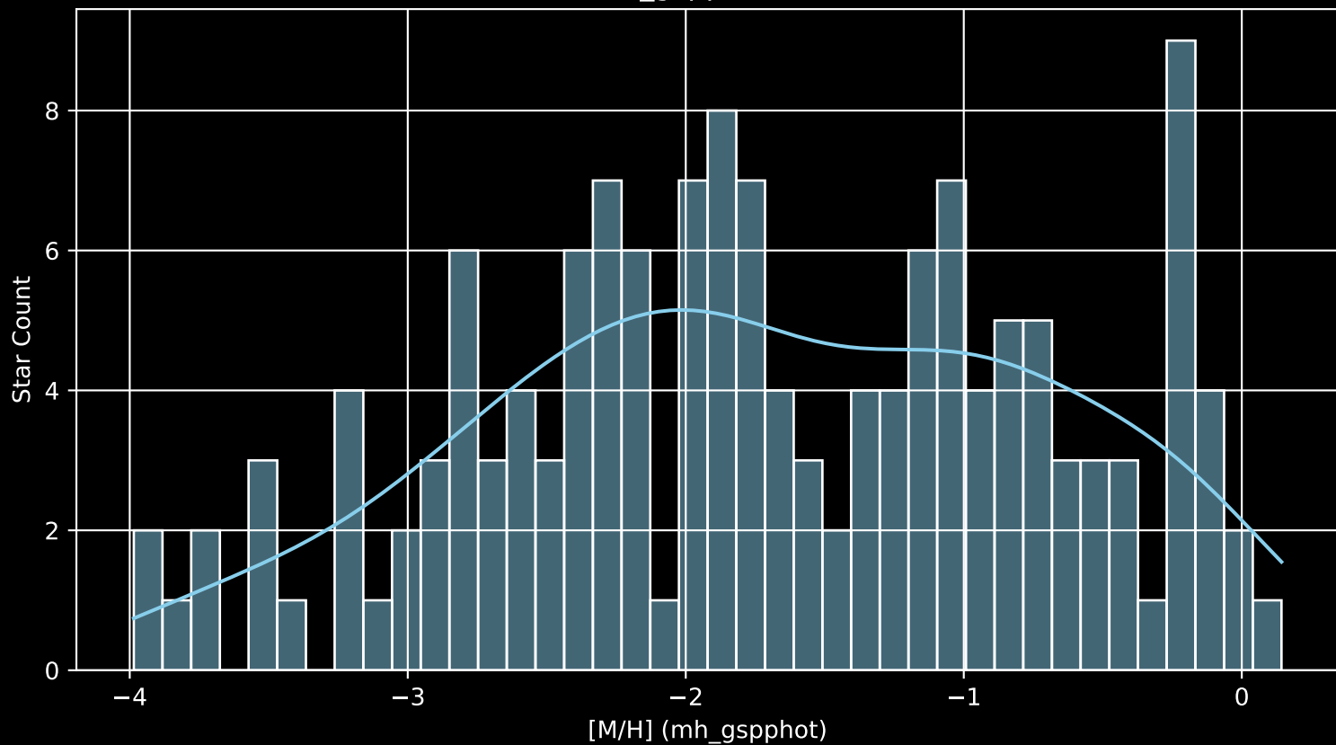
Gaia Cluster: [Dias_2 [M/H] (mh_gspphot) (n= 147)
