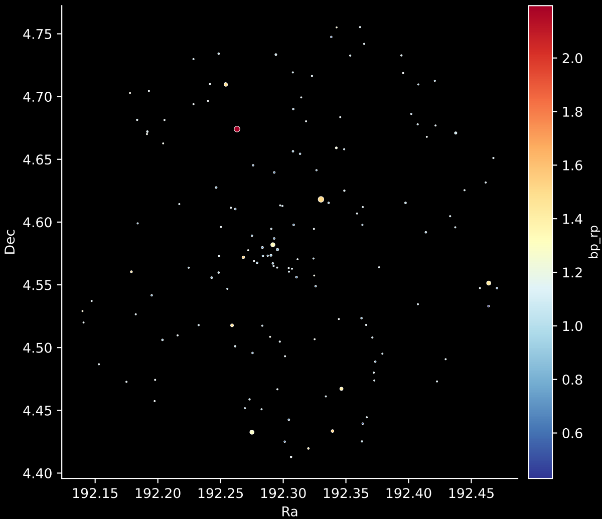
Gaia Cluster: [Dias_2] Stars: 147
