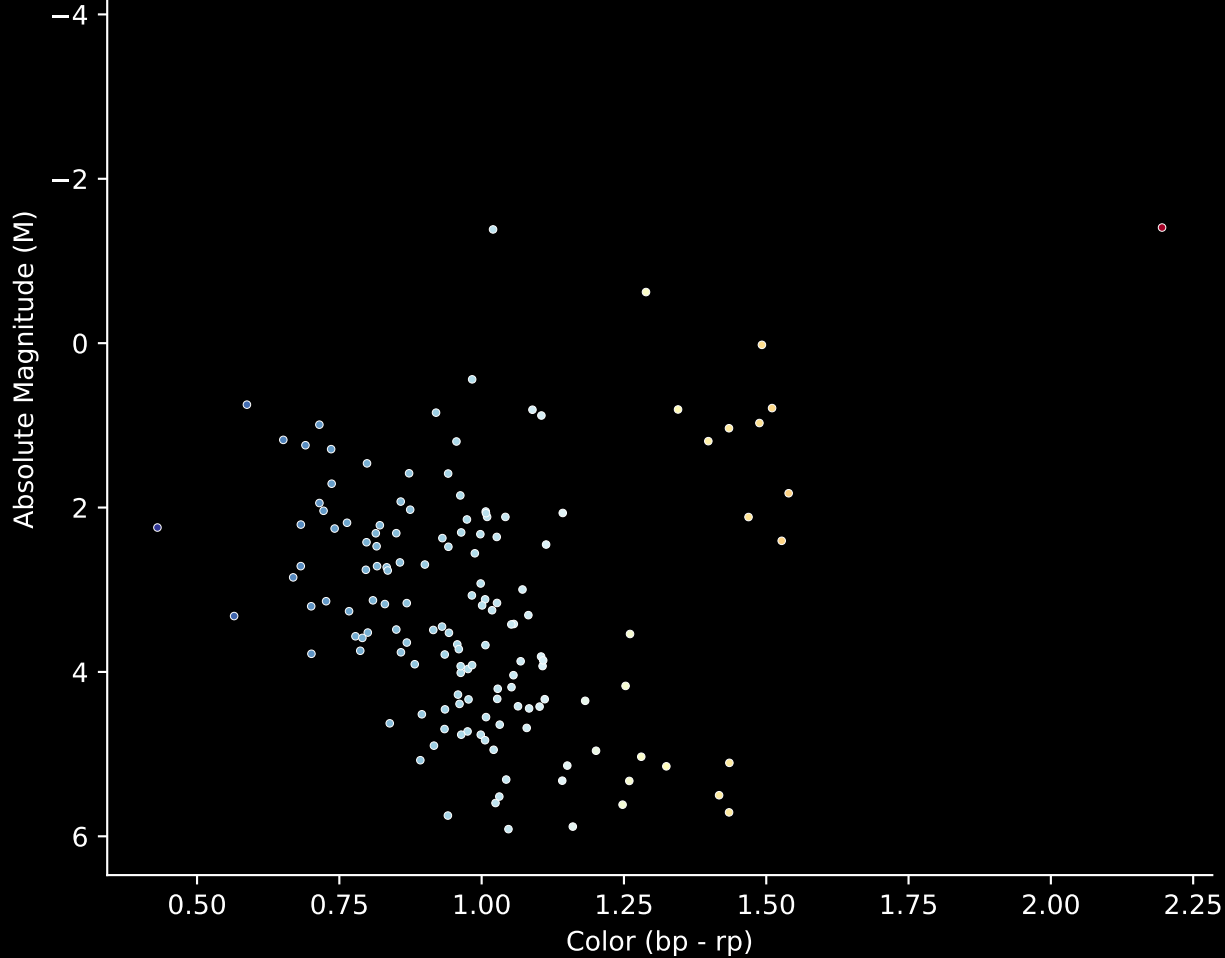
Gaia Cluster: [Dias_2] Stars (n= 147) Hertzsprung-Russel Diagram
