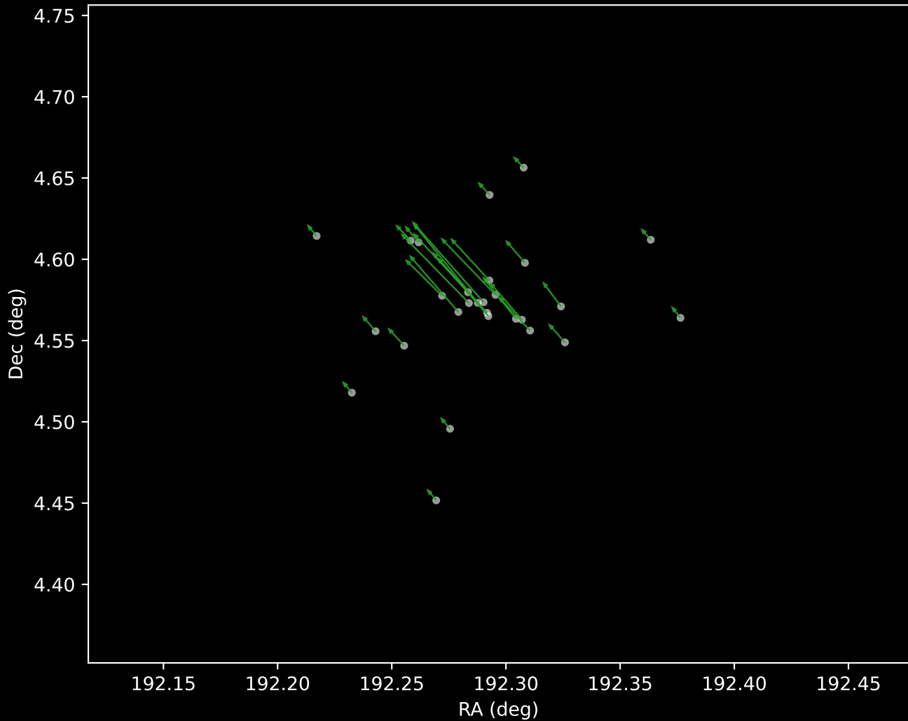
Gaia DR3 Cluster 4 Proper Motion Vectors (n=28)
