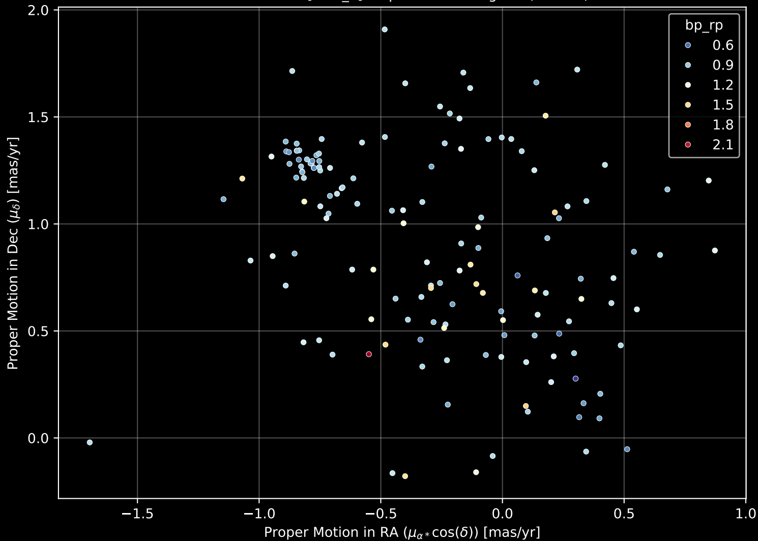
Gaia Cluster: [Dias_2] Proper Motion Diagram (n= 147)
