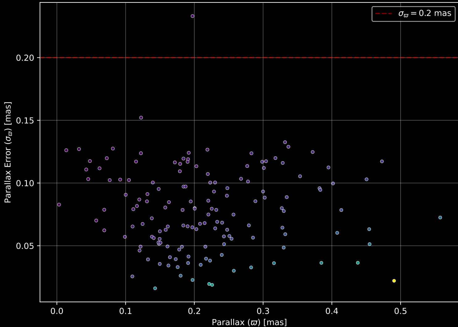
Gaia Cluster: [Dias_2] Parallax Quality (n= 147)
