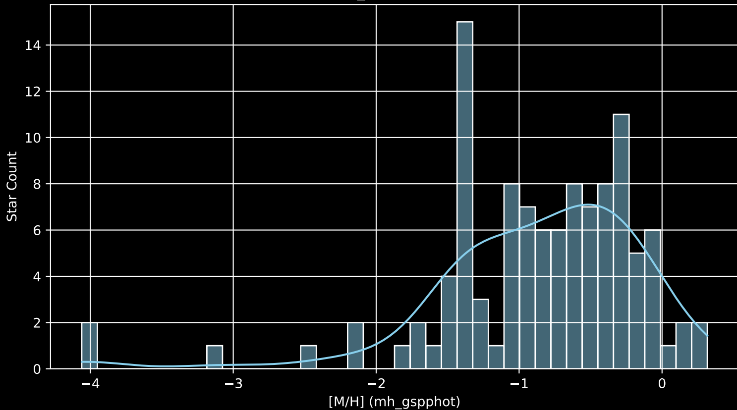
Gaia Cluster: [Dias_5 [M/H] (mh_gspphot) (n= 110)
