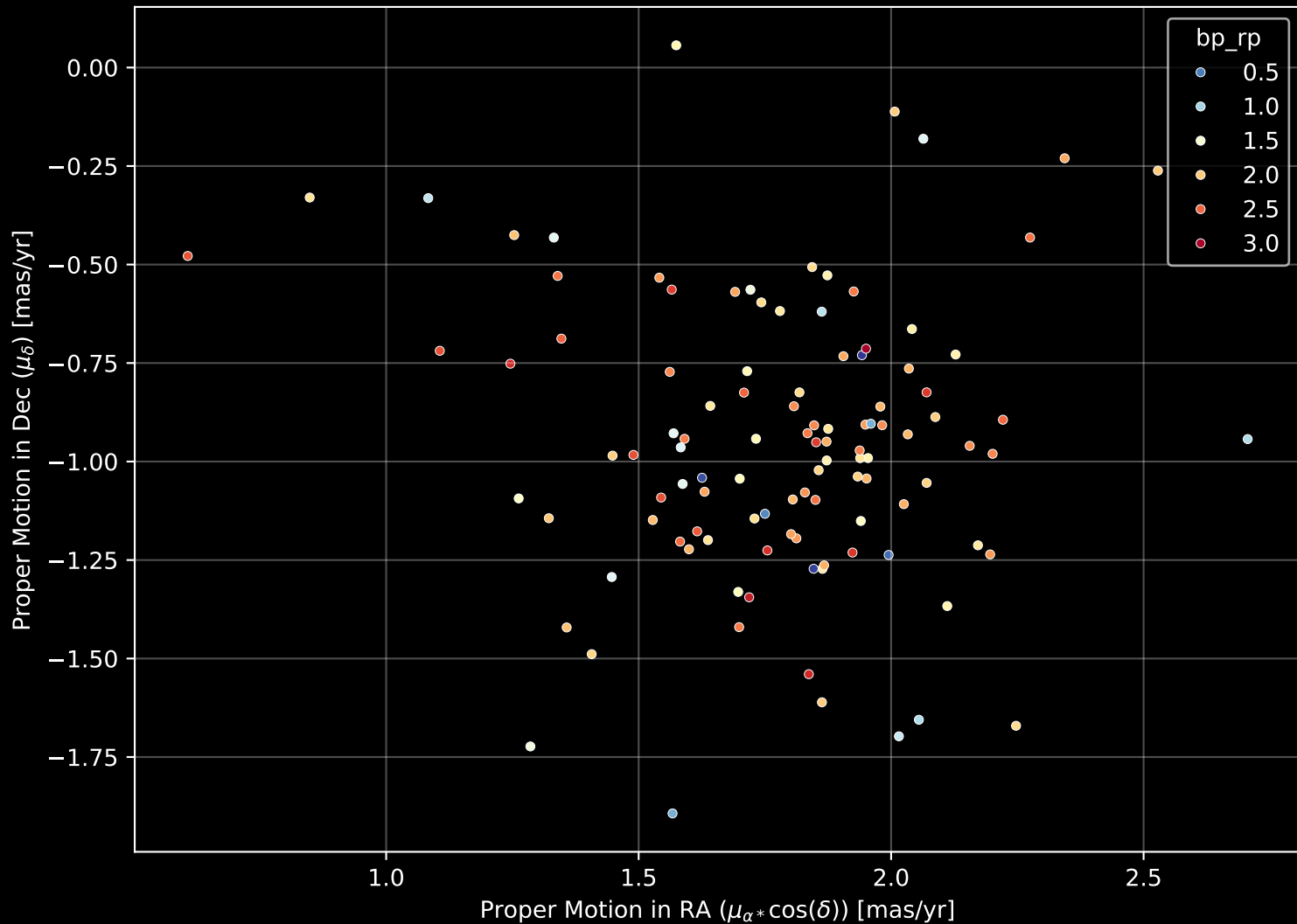
Gaia Cluster: [Dias_5] Proper Motion Diagram (n= 110)
