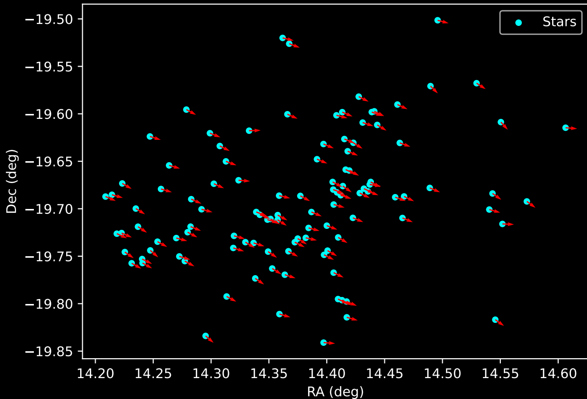
Gaia Cluster: [Dias_5] Proper Motion Vectors for Gaia Star Field (n= 110)
