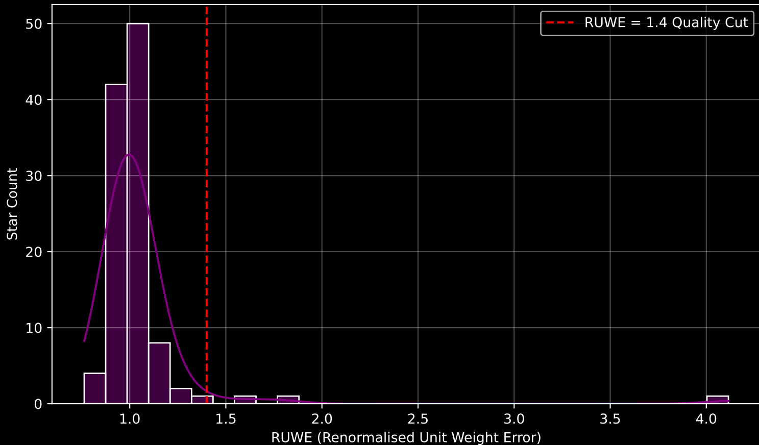
Gaia Cluster: [Dias_5] RUWE Distribution (n= 110)
