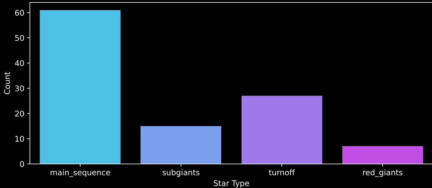
Gaia Cluster: [Dias_5] Count plot of Star Type
