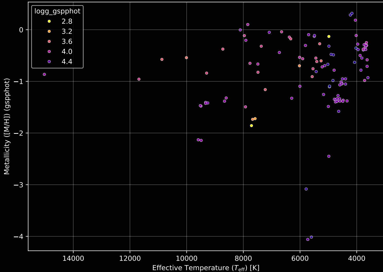
Gaia Cluster: [Dias_5] Stellar Population Parameters (n= 110)
