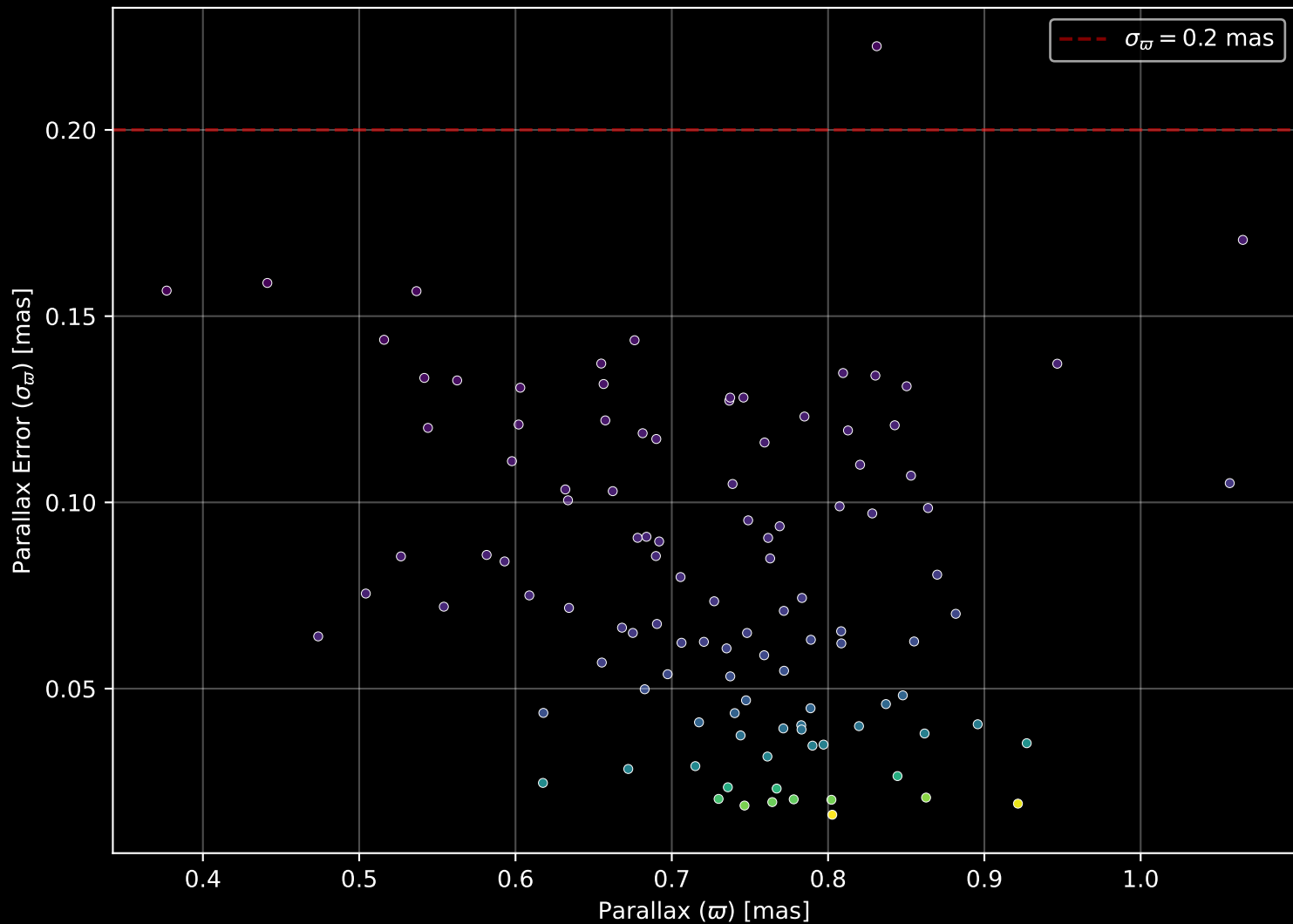
Gaia Cluster: [Dias_5] Parallax Quality (n= 110)
