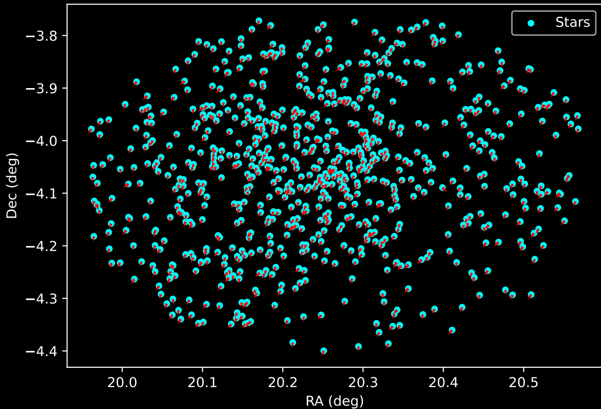
Gaia Cluster: [Dolidze_32] Proper Motion Vectors for Gaia Star Field (n= 754)
