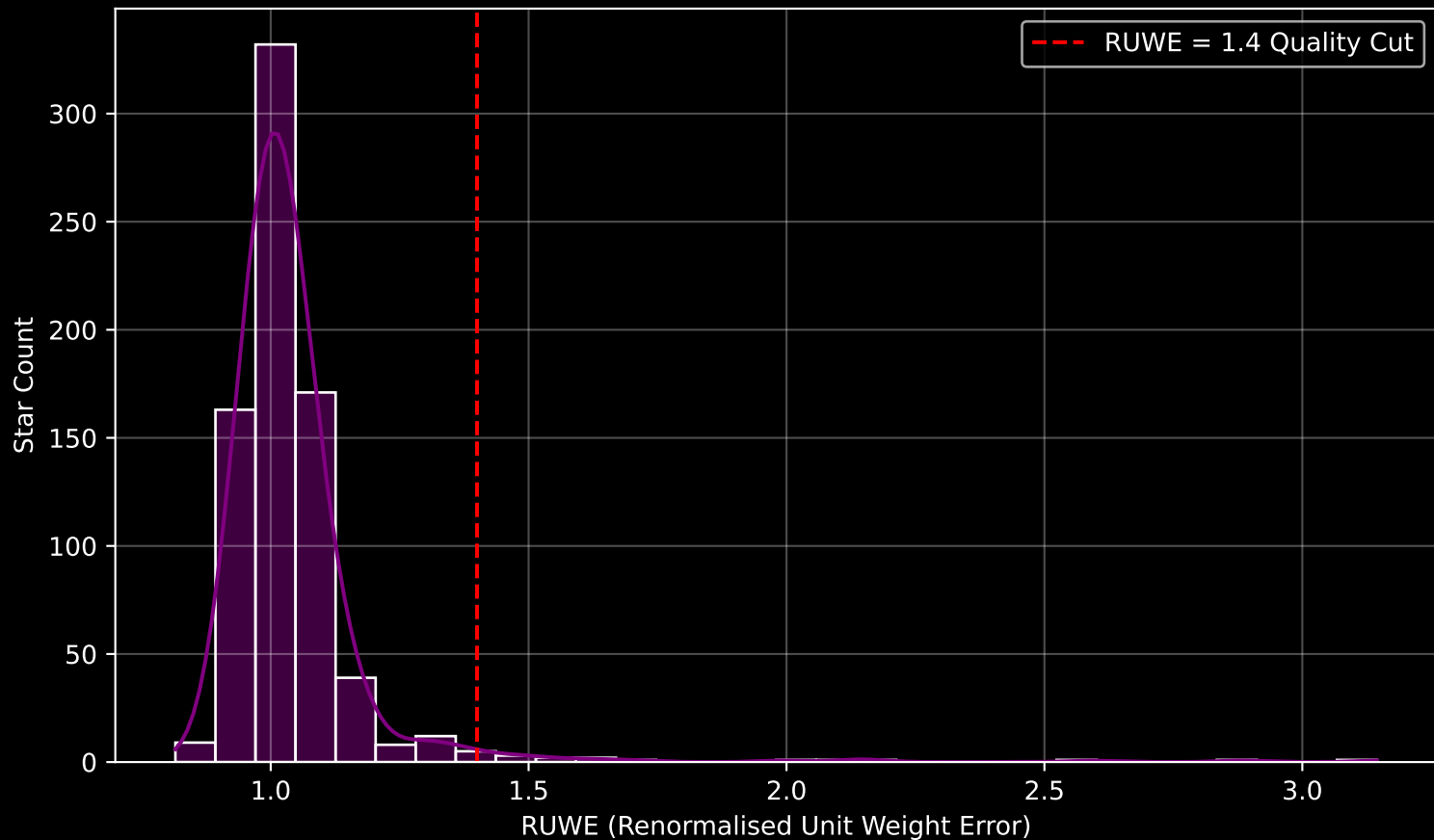
Gaia Cluster: [Dolidze_32] RUWE Distribution (n= 753)
