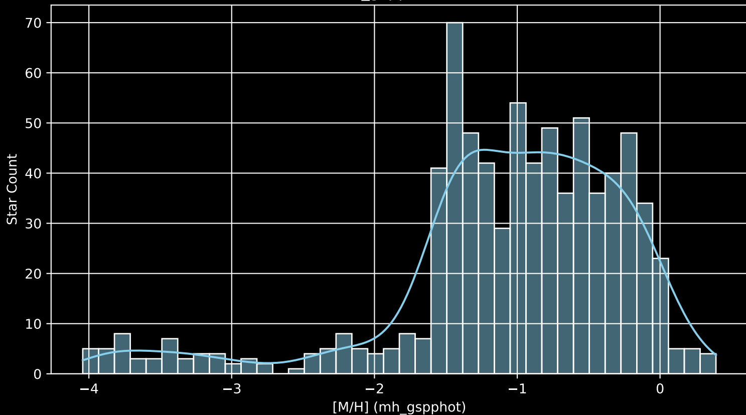
Gaia Cluster: [Dolidze_32 [M/H] (mh_gspphot) (n= 753)
