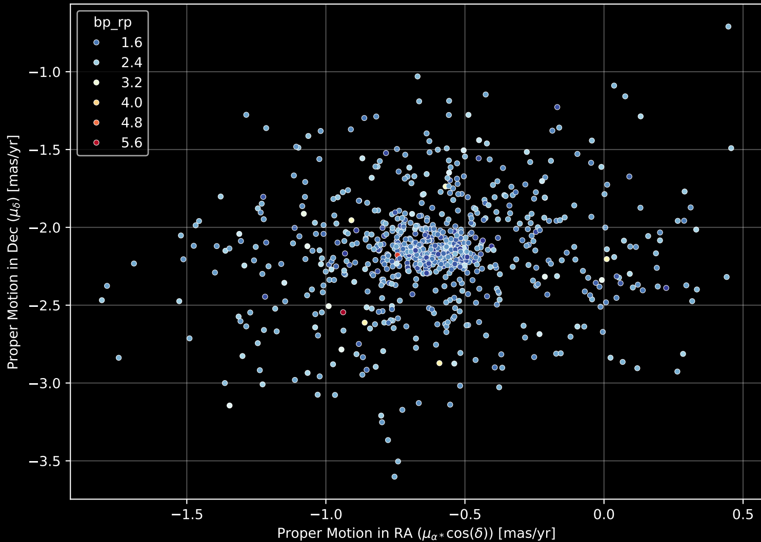
Gaia Cluster: [Dolidze_32] Proper Motion Diagram (n= 754)
