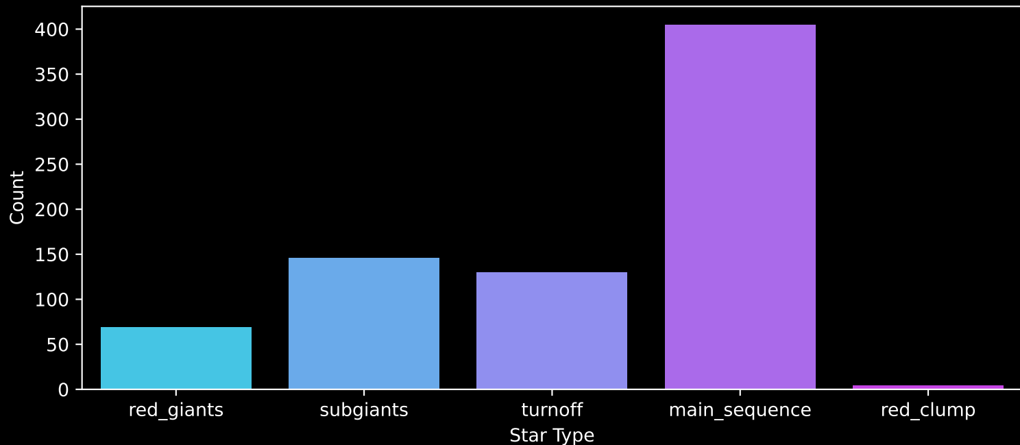
Gaia Cluster: [Dolidze_32] Count plot of Star Type
