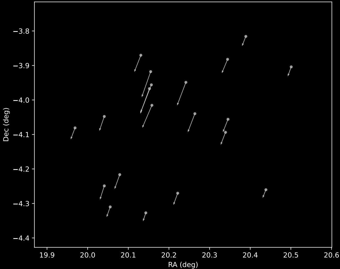
Gaia DR3 Cluster 15 Proper Motion Vectors (n=20)
