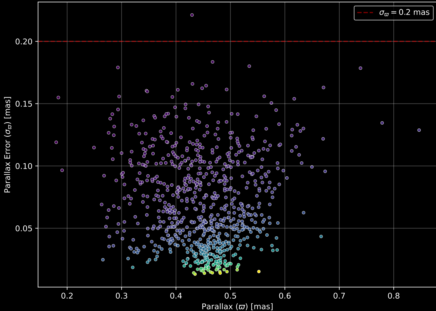
Gaia Cluster: [Dolidze_32] Parallax Quality (n= 754)
