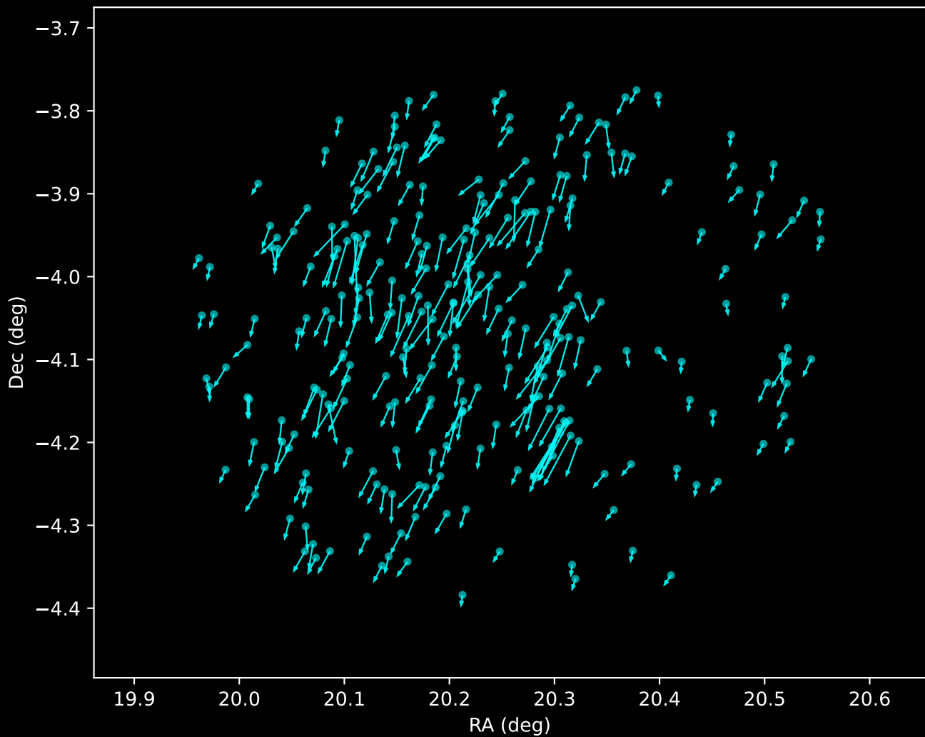
Gaia DR3 Noise Stream Proper Motion Vectors (n=269)
