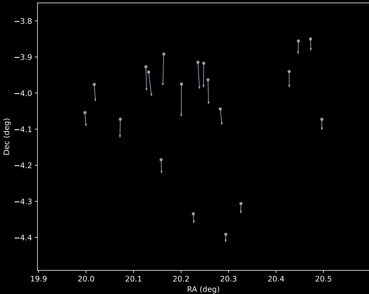
Gaia DR3 Cluster 9 Proper Motion Vectors (n=19)
