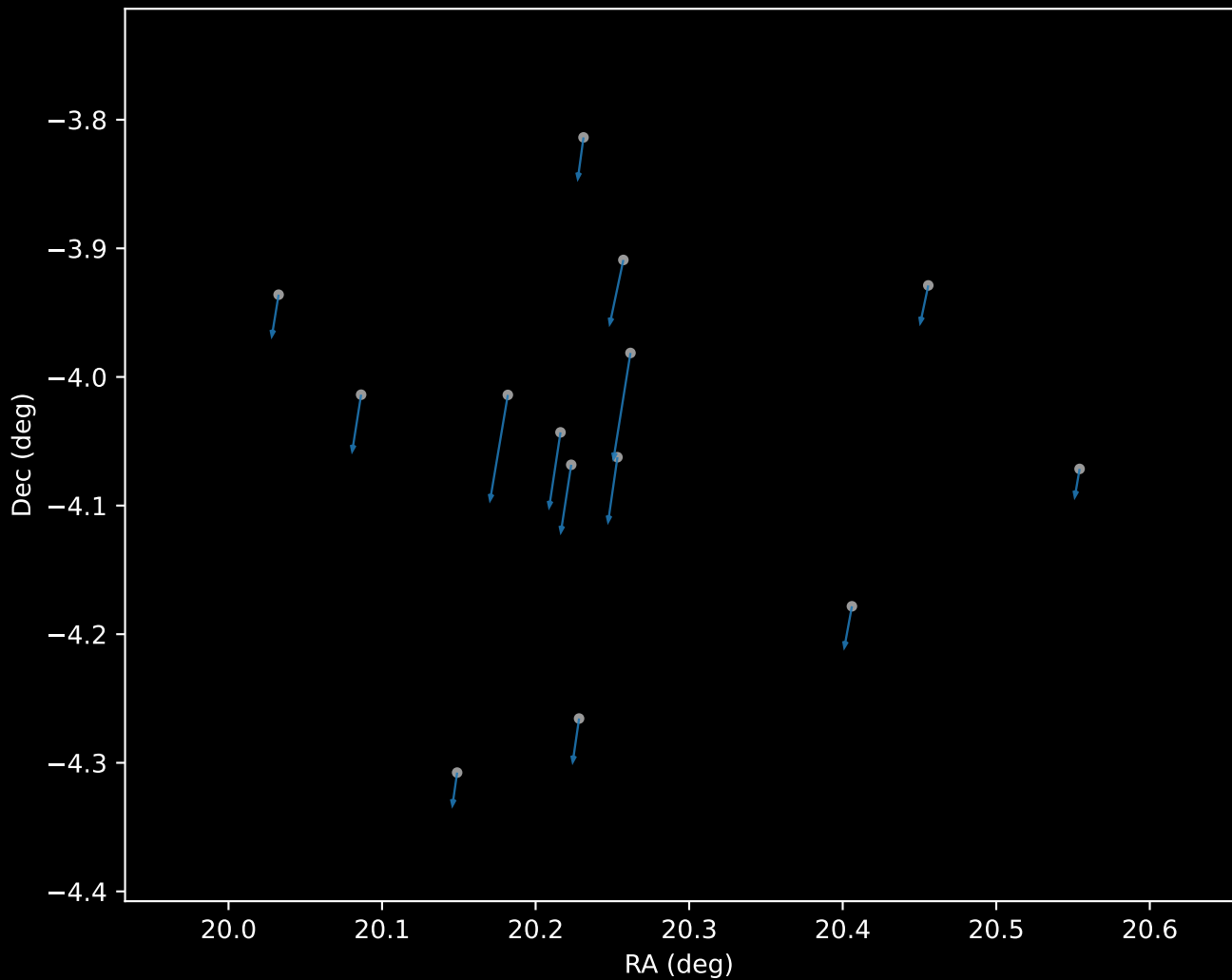
Gaia DR3 Cluster 20 Proper Motion Vectors (n=14)
