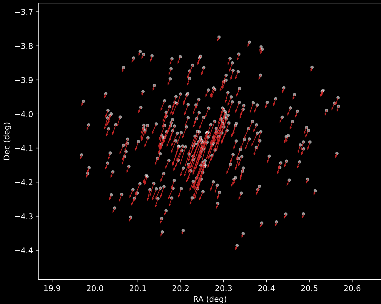
Gaia DR3 Cluster 26 Proper Motion Vectors (n=269)
