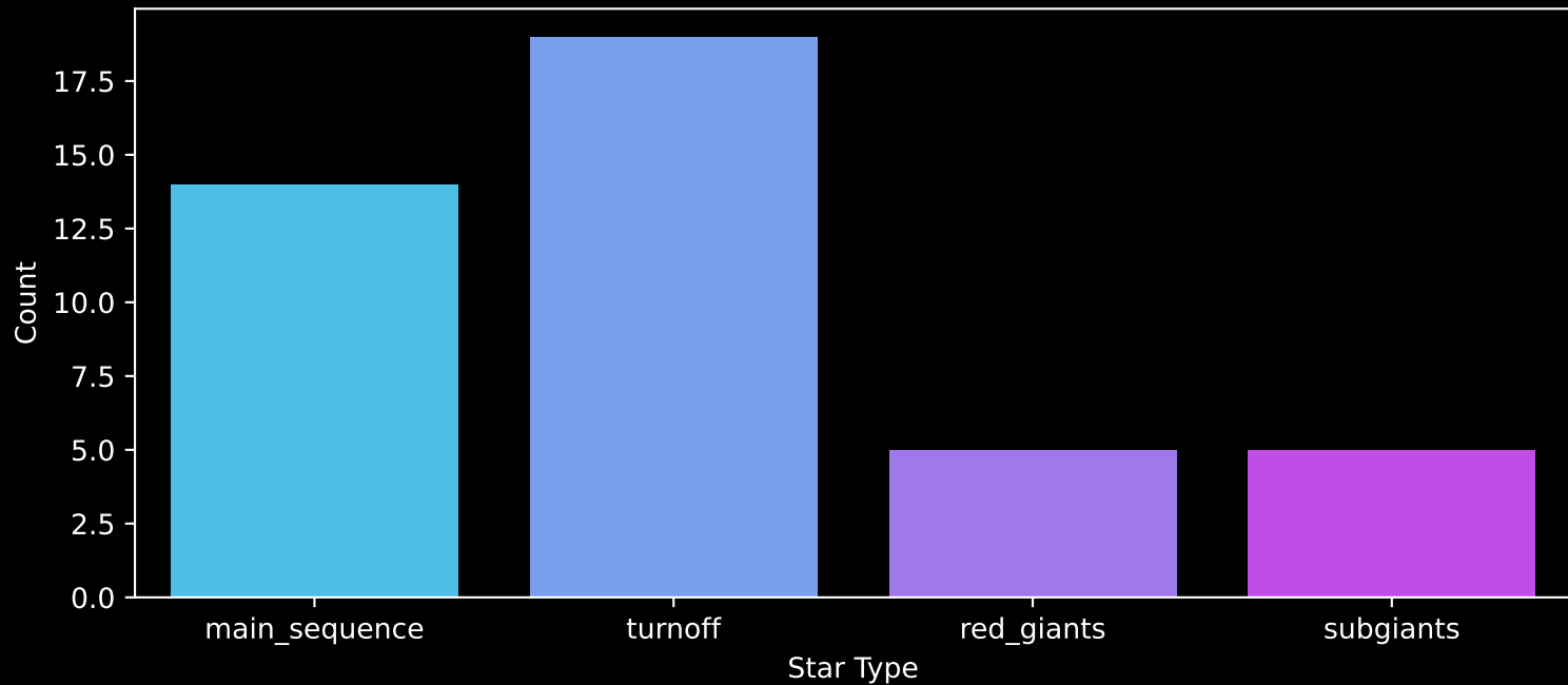
Gaia Cluster: [Dolidze_8] Count plot of Star Type
