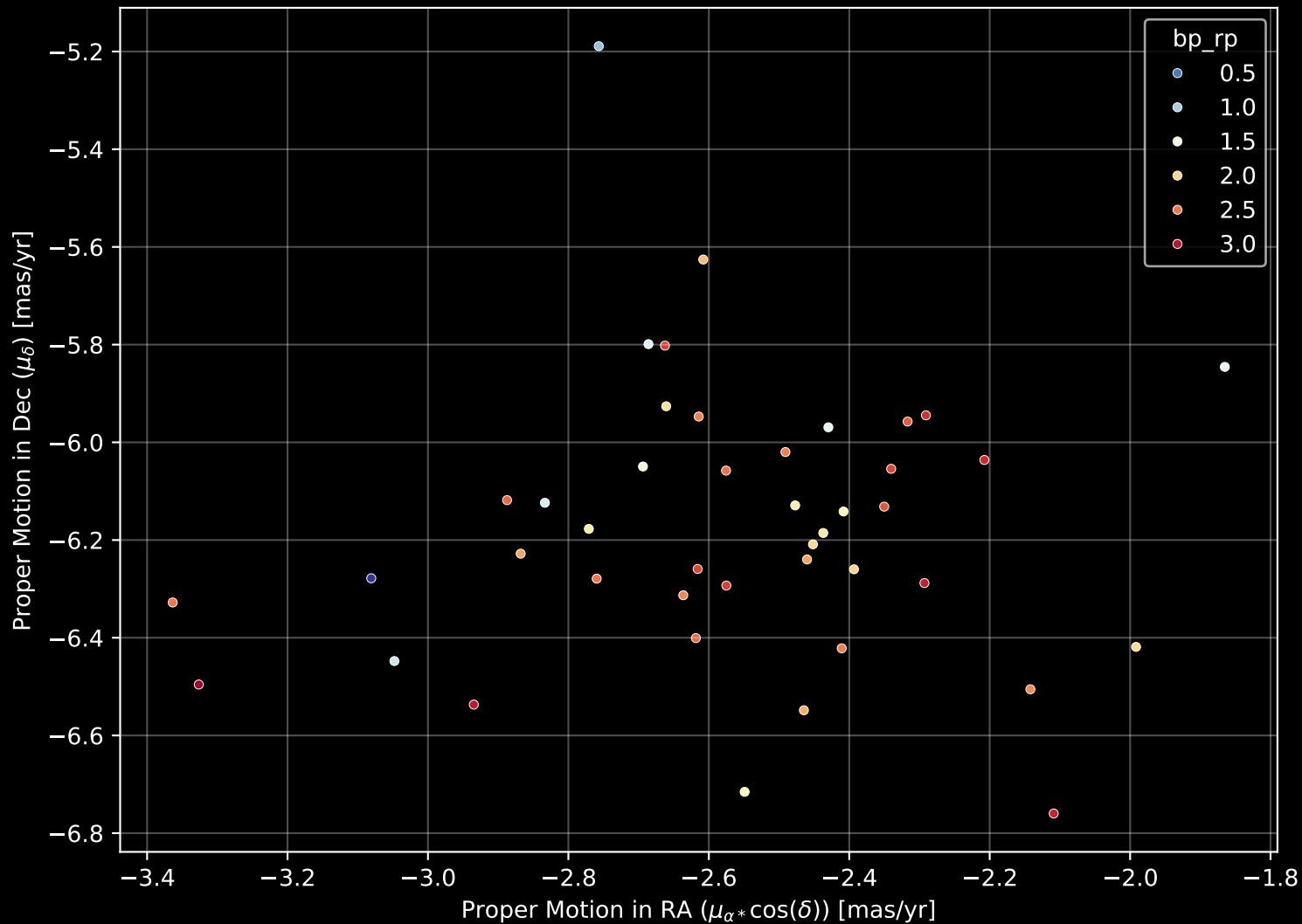
Gaia Cluster: [Dolidze_8] Proper Motion Diagram (n= 43)
