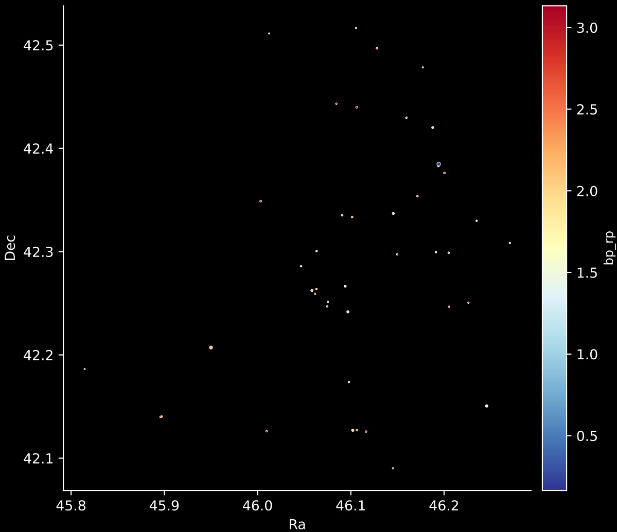
Gaia Cluster: [Dolidze_8] Stars: 43
