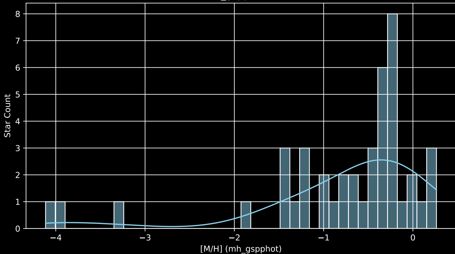
Gaia Cluster: [Dolidze_8 [M/H] (mh_gspphot) (n= 43)
