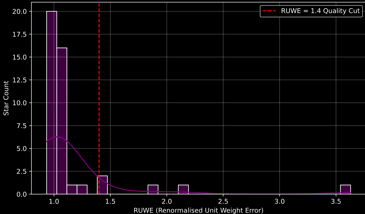
Gaia Cluster: [Dolidze_8] RUWE Distribution (n= 43)
