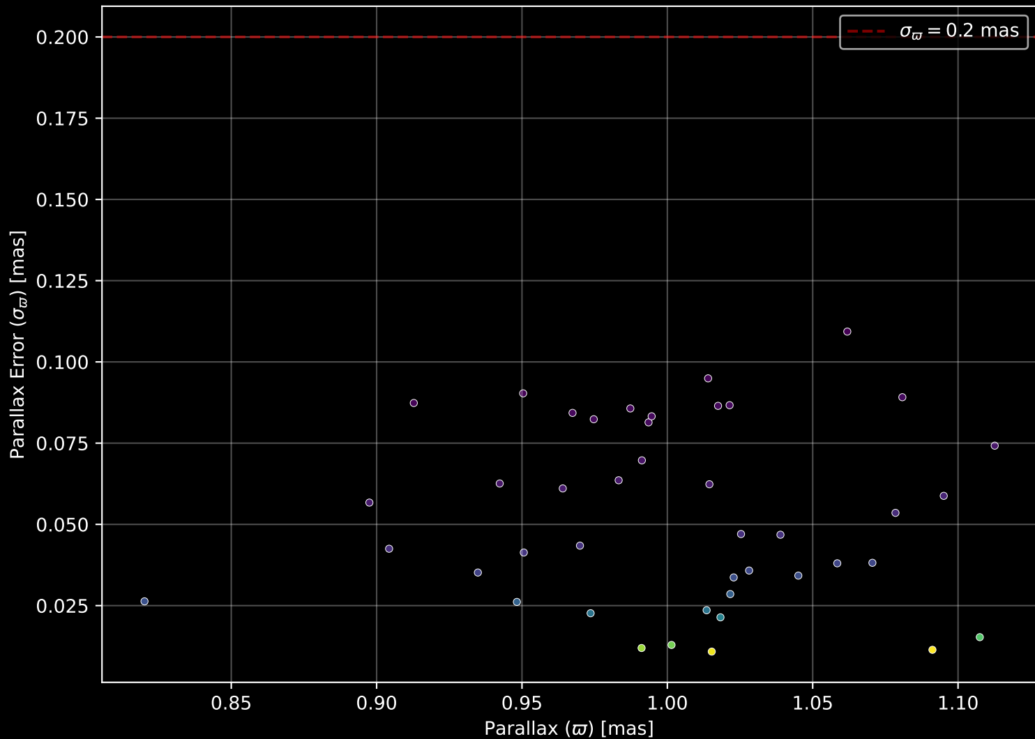
Gaia Cluster: [Dolidze_8] Parallax Quality (n= 43)
