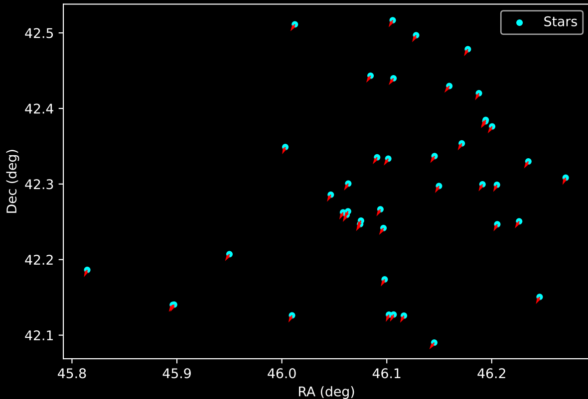
Gaia Cluster: [Dolidze_8] Proper Motion Vectors for Gaia Star Field (n= 43)
