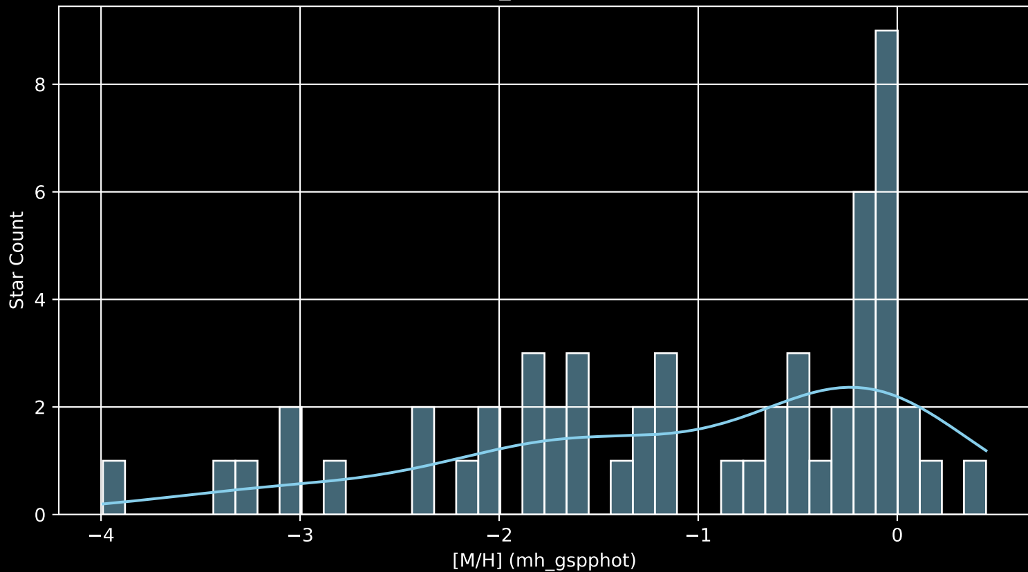
Gaia Cluster: [ESO_092_18 [M/H] (mh_gspphot) (n= 54)
