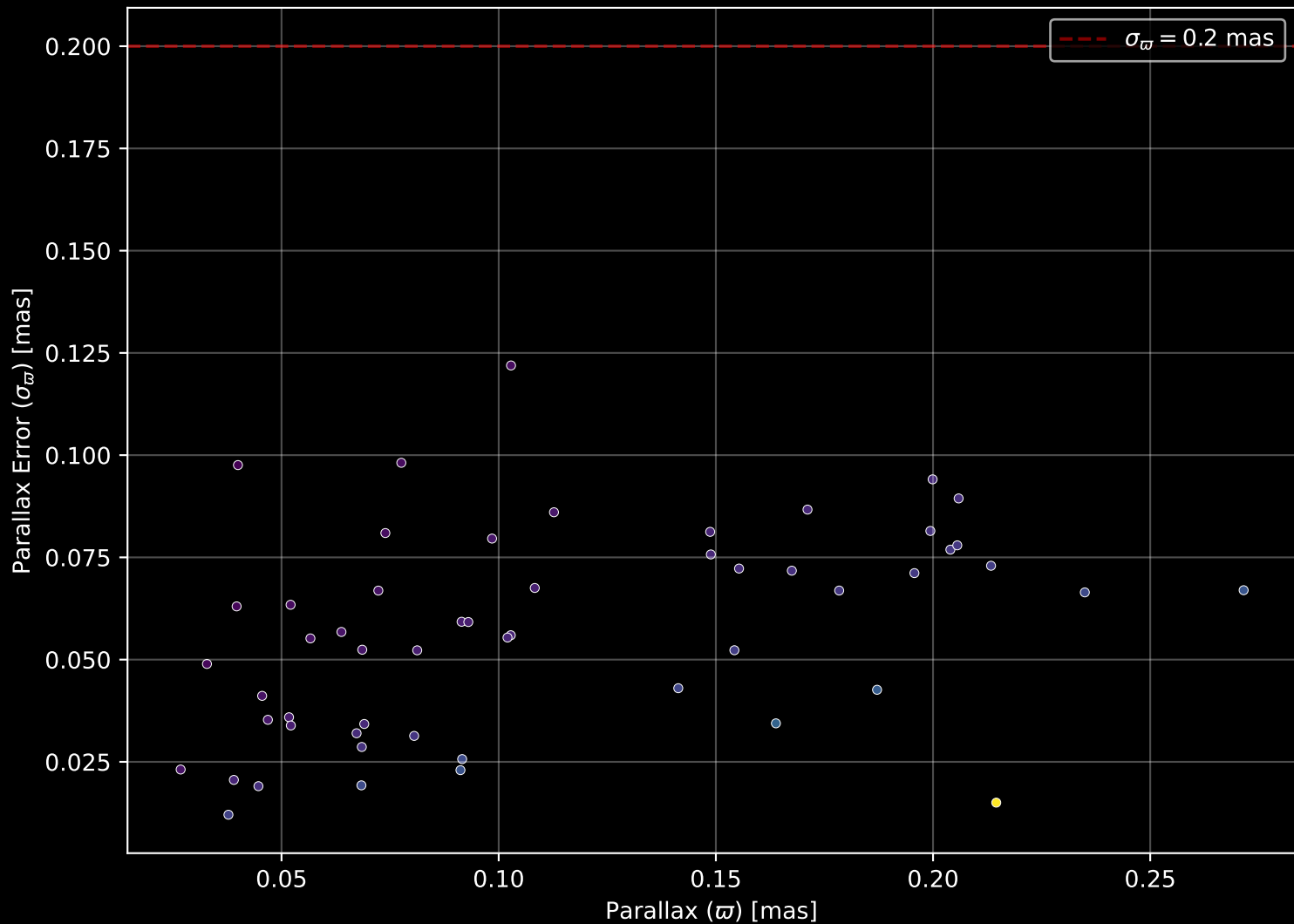
Gaia Cluster: [ESO_092_18] Parallax Quality (n= 54)
