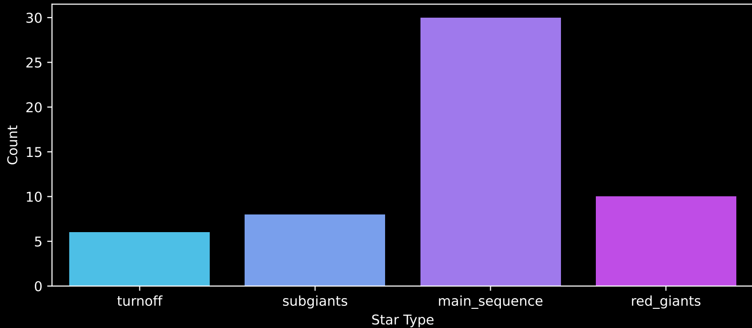
Gaia Cluster: [ESO_092_18] Count plot of Star Type
