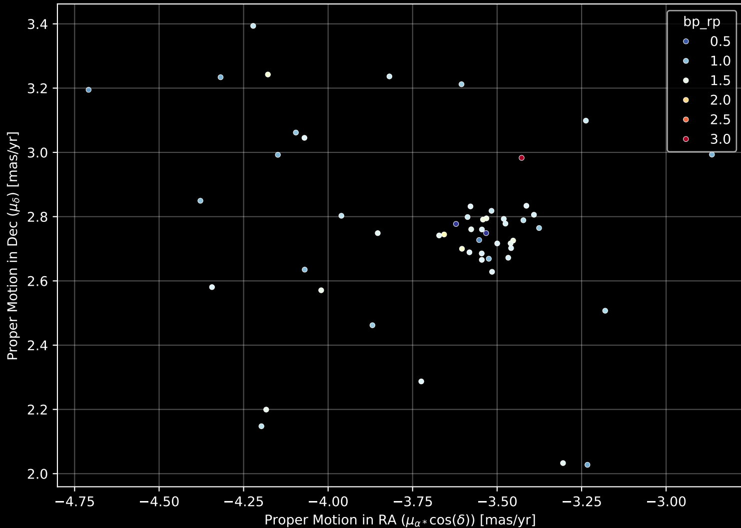
Gaia Cluster: [ESO_092_18] Proper Motion Diagram (n= 54)
