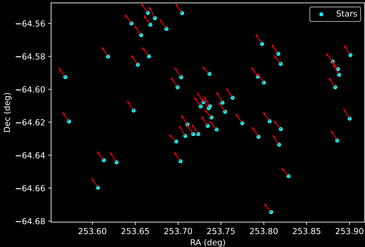
Gaia Cluster: [ESO_092_18] Proper Motion Vectors for Gaia Star Field (n= 54)
