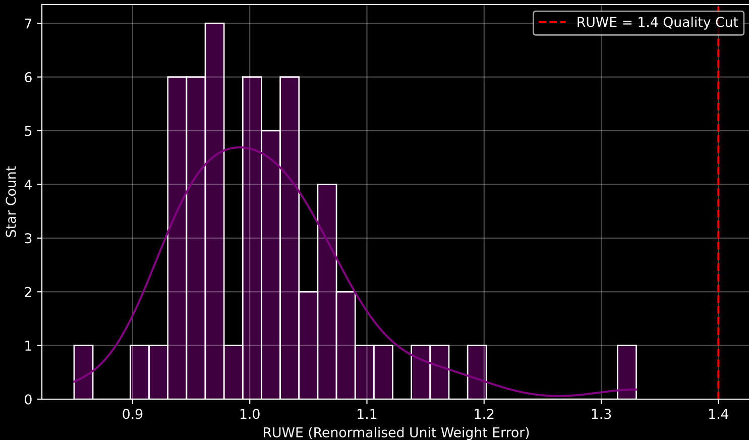
Gaia Cluster: [ESO_092_18] RUWE Distribution (n= 54)
