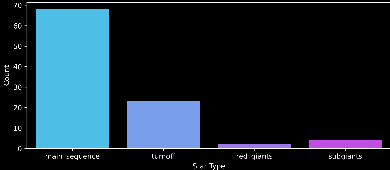
Gaia Cluster: [ESO_130_08] Count plot of Star Type
