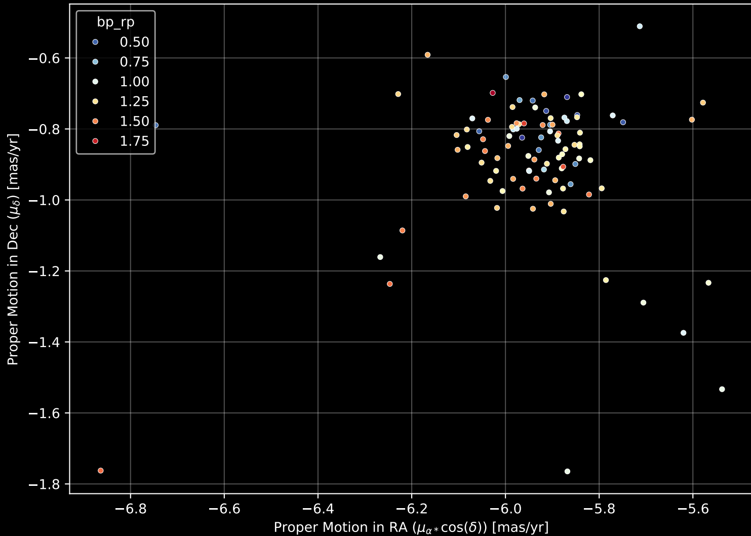
Gaia Cluster: [ESO_130_08] Proper Motion Diagram (n= 97)
