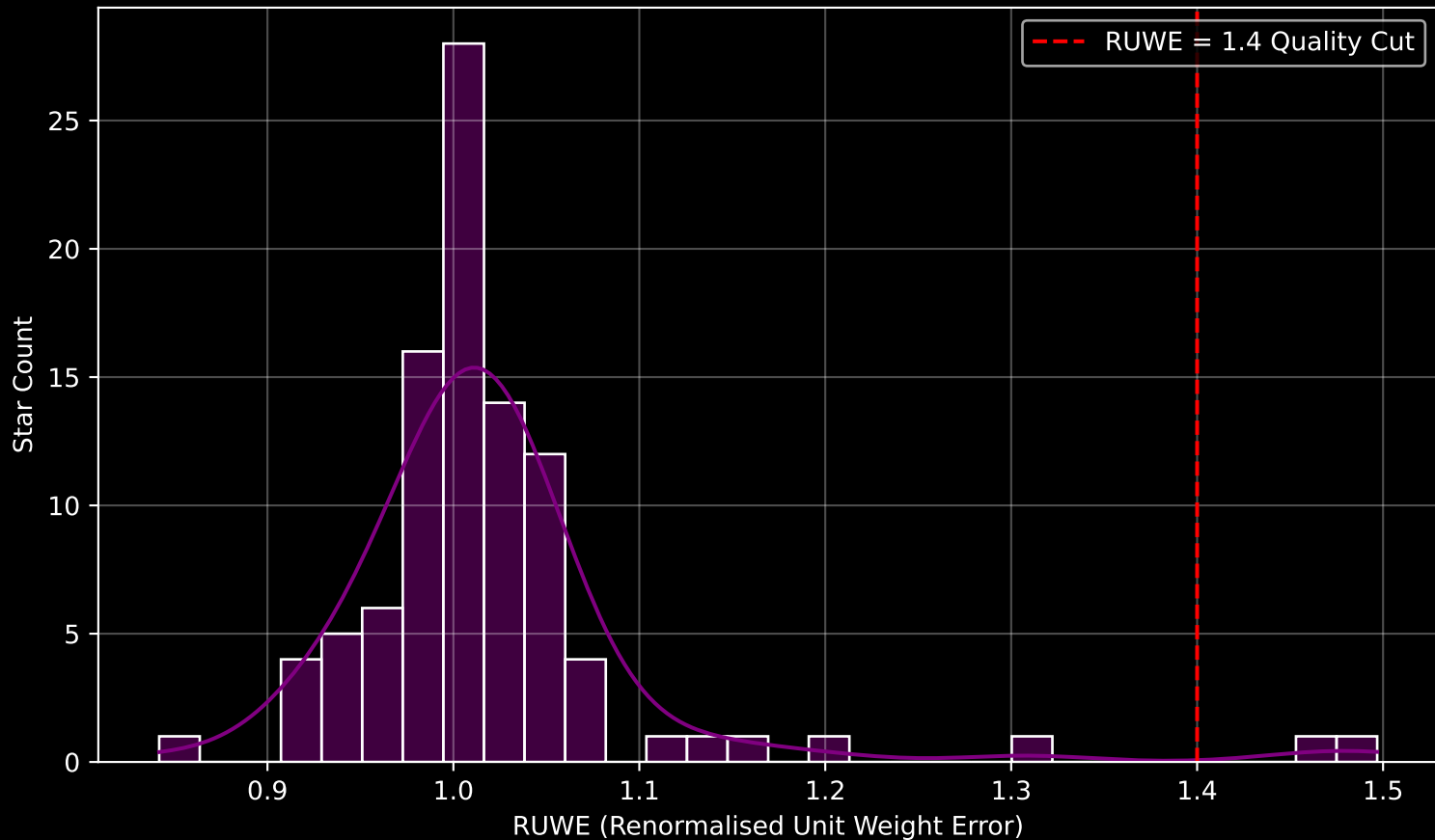
Gaia Cluster: [ESO_130_08] RUWE Distribution (n= 97)
