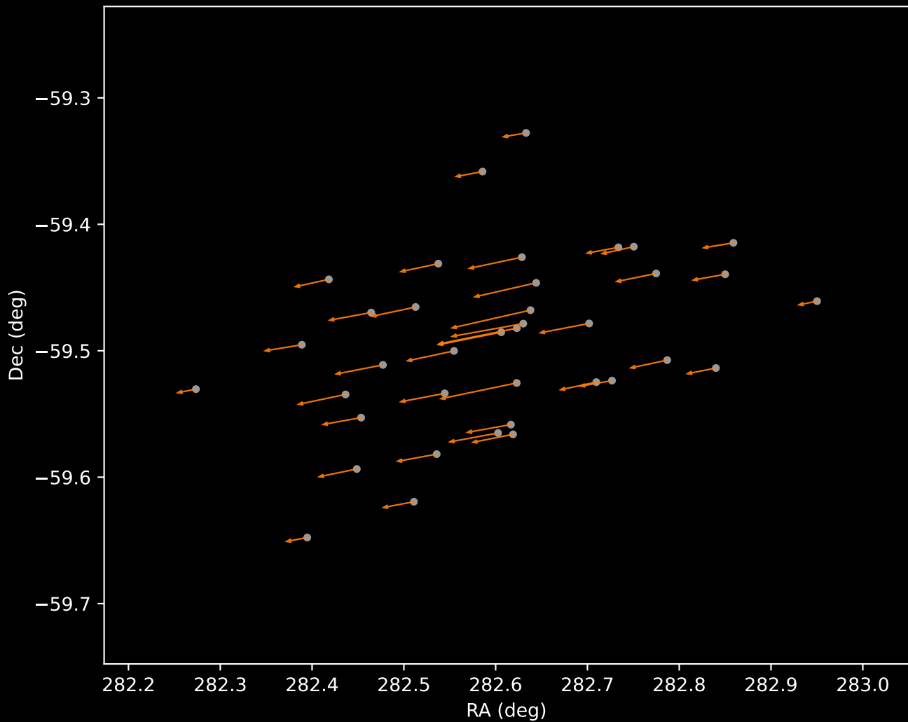
Gaia DR3 Cluster 2 Proper Motion Vectors (n=38)
