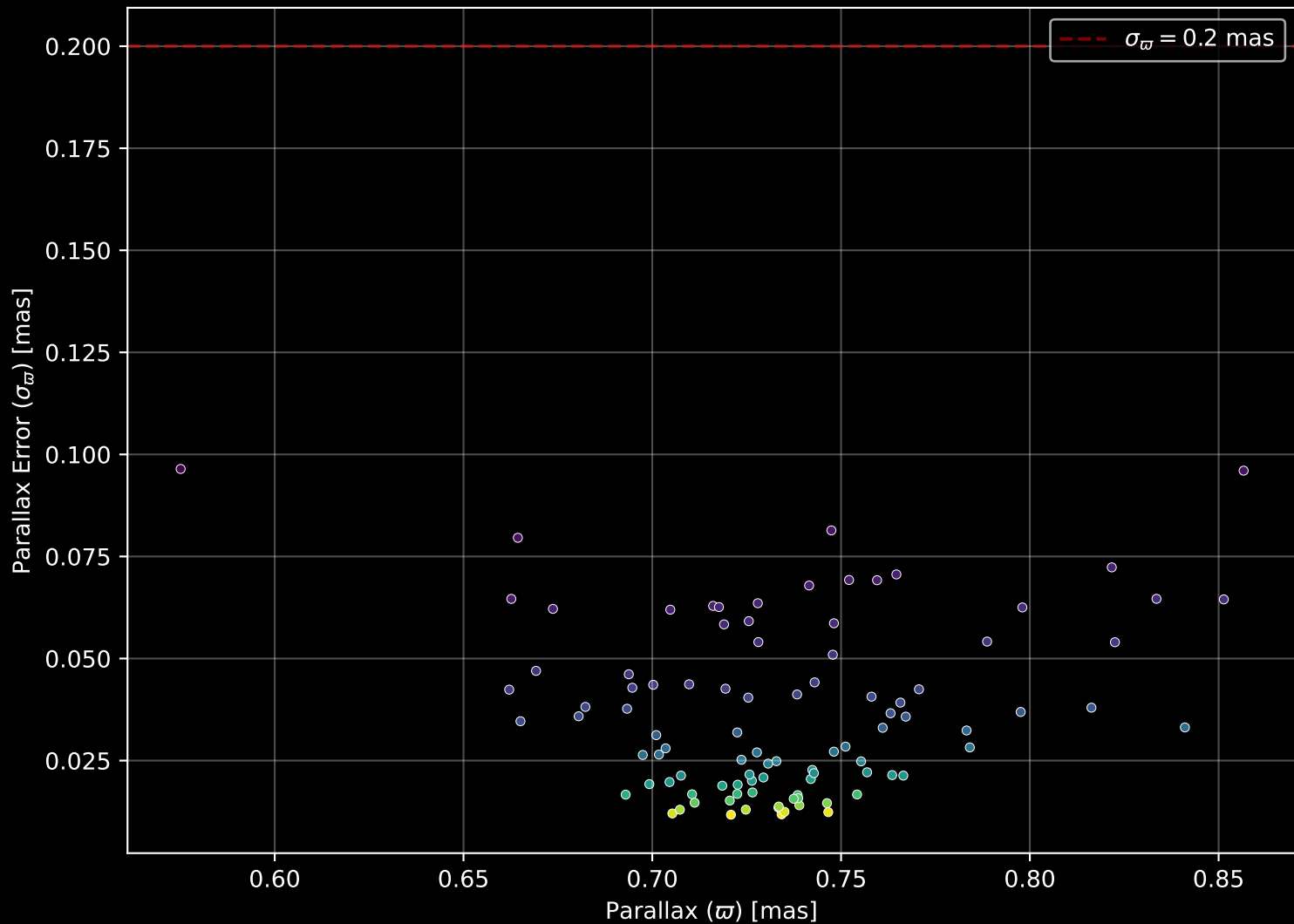
Gaia Cluster: [ESO_130_08] Parallax Quality (n= 97)
