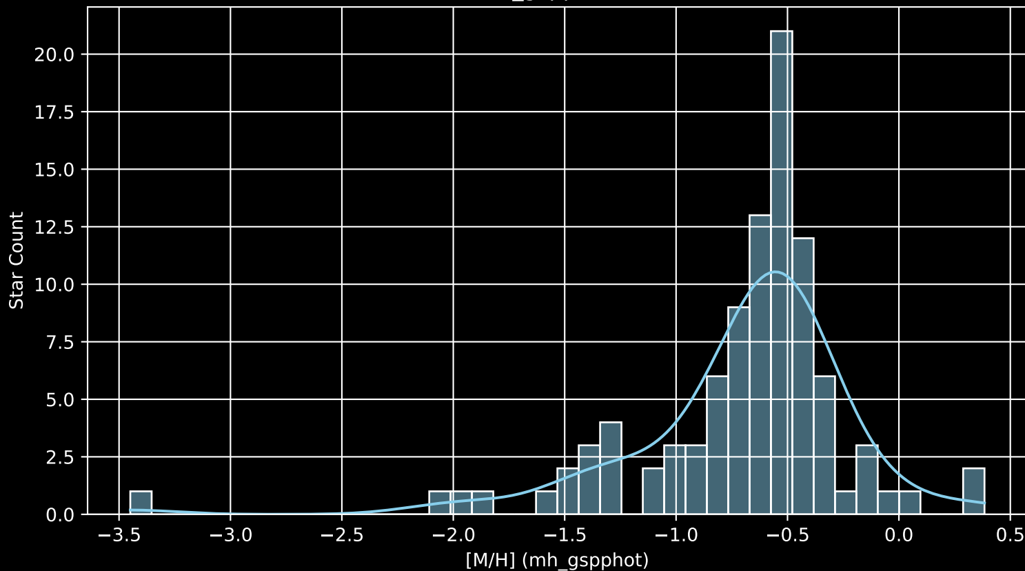
Gaia Cluster: [ESO_130_08 [M/H] (mh_gspphot) (n= 97)
