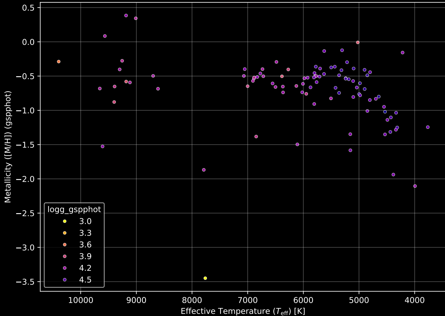
Gaia Cluster: [ESO_130_08] Stellar Population Parameters (n= 97)
