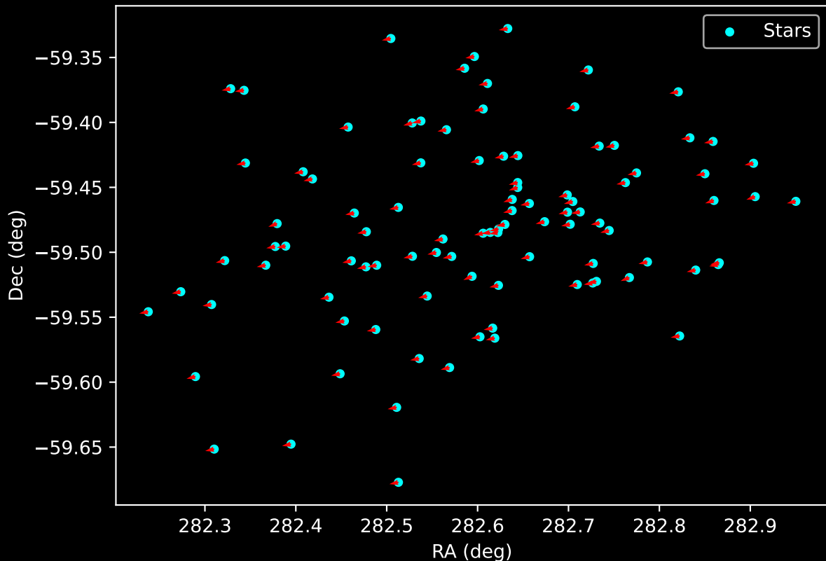
Gaia Cluster: [ESO_130_08] Proper Motion Vectors for Gaia Star Field (n= 97)
