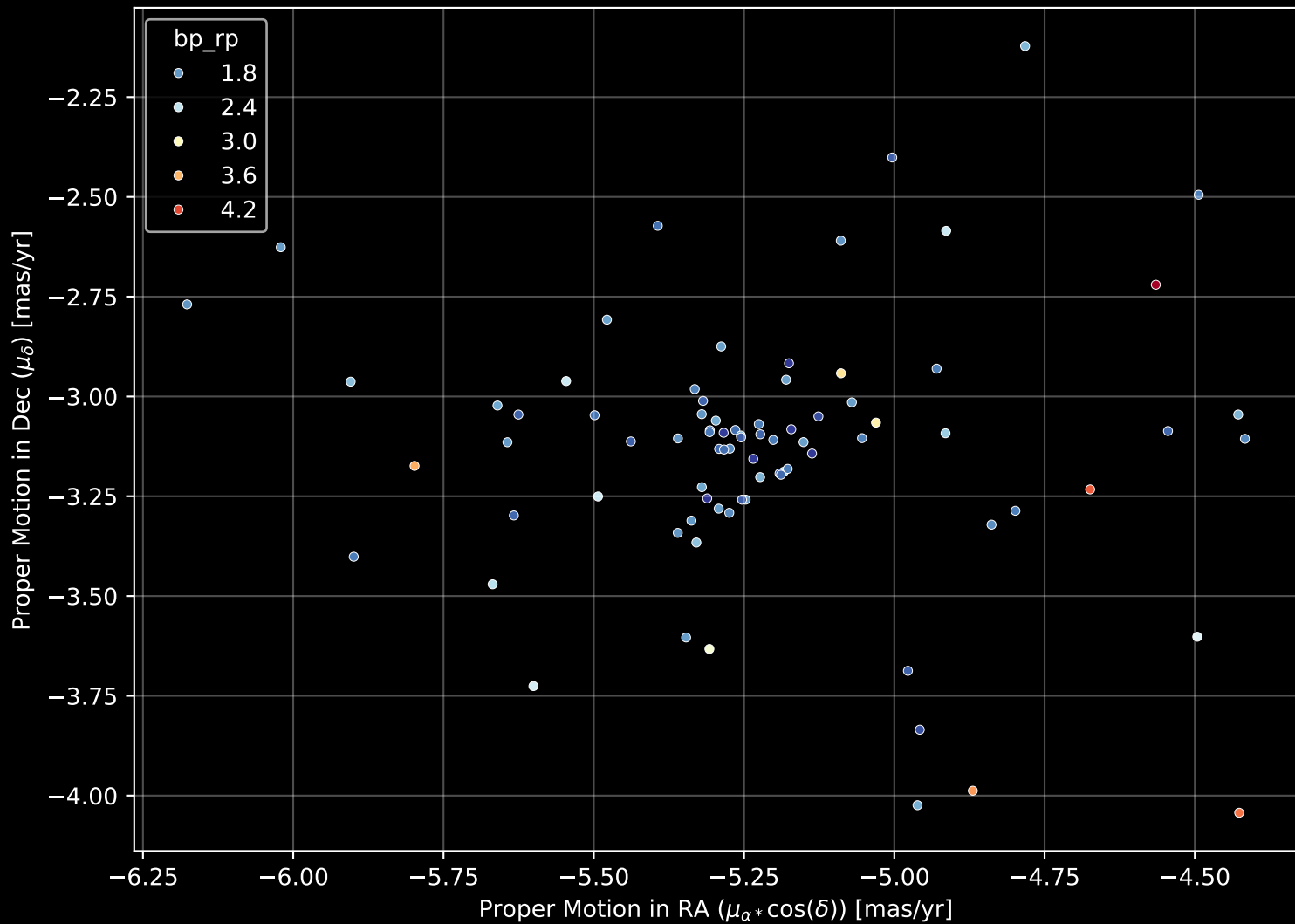
Gaia Cluster: [ESO_134_12] Proper Motion Diagram (n= 82)
