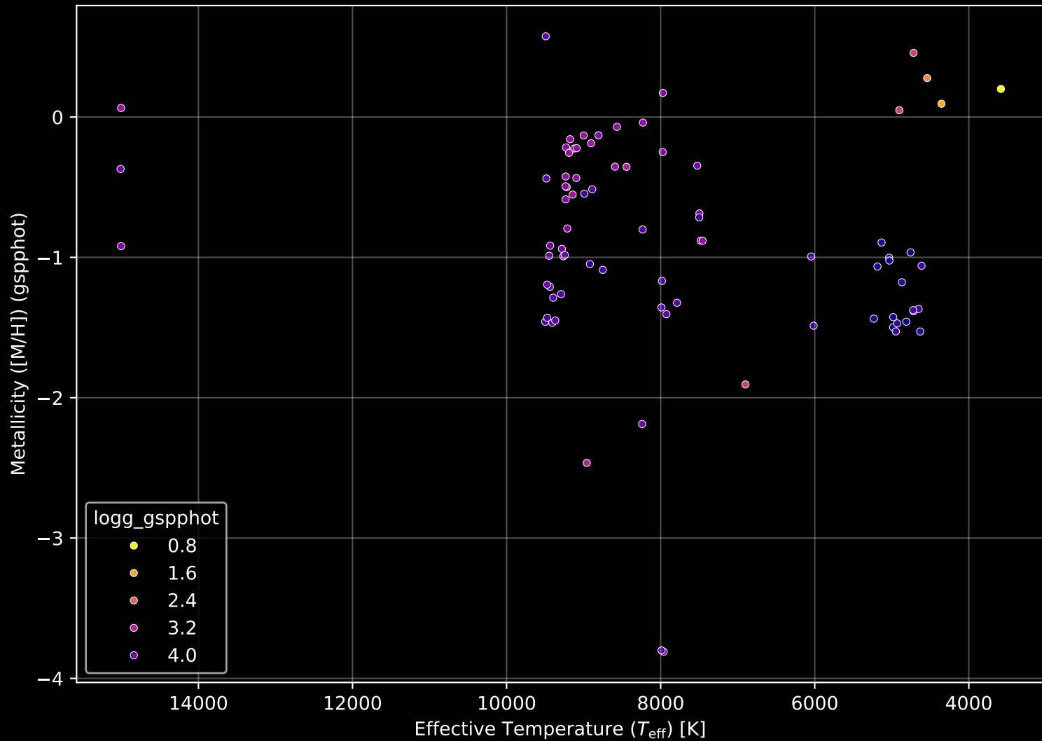
Gaia Cluster: [ESO_134_12] Stellar Population Parameters (n= 82)
