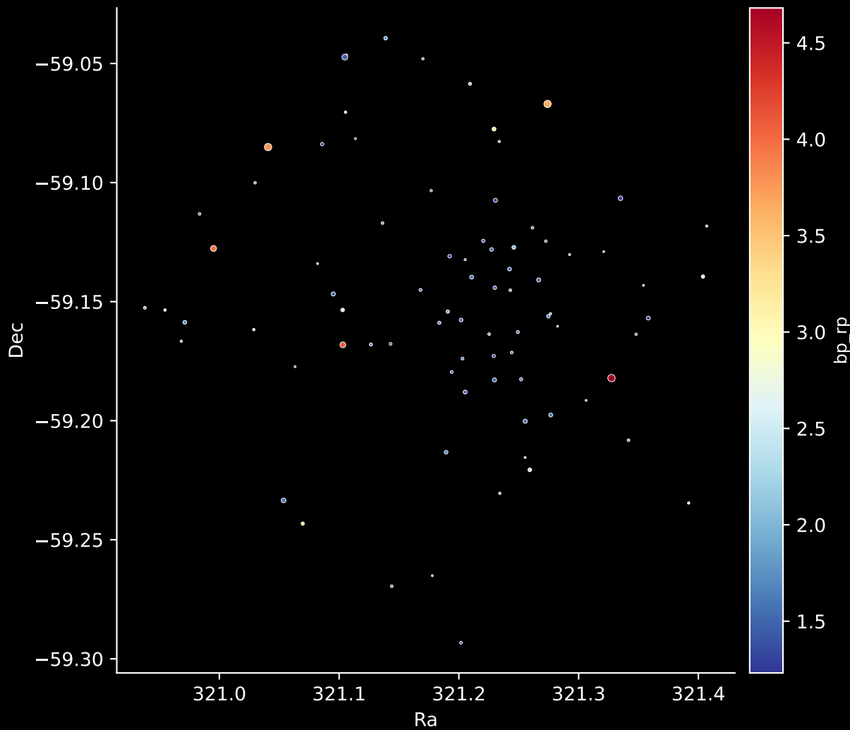
Gaia Cluster: [ESO_134_12] Stars: 82
