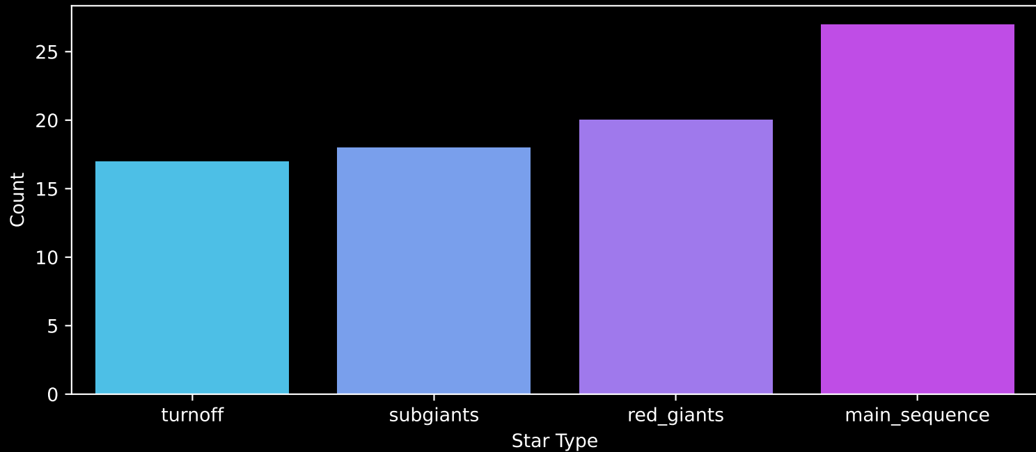
Gaia Cluster: [ESO_134_12] Count plot of Star Type
