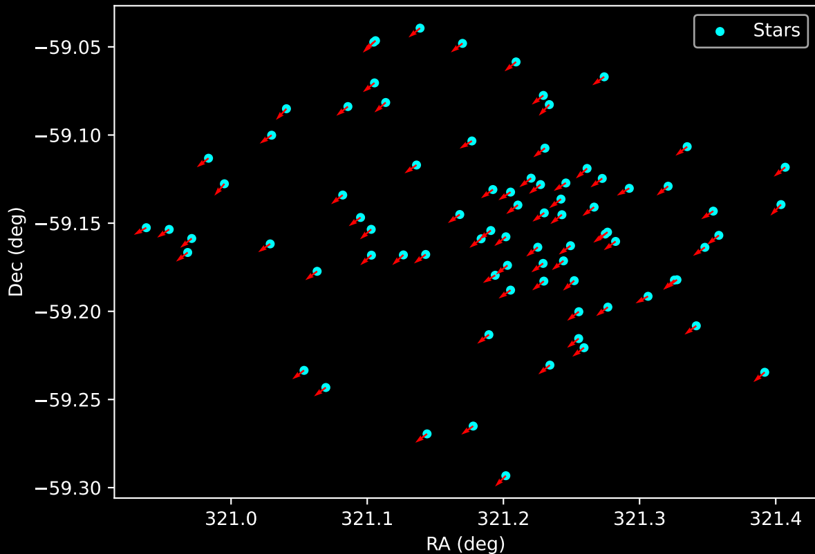
Gaia Cluster: [ESO_134_12] Proper Motion Vectors for Gaia Star Field (n= 82)
