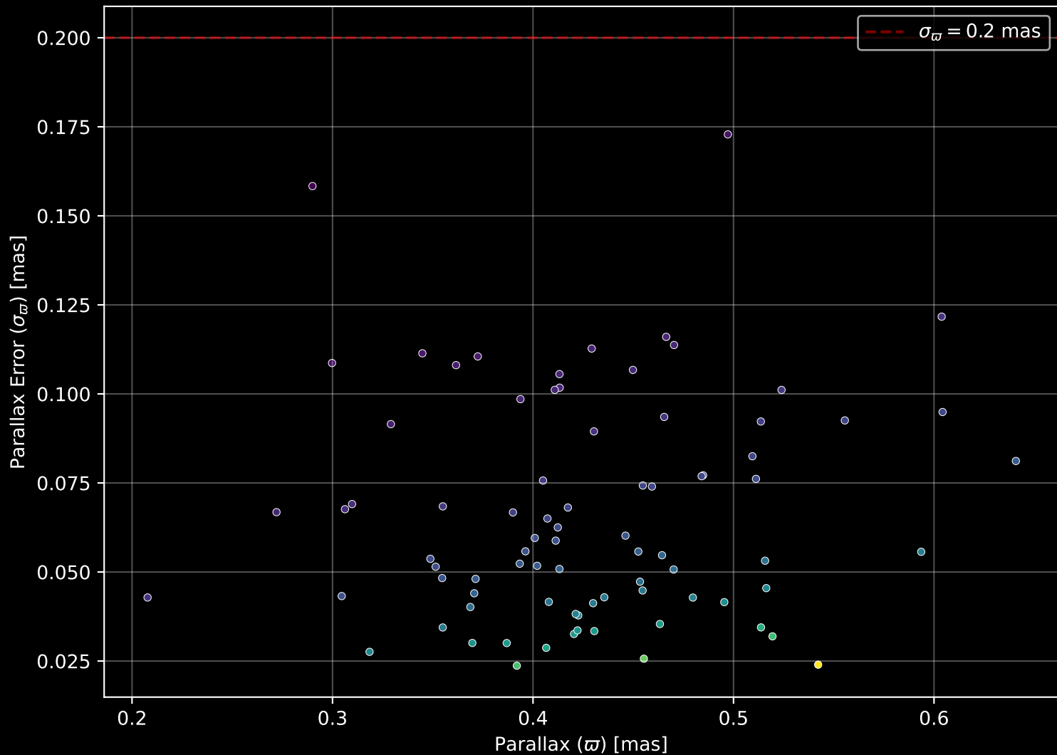
Gaia Cluster: [ESO_134_12] Parallax Quality (n= 82)
