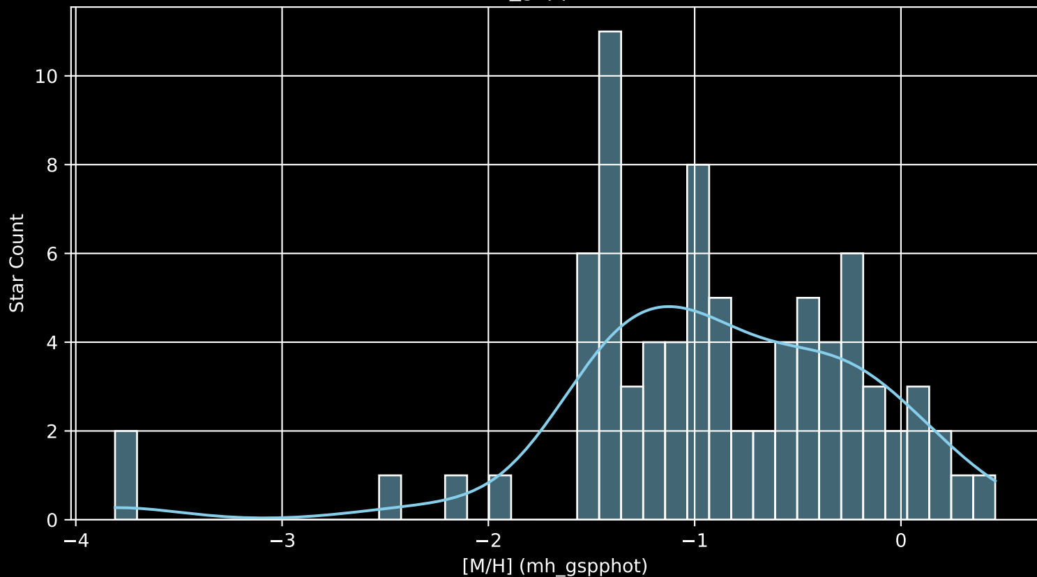
Gaia Cluster: [ESO_134_12 [M/H] (mh_gspphot) (n= 81)
