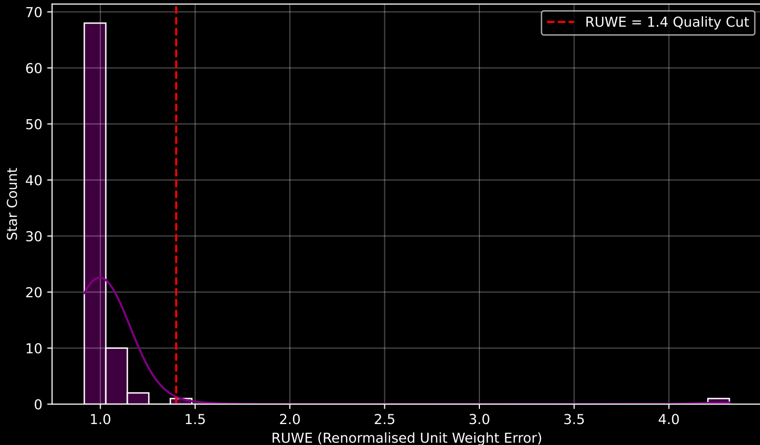
Gaia Cluster: [ESO_134_12] RUWE Distribution (n= 82)
