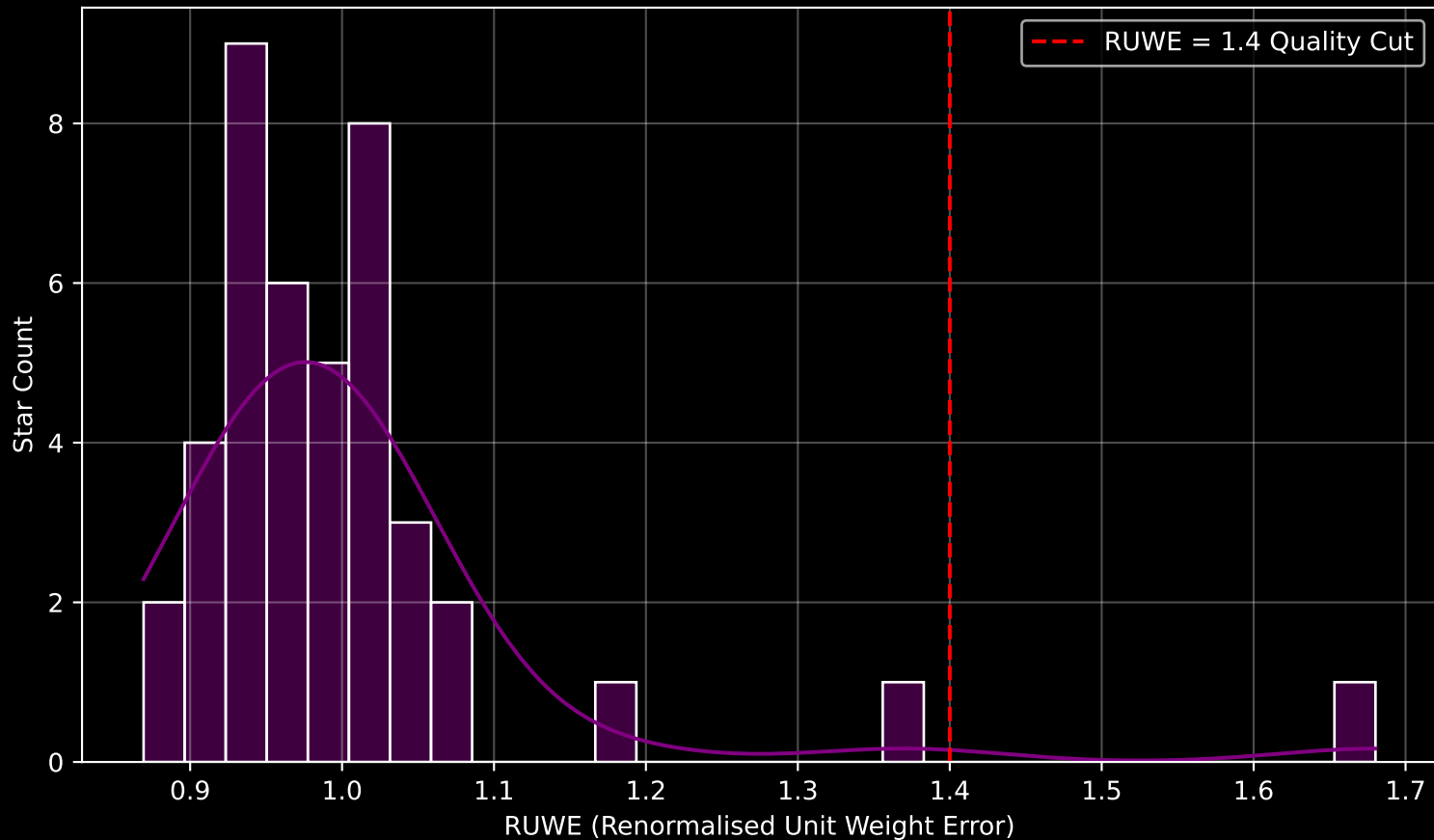
Gaia Cluster: [ESO_166_04] RUWE Distribution (n= 42)
