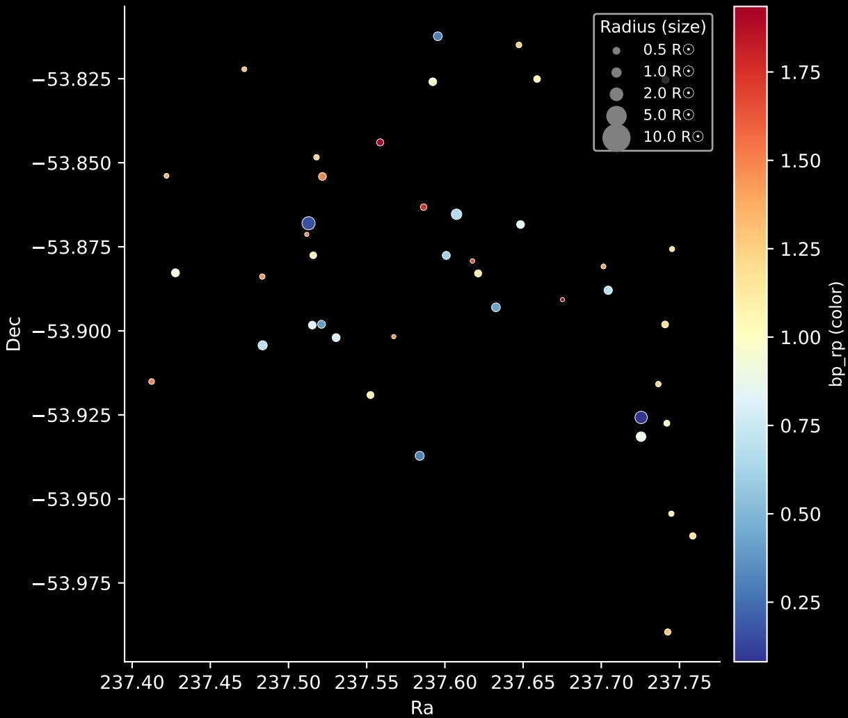
Stars: 42
