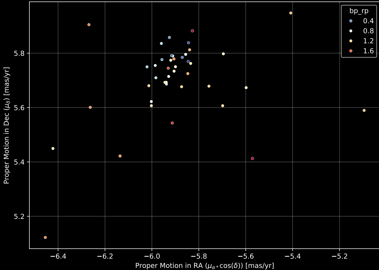
Gaia Cluster: [ESO_166_04] Proper Motion Diagram (n= 42)
