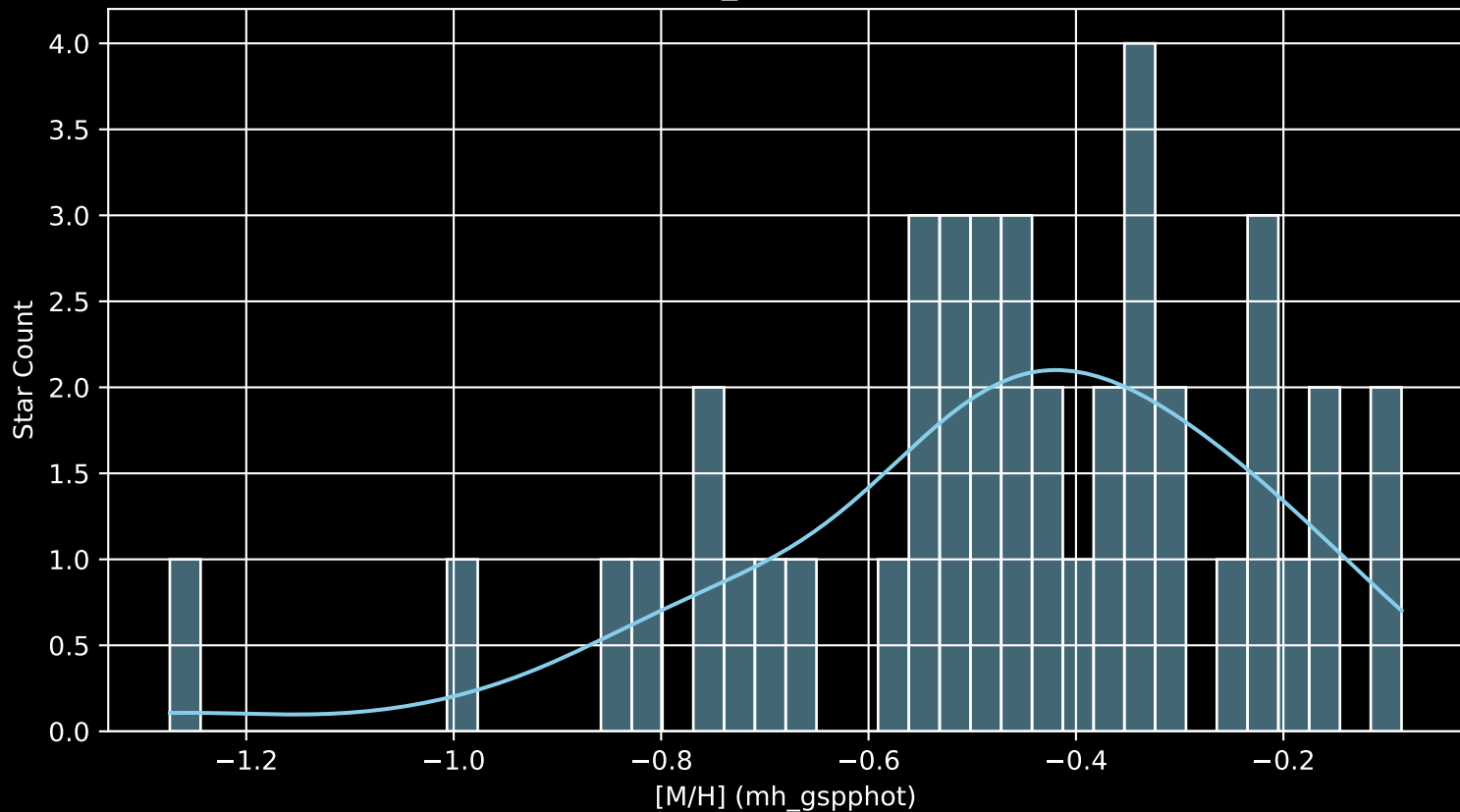
Gaia Cluster: [ESO_166_04 [M/H] (mh_gspphot) (n= 42)
