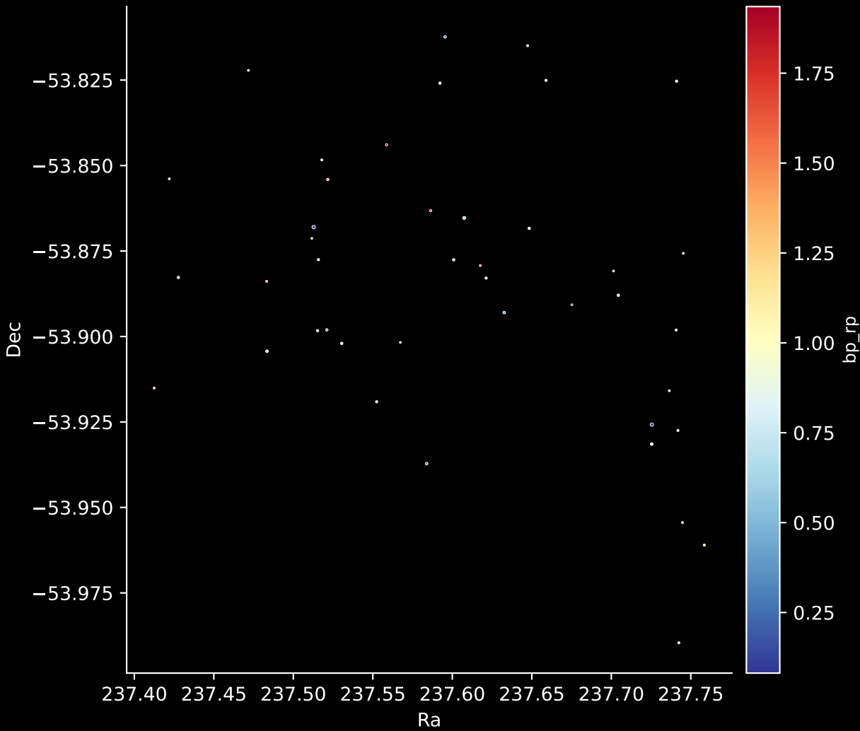
Gaia Cluster: [ESO_166_04]
