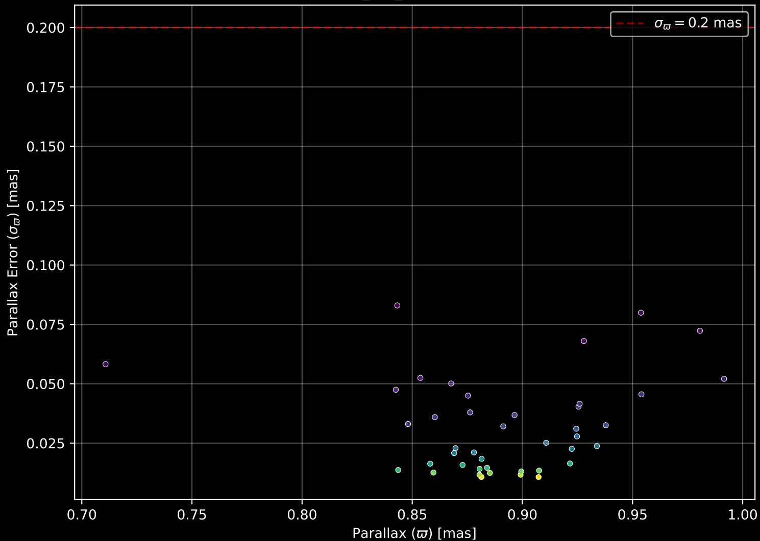
Gaia Cluster: [ESO_166_04] Parallax Quality (n= 42)
