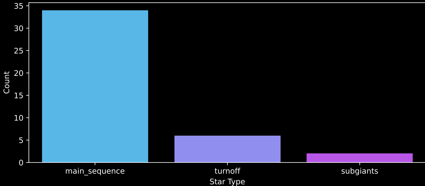
Gaia Cluster: [ESO_166_04] Count plot of Star Type
