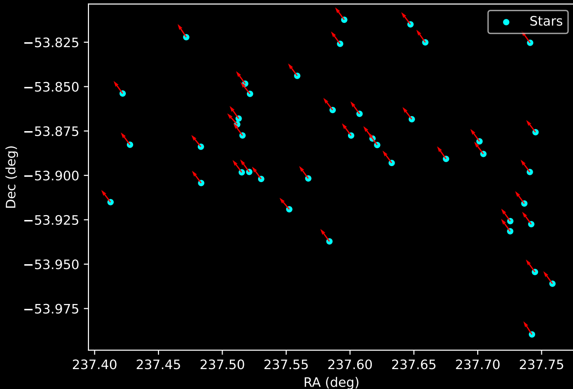
Gaia Cluster: [ESO_166_04] Proper Motion Vectors for Gaia Star Field (n= 42)
