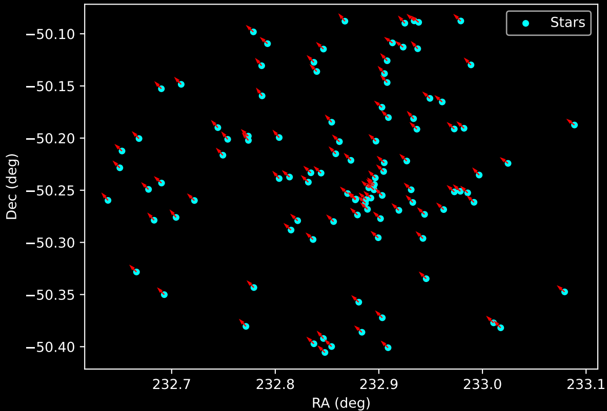
Gaia Cluster: [ESO_211_03] Proper Motion Vectors for Gaia Star Field (n= 106)
