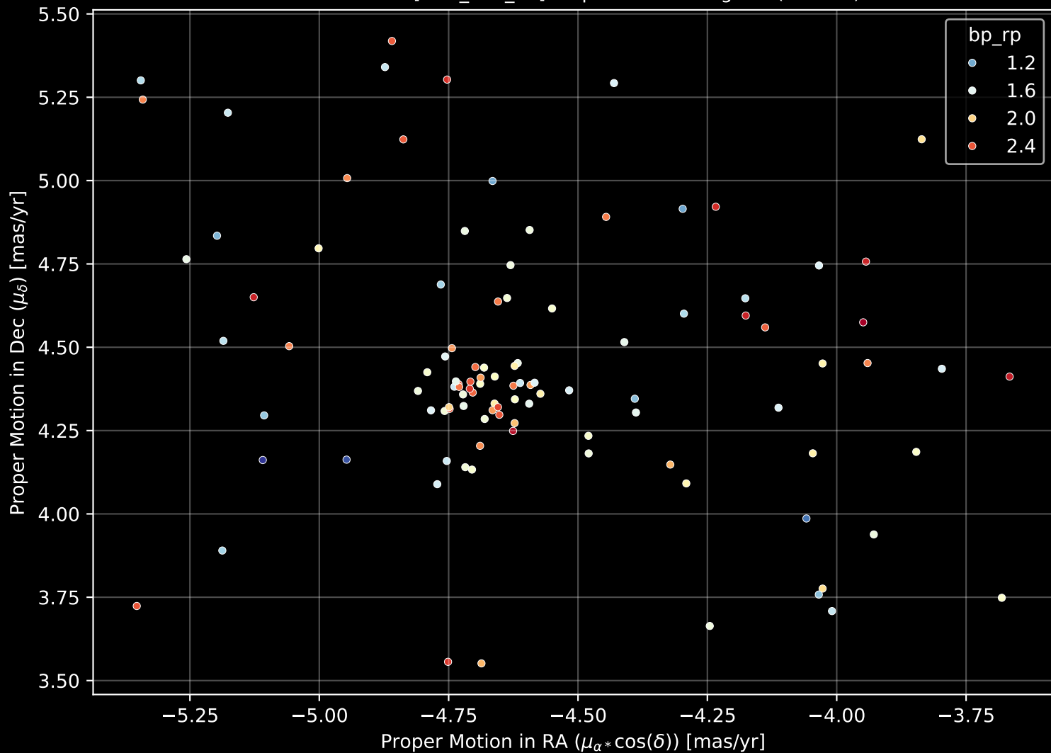
Gaia Cluster: [ESO_211_03] Proper Motion Diagram (n= 106)
