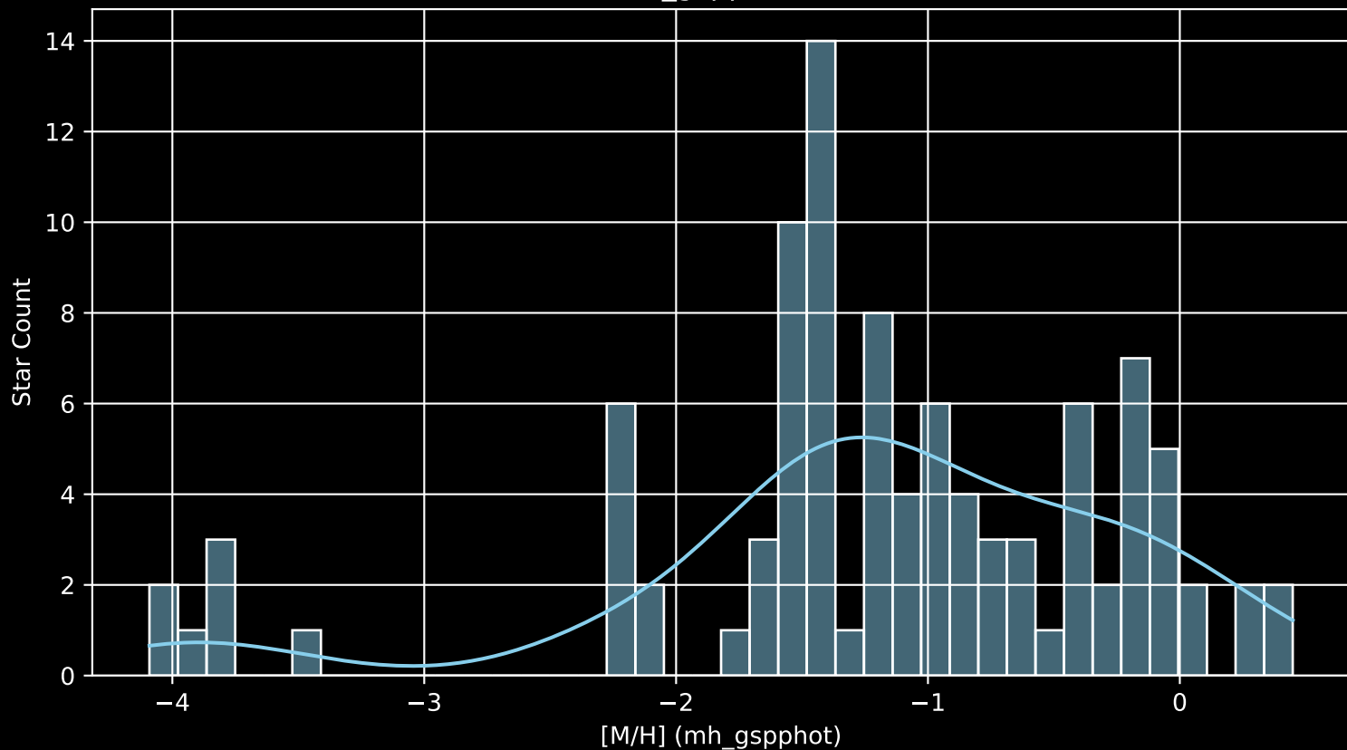
Gaia Cluster: [ESO_211_03 [M/H] (mh_gspphot) (n= 99)
