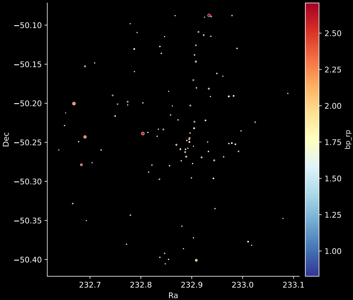
Gaia Cluster: [ESO_211_03] Stars: 106
