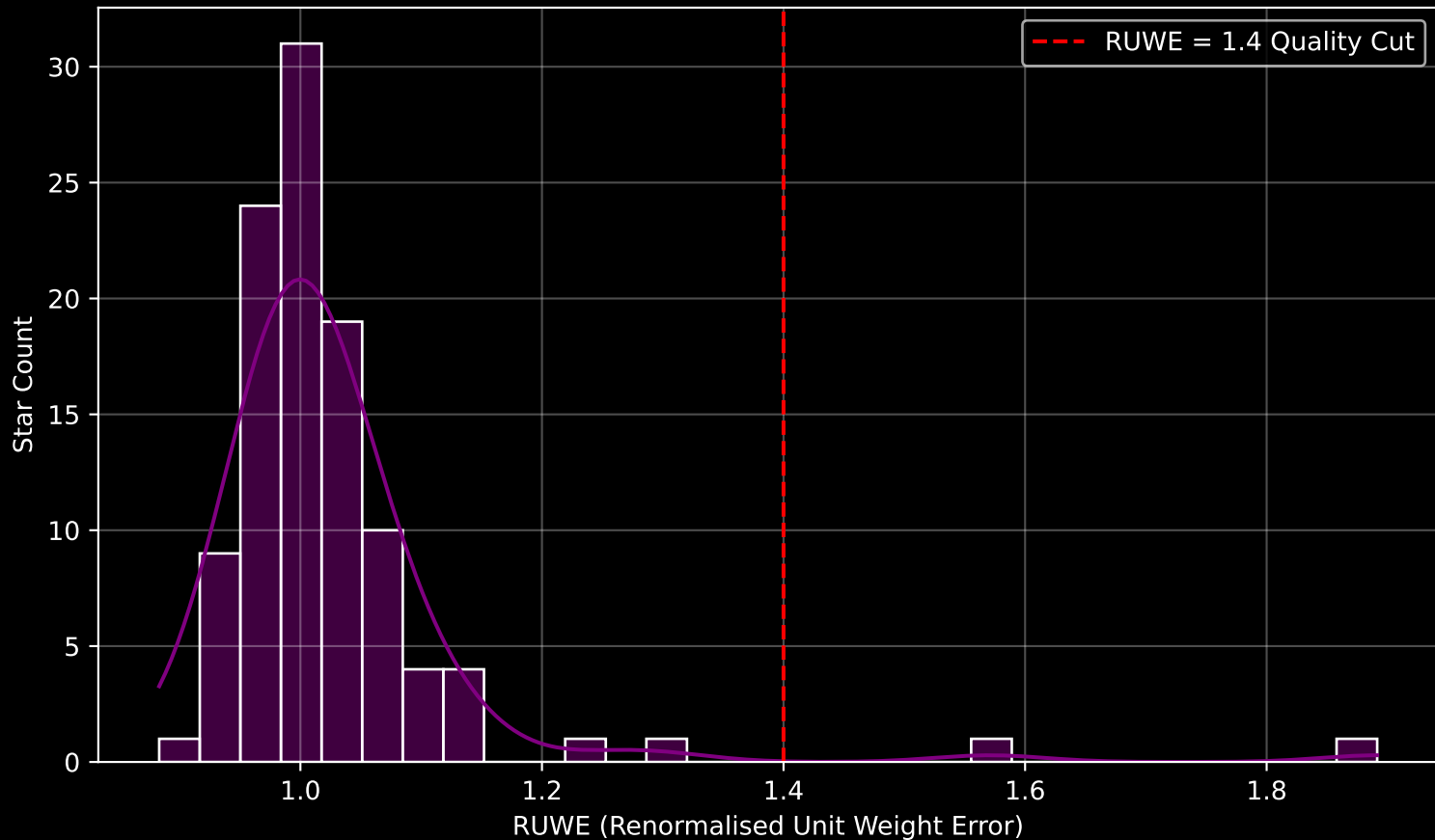
Gaia Cluster: [ESO_211_03] RUWE Distribution (n= 106)
