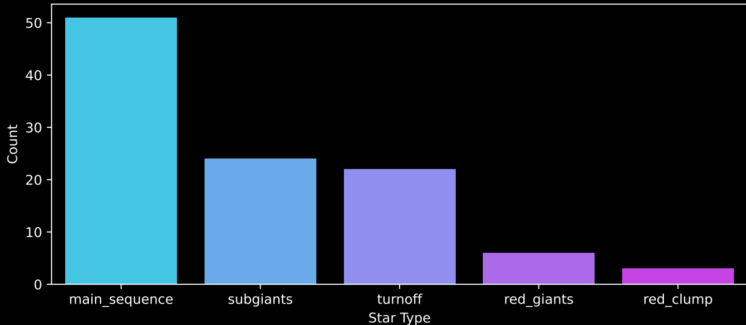
Gaia Cluster: [ESO_211_03] Count plot of Star Type
