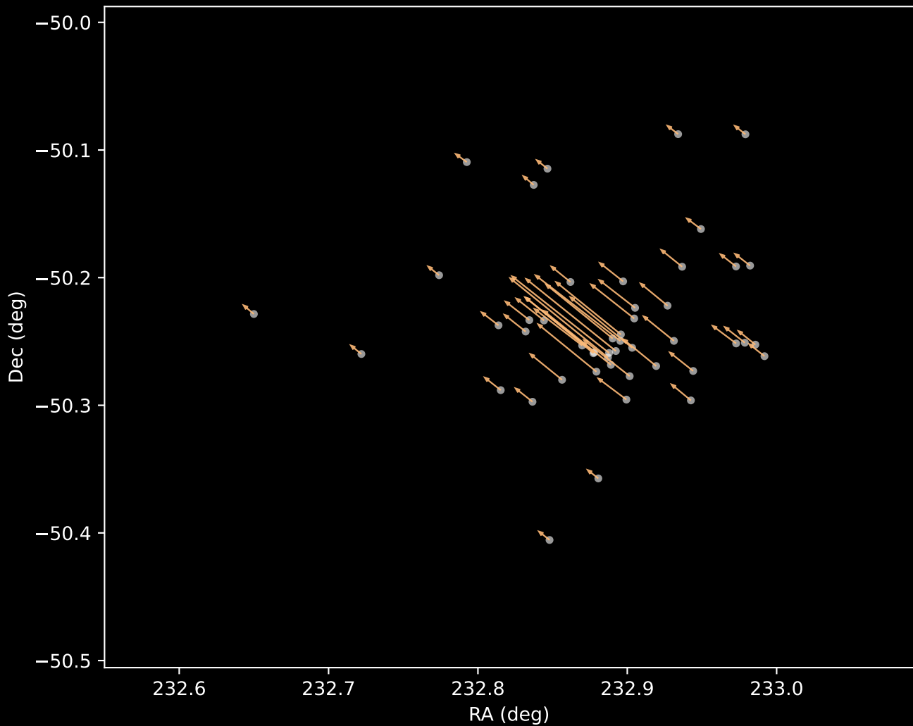
Gaia DR3 Cluster 3 Proper Motion Vectors (n=48)
