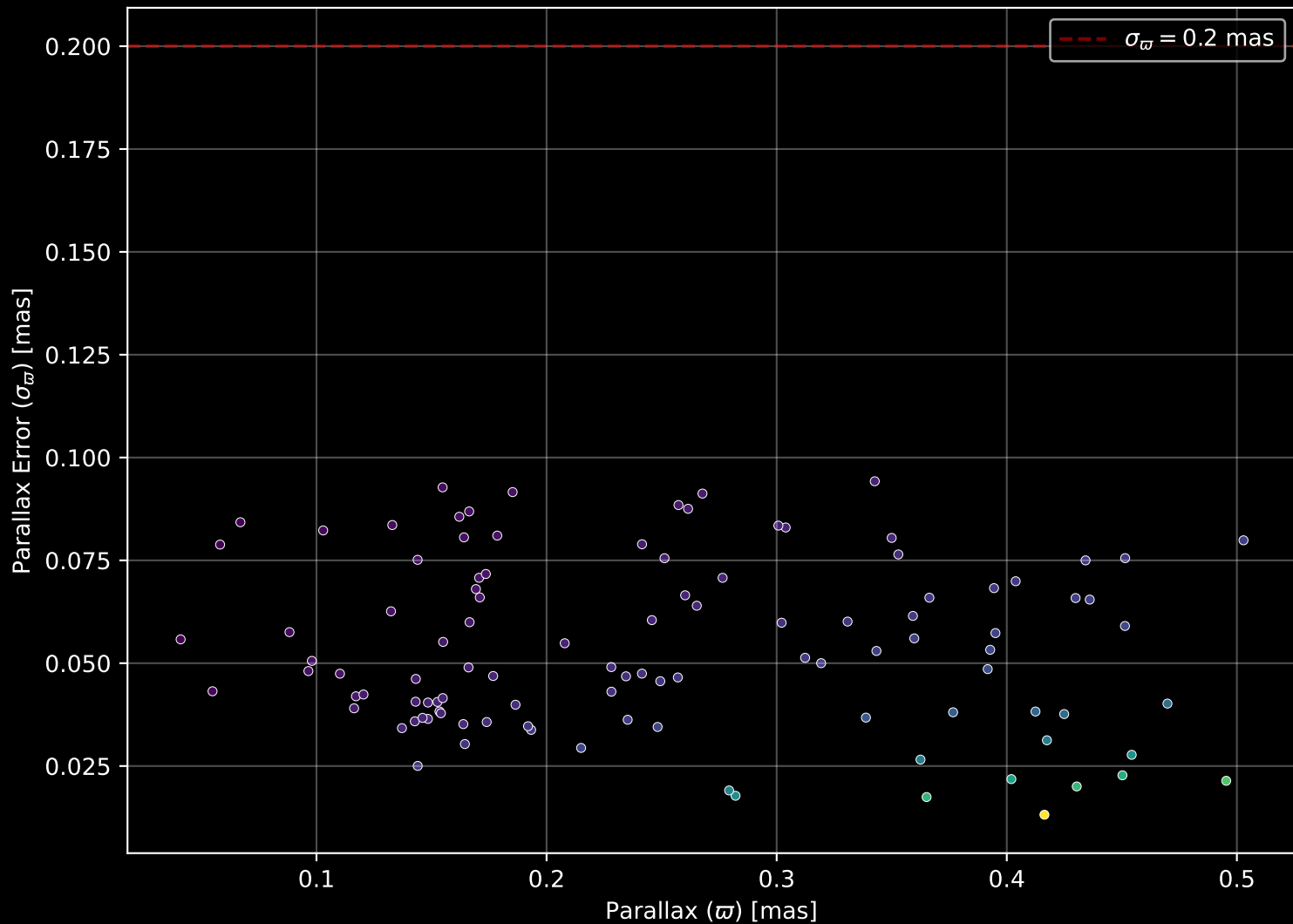
Gaia Cluster: [ESO_211_03] Parallax Quality (n= 106)
