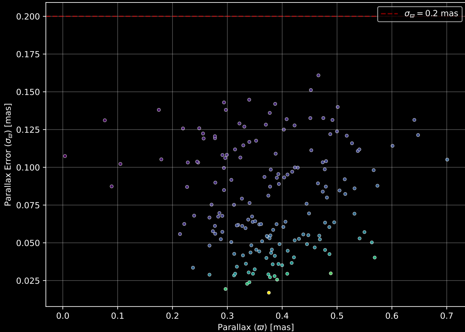
Gaia Cluster: [ESO_226_06] Parallax Quality (n= 175)
