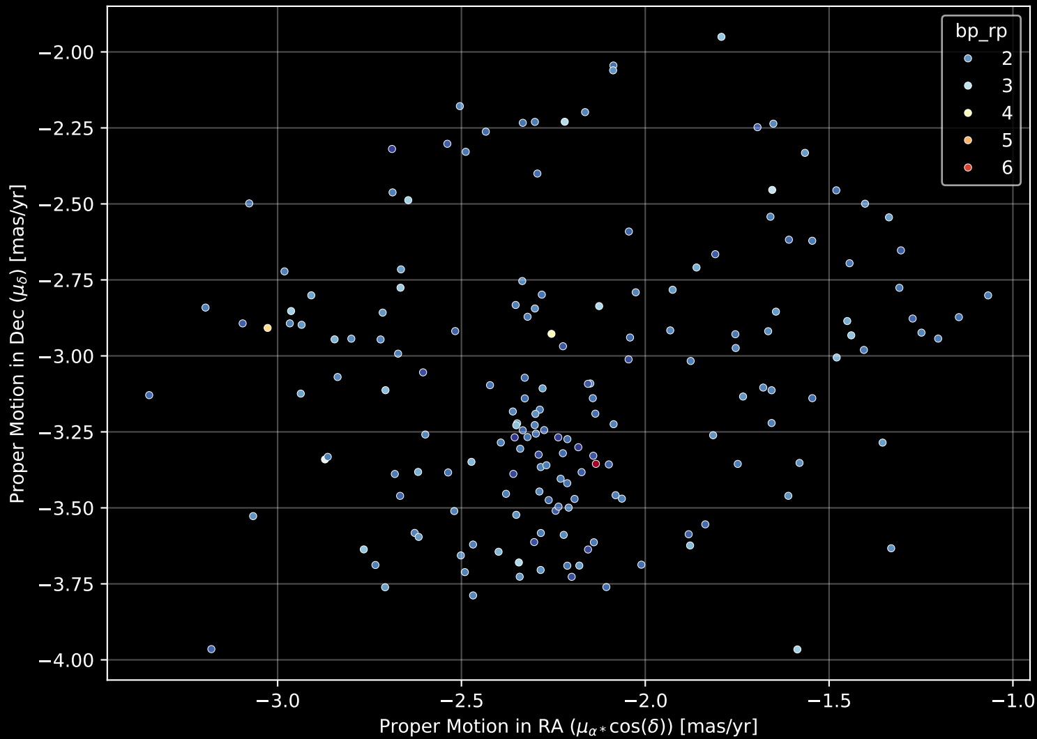
Gaia Cluster: [ESO_226_06] Proper Motion Diagram (n= 175)
