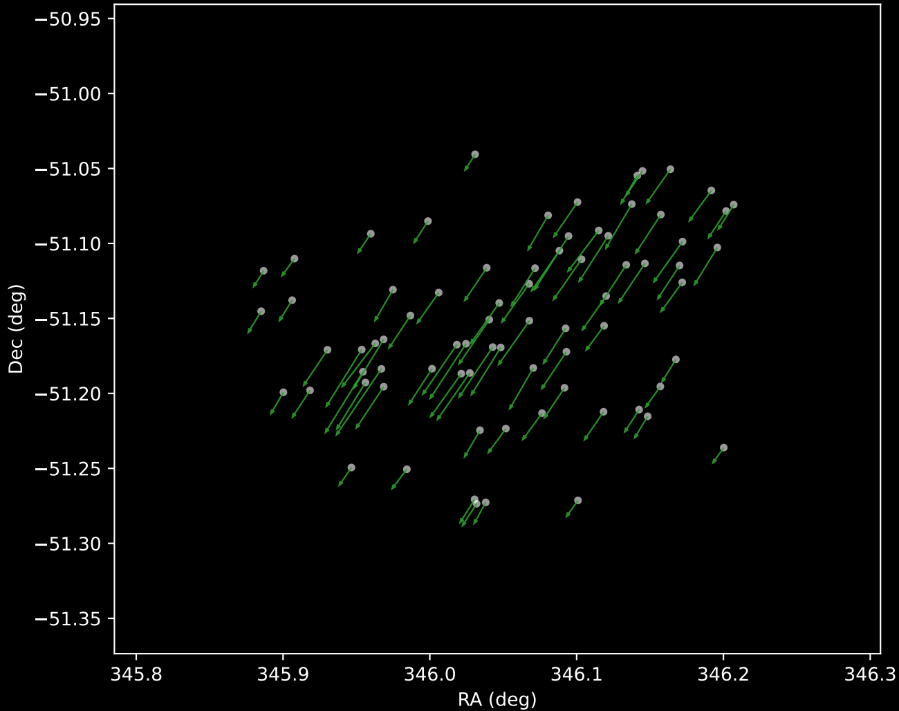
Gaia DR3 Cluster 4 Proper Motion Vectors (n=75)
