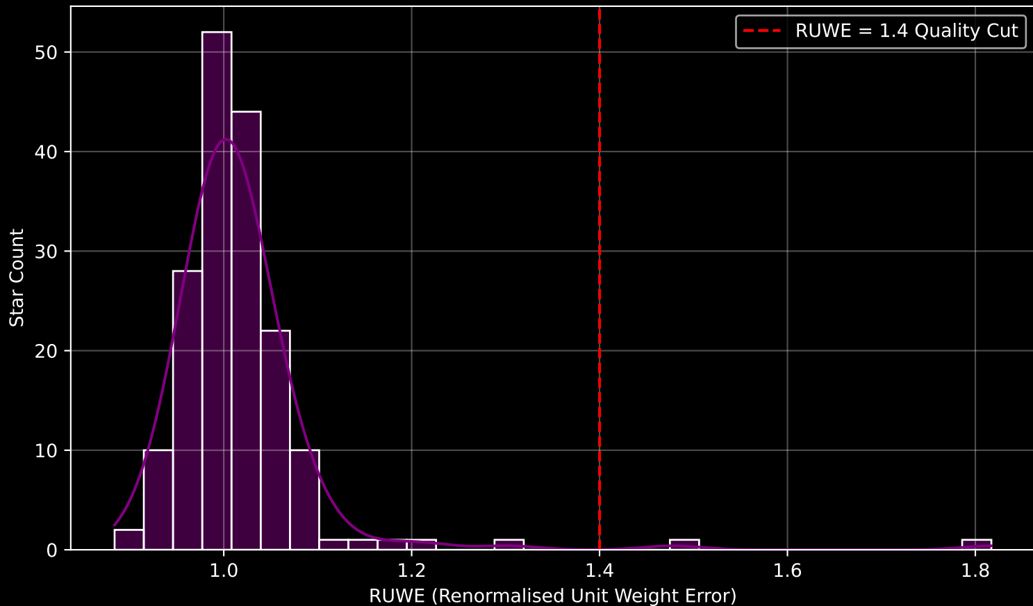
Gaia Cluster: [ESO_226_06] RUWE Distribution (n= 175)
