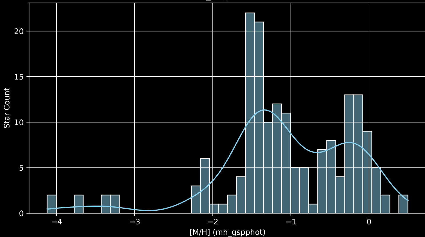
Gaia Cluster: [ESO_226_06 [M/H] (mh_gspphot) (n= 175)
