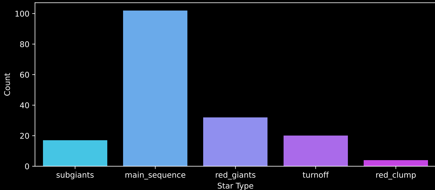
Gaia Cluster: [ESO_226_06] Count plot of Star Type
