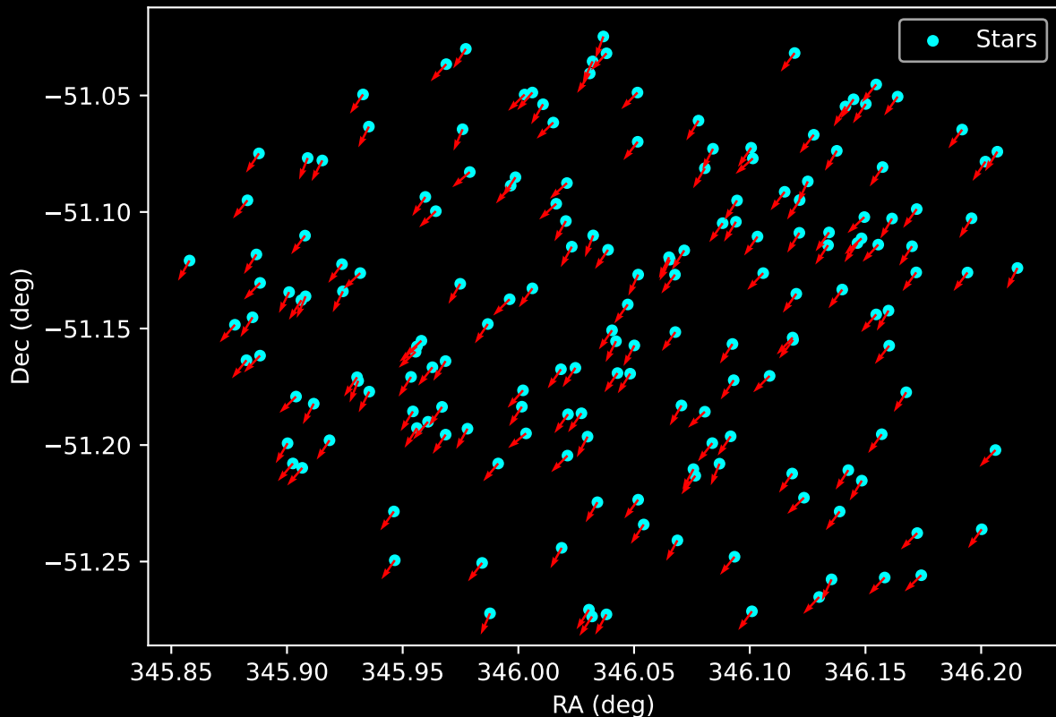
Gaia Cluster: [ESO_226_06] Proper Motion Vectors for Gaia Star Field (n= 175)
