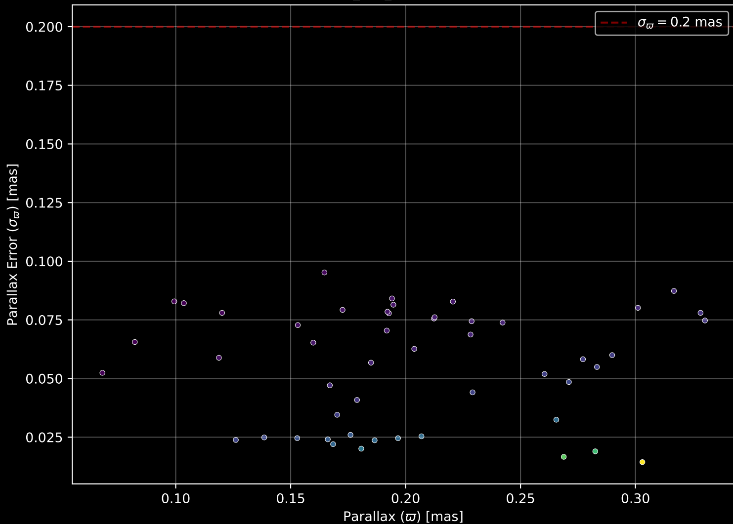
Gaia Cluster: [ESO_311_21] Parallax Quality (n= 50)
