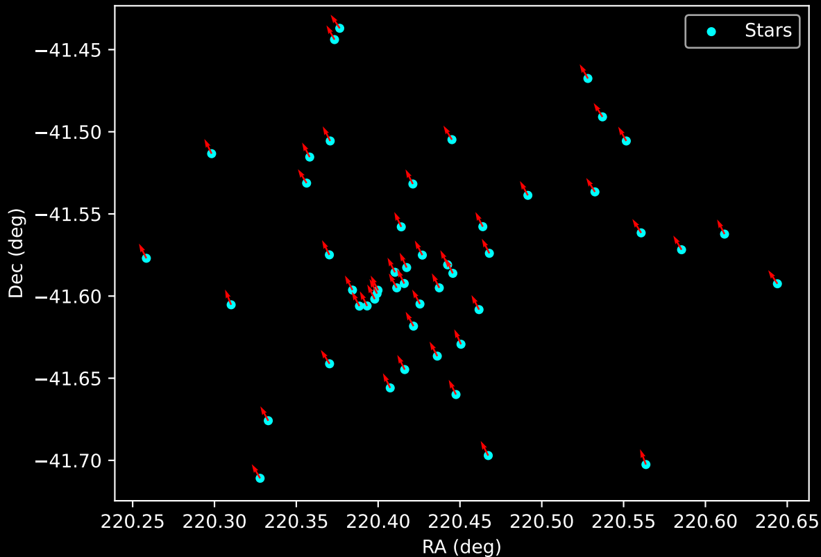
Gaia Cluster: [ESO_311_21] Proper Motion Vectors for Gaia Star Field (n= 50)
