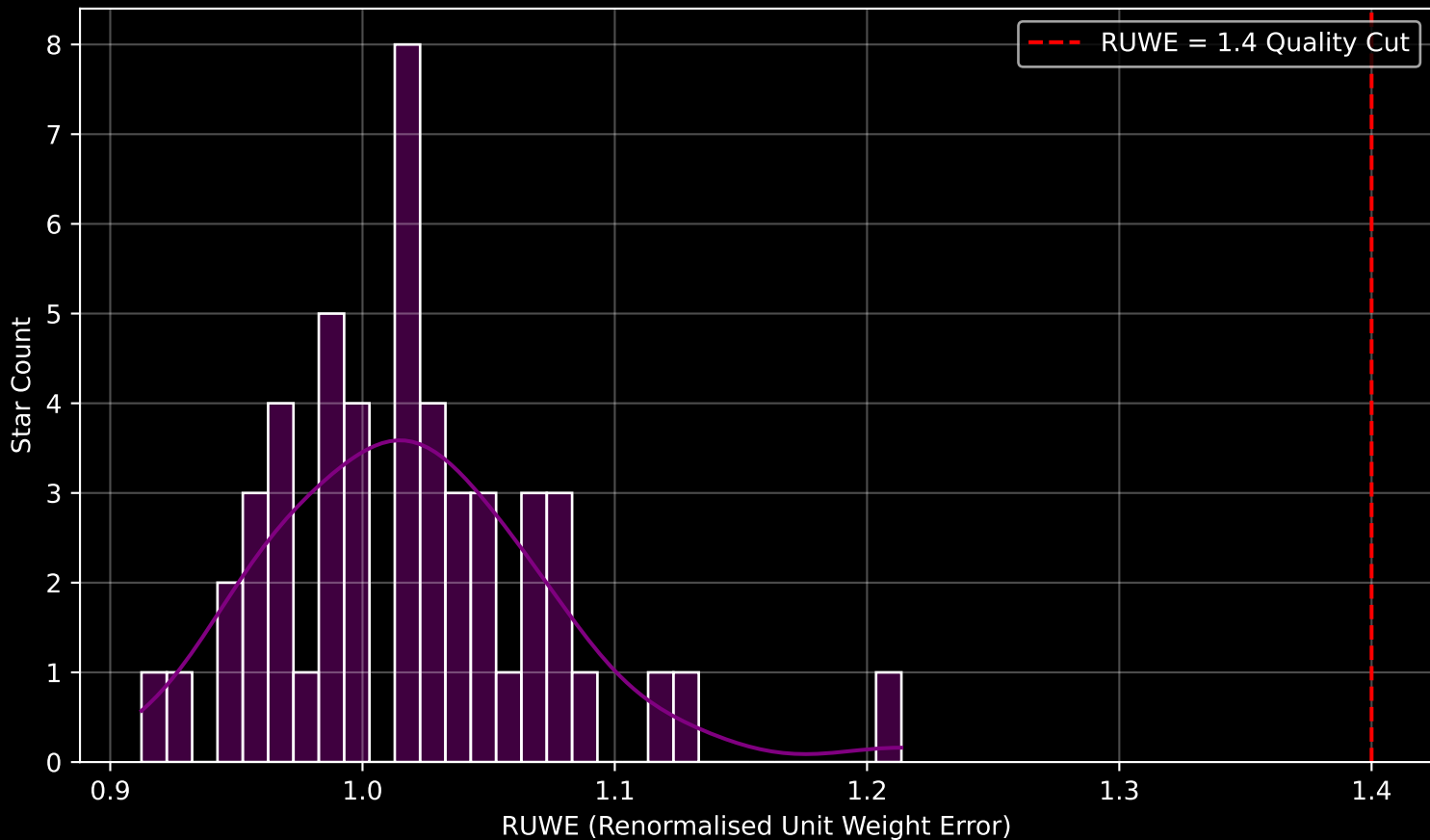
Gaia Cluster: [ESO_311_21] RUWE Distribution (n= 50)
