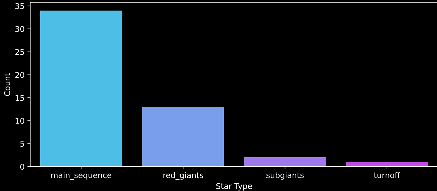
Gaia Cluster: [ESO_311_21] Count plot of Star Type
