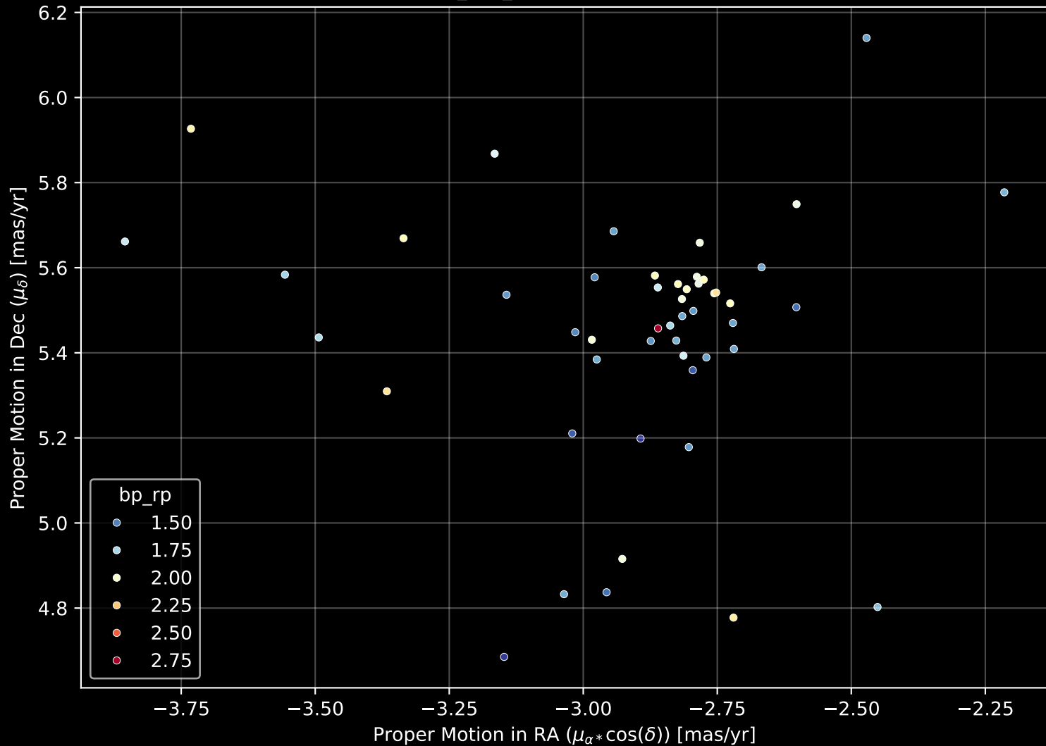
Gaia Cluster: [ESO_311_21] Proper Motion Diagram (n= 50)
