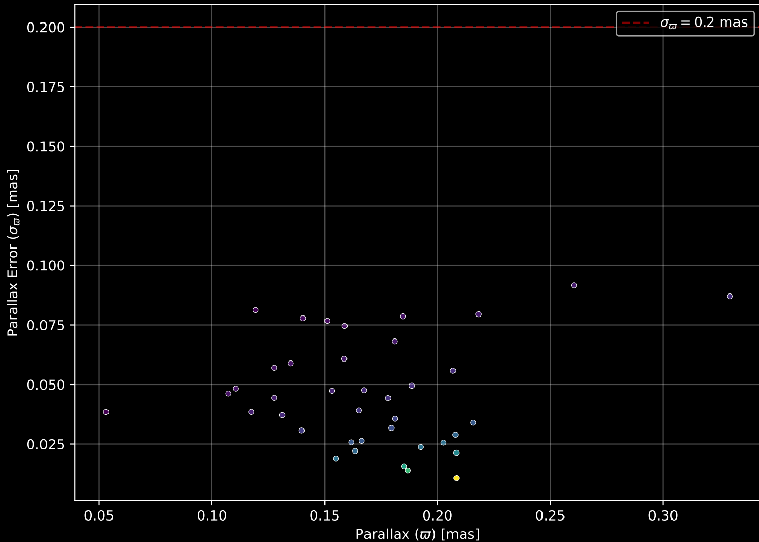
Gaia Cluster: [ESO_312_04] Parallax Quality (n= 39)
