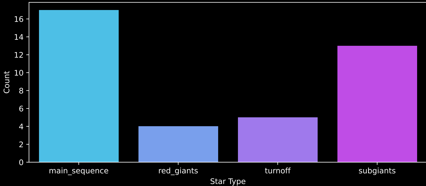
Gaia Cluster: [ESO_312_04] Count plot of Star Type
