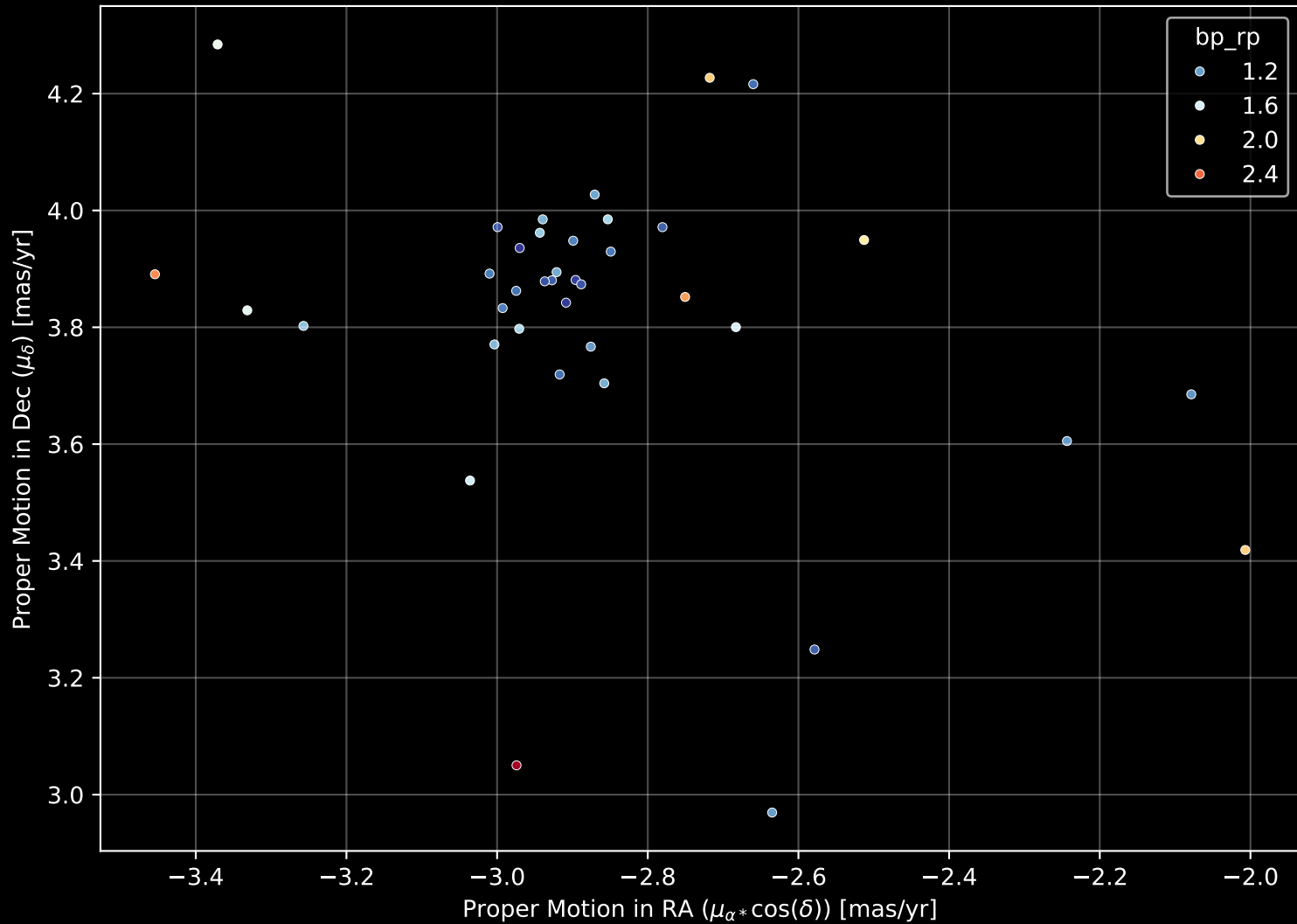
Gaia Cluster: [ESO_312_04] Proper Motion Diagram (n= 39)
