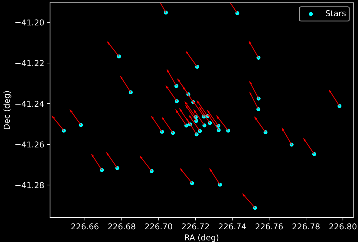
Gaia Cluster: [ESO_312_04] Proper Motion Vectors for Gaia Star Field (n= 39)
