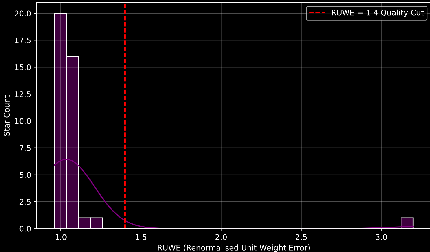
Gaia Cluster: [ESO_312_04] RUWE Distribution (n= 39)
