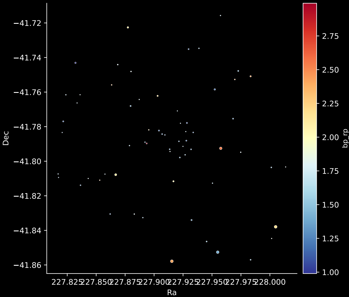
Gaia Cluster: [ESO_313_03] Stars: 64
