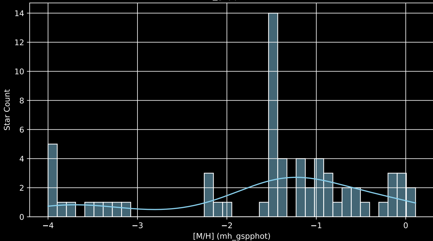
Gaia Cluster: [ESO_313_03 [M/H] (mh_gspphot) (n= 64)
