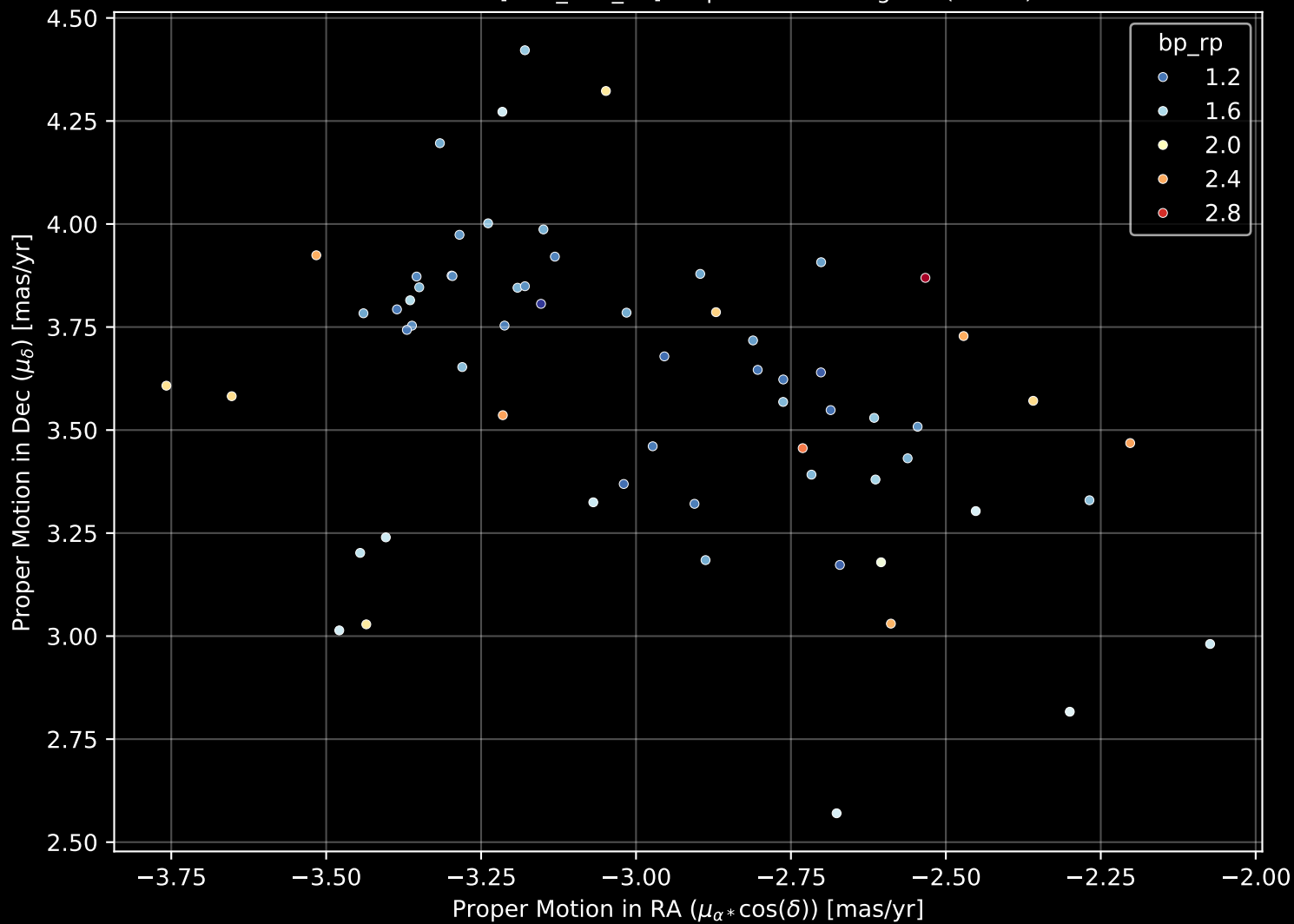
Gaia Cluster: [ESO_313_03] Proper Motion Diagram (n= 64)
