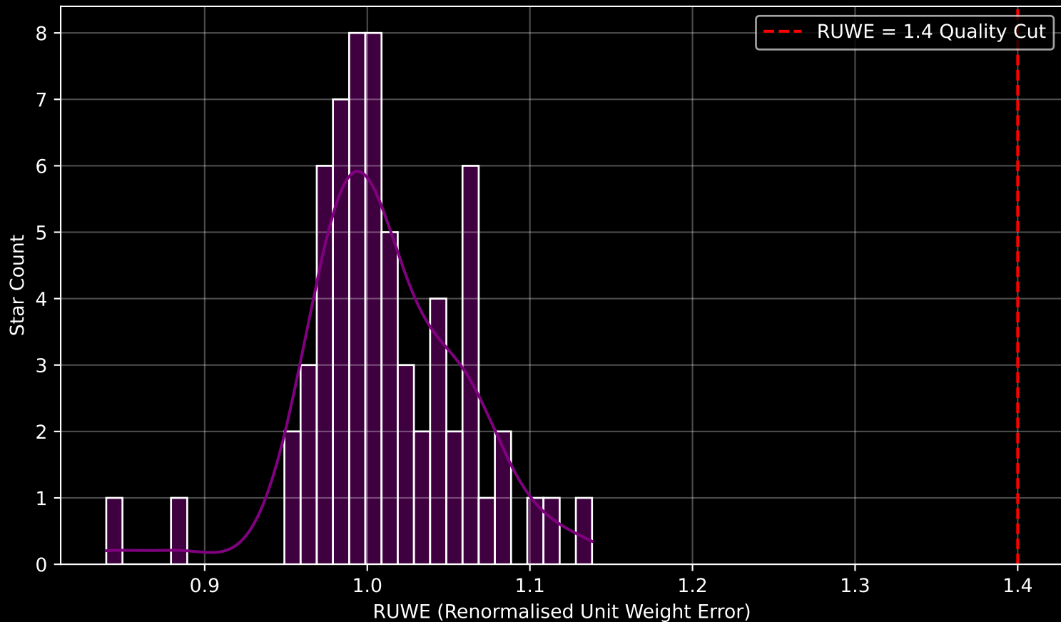
Gaia Cluster: [ESO_313_03] RUWE Distribution (n= 64)
