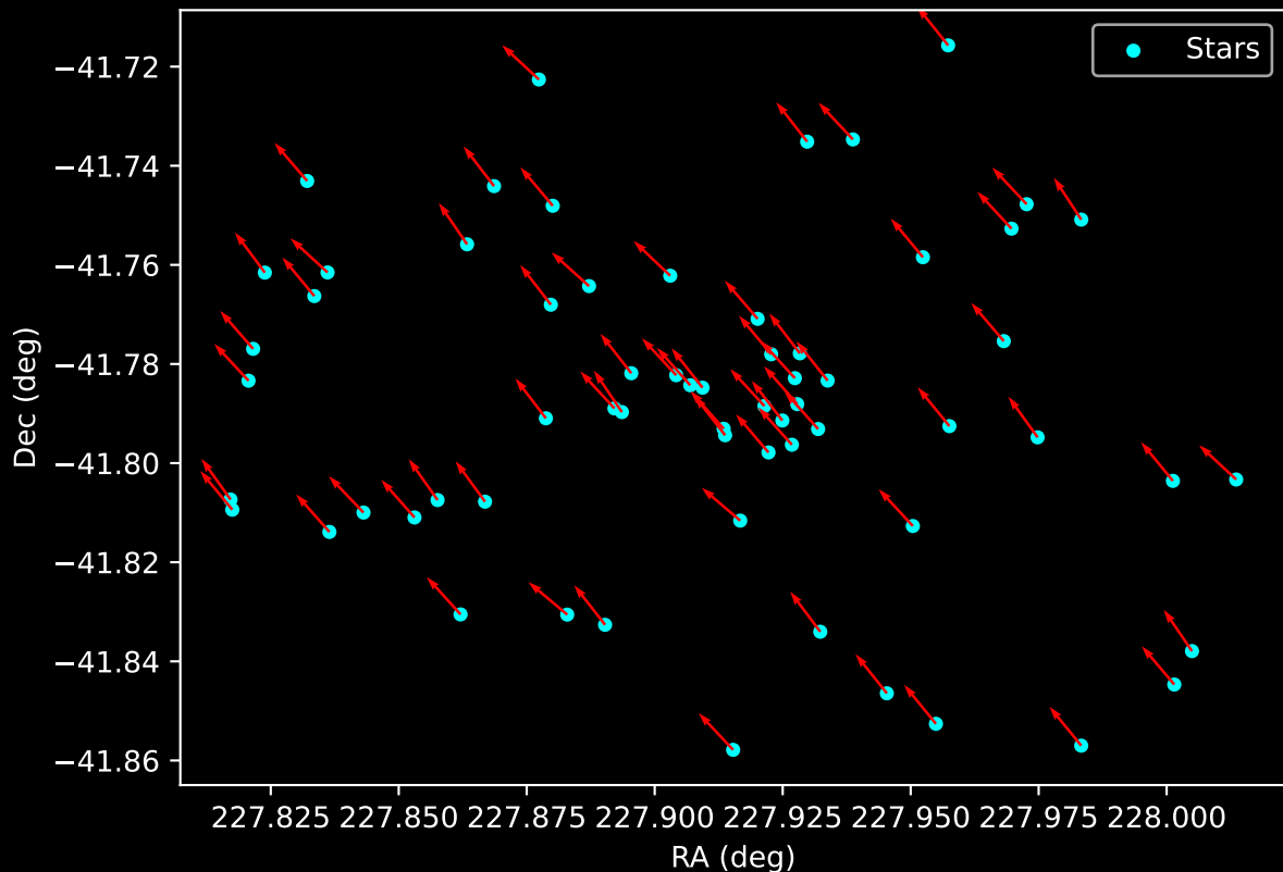
Gaia Cluster: [ESO_313_03] Proper Motion Vectors for Gaia Star Field (n= 64)
