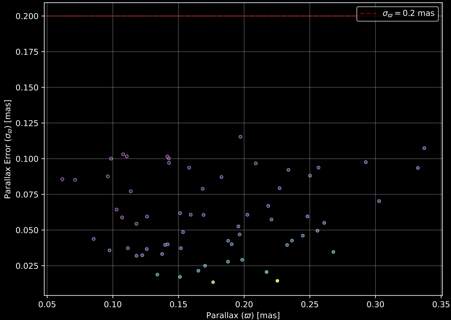
Gaia Cluster: [ESO_313_03] Parallax Quality (n= 64)
