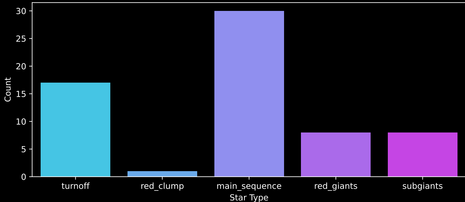
Gaia Cluster: [ESO_313_03] Count plot of Star Type
