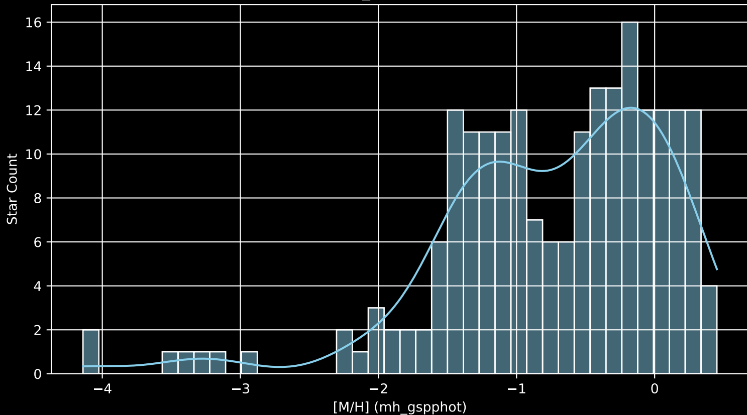
Gaia Cluster: [ESO_393_15 [M/H] (mh_gspphot) (n= 206)
