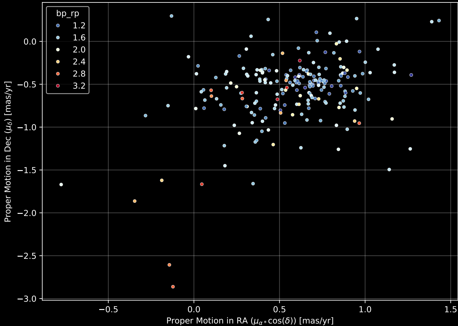
Gaia Cluster: [ESO_393_15] Proper Motion Diagram (n= 217)
