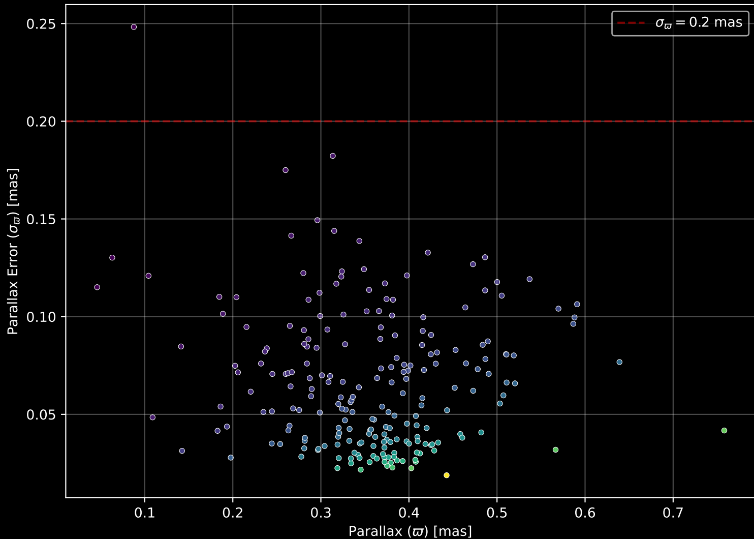
Gaia Cluster: [ESO_393_15] Parallax Quality (n= 217)
