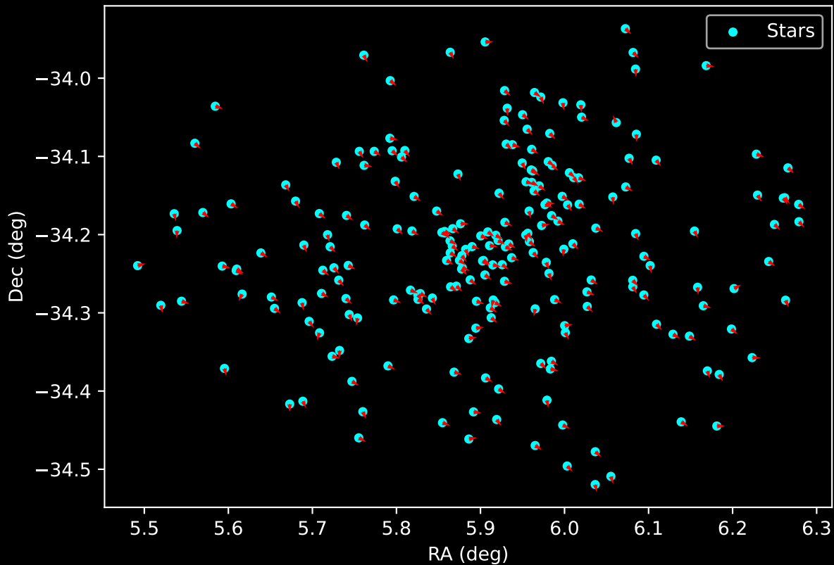
Gaia Cluster: [ESO_393_15] Proper Motion Vectors for Gaia Star Field (n= 217)
