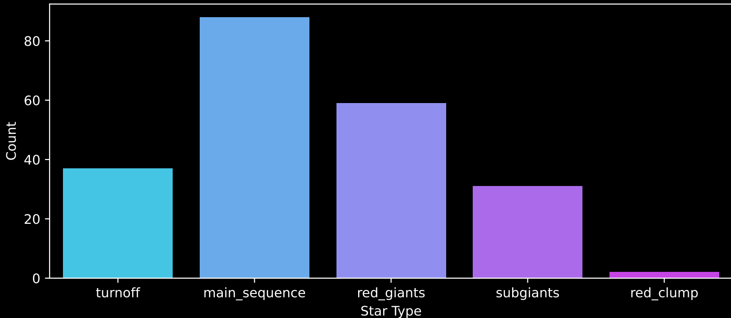
Gaia Cluster: [ESO_393_15] Count plot of Star Type
