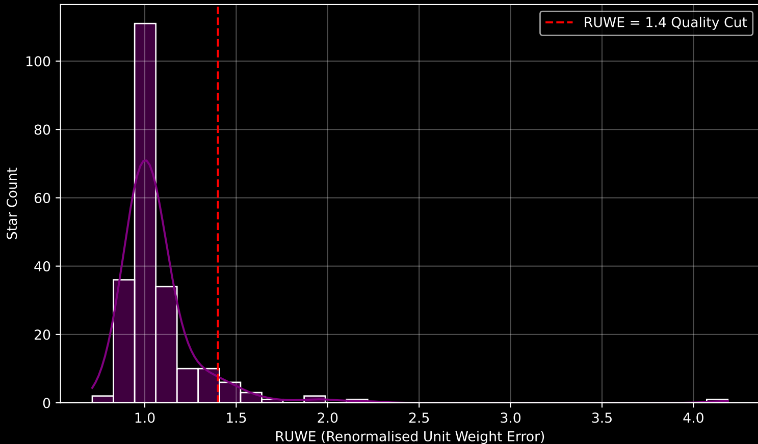
Gaia Cluster: [ESO_393_15] RUWE Distribution (n= 217)
