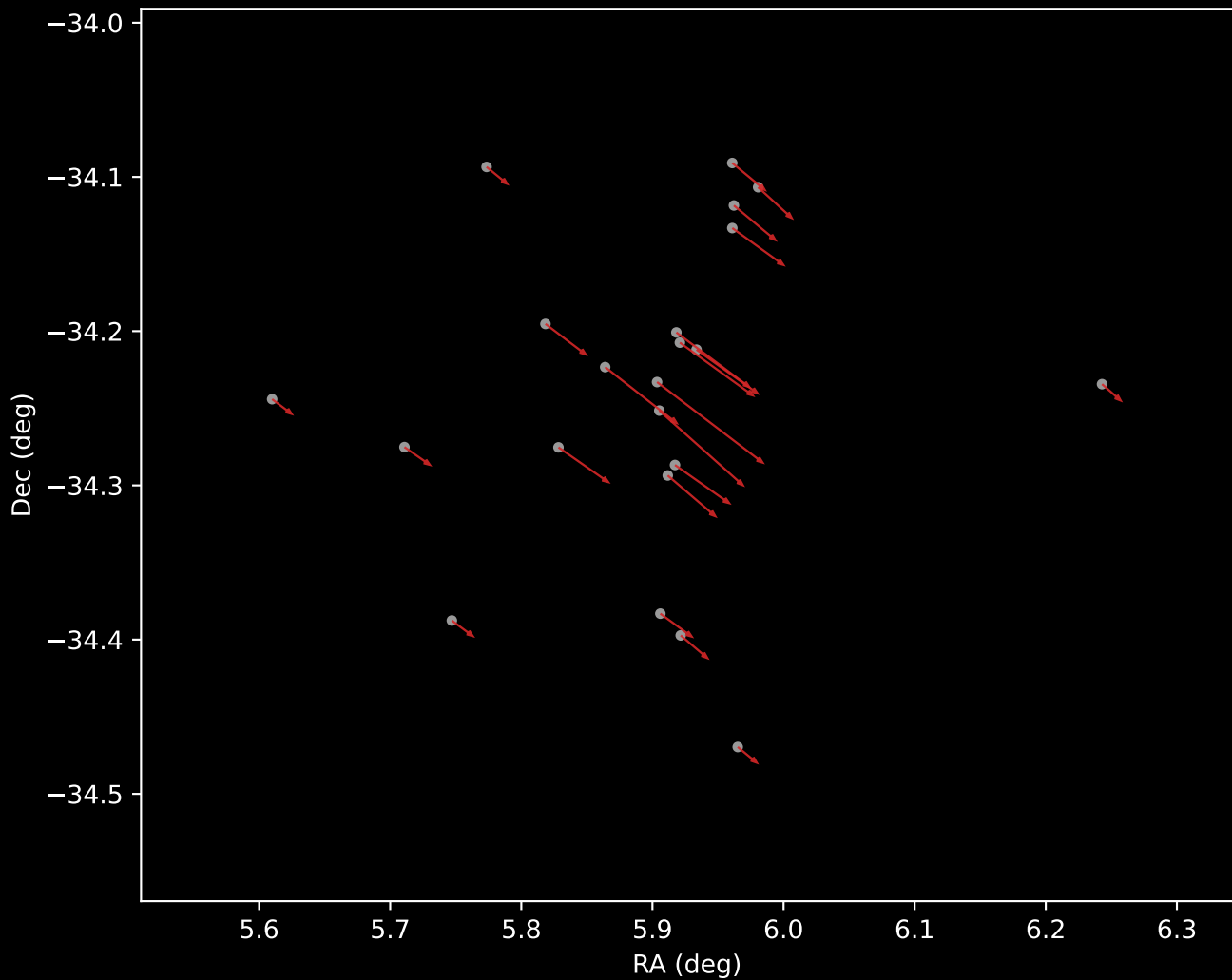
Gaia DR3 Cluster 6 Proper Motion Vectors (n=22)
