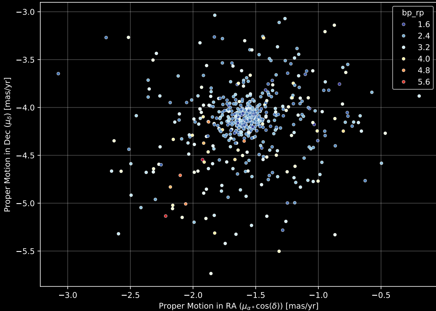
Gaia Cluster: [FSR_0088] Proper Motion Diagram (n= 540)
