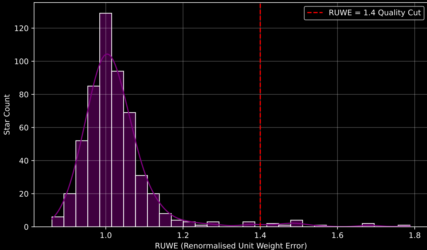
Gaia Cluster: [FSR_0088] RUWE Distribution (n= 539)
