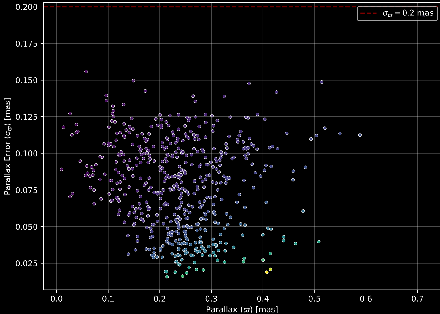
Gaia Cluster: [FSR_0088] Parallax Quality (n= 540)
