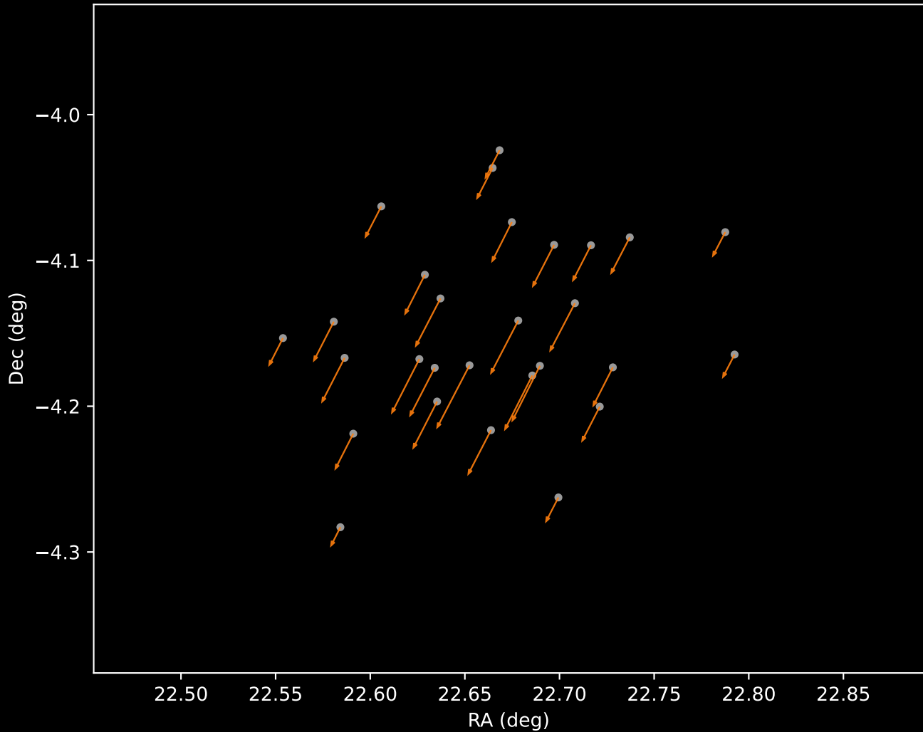
Gaia DR3 Cluster 22 Proper Motion Vectors (n=28)
