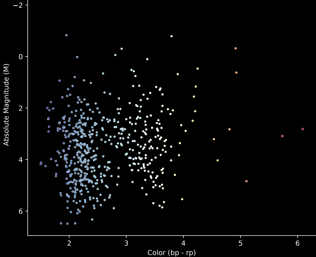
Gaia Cluster: [FSR_0088] Stars (n= 540) Hertzsprung-Russel Diagram
