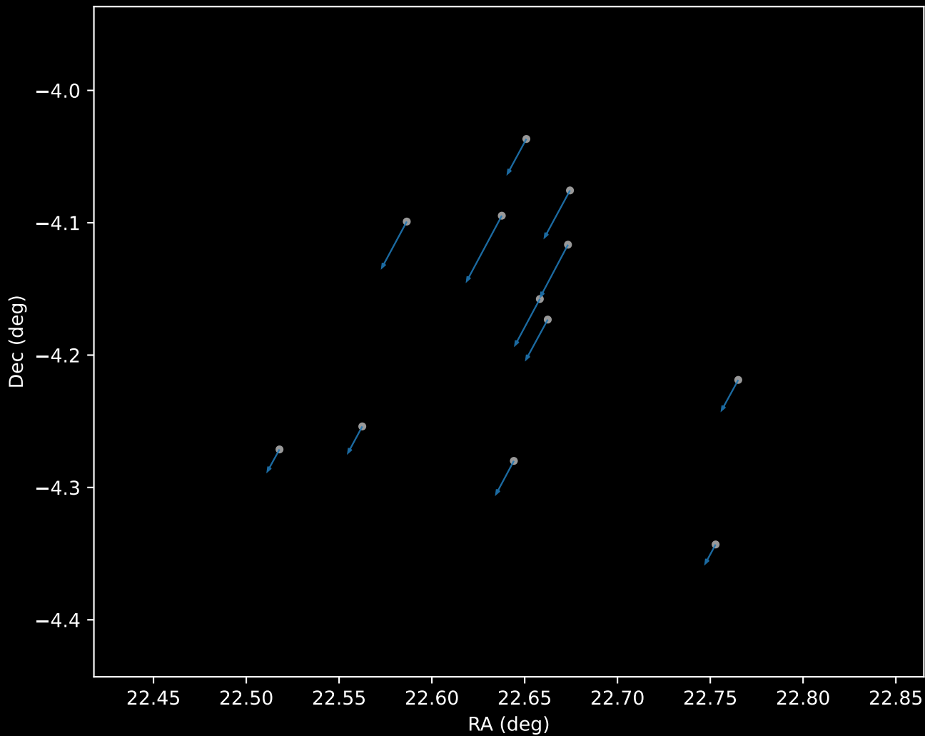
Gaia DR3 Cluster 20 Proper Motion Vectors (n=12)
