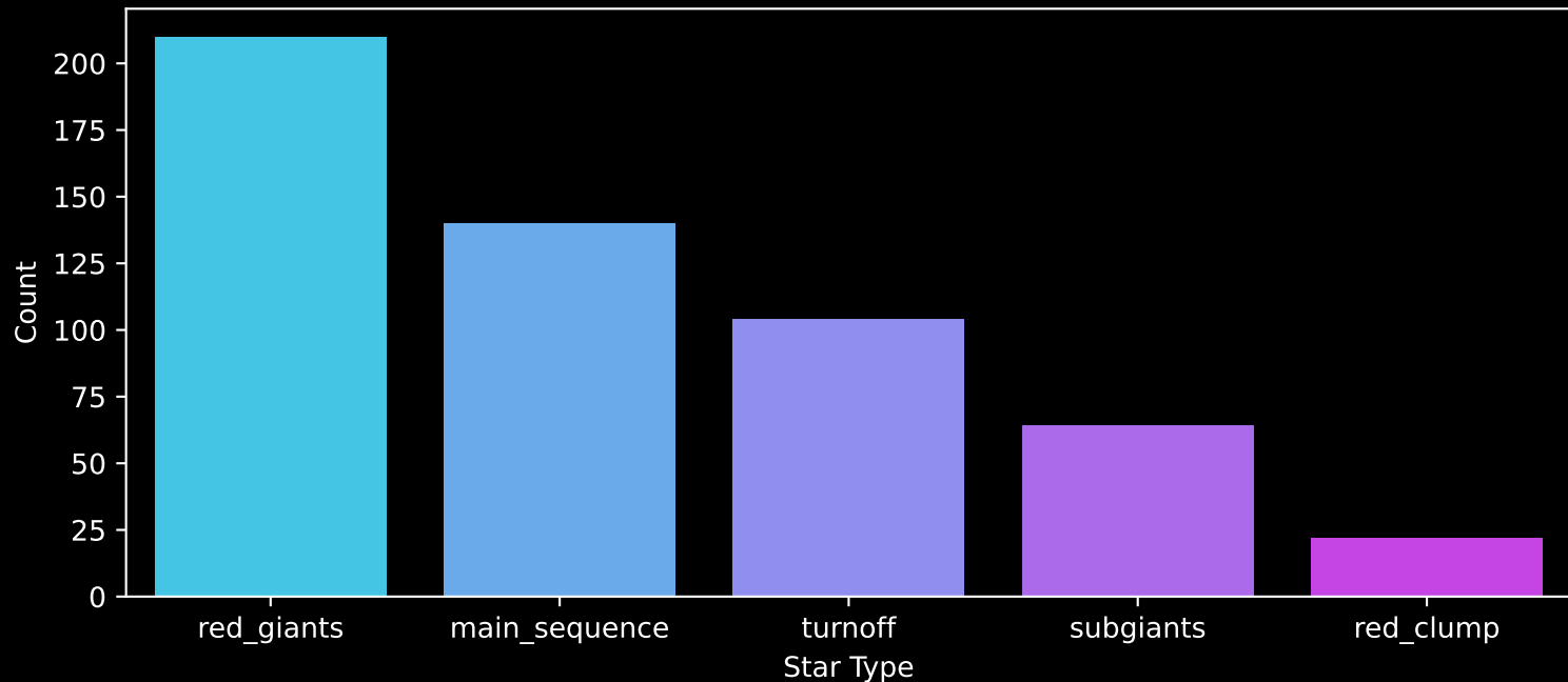
Gaia Cluster: [FSR_0088] Count plot of Star Type
