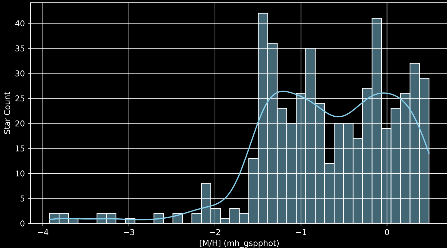
Gaia Cluster: [FSR_0088 [M/H] (mh_gspphot) (n= 518)
