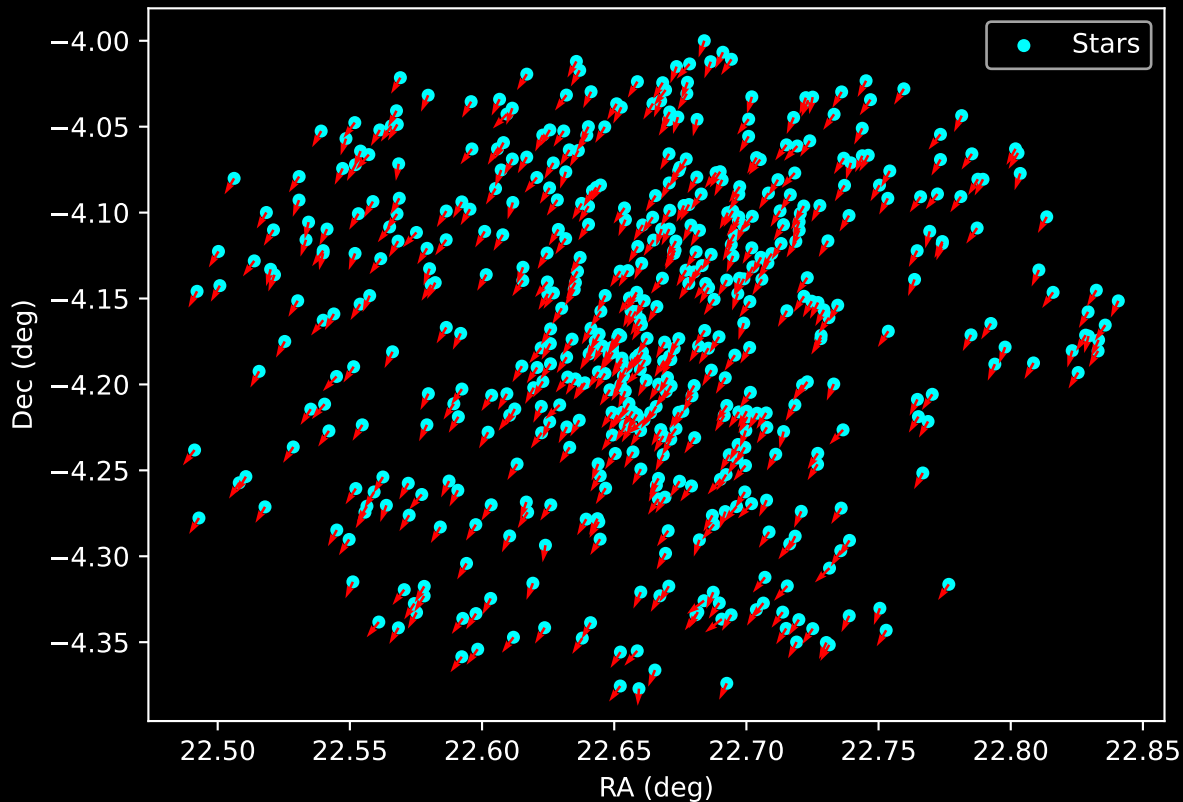
Gaia Cluster: [FSR_0088] Proper Motion Vectors for Gaia Star Field (n= 540)
