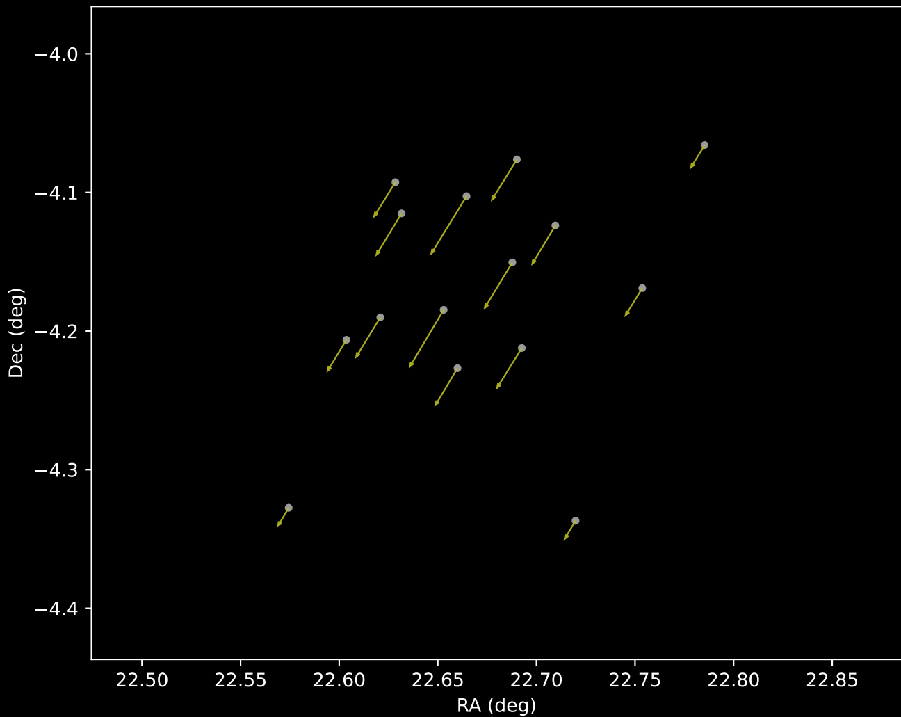
Gaia DR3 Cluster 16 Proper Motion Vectors (n=15)
