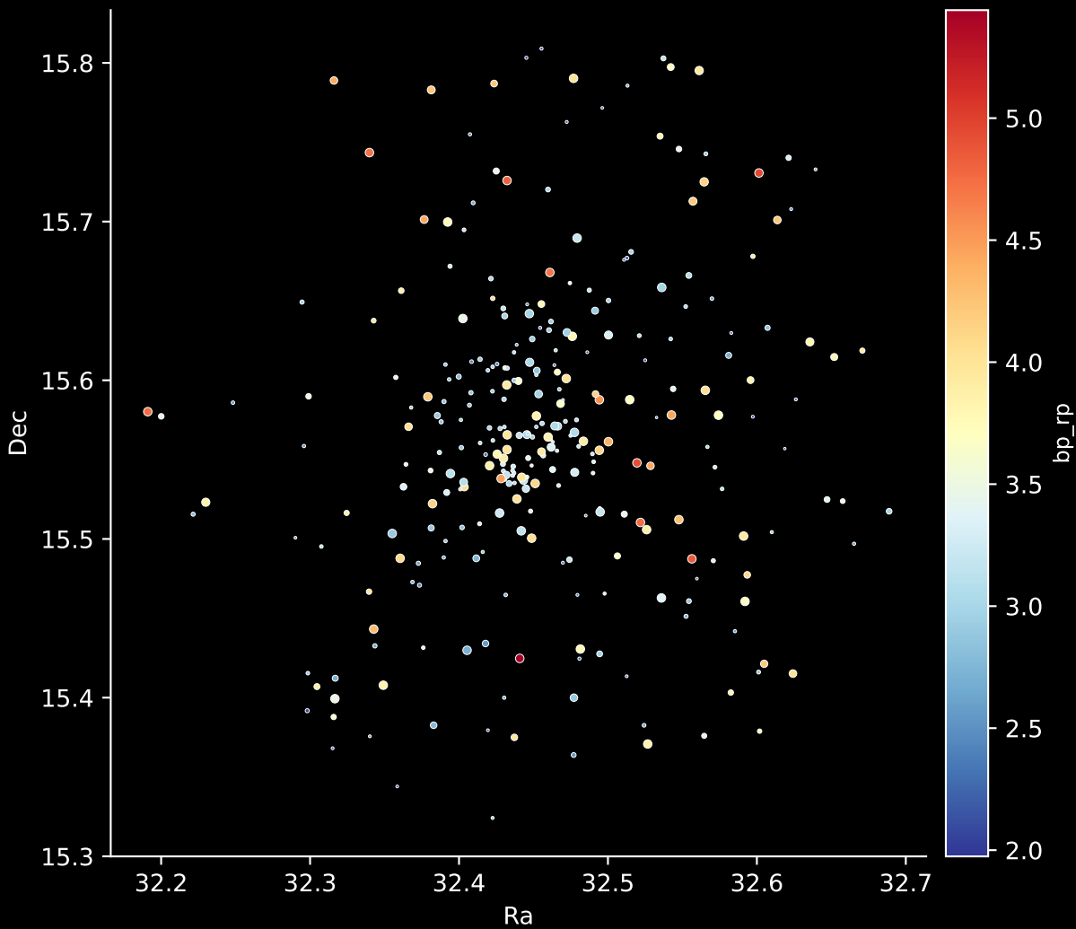
Gaia Cluster: [FSR_0133] Stars: 293
