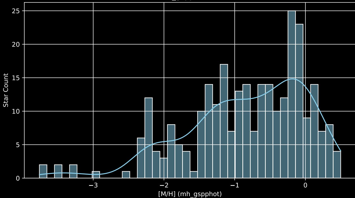
Gaia Cluster: [FSR_0133 [M/H] (mh_gspphot) (n= 284)
