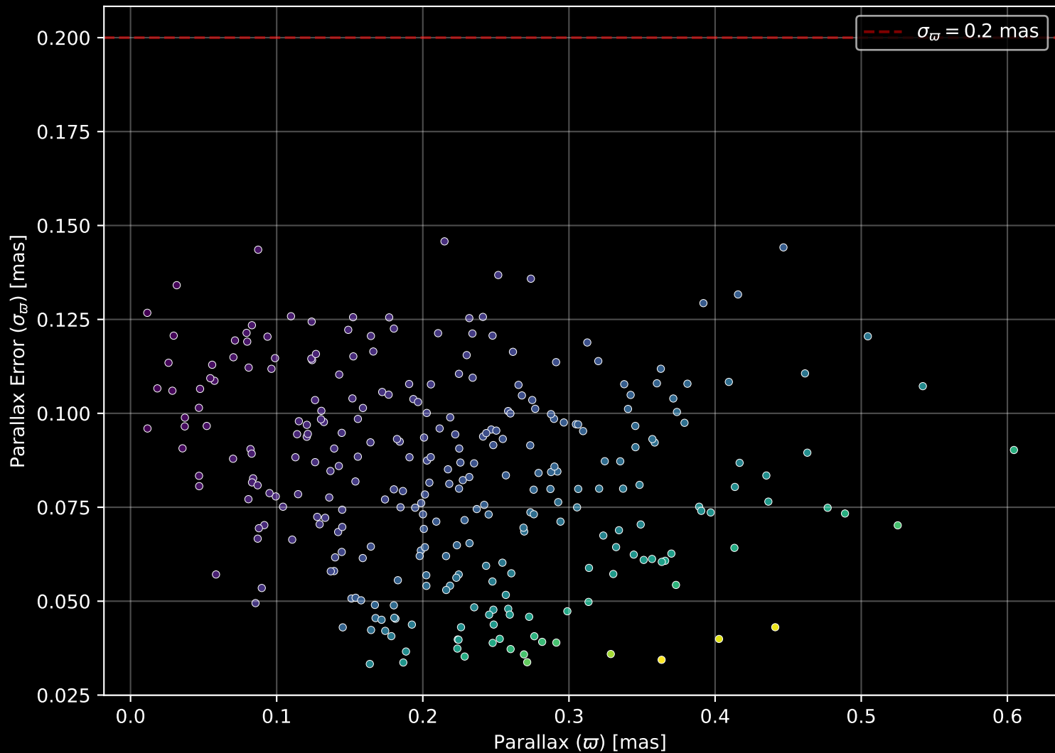
Gaia Cluster: [FSR_0133] Parallax Quality (n= 293)
