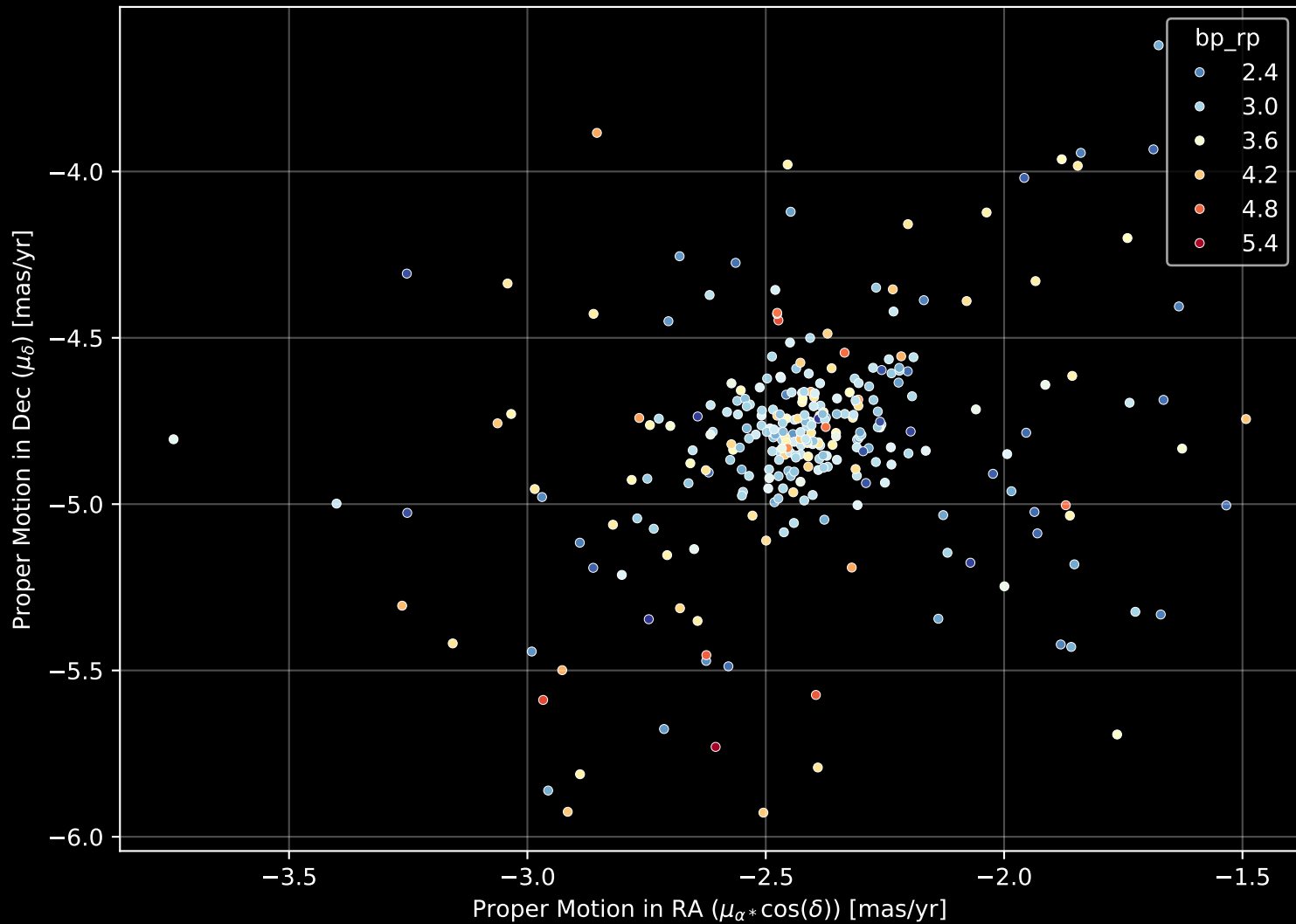
Gaia Cluster: [FSR_0133] Proper Motion Diagram (n= 293)
