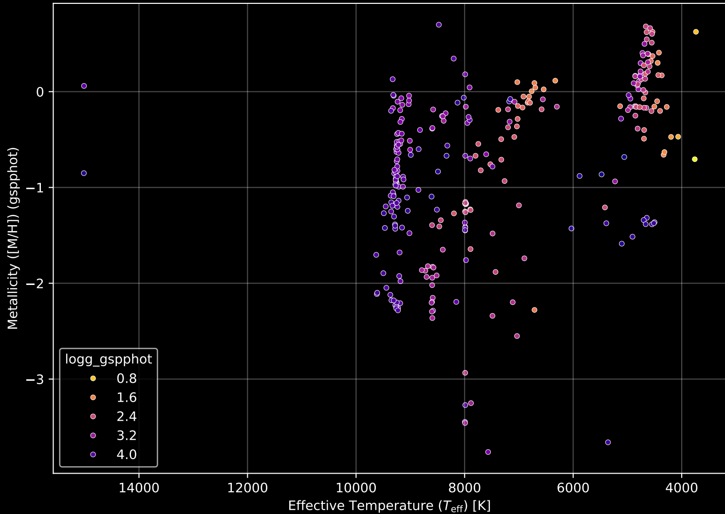
Gaia Cluster: [FSR_0133] Stellar Population Parameters (n= 293)
