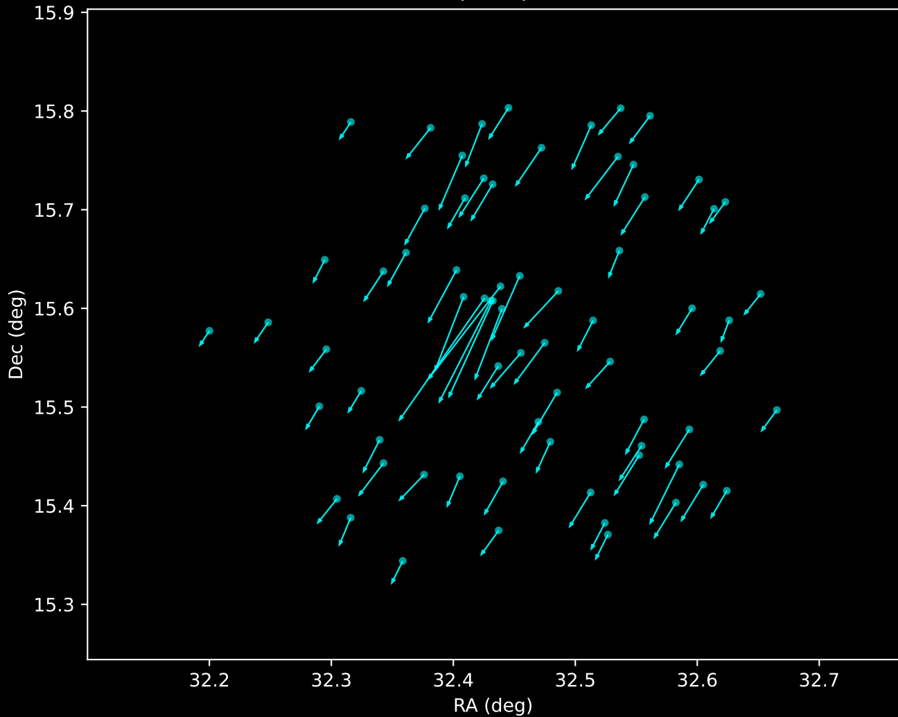
Gaia DR3 Noise Stream Proper Motion Vectors (n=70)
