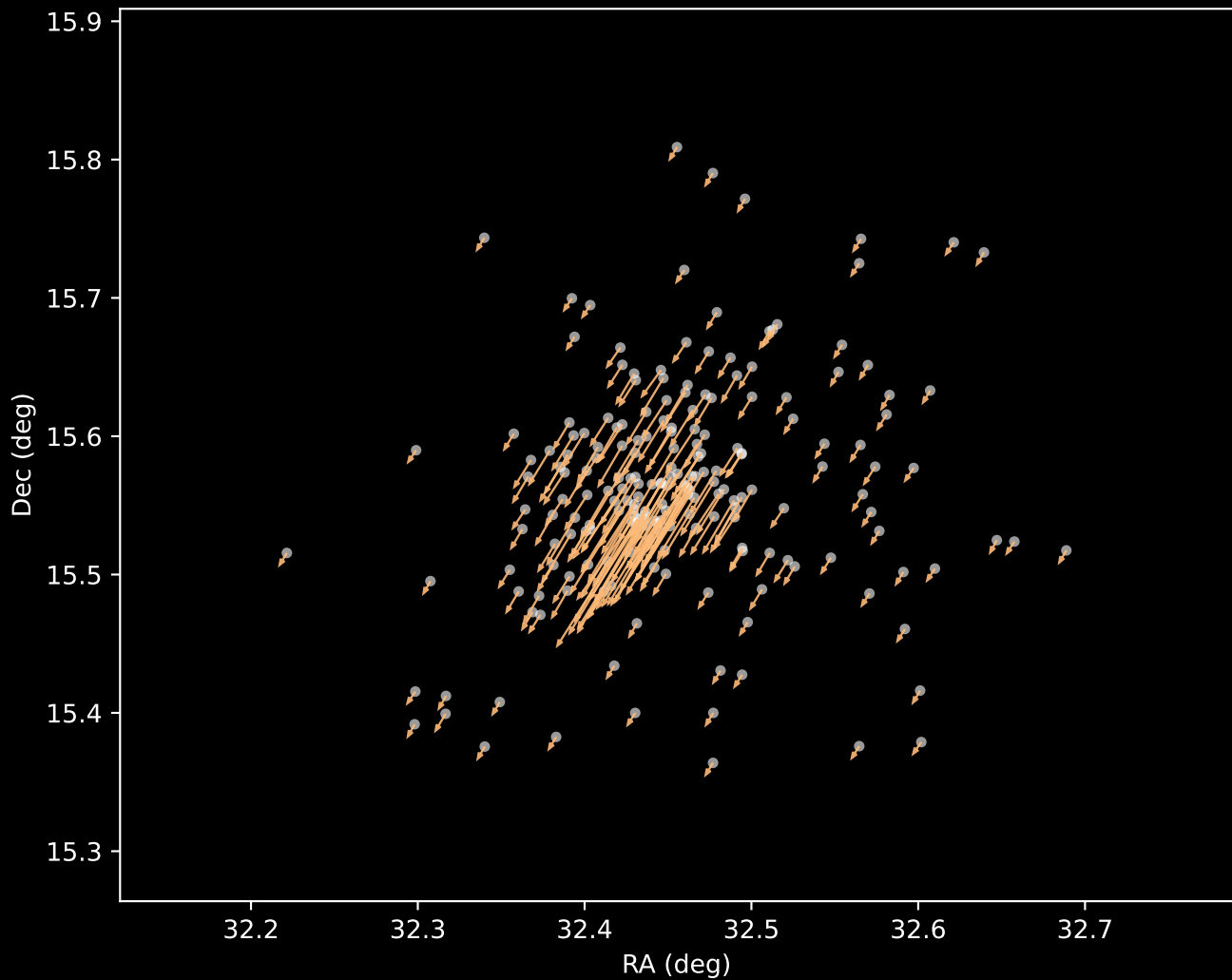
Gaia DR3 Cluster 3 Proper Motion Vectors (n=205)
