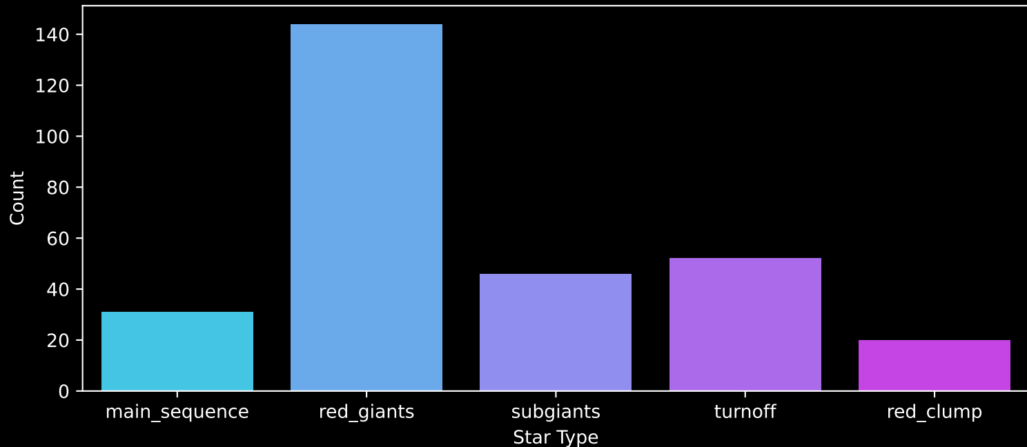
Gaia Cluster: [FSR_0133] Count plot of Star Type
