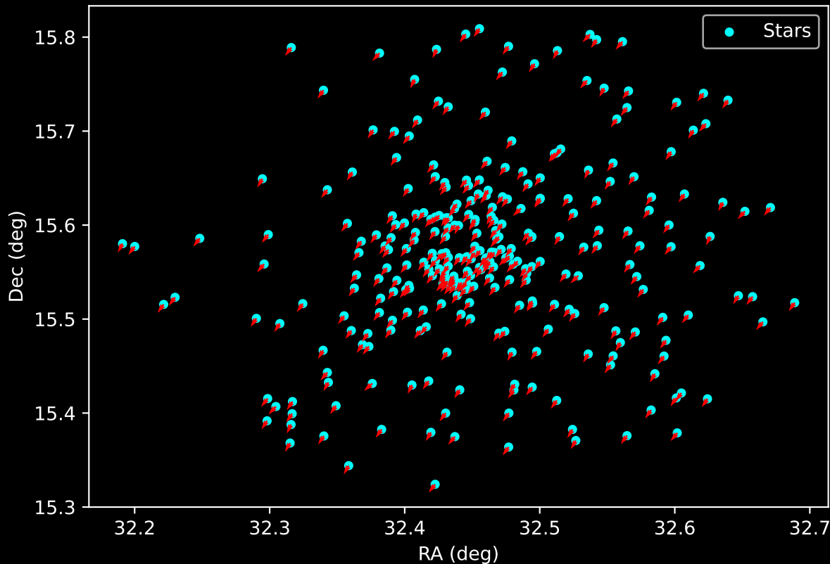
Gaia Cluster: [FSR_0133] Proper Motion Vectors for Gaia Star Field (n= 293)
