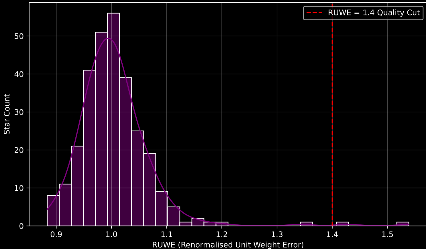
Gaia Cluster: [FSR_0133] RUWE Distribution (n= 293)
