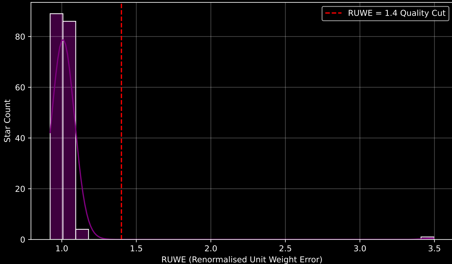
Gaia Cluster: [FSR_0166] RUWE Distribution (n= 180)
