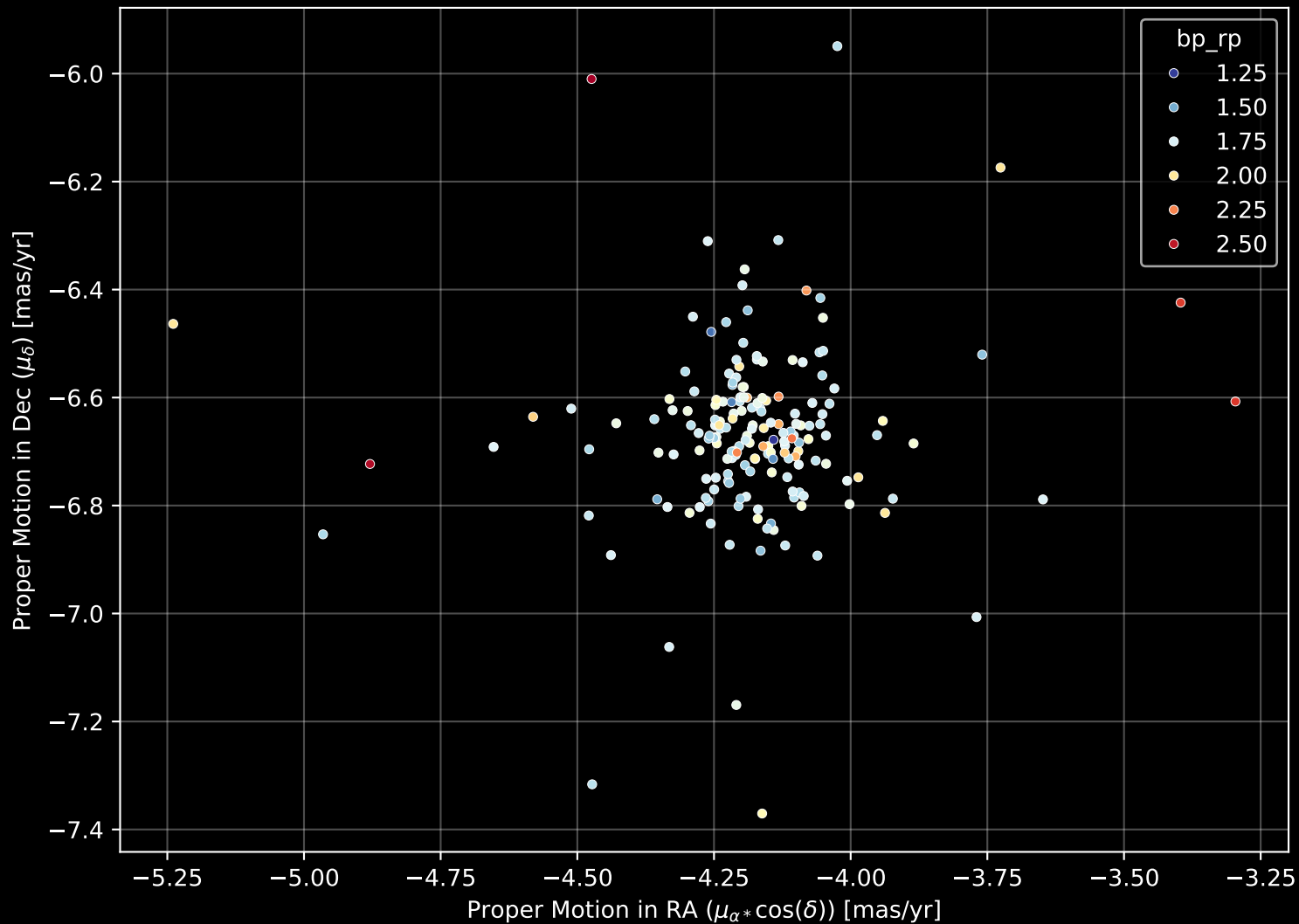
Gaia Cluster: [FSR_0166] Proper Motion Diagram (n= 180)
