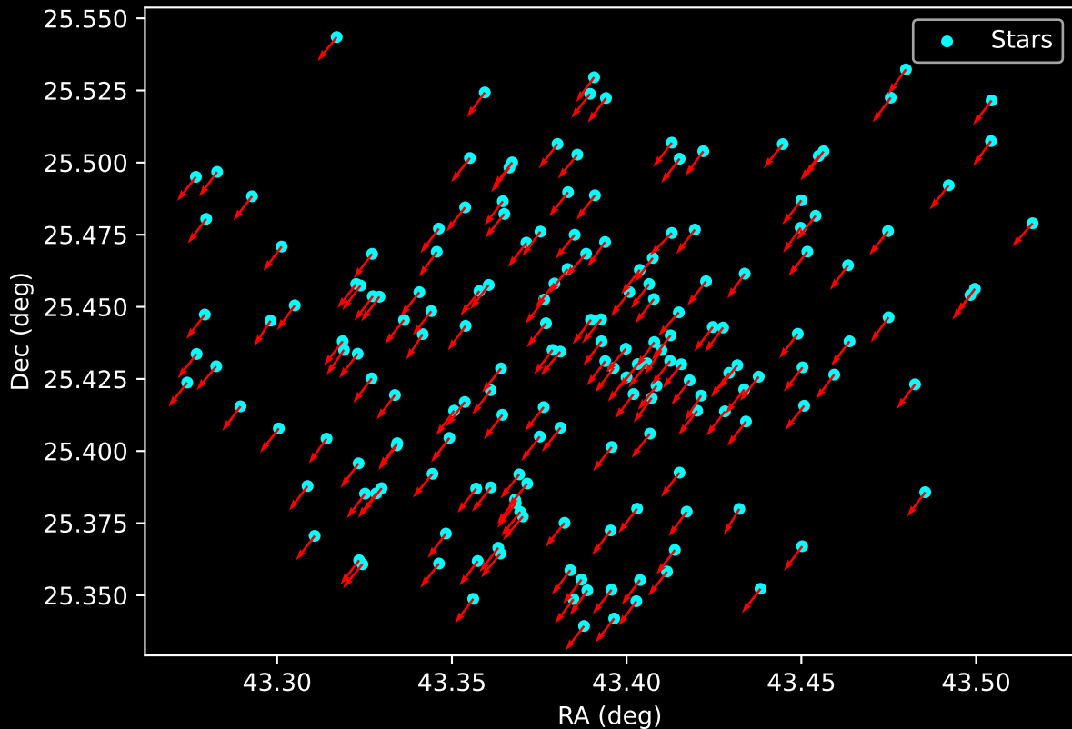
Gaia Cluster: [FSR_0166] Proper Motion Vectors for Gaia Star Field (n= 180)
