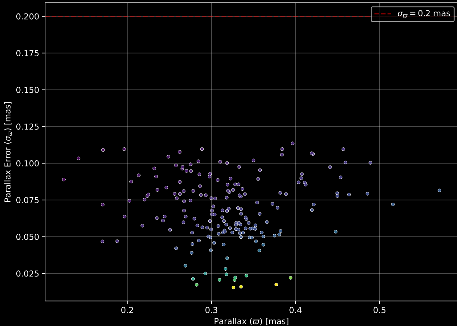
Gaia Cluster: [FSR_0166] Parallax Quality (n= 180)
