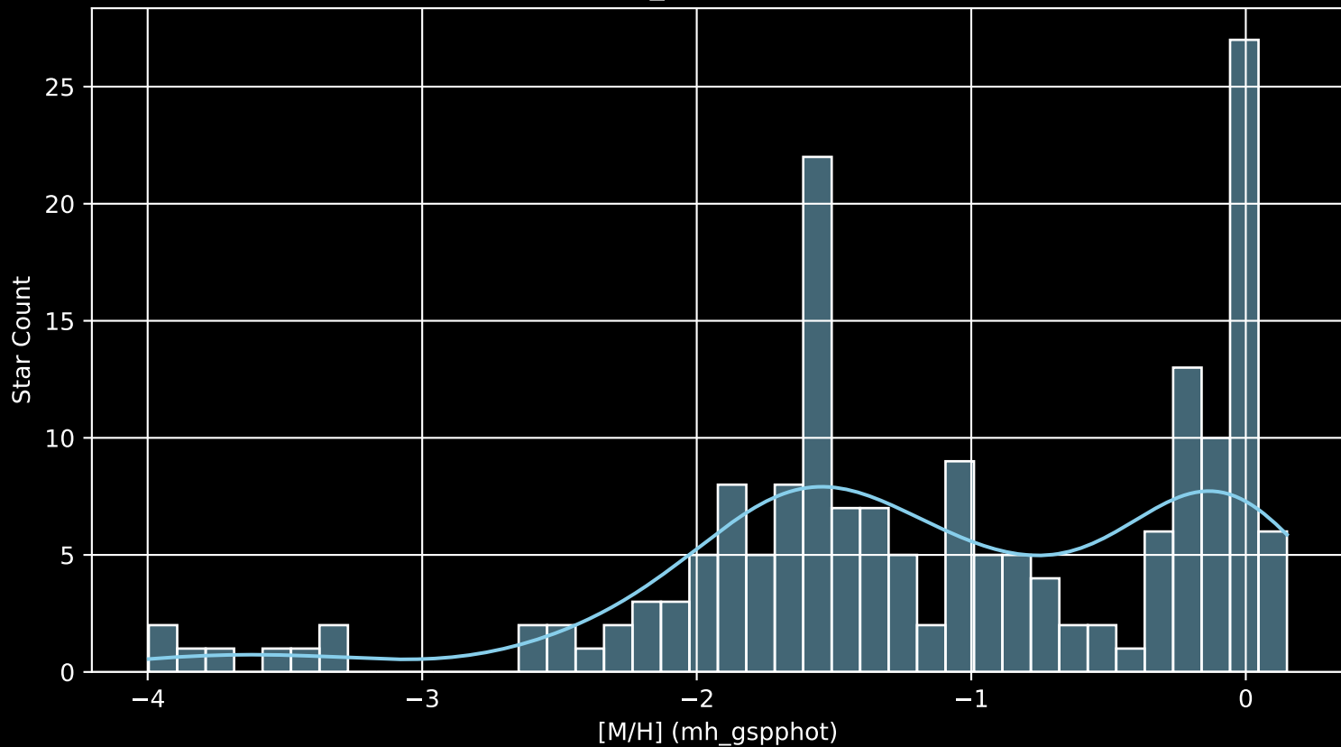
Gaia Cluster: [FSR_0166 [M/H] (mh_gspphot) (n= 180)
