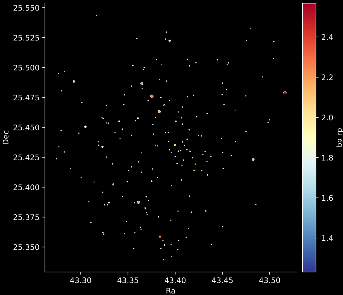
Gaia Cluster: [FSR_0166] Stars: 180
