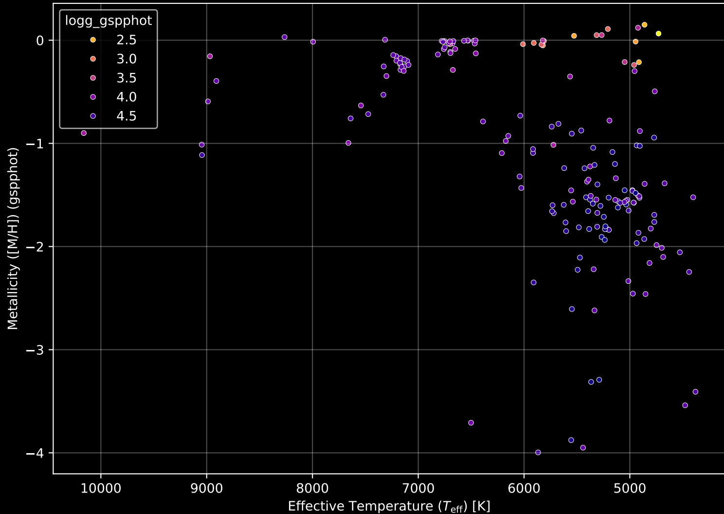
Gaia Cluster: [FSR_0166] Stellar Population Parameters (n= 180)
