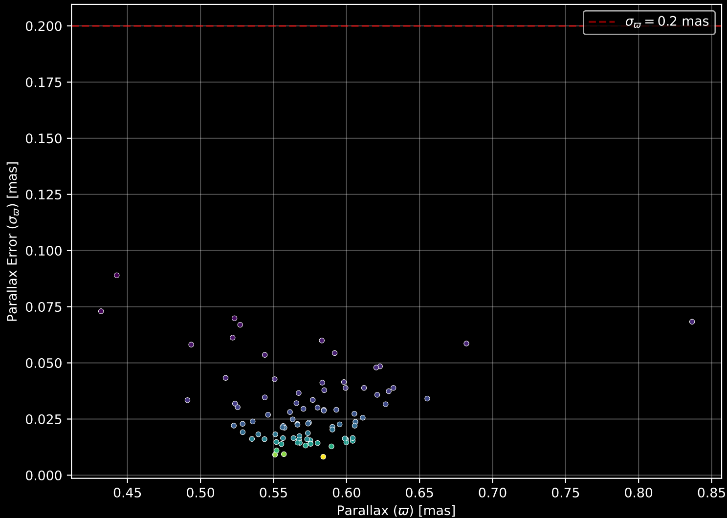
Gaia Cluster: [FSR_0278] Parallax Quality (n= 87)
