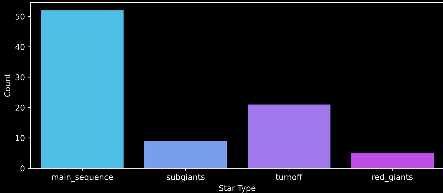
Gaia Cluster: [FSR_0278] Count plot of Star Type
