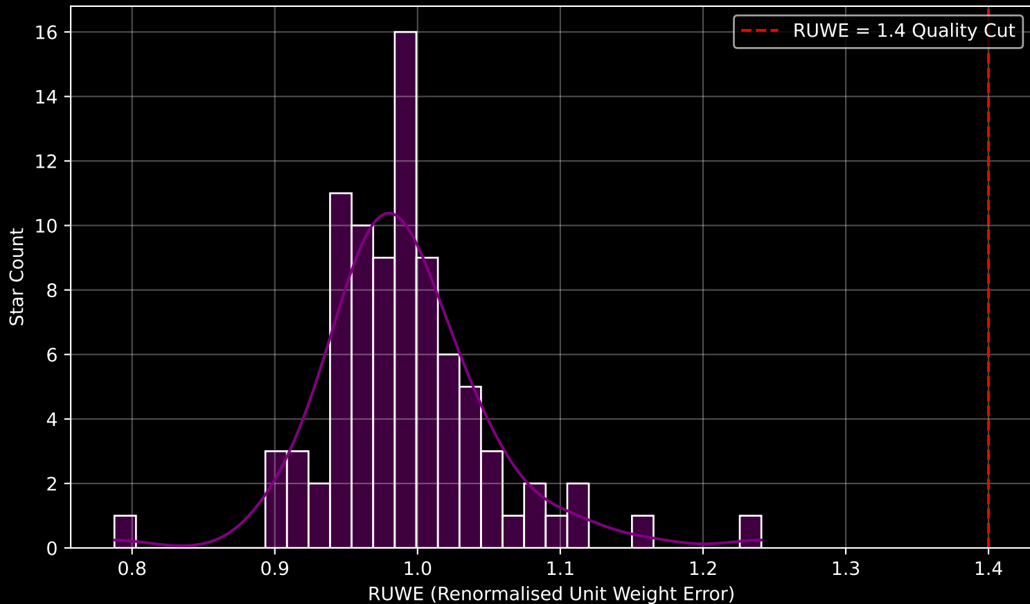
Gaia Cluster: [FSR_0278] RUWE Distribution (n= 86)
