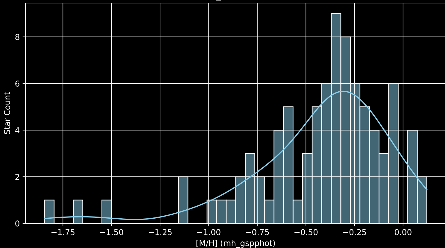
Gaia Cluster: [FSR_0278 [M/H] (mh_gspphot) (n= 87)
