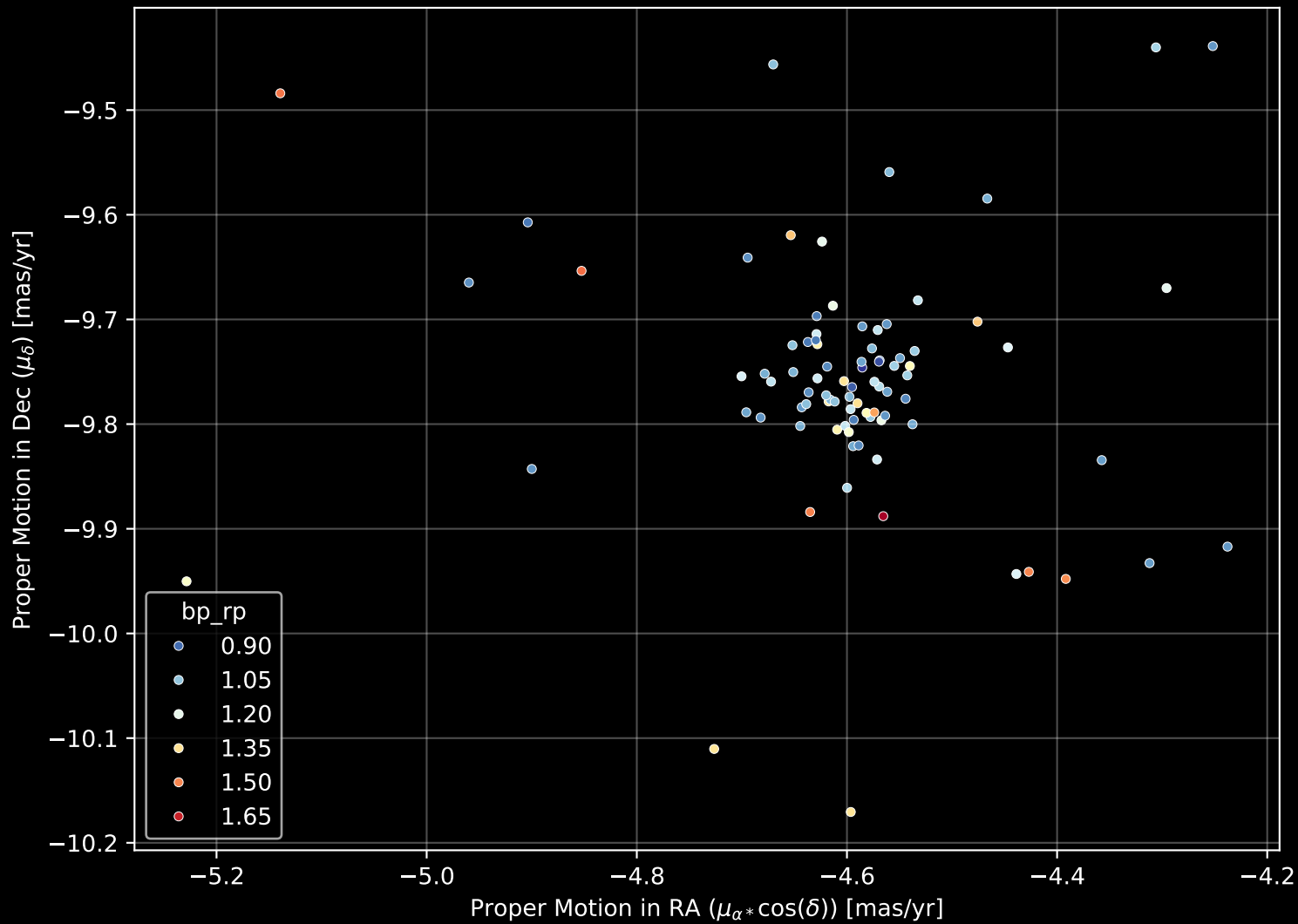
Gaia Cluster: [FSR_0278] Proper Motion Diagram (n= 87)
