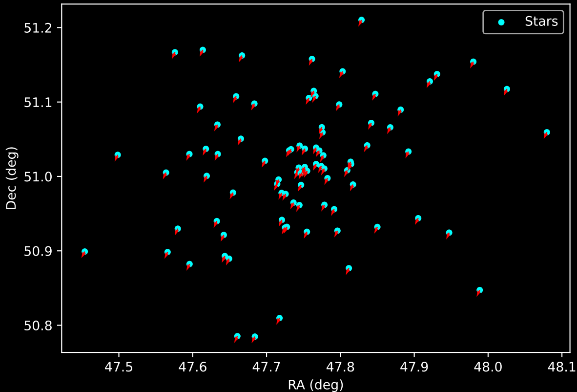
Gaia Cluster: [FSR_0278] Proper Motion Vectors for Gaia Star Field (n= 87)
