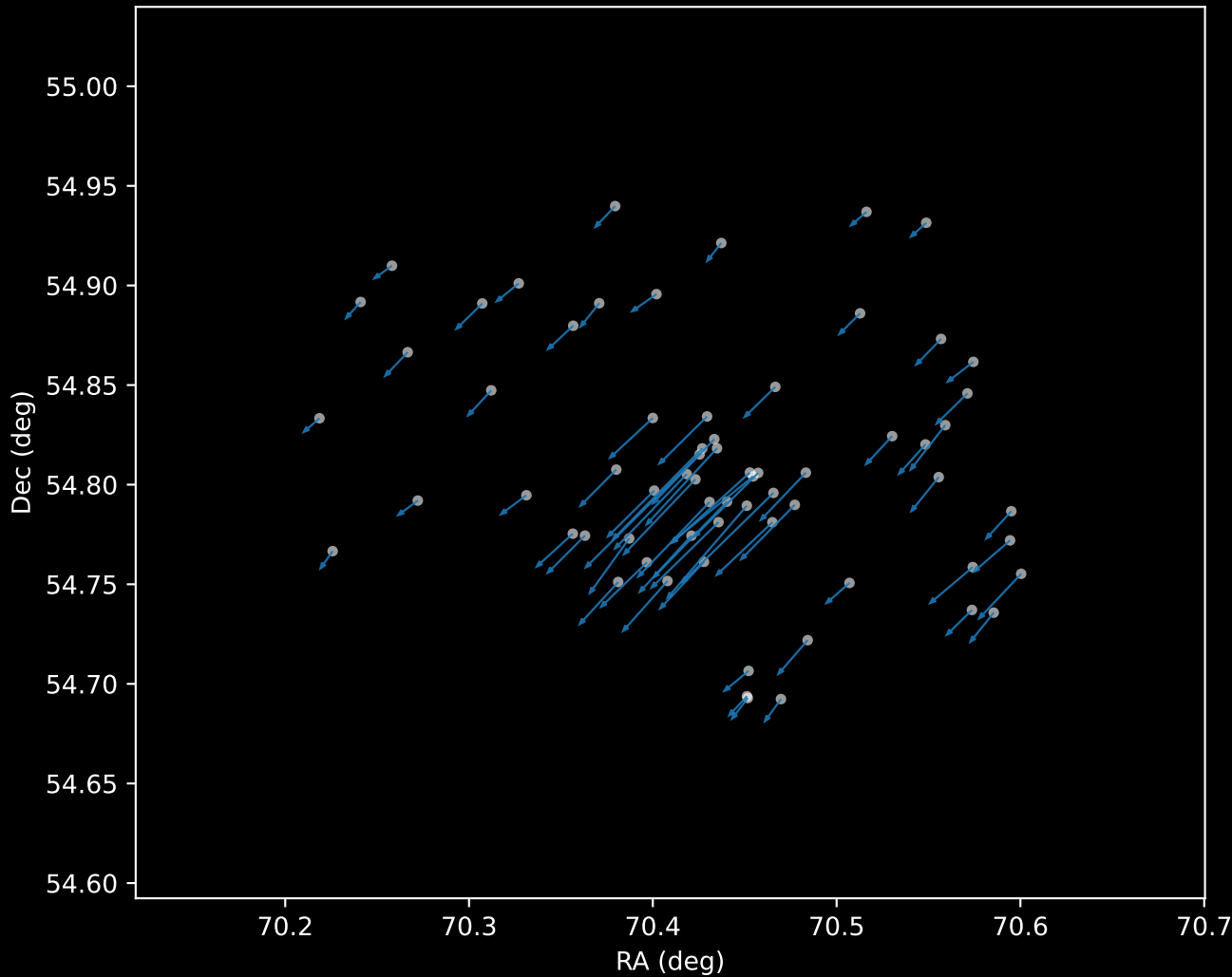
Gaia DR3 Cluster 0 Proper Motion Vectors (n=67)
