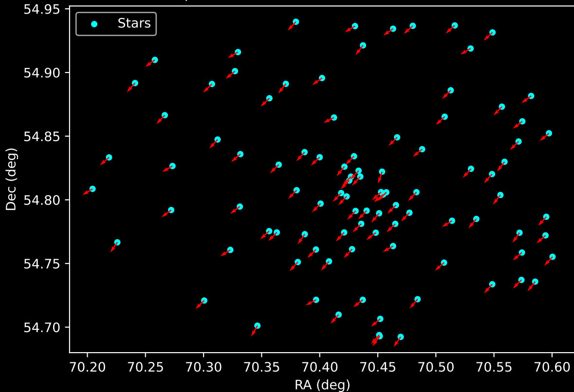
Gaia Cluster: [FSR_0344] Proper Motion Vectors for Gaia Star Field (n= 96)
