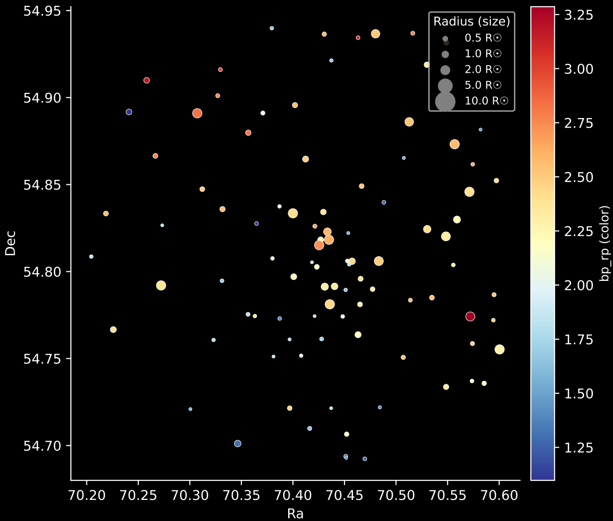
Gaia Cluster: [FSR_0344] Stars: 96
