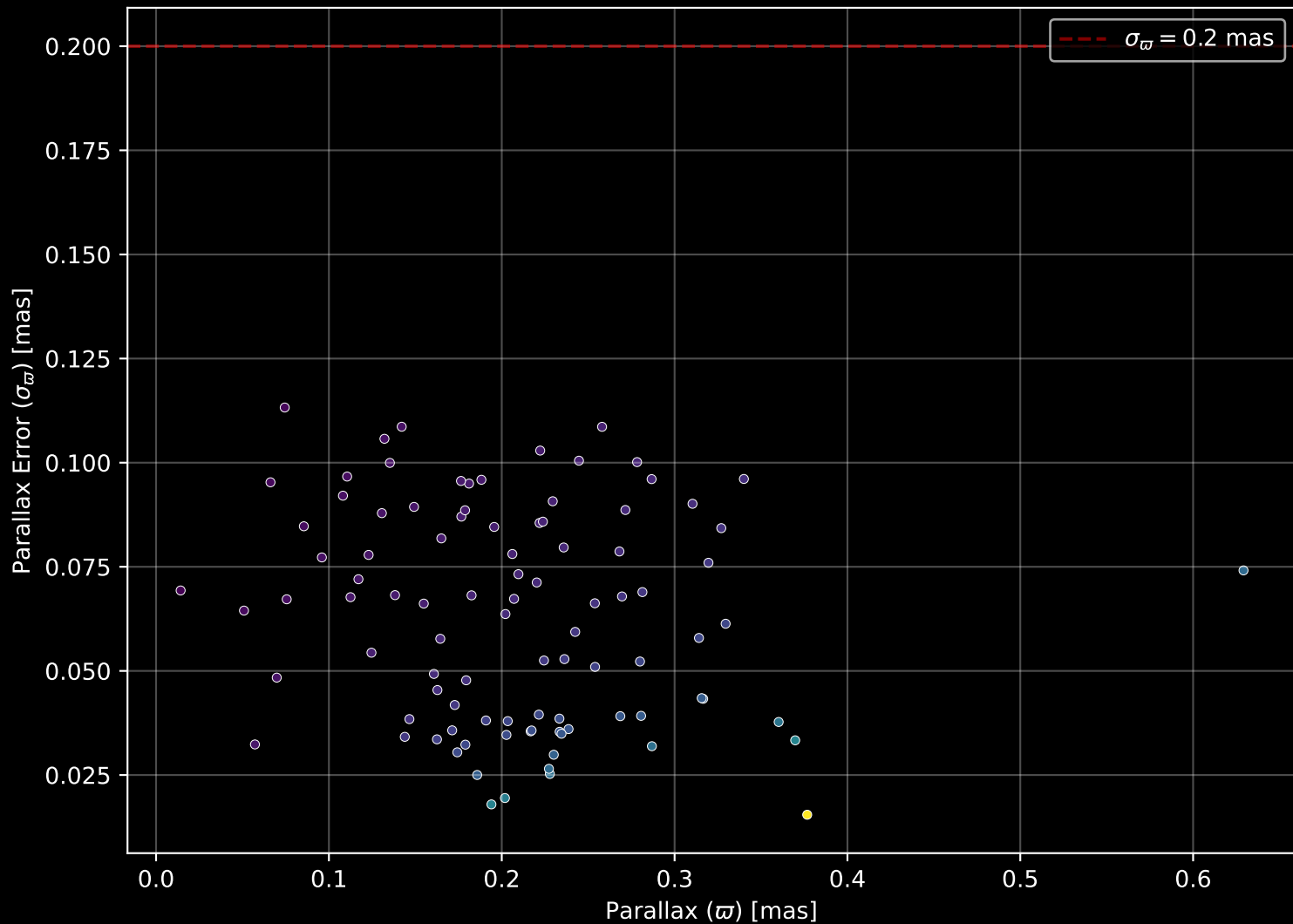
Gaia Cluster: [FSR_0344] Parallax Quality (n= 96)
