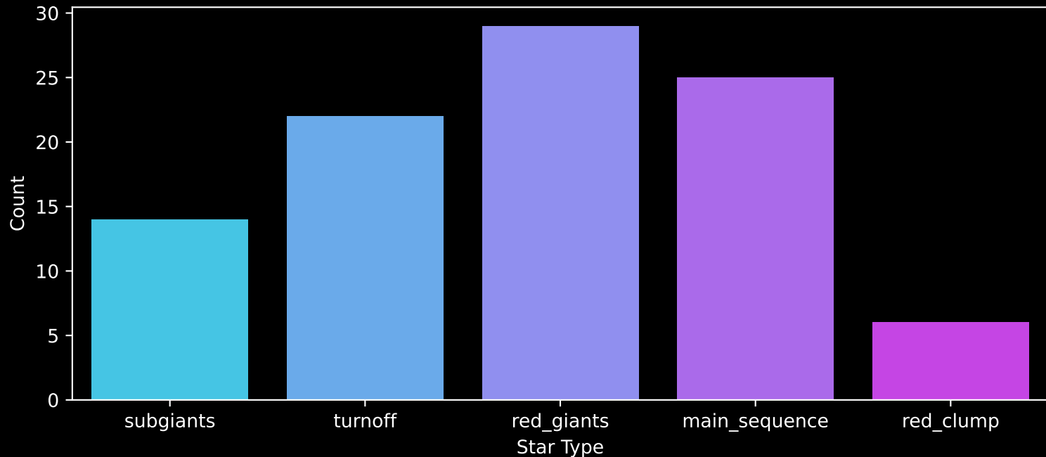
Gaia Cluster: [FSR_0344] Count plot of Star Type
