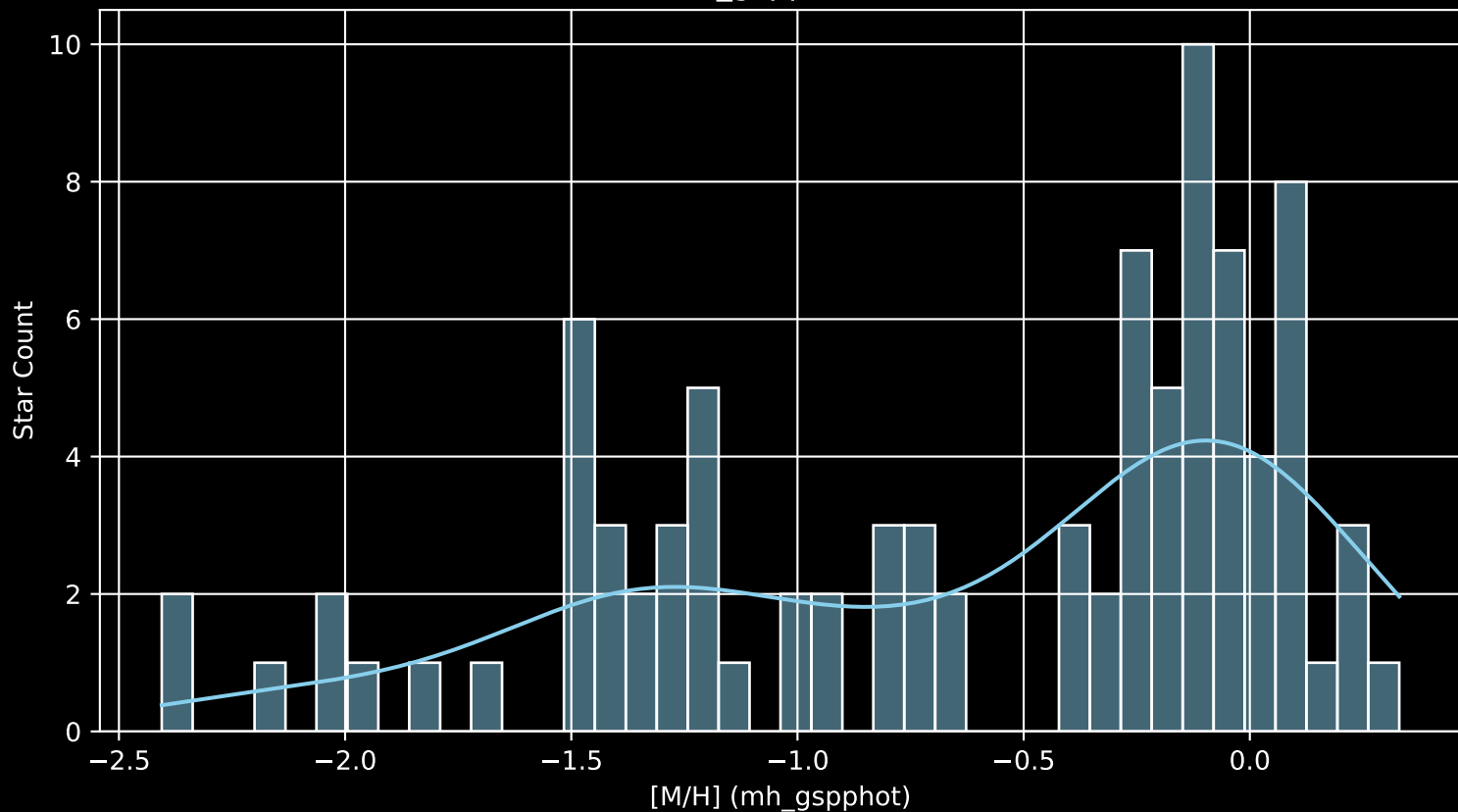
Gaia Cluster: [FSR_0344 [M/H] (mh_gspphot) (n= 91)
