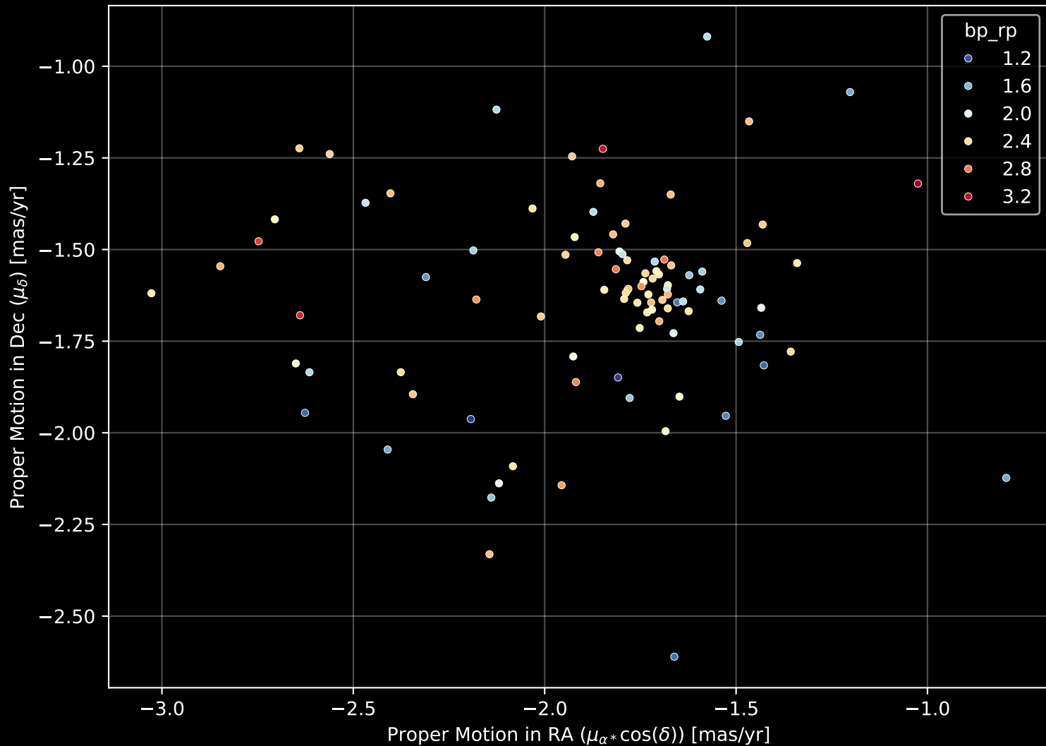
Gaia Cluster: [FSR_0344] Proper Motion Diagram (n= 96)
