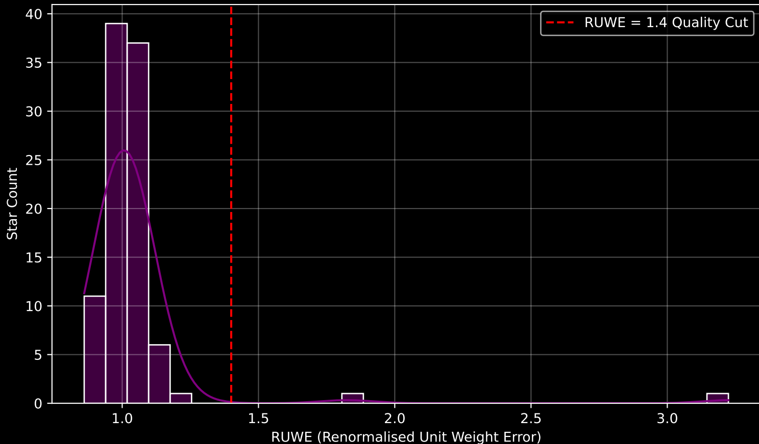
Gaia Cluster: [FSR_0344] RUWE Distribution (n= 96)
