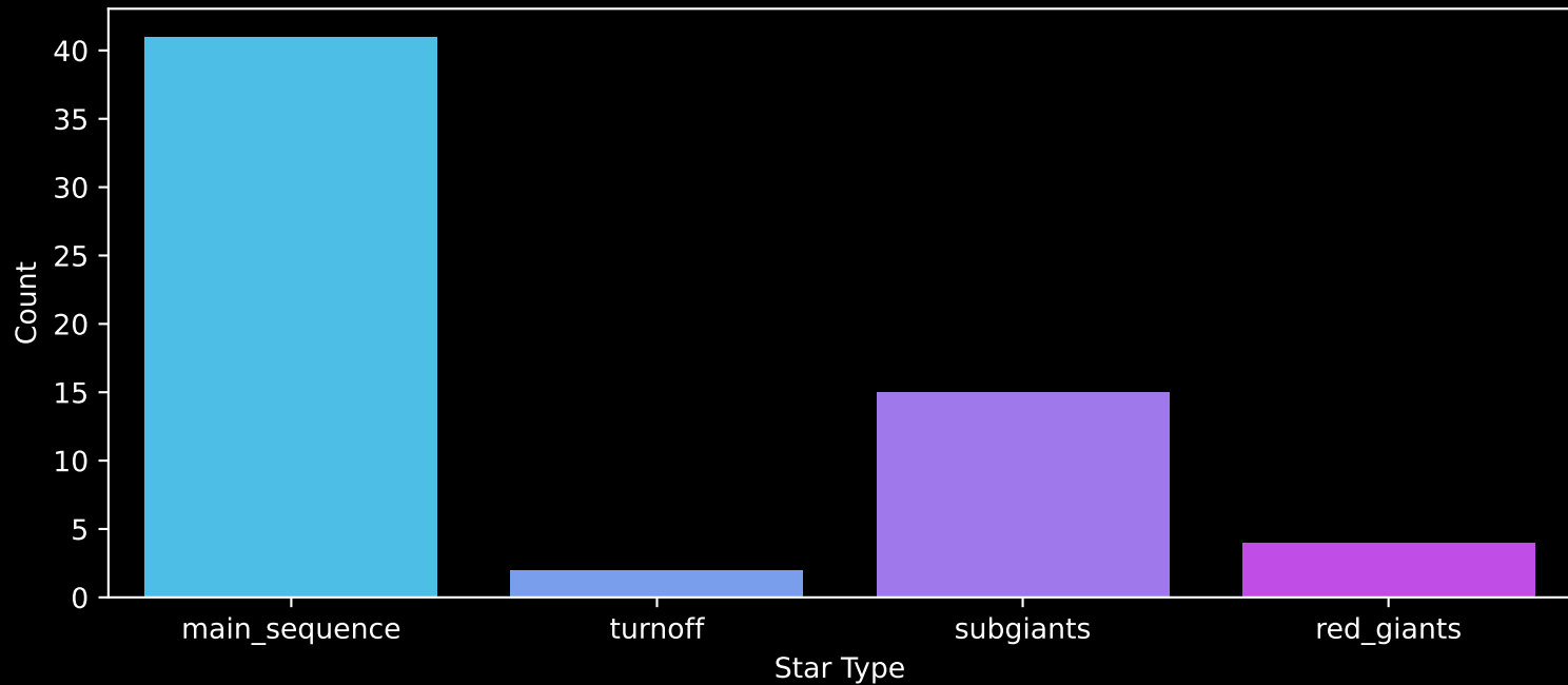
Gaia Cluster: [FSR_0357] Count plot of Star Type
