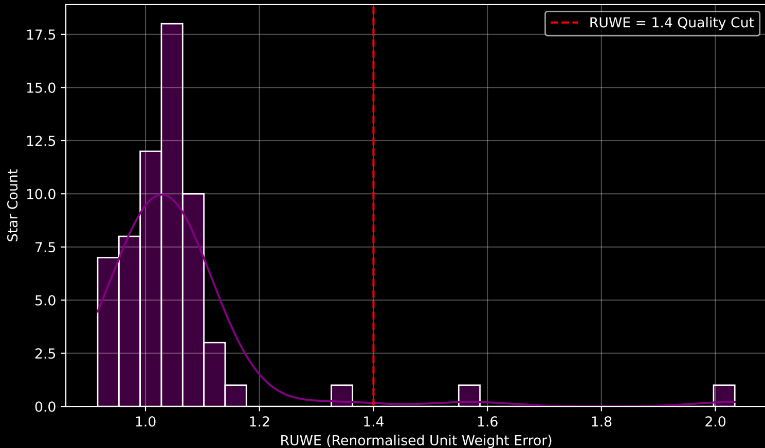
Gaia Cluster: [FSR_0357] RUWE Distribution (n= 62)
