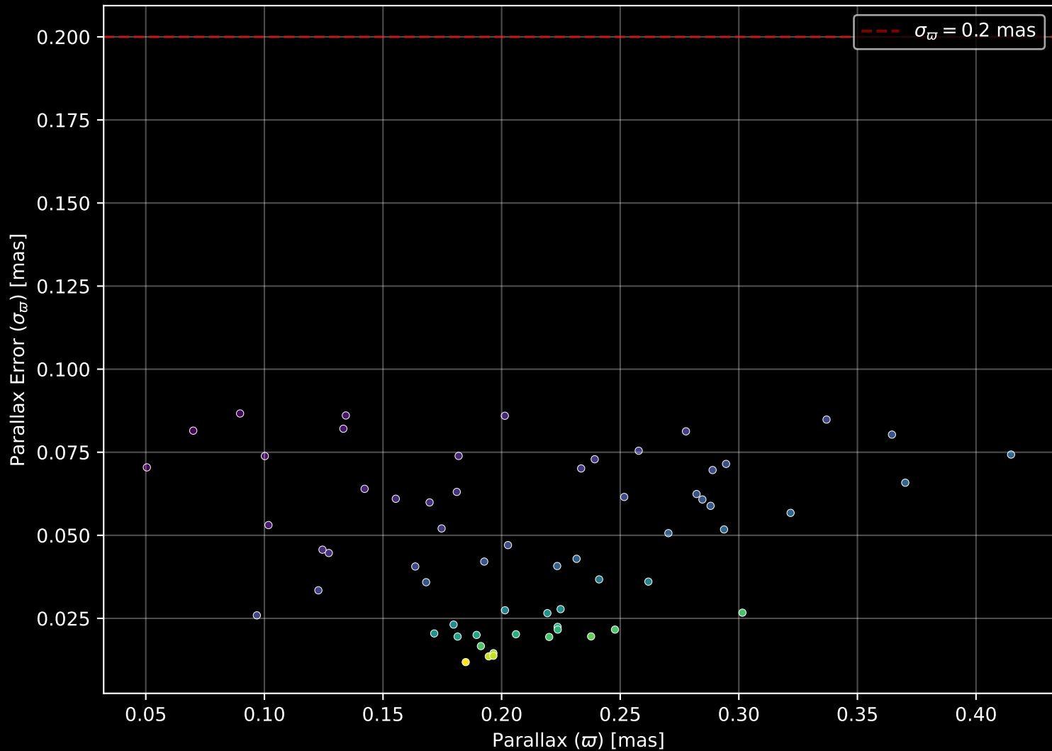
Gaia Cluster: [FSR_0357] Parallax Quality (n= 62)
