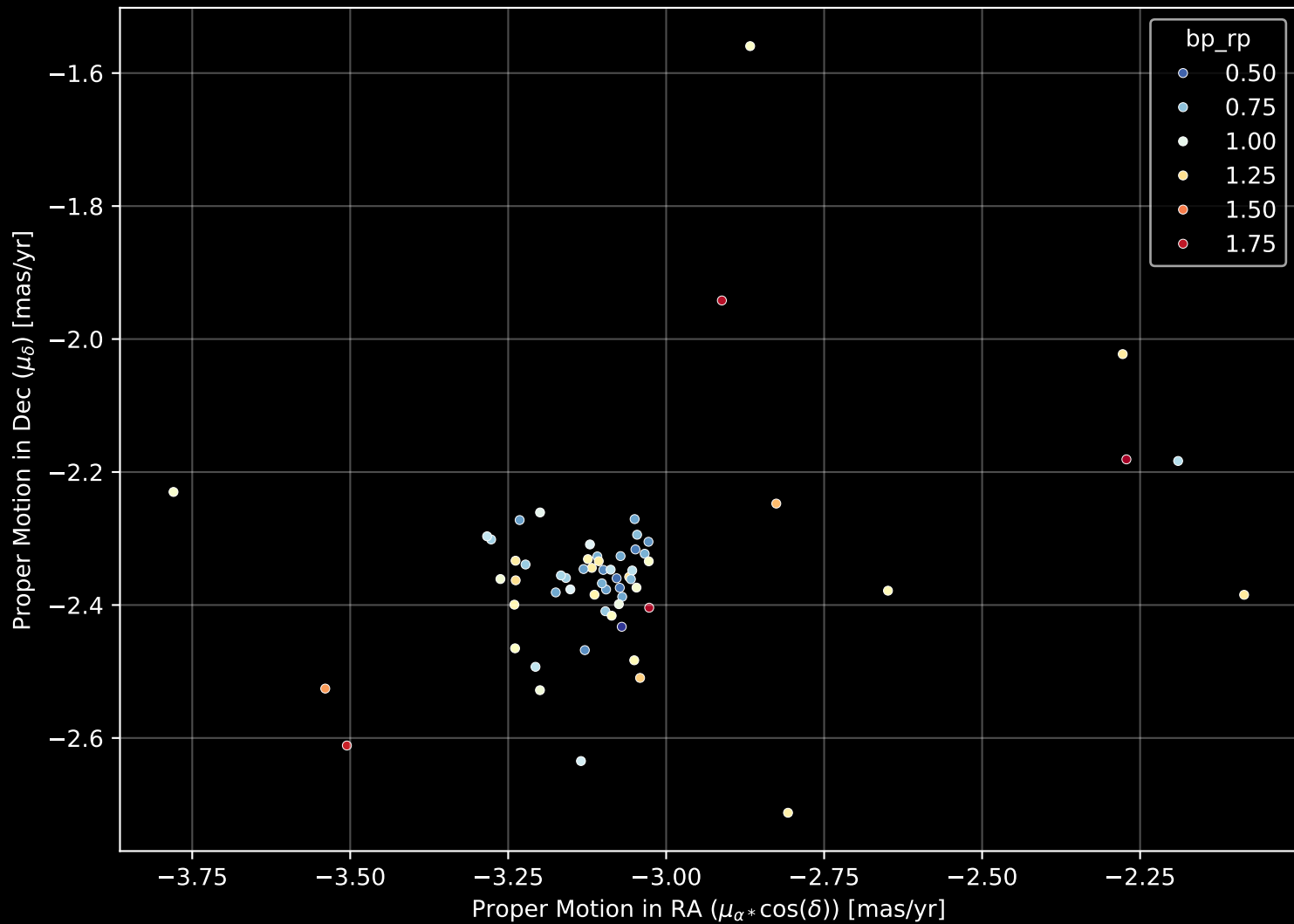
Gaia Cluster: [FSR_0357] Proper Motion Diagram (n= 62)
