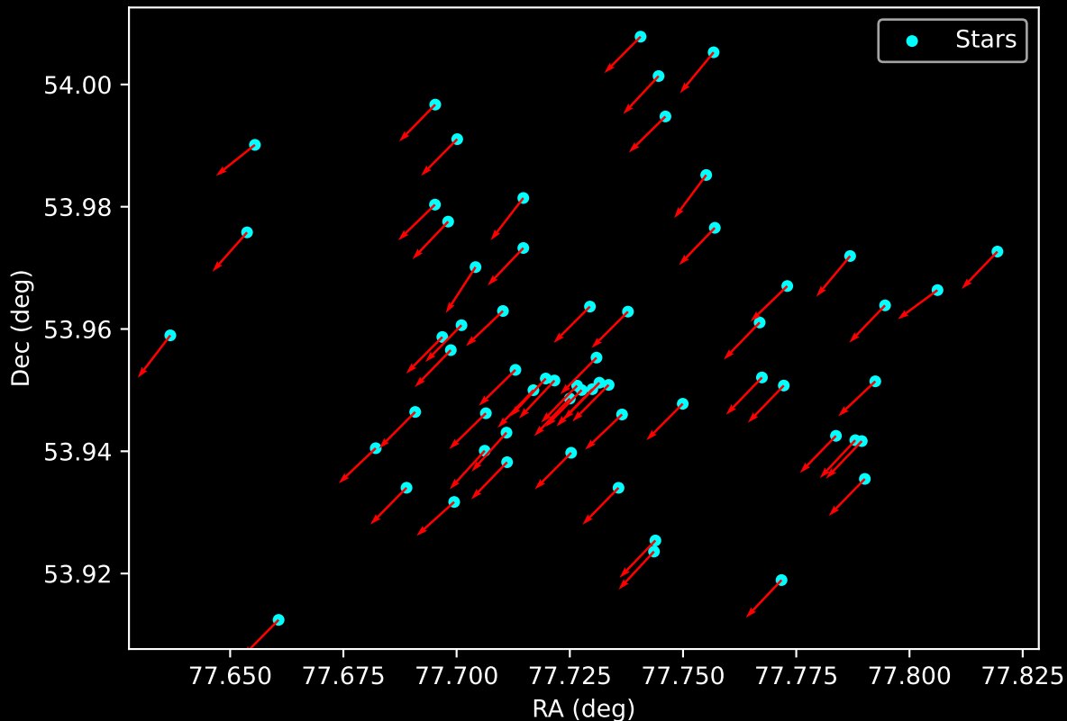
Gaia Cluster: [FSR_0357] Proper Motion Vectors for Gaia Star Field (n= 62)
