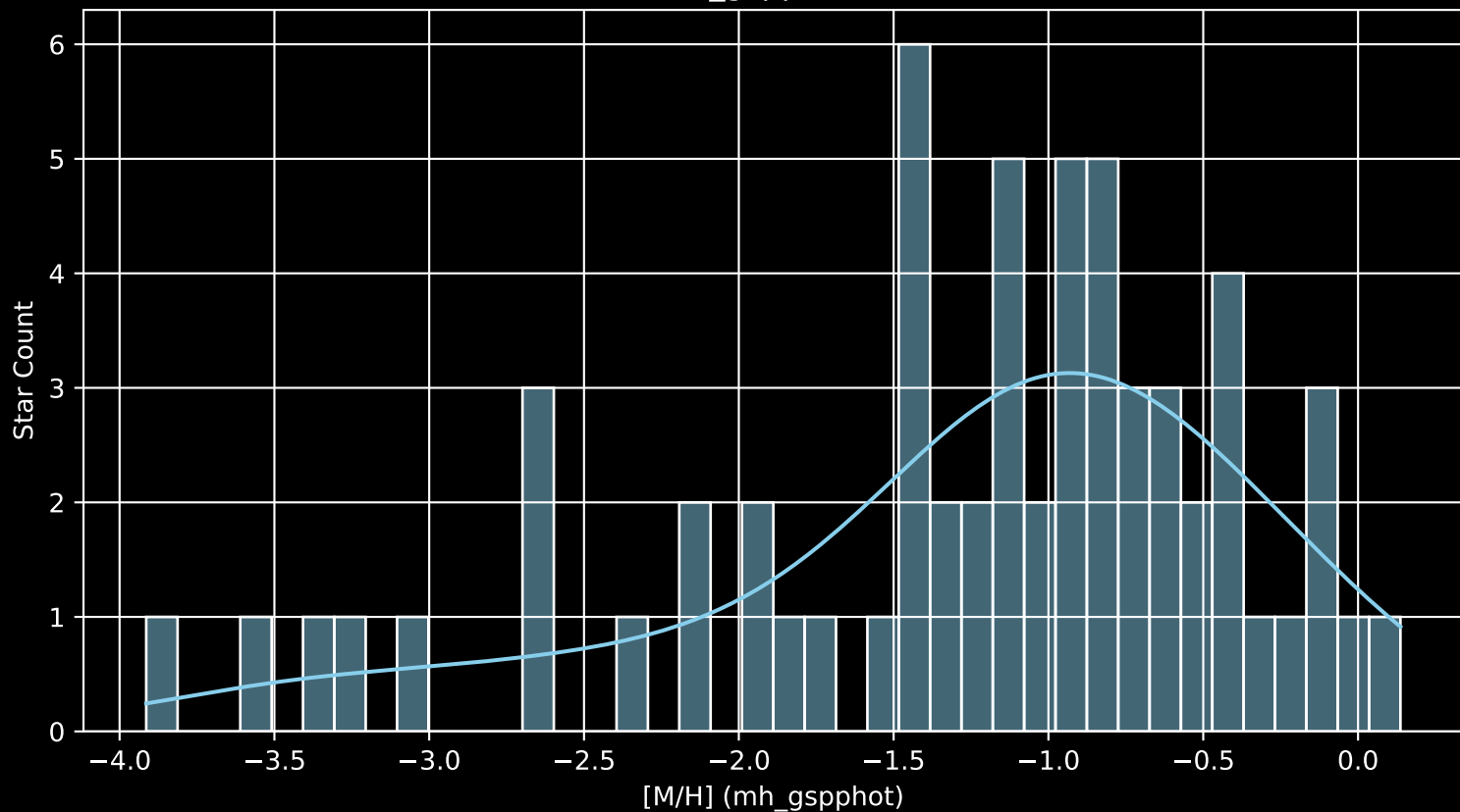
Gaia Cluster: [FSR_0357 [M/H] (mh_gspphot) (n= 62)
