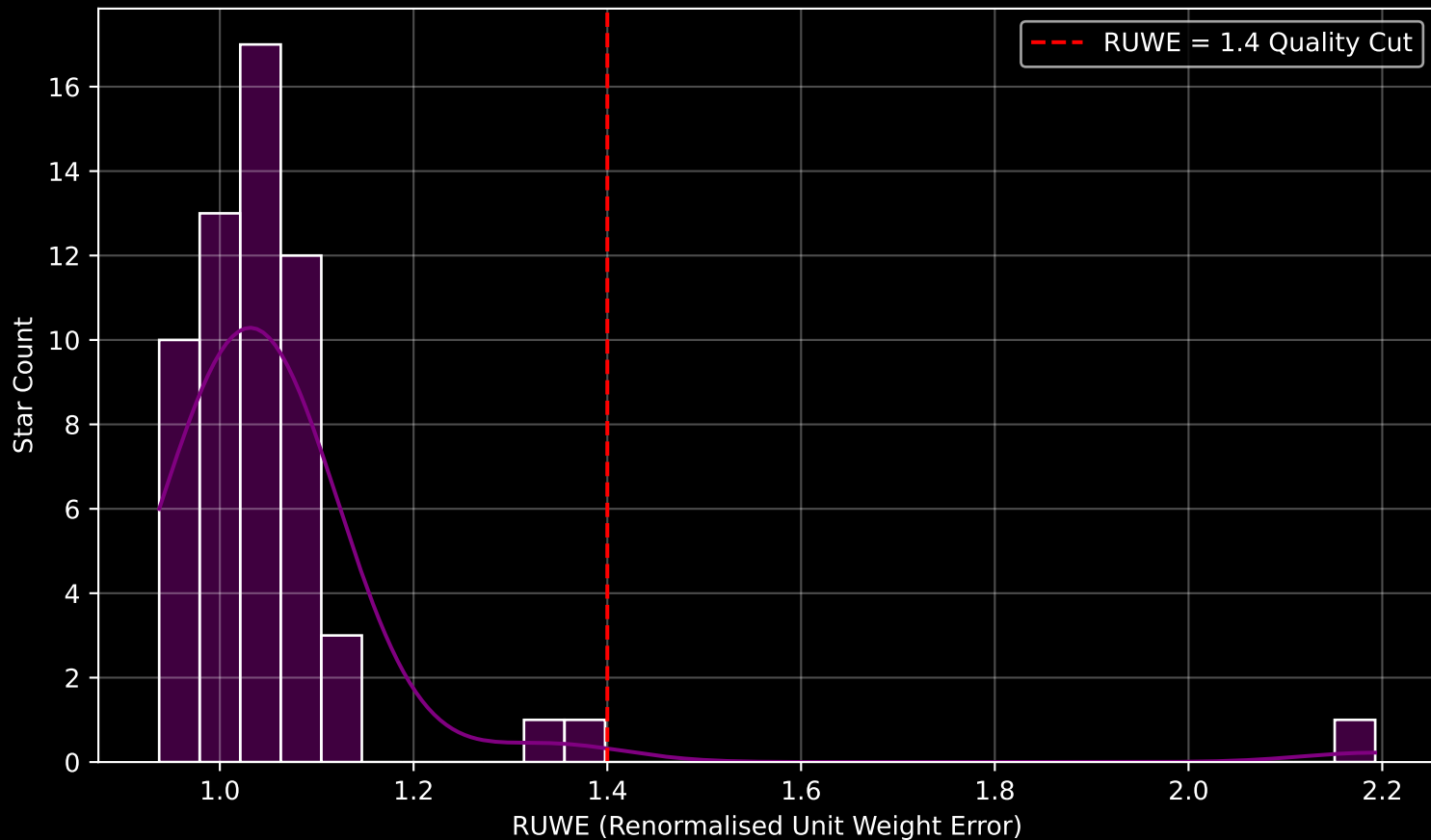
Gaia Cluster: [FSR_0384] RUWE Distribution (n= 58)
