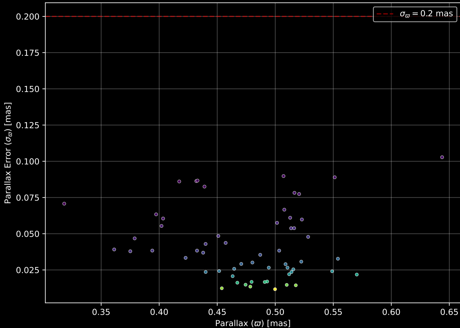
Gaia Cluster: [FSR_0384] Parallax Quality (n= 58)
