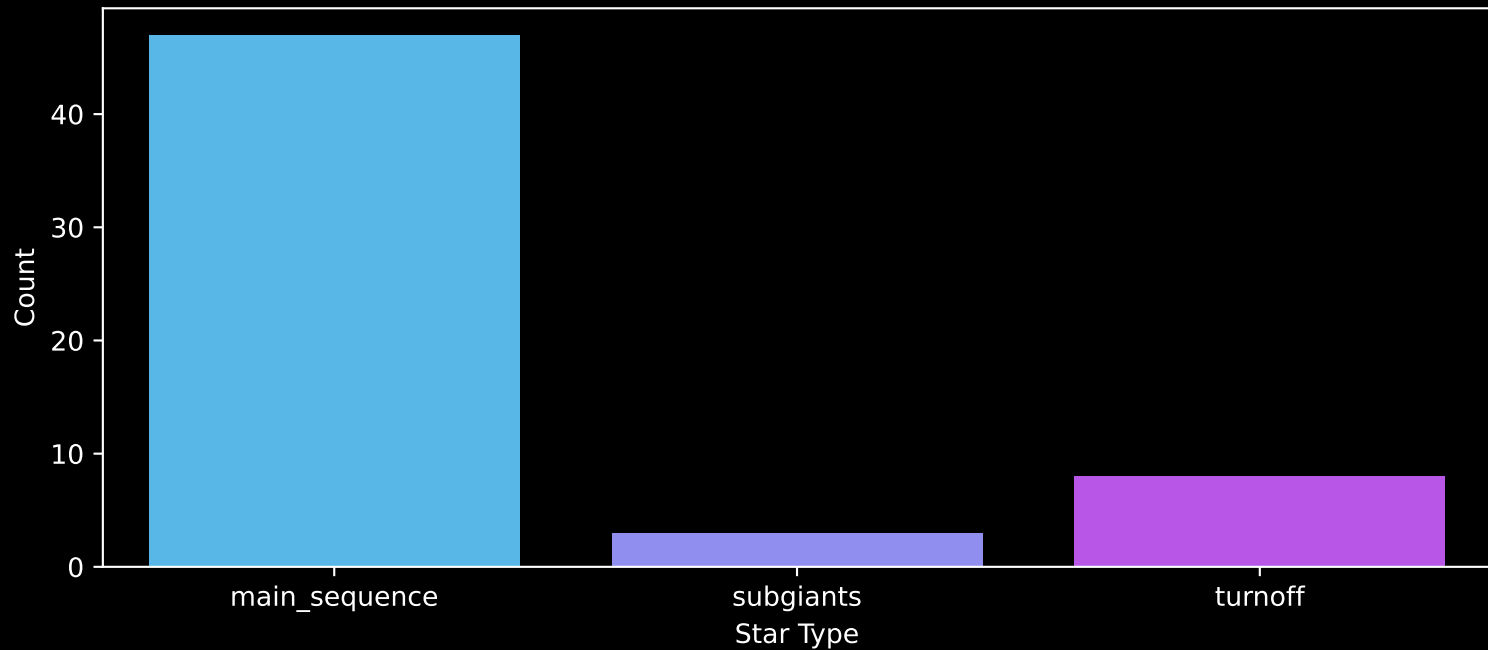
Gaia Cluster: [FSR_0384] Count plot of Star Type
