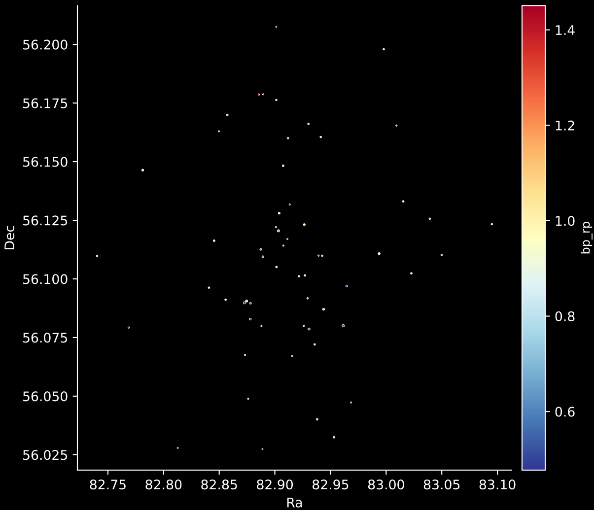
Gaia Cluster: [FSR_0384] Stars: 58
