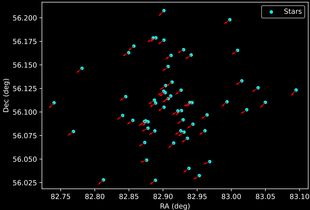
Gaia Cluster: [FSR_0384] Proper Motion Vectors for Gaia Star Field (n= 58)
