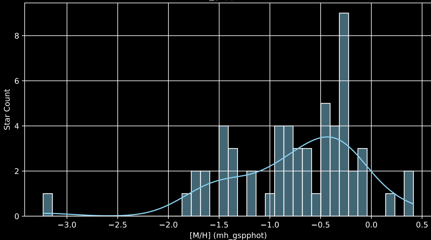
Gaia Cluster: [FSR_0384 [M/H] (mh_gspphot) (n= 57)
