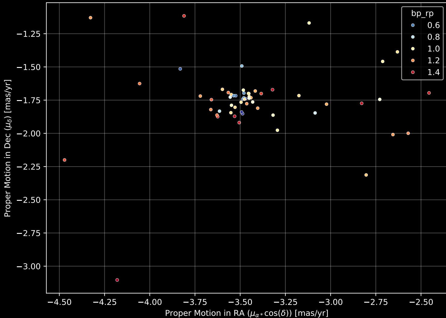
Gaia Cluster: [FSR_0384] Proper Motion Diagram (n= 58)
