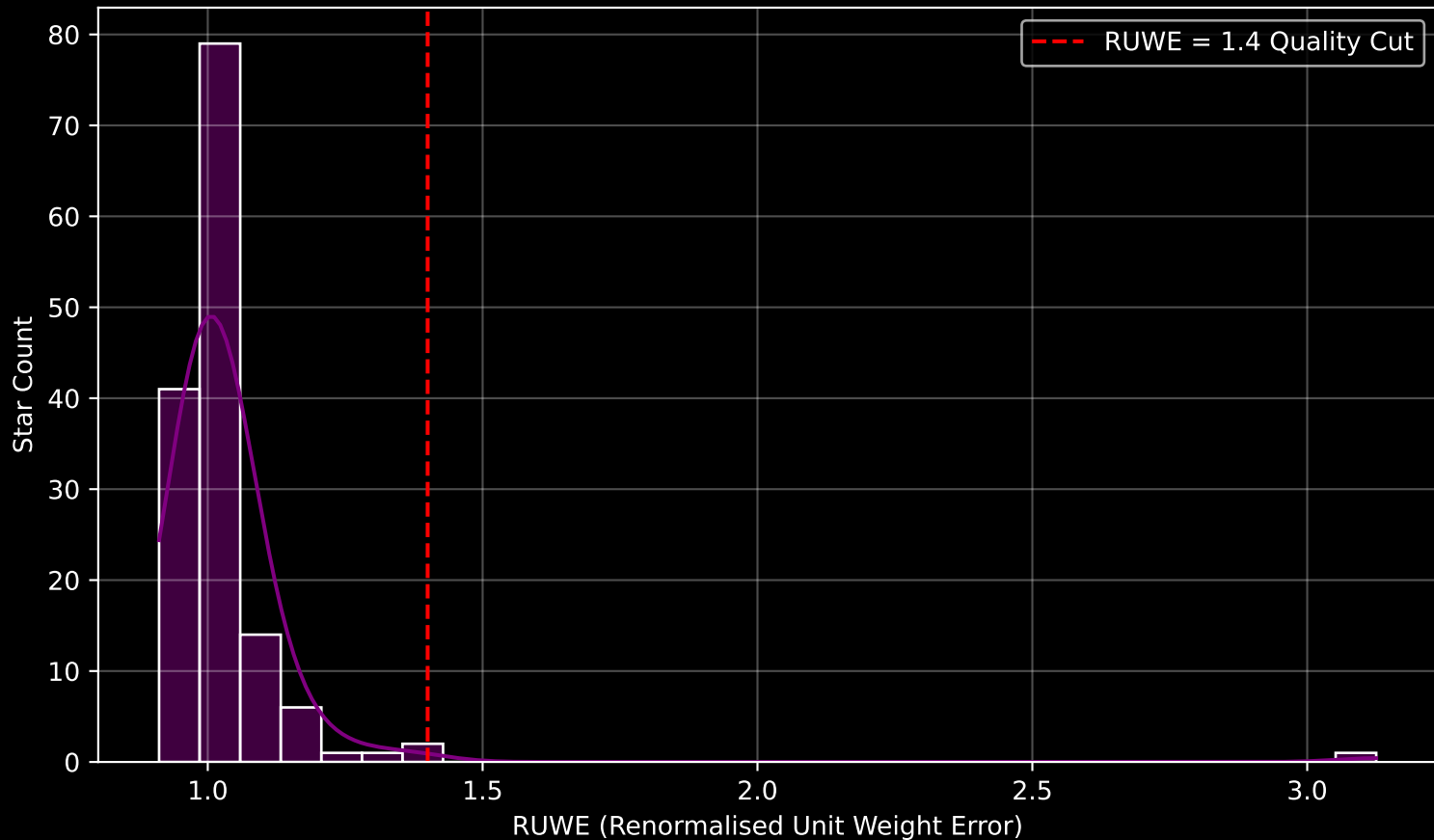
Gaia Cluster: [FSR_0442] RUWE Distribution (n= 145)
