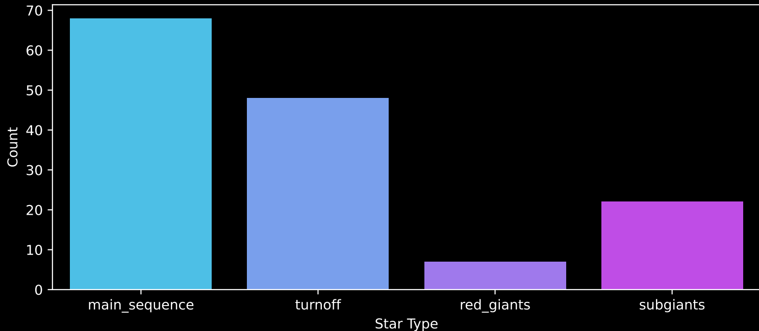
Gaia Cluster: [FSR_0442] Count plot of Star Type
