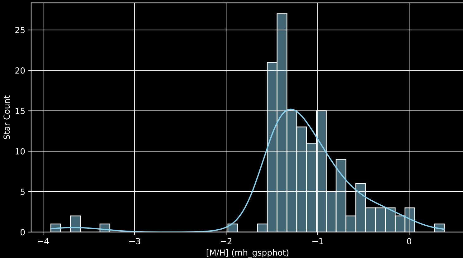
Gaia Cluster: [FSR_0442 [M/H] (mh_gspphot) (n= 145)
