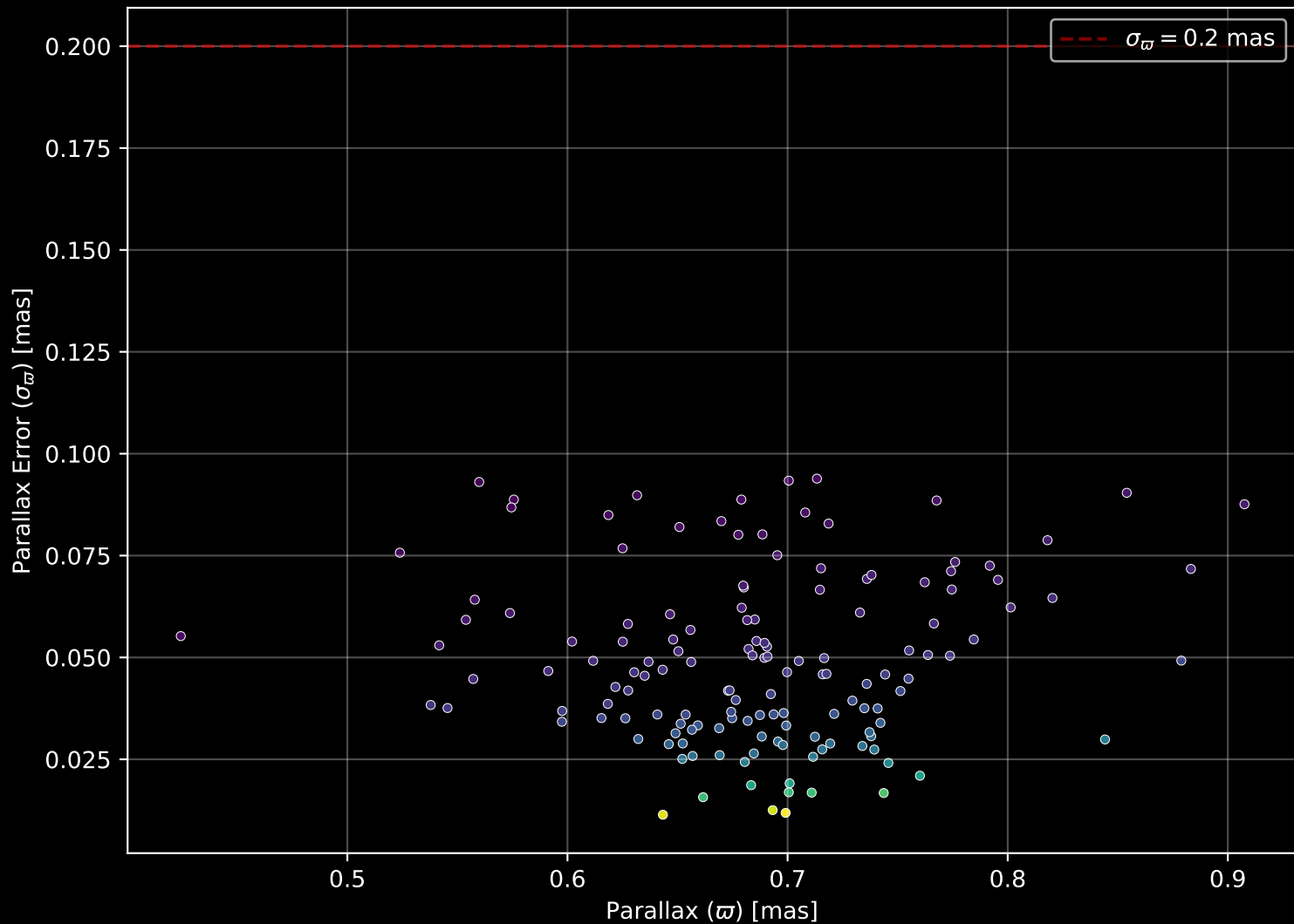
Gaia Cluster: [FSR_0442] Parallax Quality (n= 145)
