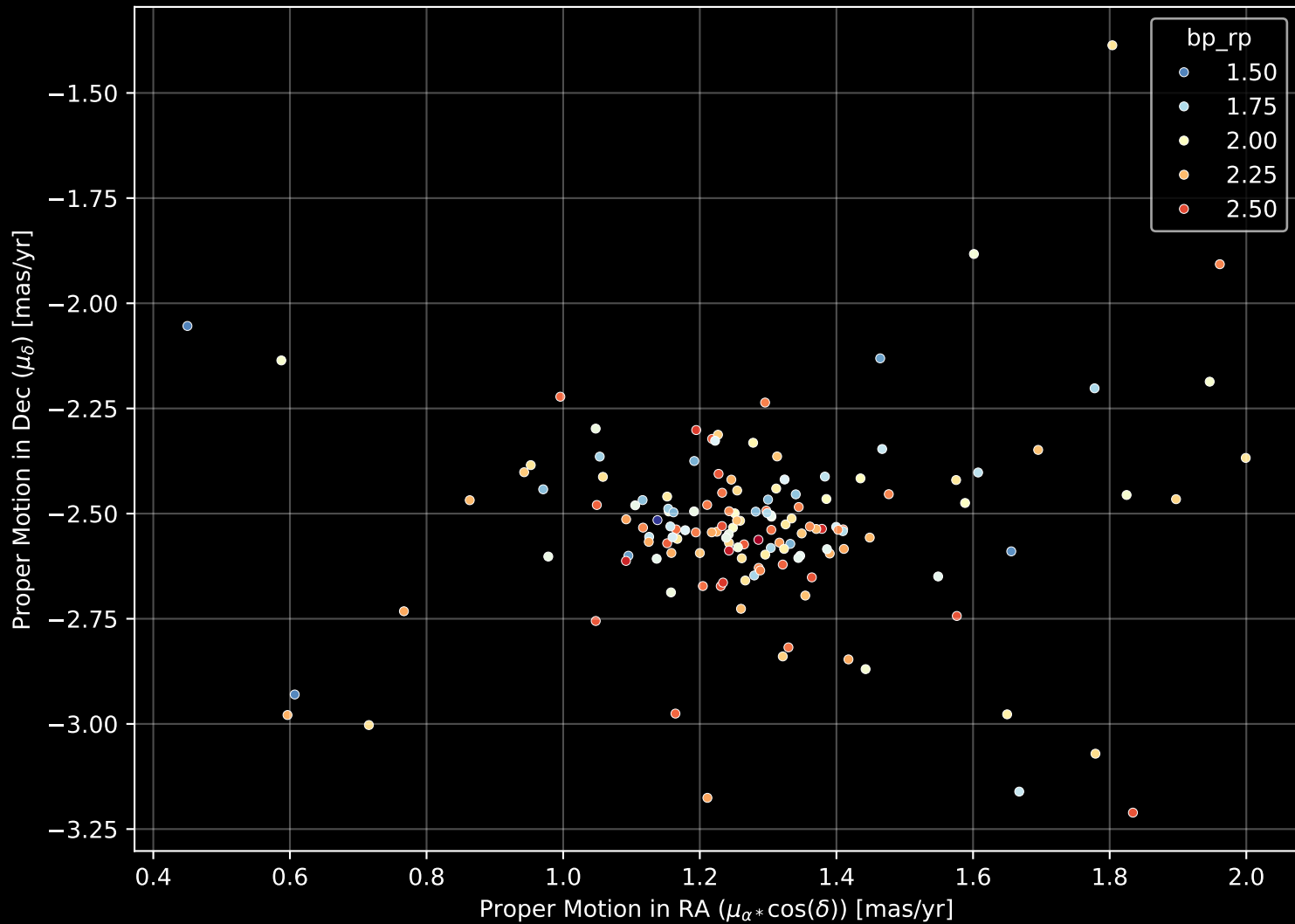
Gaia Cluster: [FSR_0442] Proper Motion Diagram (n= 145)
