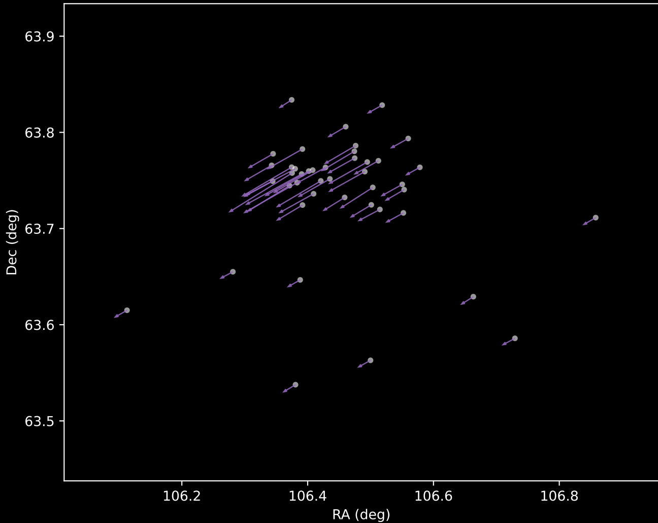
Gaia DR3 Cluster 8 Proper Motion Vectors (n=43)
