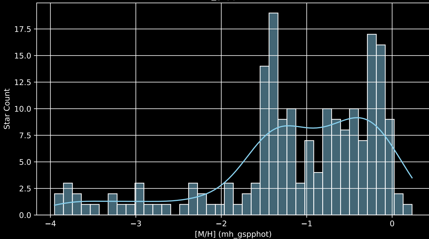
Gaia Cluster: [FSR_0494 [M/H] (mh_gspphot) (n= 191)
