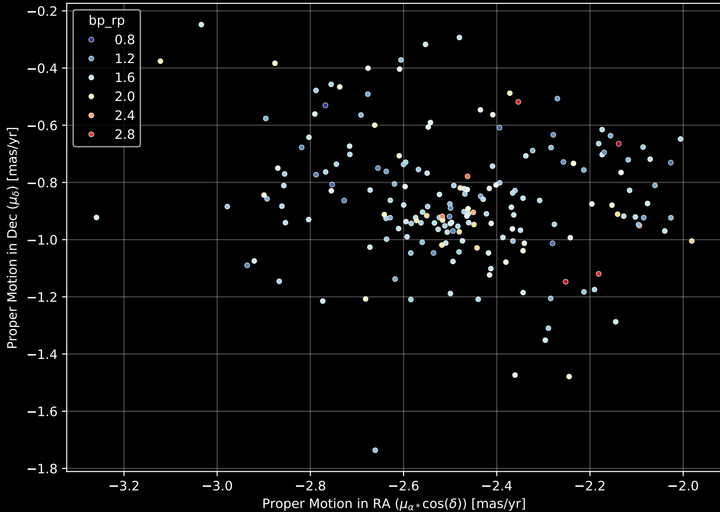
Gaia Cluster: [FSR_0494] Proper Motion Diagram (n= 191)
