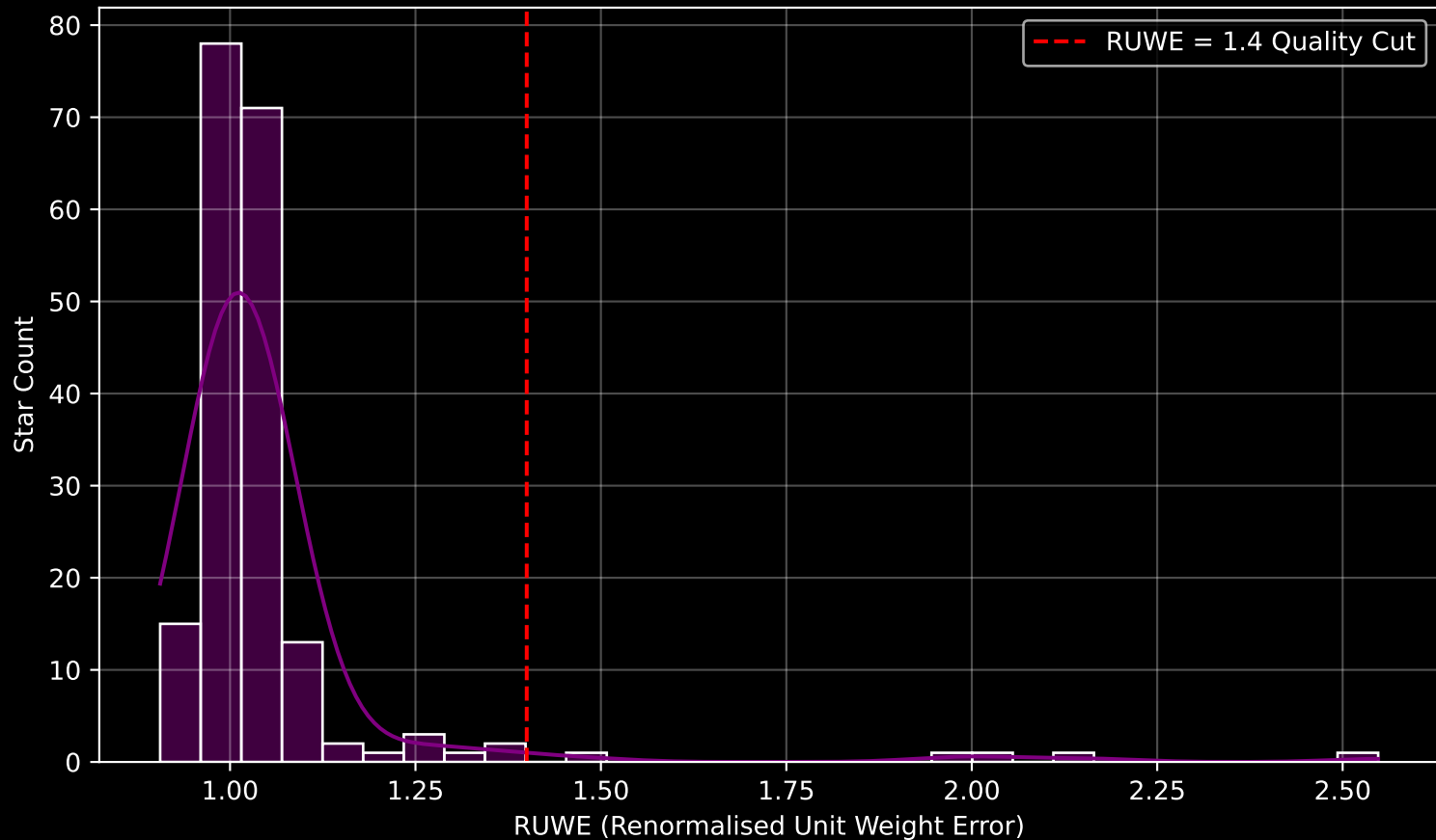
Gaia Cluster: [FSR_0494] RUWE Distribution (n= 191)
