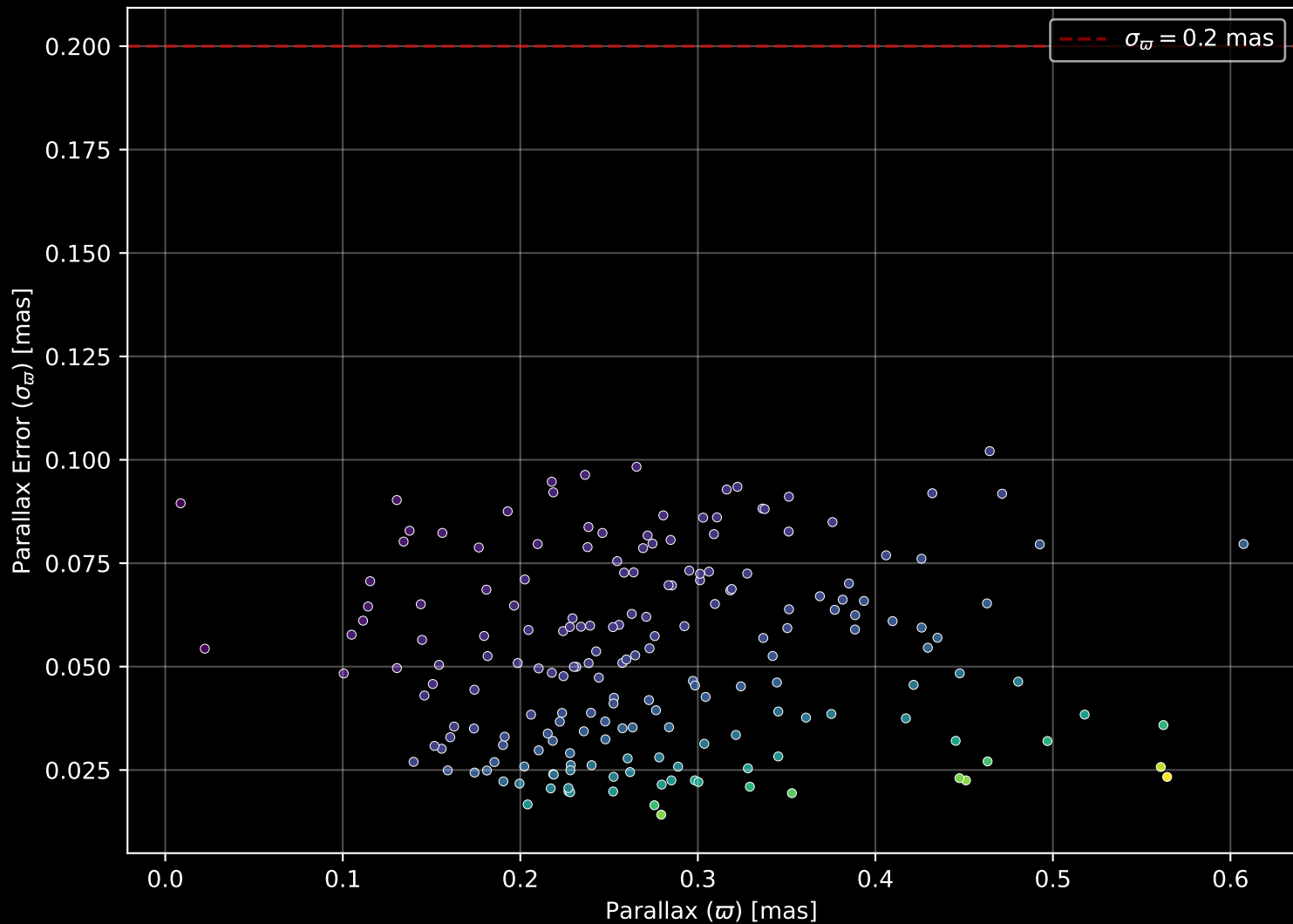
Gaia Cluster: [FSR_0494] Parallax Quality (n= 191)
