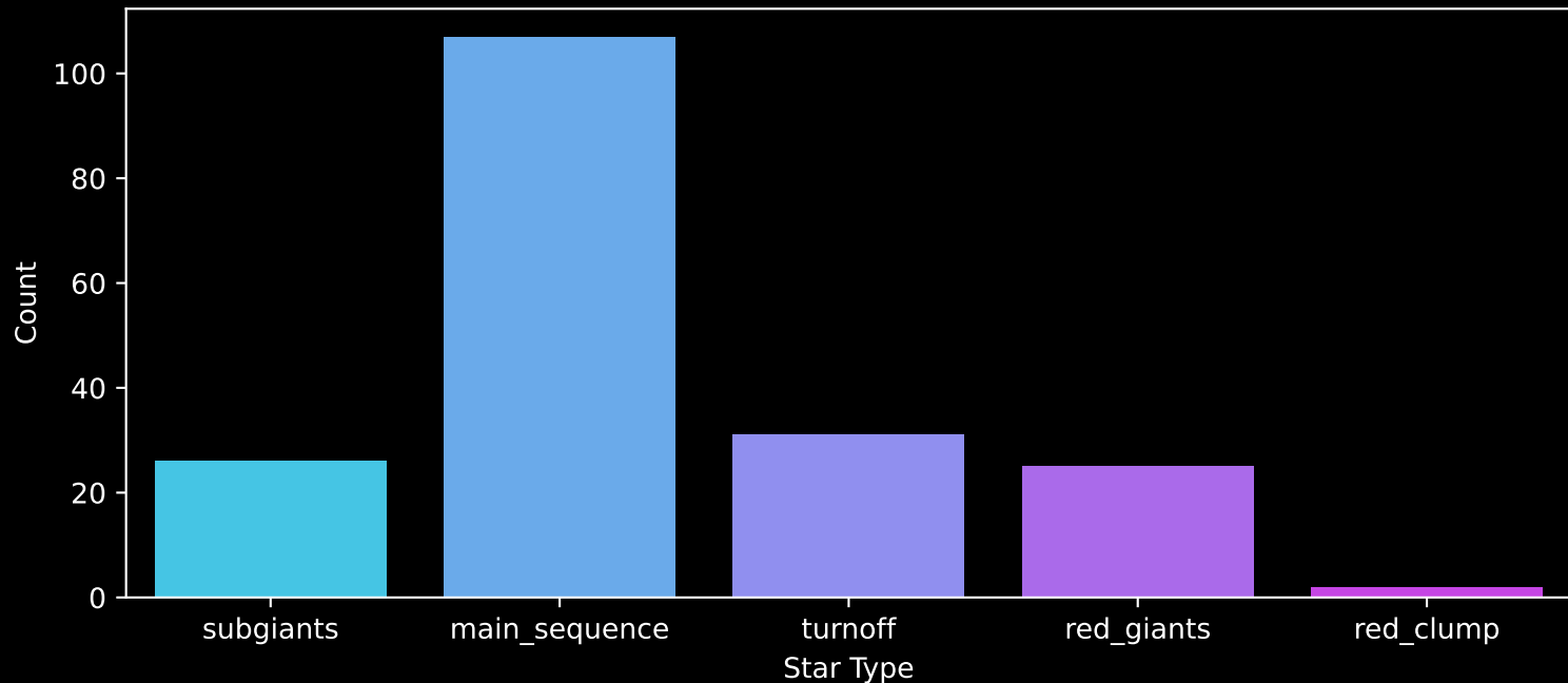
Gaia Cluster: [FSR_0494] Count plot of Star Type
