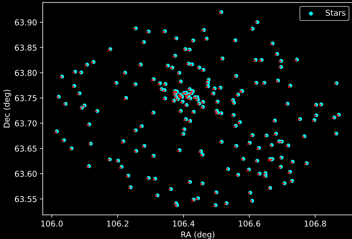
Gaia Cluster: [FSR_0494] Proper Motion Vectors for Gaia Star Field (n= 191)
