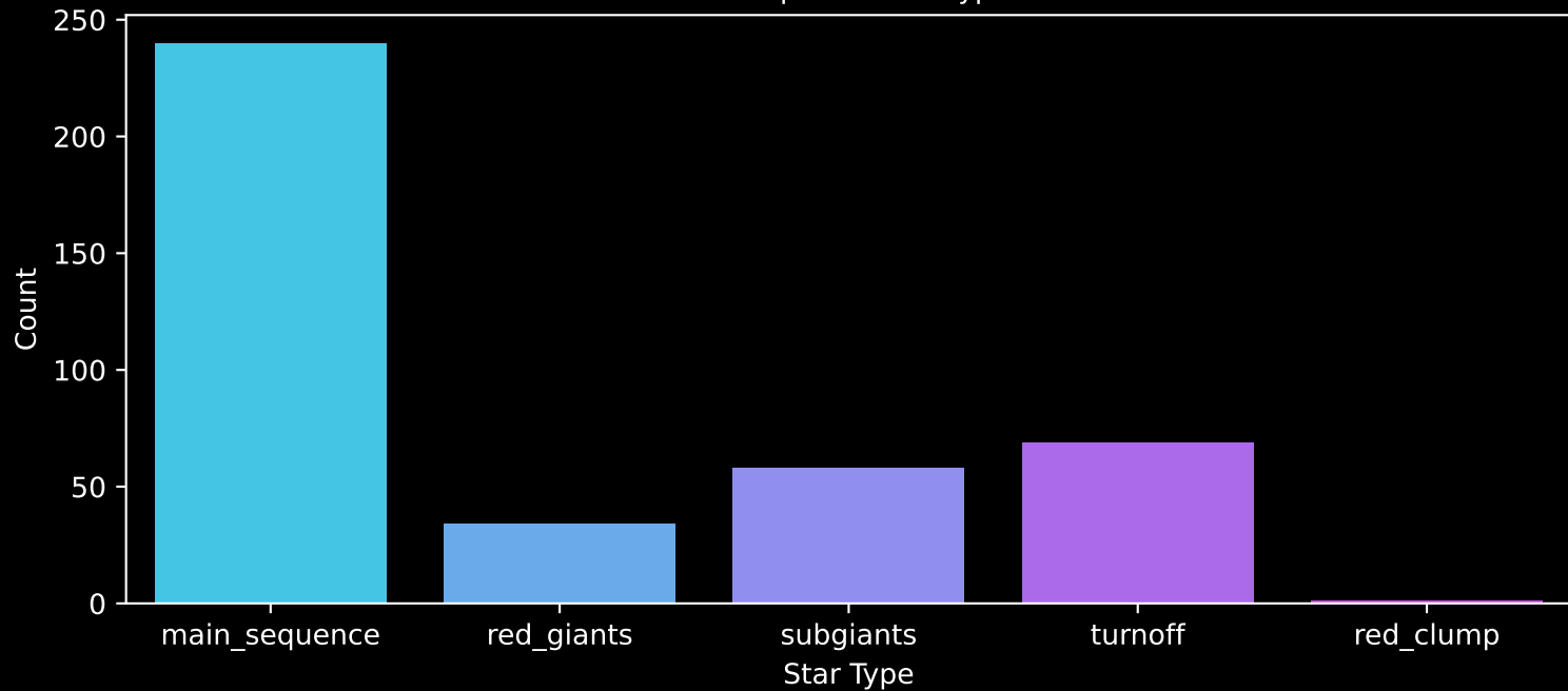
Gaia Cluster: [FSR_0519] Count plot of Star Type
