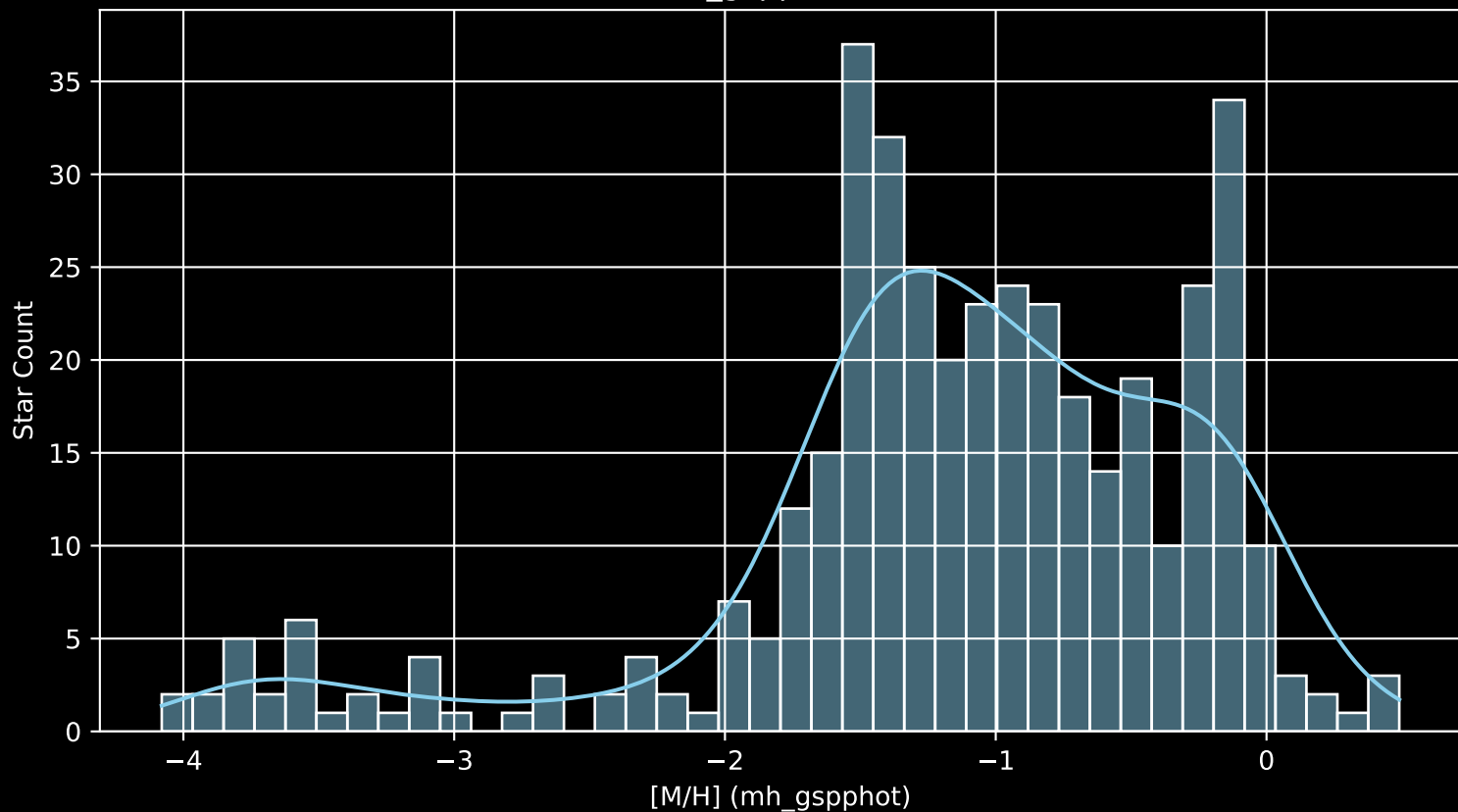
Gaia Cluster: [FSR_0519 [M/H] (mh_gspphot) (n= 400)
