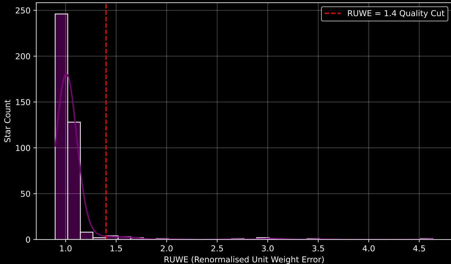
Gaia Cluster: [FSR_0519] RUWE Distribution (n= 400)
