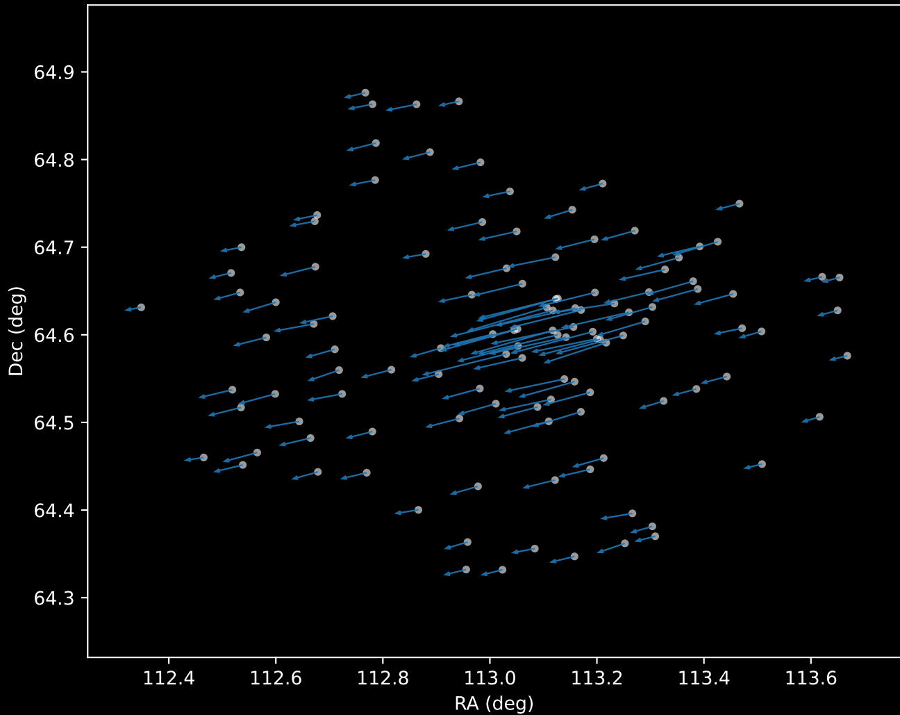
Gaia DR3 Cluster 20 Proper Motion Vectors (n=118)
