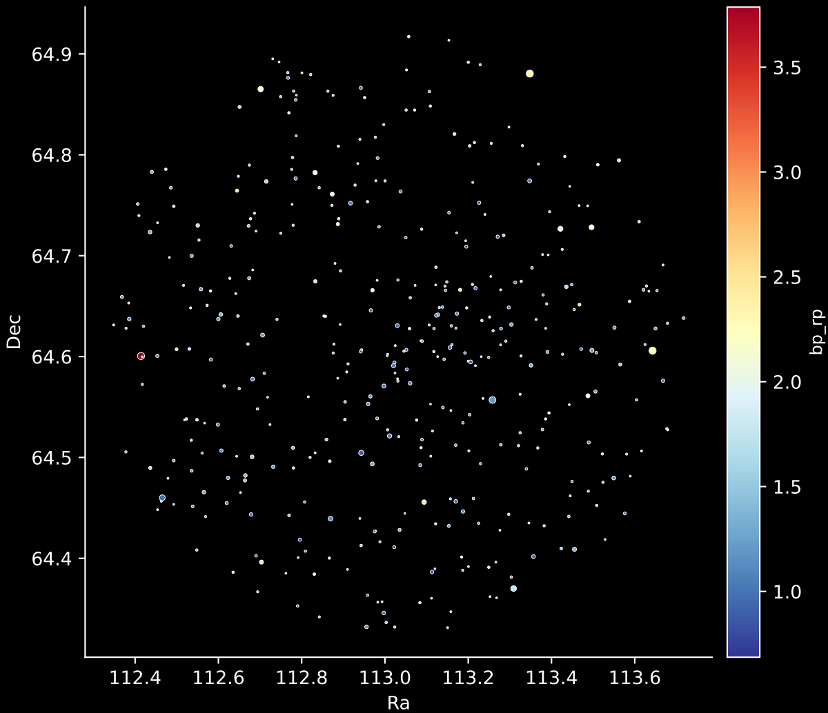
Gaia Cluster: [FSR_0519] Stars: 402
