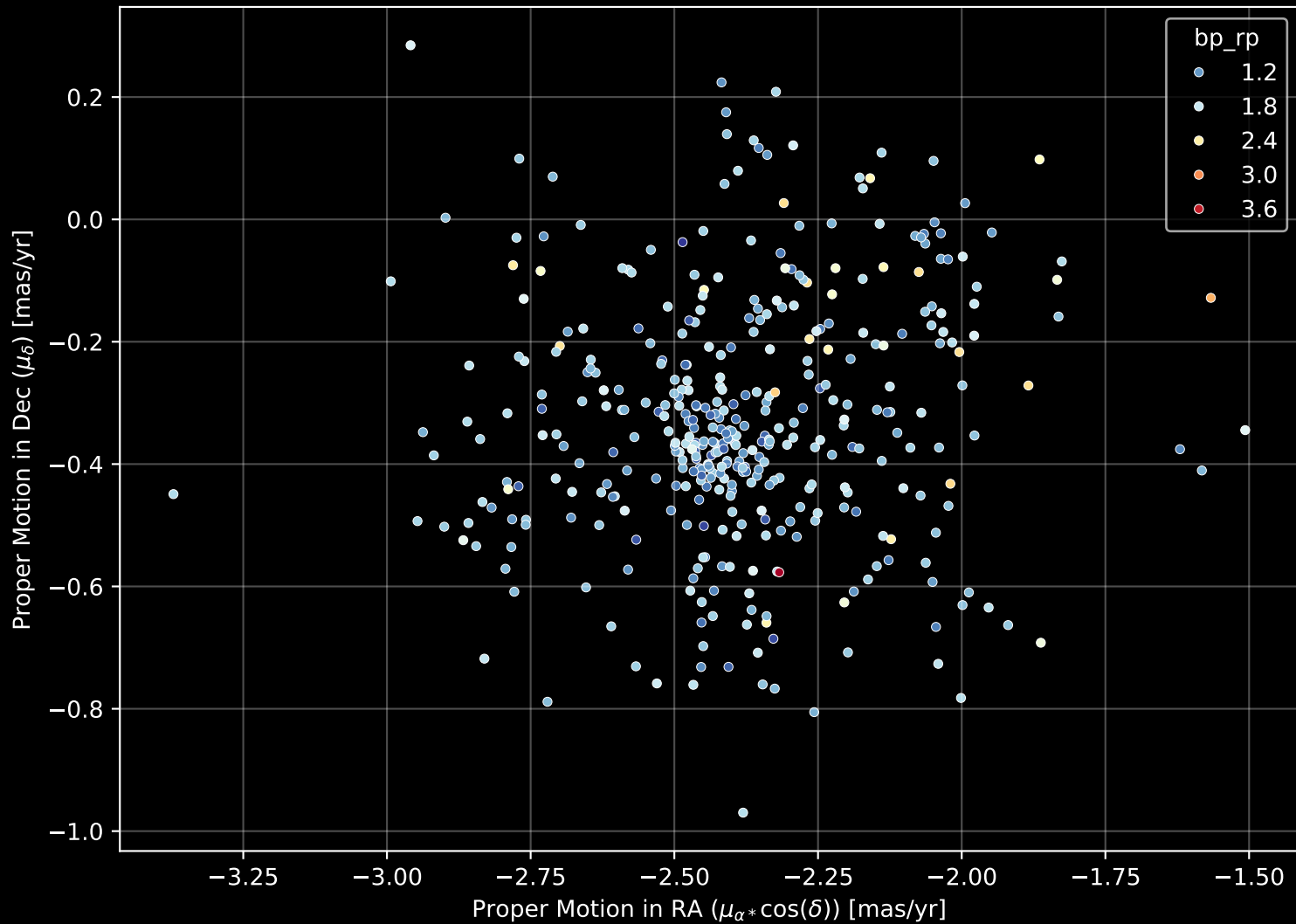
Gaia Cluster: [FSR_0519] Proper Motion Diagram (n= 402)
