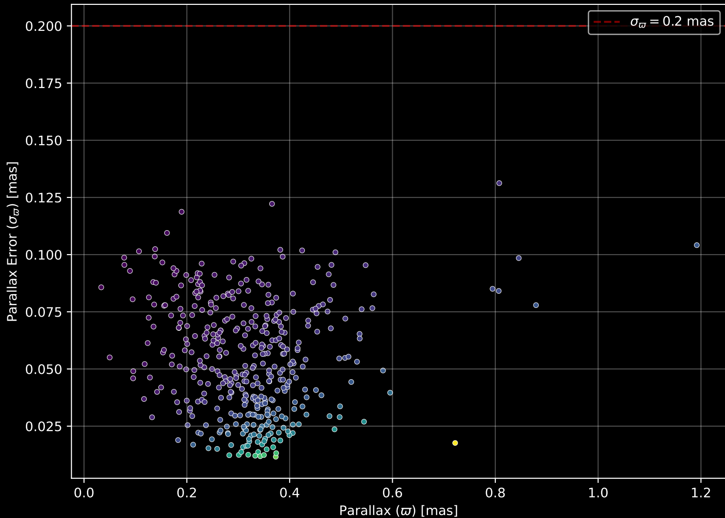
Gaia Cluster: [FSR_0519] Parallax Quality (n= 402)
