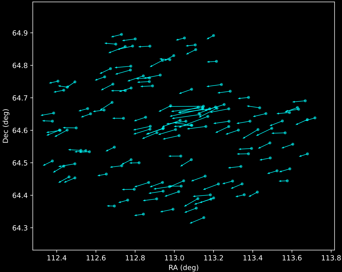
Gaia DR3 Noise Stream Proper Motion Vectors (n=136)
