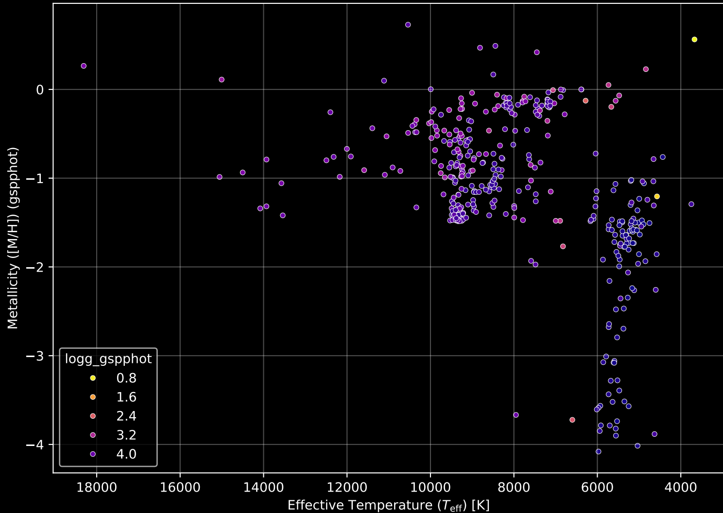
Gaia Cluster: [FSR_0519] Stellar Population Parameters (n= 402)
